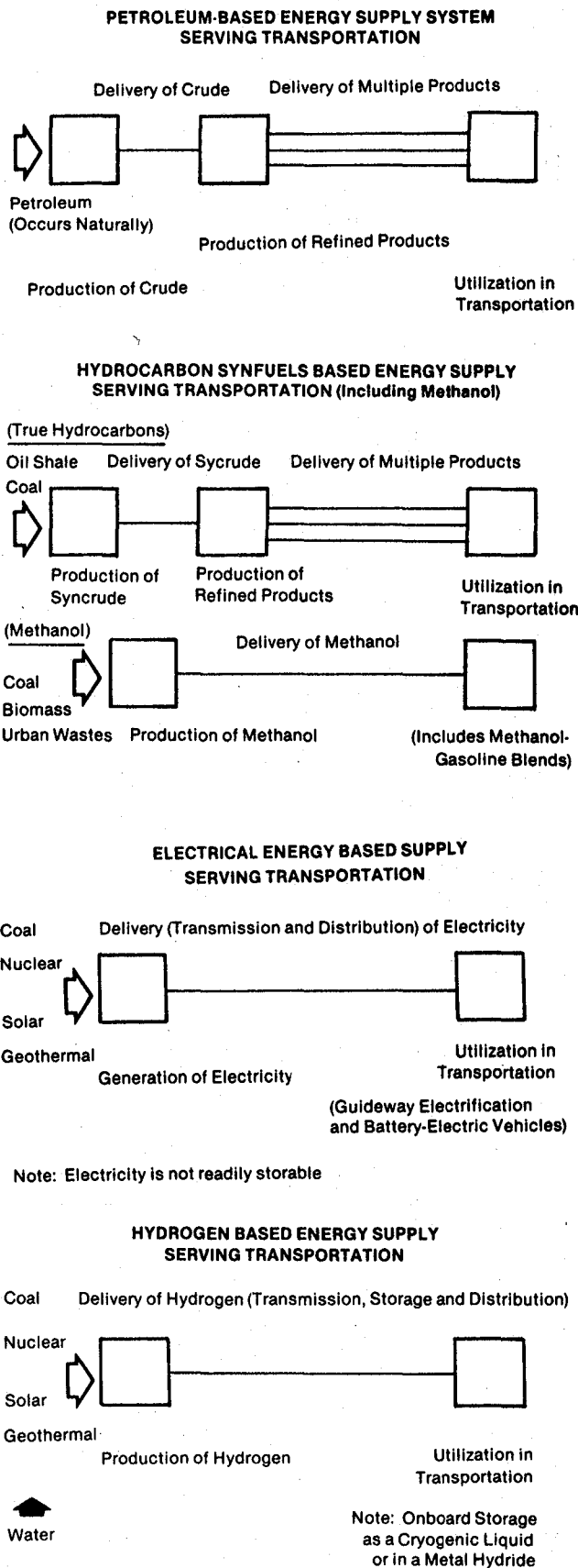
Figure 2 Present and Future Energy Systems Serving Transportation
