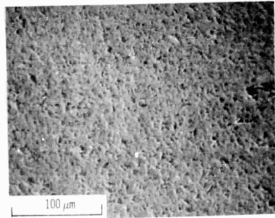
TEST BEARING SUSPENDED AFTER 663 hr FROM 49-micron-ABSOLUTE FILTER TESTS WITH CONTAMINATED LUBRICANT (9)
