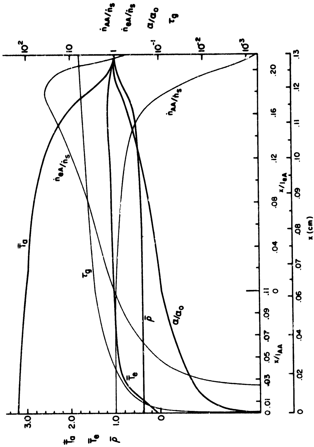
Figure 1. P = 1 cm Hg, Trapped Radiation, Mach 24 Shock Wave in Argon: \rho_0 = 2.285 \times 10^{-4} gm/cm 3 , T_0 = 16,828 K, and \alpha_0 = 0.449 .
