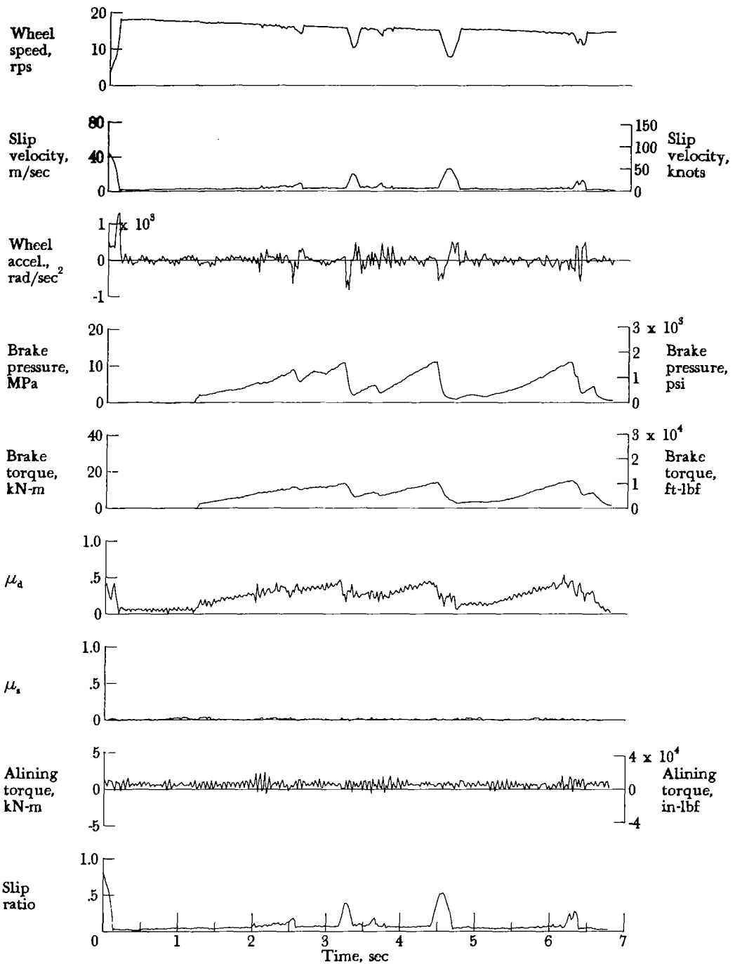
Figure A35.- Time histories for run 35. Nominal carriage speed, 97 knots; vertical load, 69.8 kN (15 700 lbf); yaw angle, 0°; brake pressure, 13 MPa (1950 psi); tire condition, new; surface condition, alternating dry and damp at 30.5-m (100-ft) intervals.
