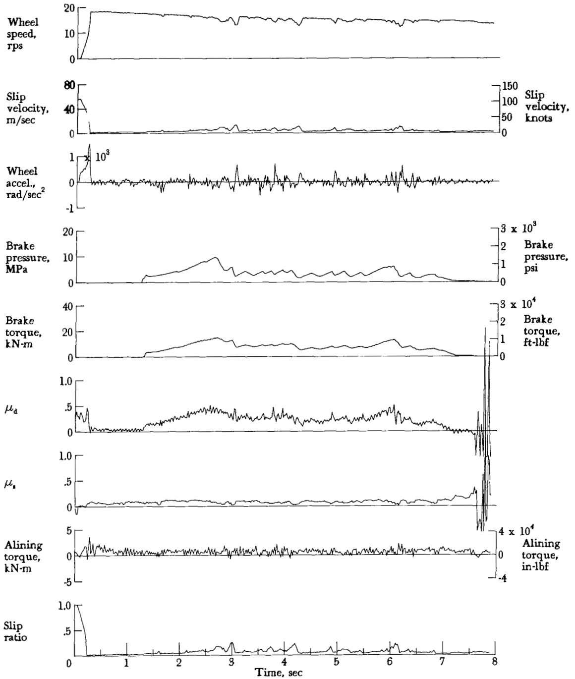
Figure A47.- Time histories for run 47. Nominal carriage speed, 95 knots; vertical load, 69.8 kN (15 700 lbf); yaw angle, 1°; brake pressure, 13 MPa (1850 psi); tire condition, new; surface condition, damp.
