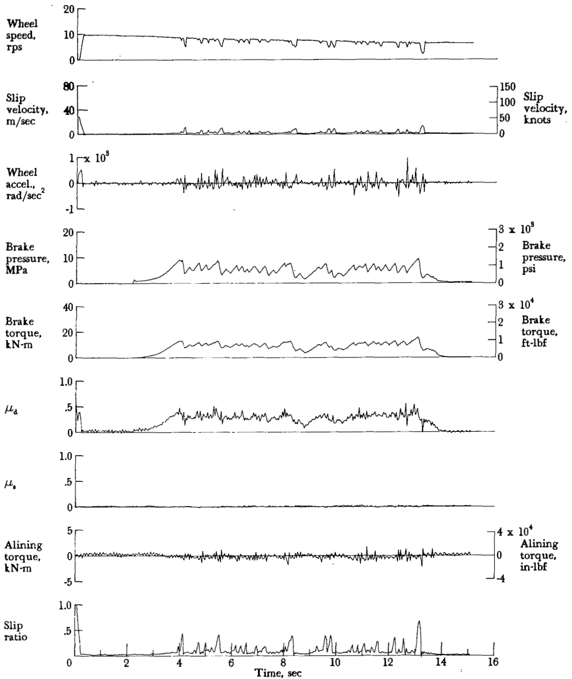
Figure A73.- Time histories for run 73. Nominal carriage speed, 44 knots; vertical load, 69.6 kN (15 600 lbf); yaw angle, 0°; brake pressure, 13 MPa (1900 psi); tire condition, worn; surface condition, damp.
