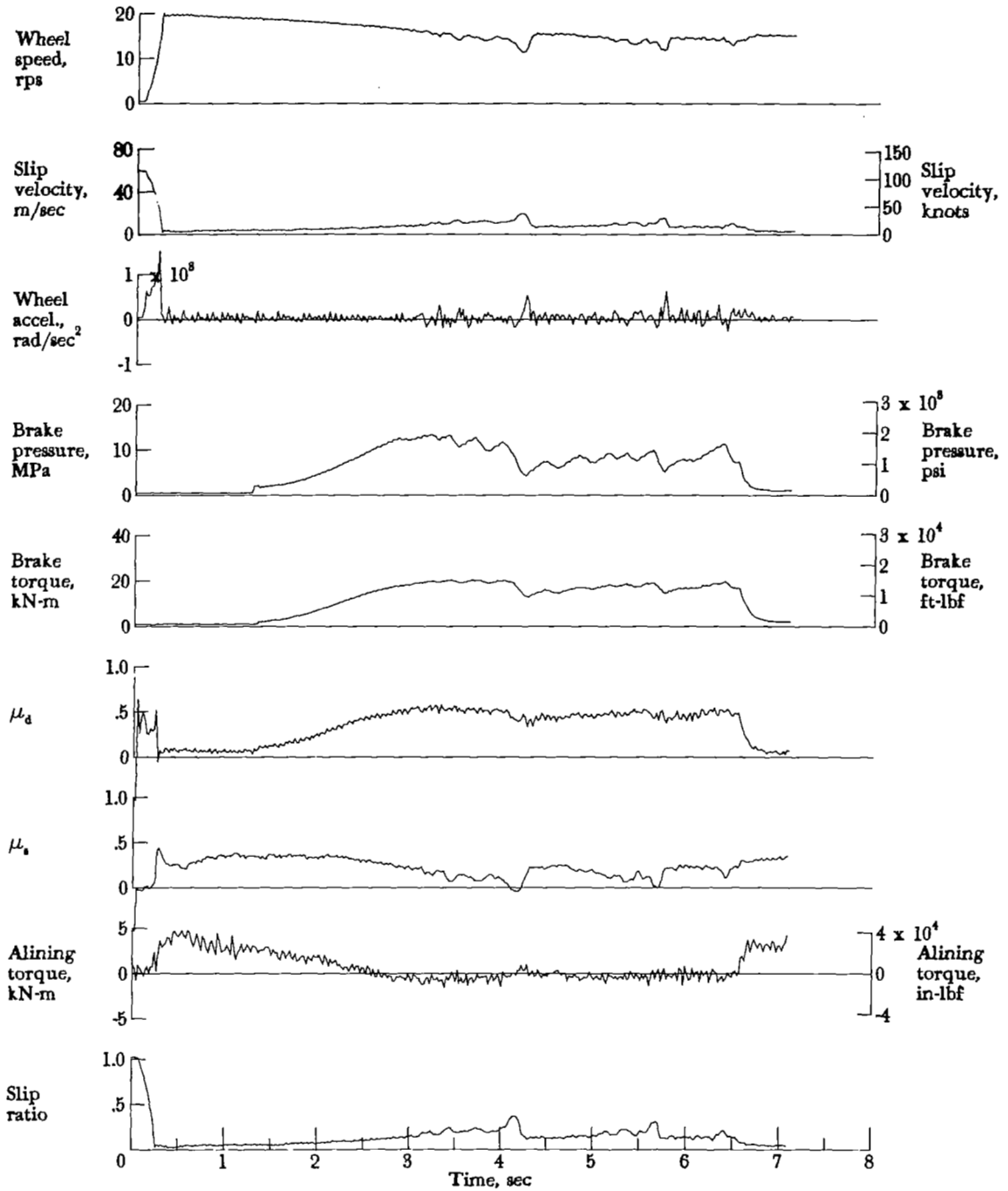
Figure A83.- Time histories for run 83. Nominal carriage speed, 97 knots; vertical load, 72.9 kN (16 400 lbf); yaw angle, 6°; brake pressure, 13 MPa (1950 psi); tire condition, worn; surface condition, dry.
