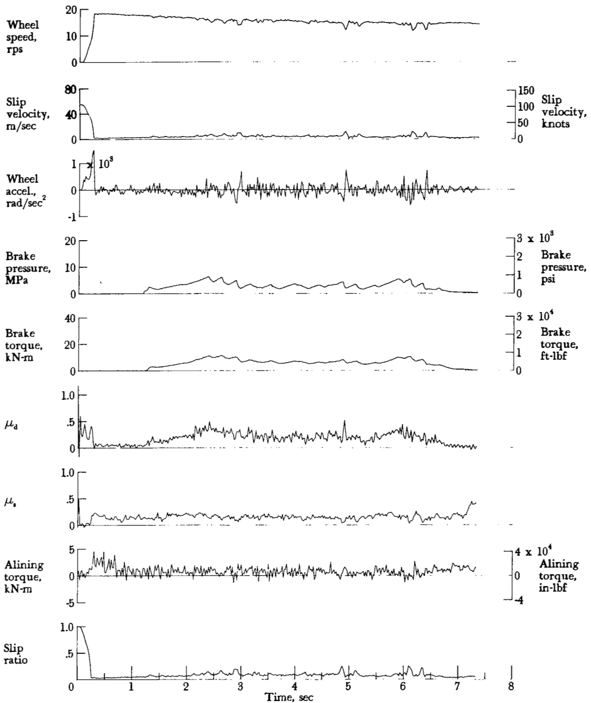
Figure A57.- Time histories for run 57. Nominal carriage speed, 96 knots; vertical load, 69.8 kN (15 700 lbf); yaw angle, 3^\circ ; brake pressure, 13 MPa (1850 psi); tire condition, new; surface condition, damp.
