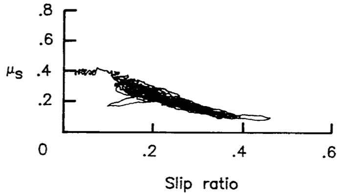
Figure 20.- Interaction between braking and cornering. Run 62; nominal carriage speed, 56 knots; vertical load, 71 kN (15 900 lbf); yaw angle, 6^\circ ; tire condition, new; surface condition, dry.
