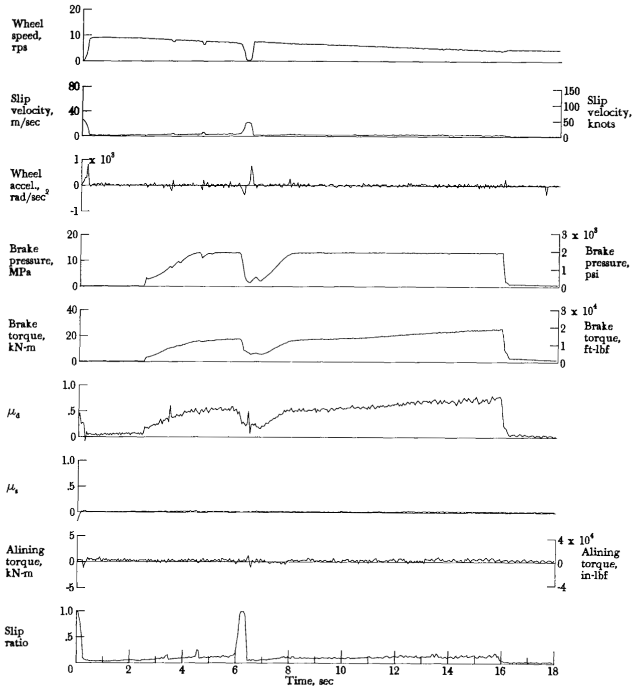
Figure A39.- Time histories for run 39. Nominal carriage speed, 36 knots; vertical load, 68.5 kN (15 400 lbf); yaw angle, 0°; brake pressure, 13 MPa (1950 psi); tire condition, new; surface condition, flooded/dry.
