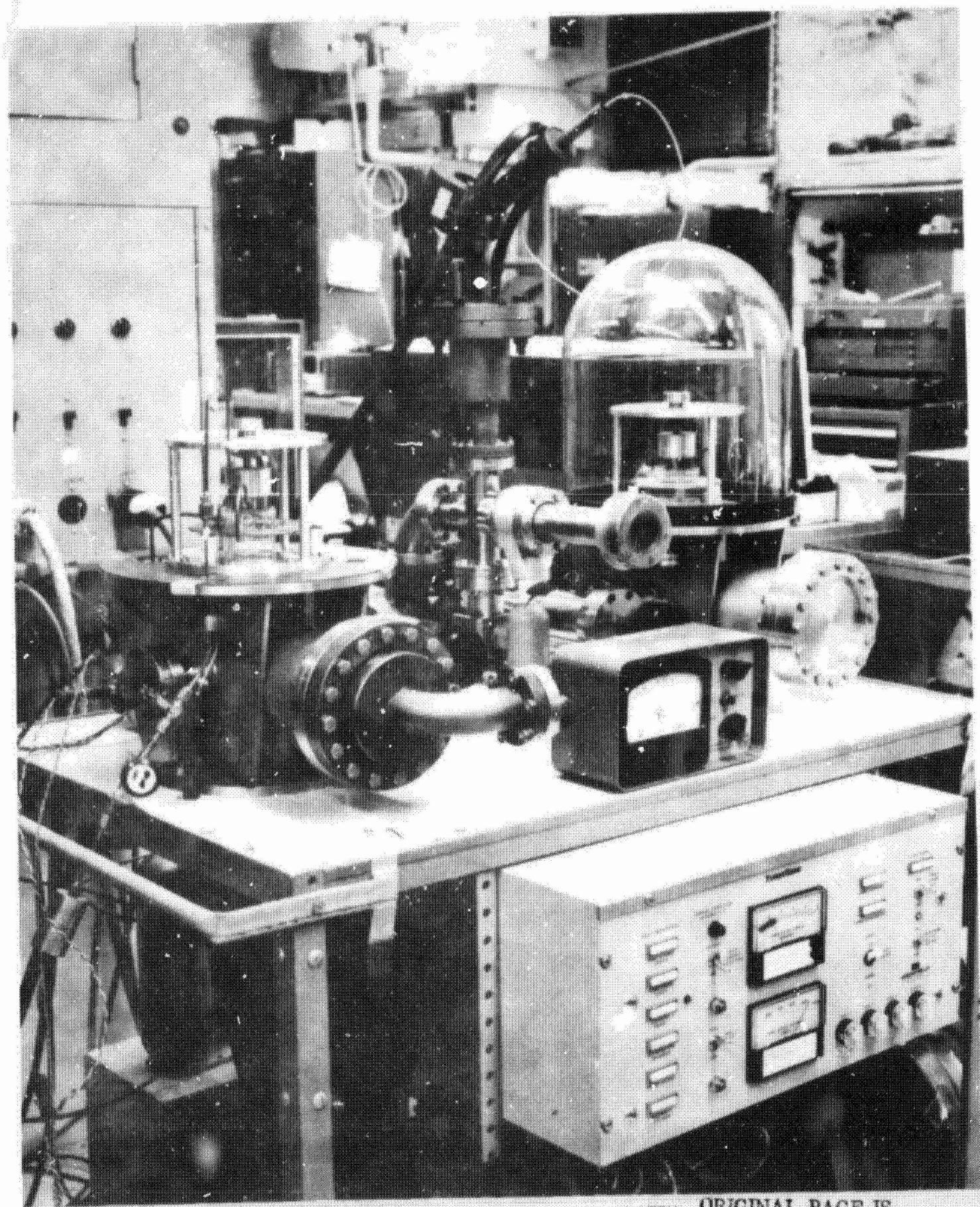
FIG. 1. HYDROGEN DISSOCIATION TEST SYSTEM ORIGINAL PAGE IS OF POOR QUALITY
