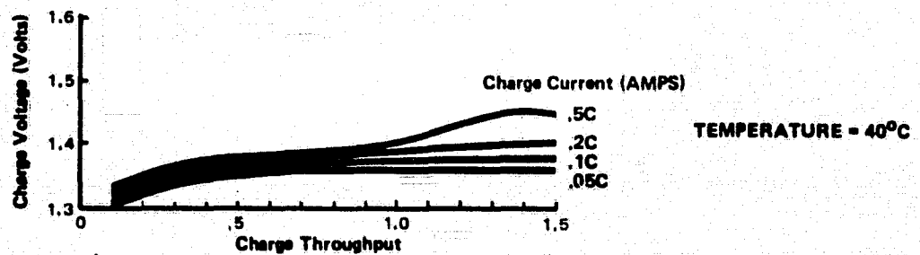
Exhibit 2.7: Example of Three-Dimensional Performance Curves (NiCd Charge Voltage vs Charge Throughput, Charge Current and Temperature)
