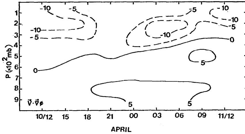
Figure 27. Pressure-time cross section of area averaged generation of kinetic energy. Units are \text{W m}^{-2}/100 \text{ mb} .
