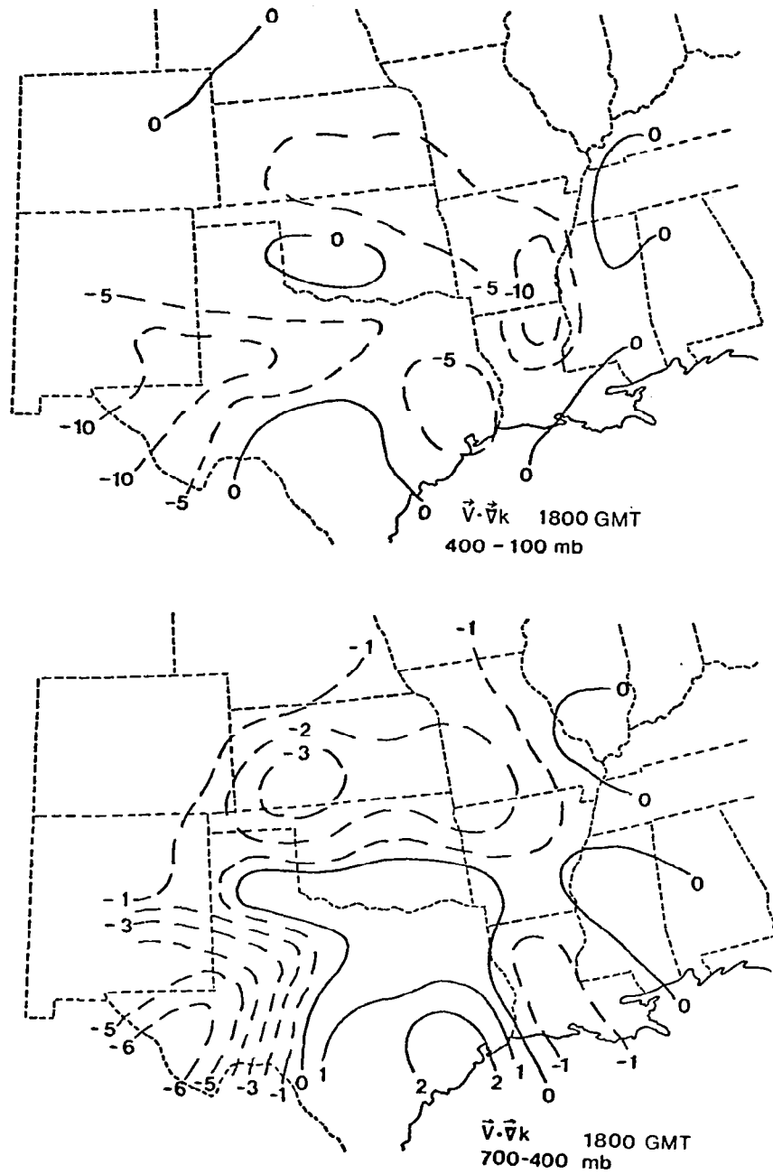
Figure 31. Horizontal fields of kinetic energy advection integrated over the 700-400 mb layer and the 400-100 mb layer for 1800 GMT 10 April 1979. Values are \times 10^4 \text{ W m}^{-2} .
