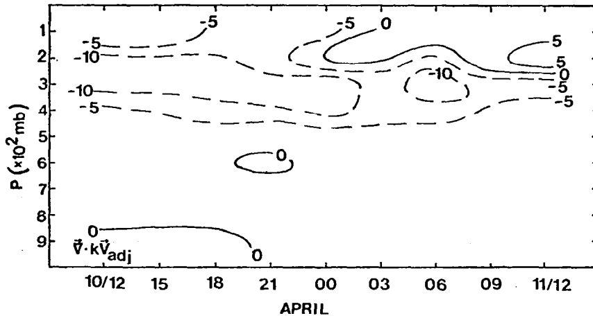
Figure 28. Pressure-time cross section of area averaged adjusted horizontal flux divergence of kinetic energy. Units are \text{W m}^{-2}/100 \text{ mb} .
