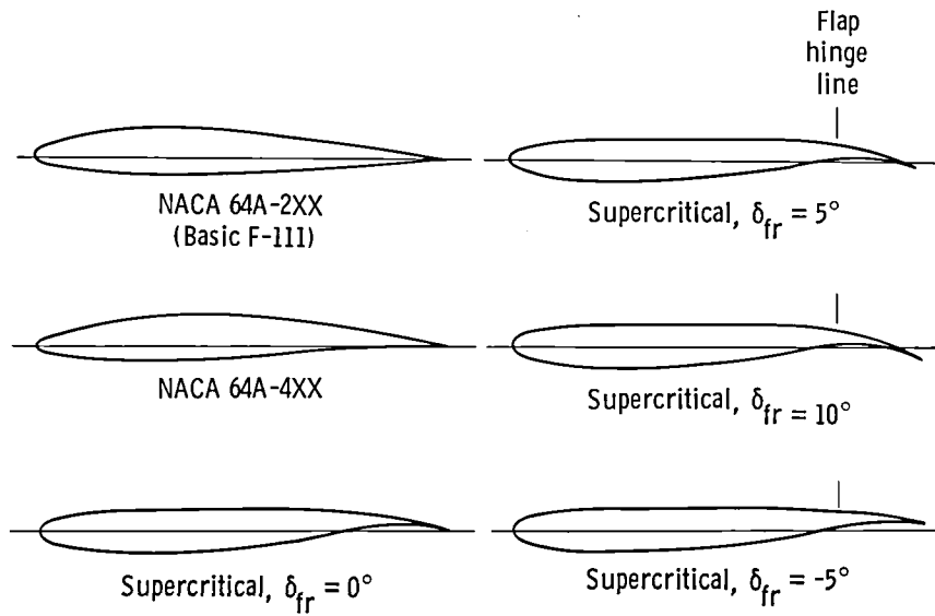
Figure 5. Airfoil shapes for exploratory investigation.
