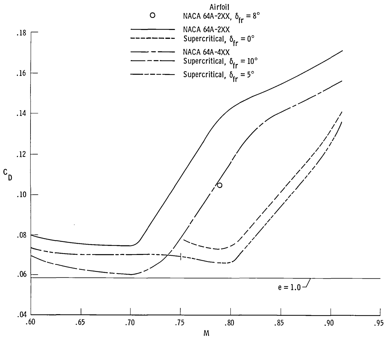
Figure 7. Effect of airfoil geometry on the trimmed maneuver drag characteristics. \Lambda = 26^\circ , C_L = 0.90 .
