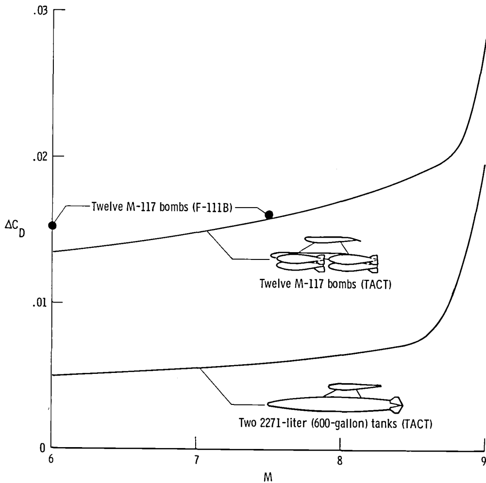
(a) Incremental stores drag.
