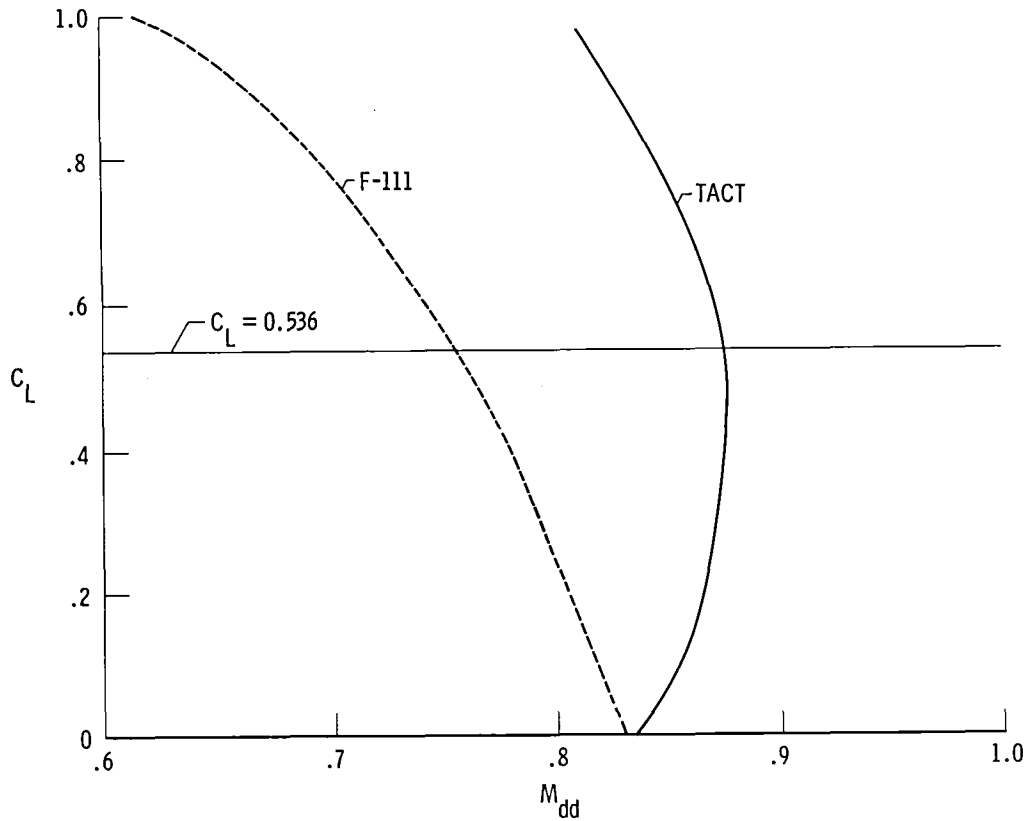
Figure 15. Comparison of F-111 and TACT drag-divergence Mach numbers. \Lambda = 26^\circ .
