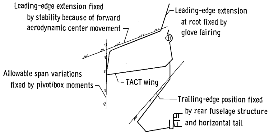
(b) Wing design.
