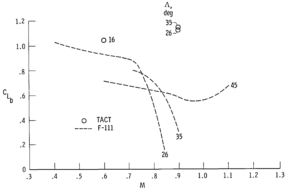
Figure 19. Comparison of buffet onset lift coefficients. \delta_h = 0^\circ .
