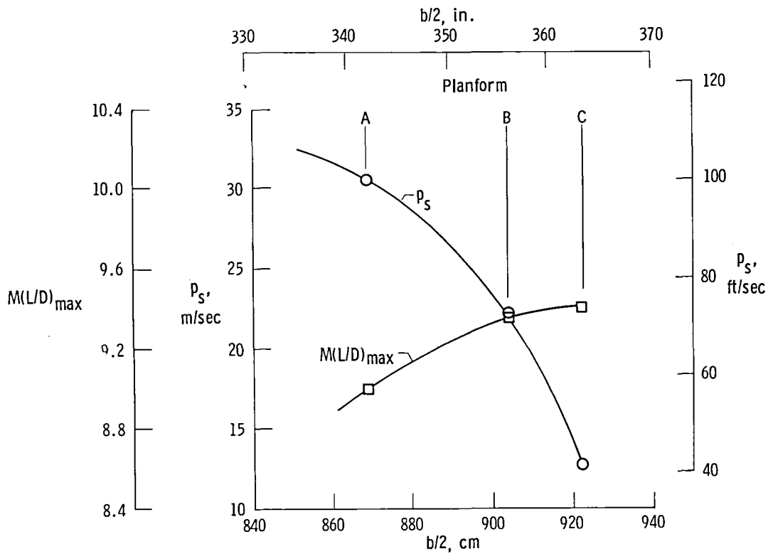
Figure 13. TACT wing planform selection. \Lambda = 16^\circ .
