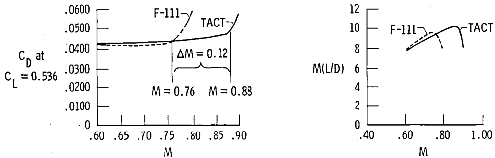
(a) Cruise drag.
