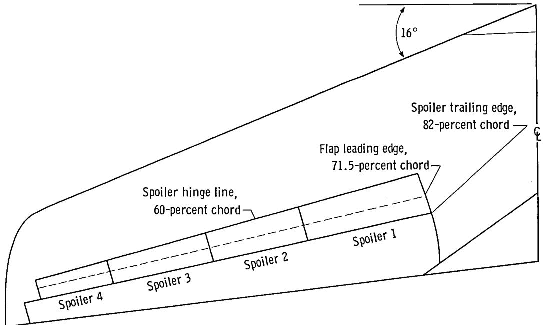
Figure 1. F-111 model wing details.
