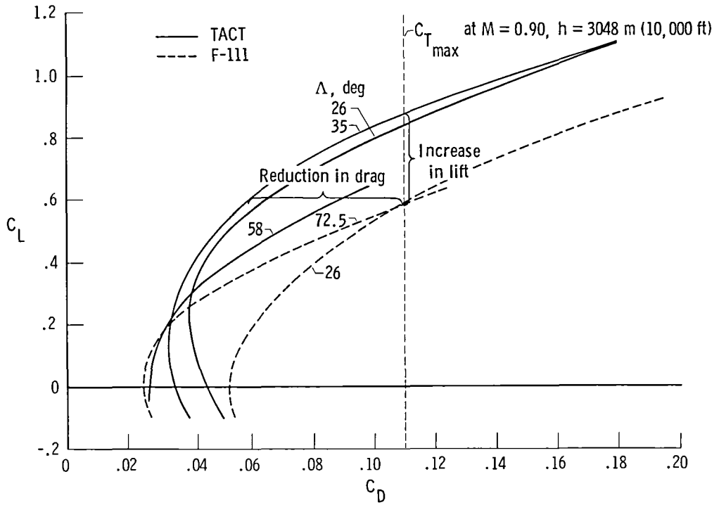
Figure 18. Comparison of F-111 and TACT maneuver drag characteristics. M = 0.90 , \delta_h = 0^\circ .
