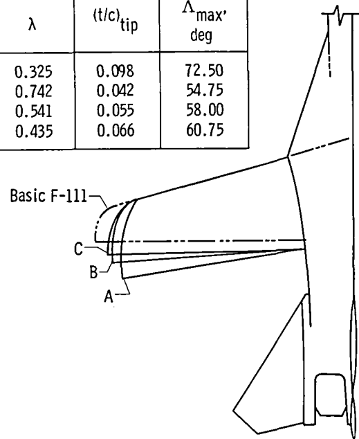
Figure 12. Candidate TACT planforms. \Lambda = 16^\circ .
