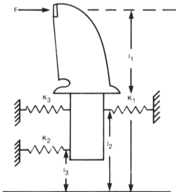
Figure 7. Simple spring model of the pick block showing the effect of preload
