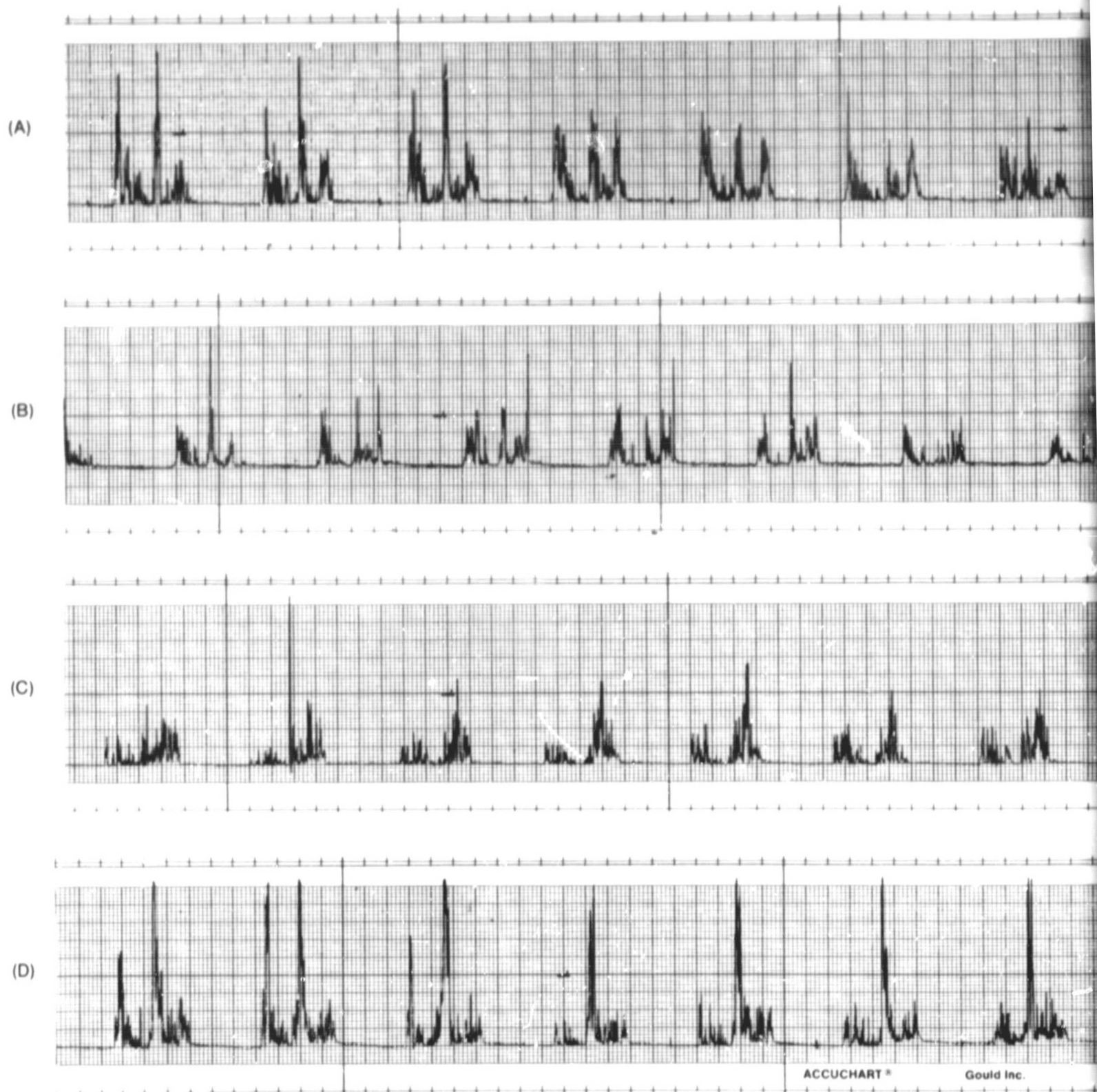
Figure 34. Cutting force signals measured (a) Typical "rock-cutting" signal (b) Typical "coal-cutting" signal (c) Typical signals where the "rock" is (d) Typical signals where the "coal" is
