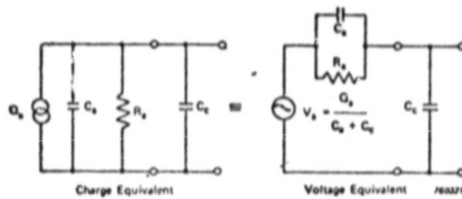
Equivalent circuits of piezoelectric accelerometer with connection cable
