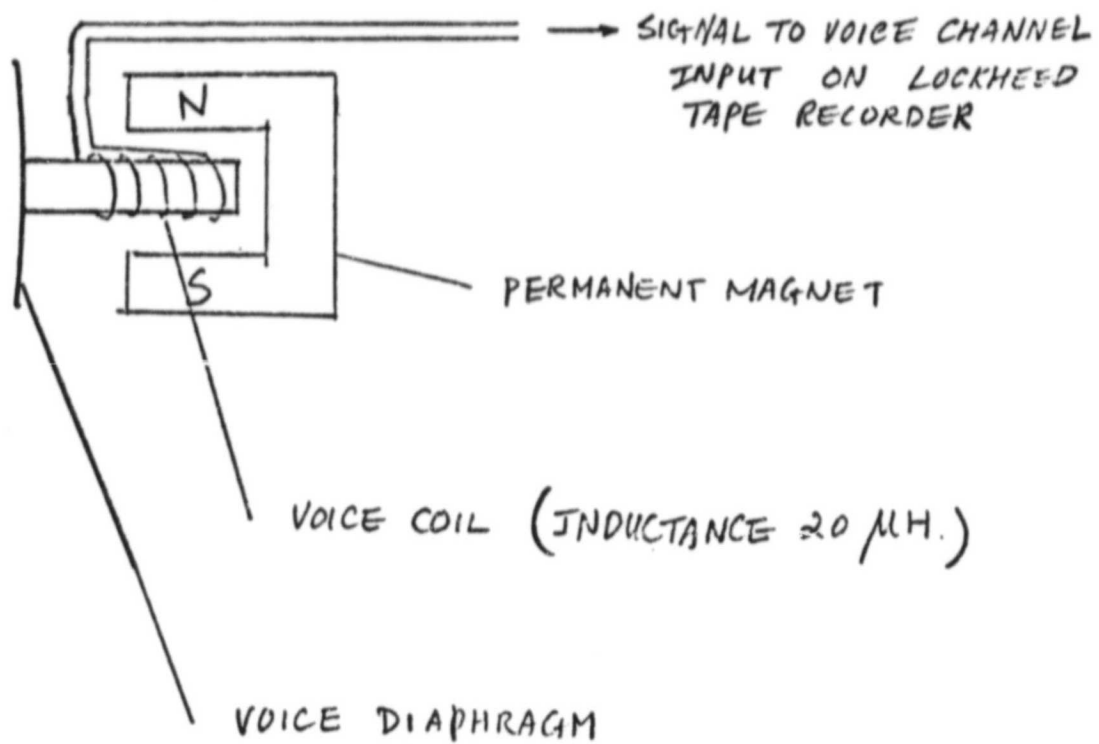
FIGURE 2. Schematic for voice microphone of the tape recorder.
