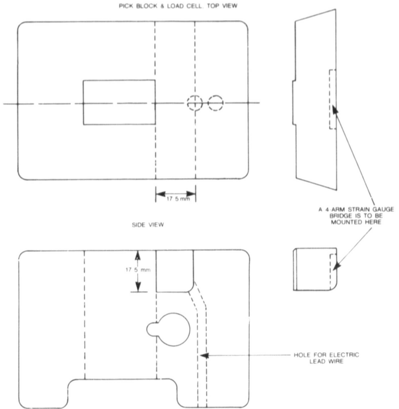
Figure 18. The square short beam load cell and the pick block
