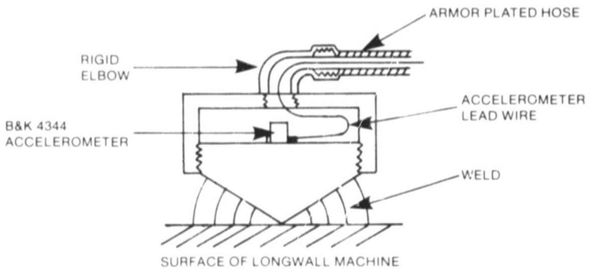
Figure 33. Drawing of accelerometer mounting cone
