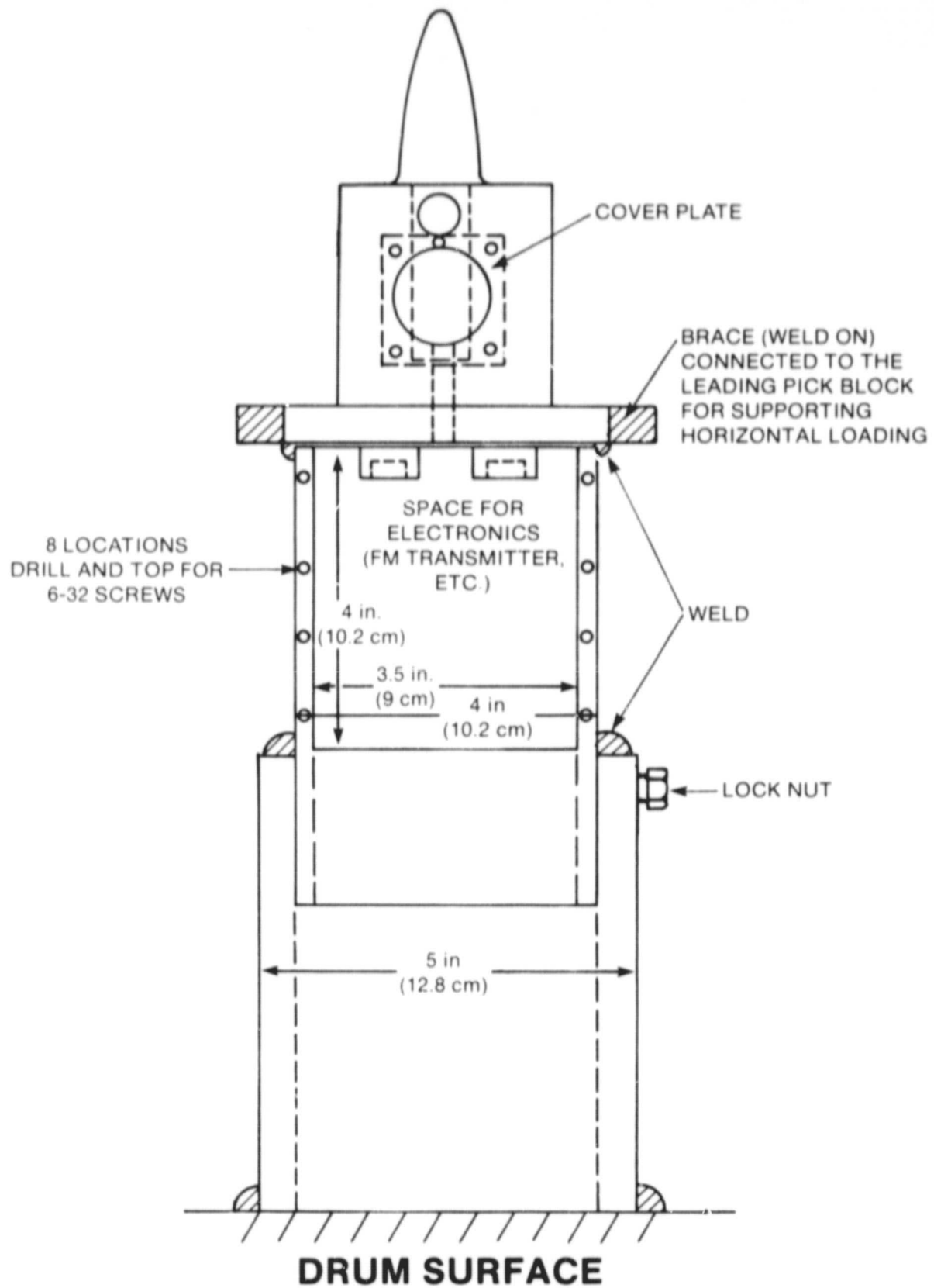
Figure 14. Drawing of mounting fixture for sensitized pick block and transmitter assembly
