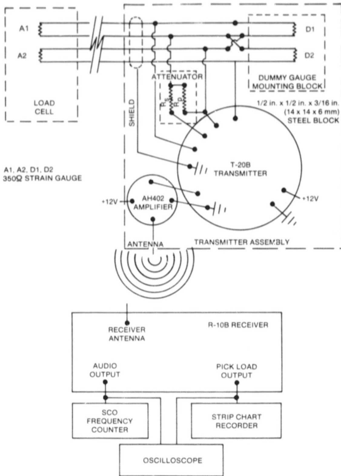
Figure 4. Instrumentation for calibration of the load cell and sensitized pick
