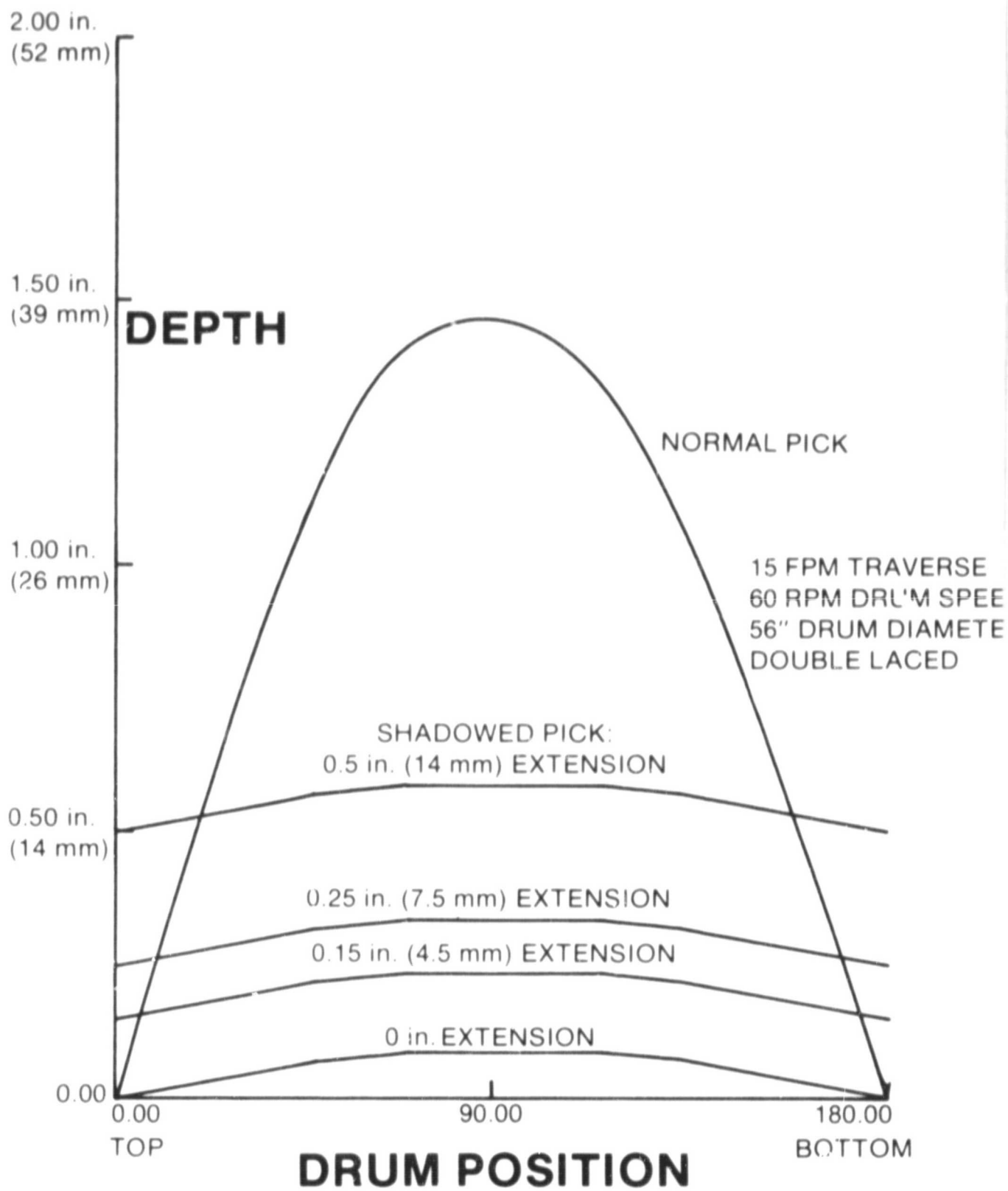
Figure 30. Cutting depth vs. drum position (15° lag shadow pick) Block diagram of sensitized pick processor
