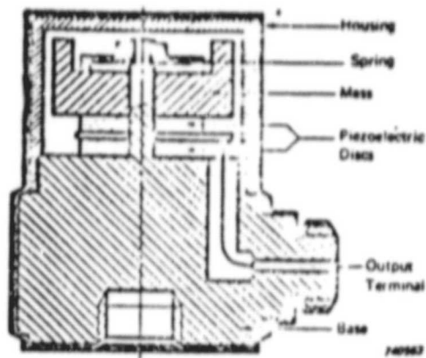
Schematic of piezoelectric accelerometer
