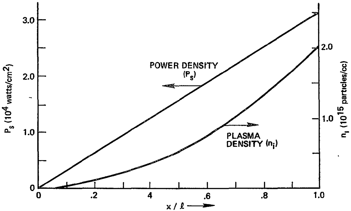
(b) POWER and PLASMA DENSITIES
