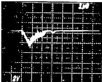
Figure 3-8. Pad Collector Currents Demonstrating Concentration of Blowoff Current in the Direction Towards Arcing Source (10- by 10-inch, 2 mil Kapton Sample)
