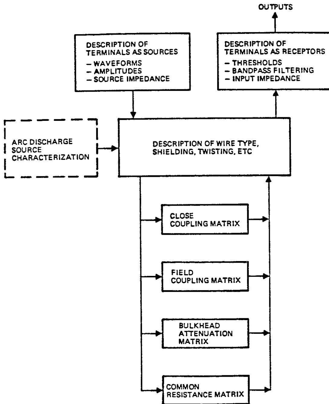
Figure 5-1. SEMCAP Overview
