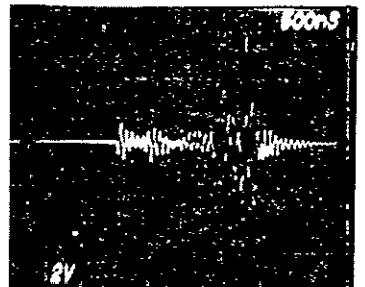
Figure 3-11. Replacement and Side Plate Currents (6- by 6-inch, 2 mil Kapton Sample)
