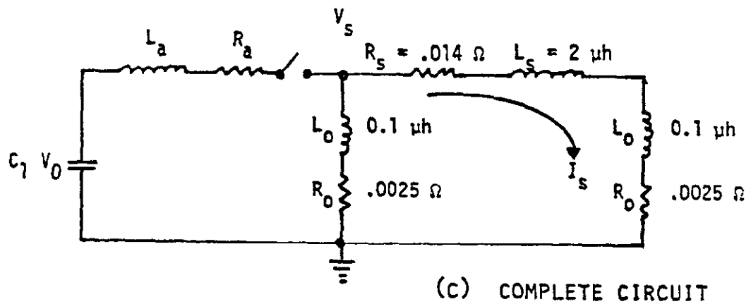
Figure 5-5. Configuration Circuits to be Solved to Determine Arc-to-Shield Currents and Voltages
