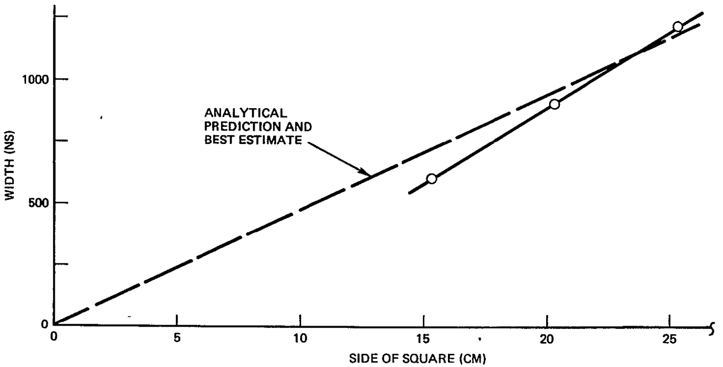
Figure 3-13. Replacement Current Pulswidth versus Side of Square ( R_0 = 1 ohm)
