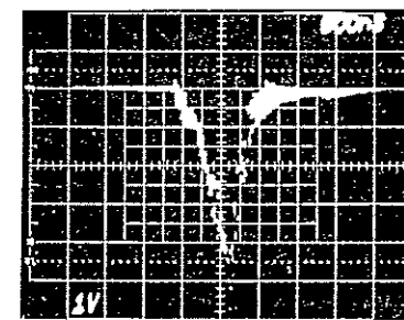
Figure 3-9. Replacement and Collector Ring Waveforms as a Function of Sample Grounding Resistance (8- by 8-inch, 2 mil Kapton Sample)
