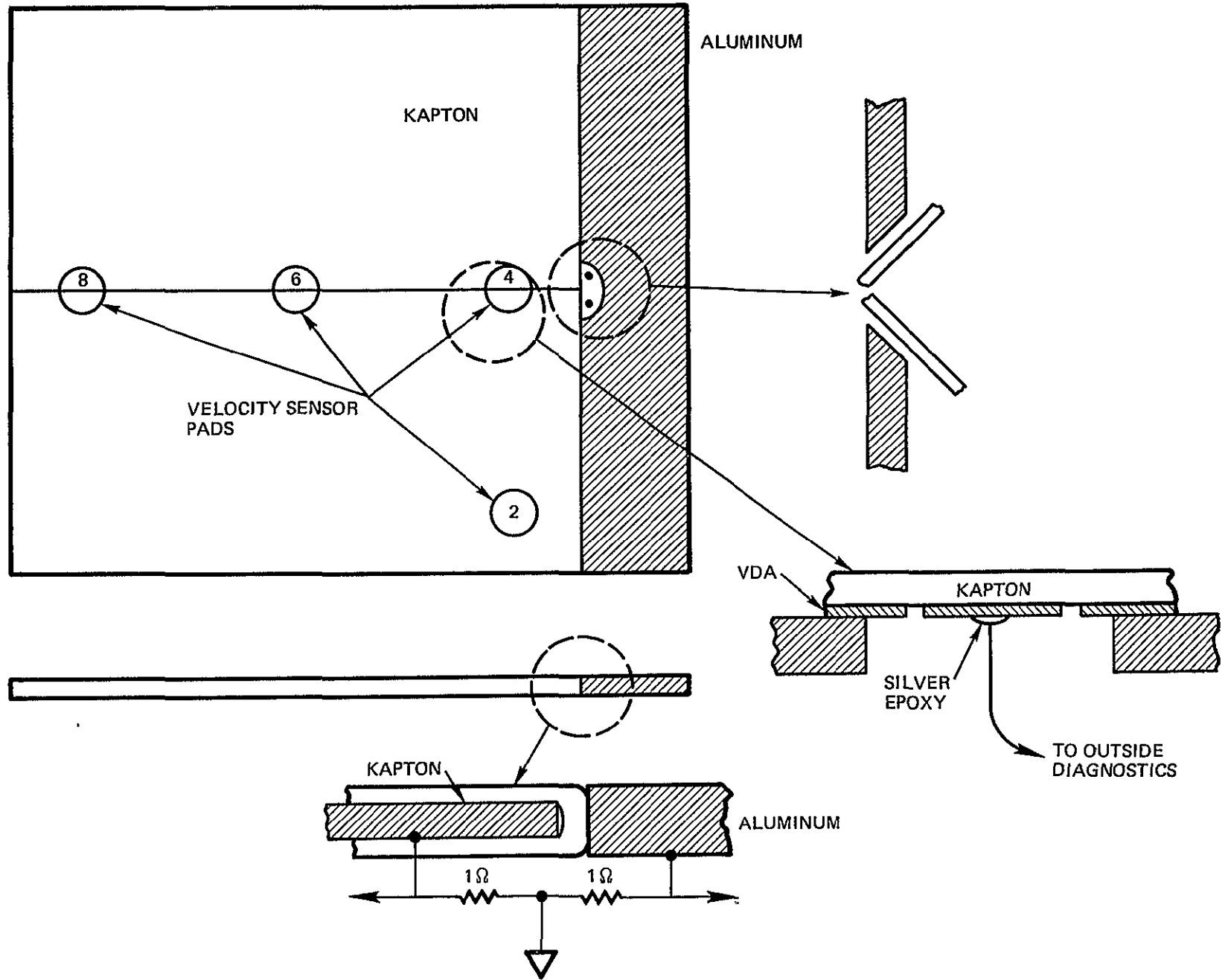
Figure 3-5. Sample Configuration Showing Capacitive Sensor Pads
