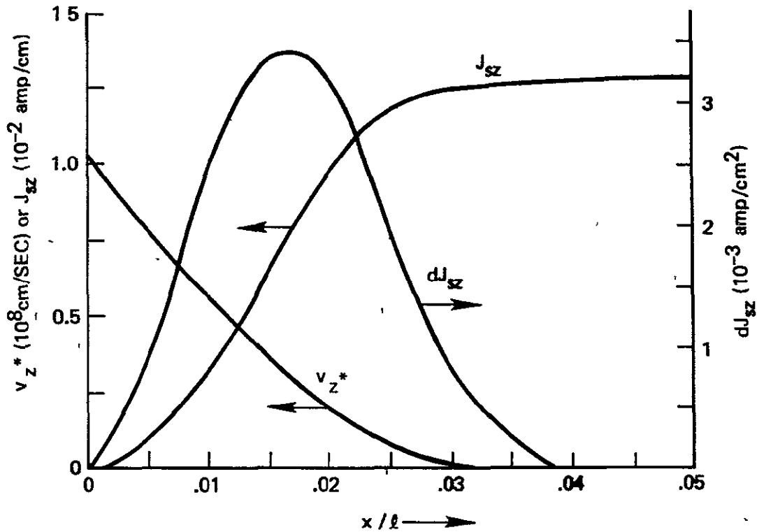
Figure 8. v_z^* , dJ_{sz} and J_{sz} Versus x/l (Shielding by Plasma)
