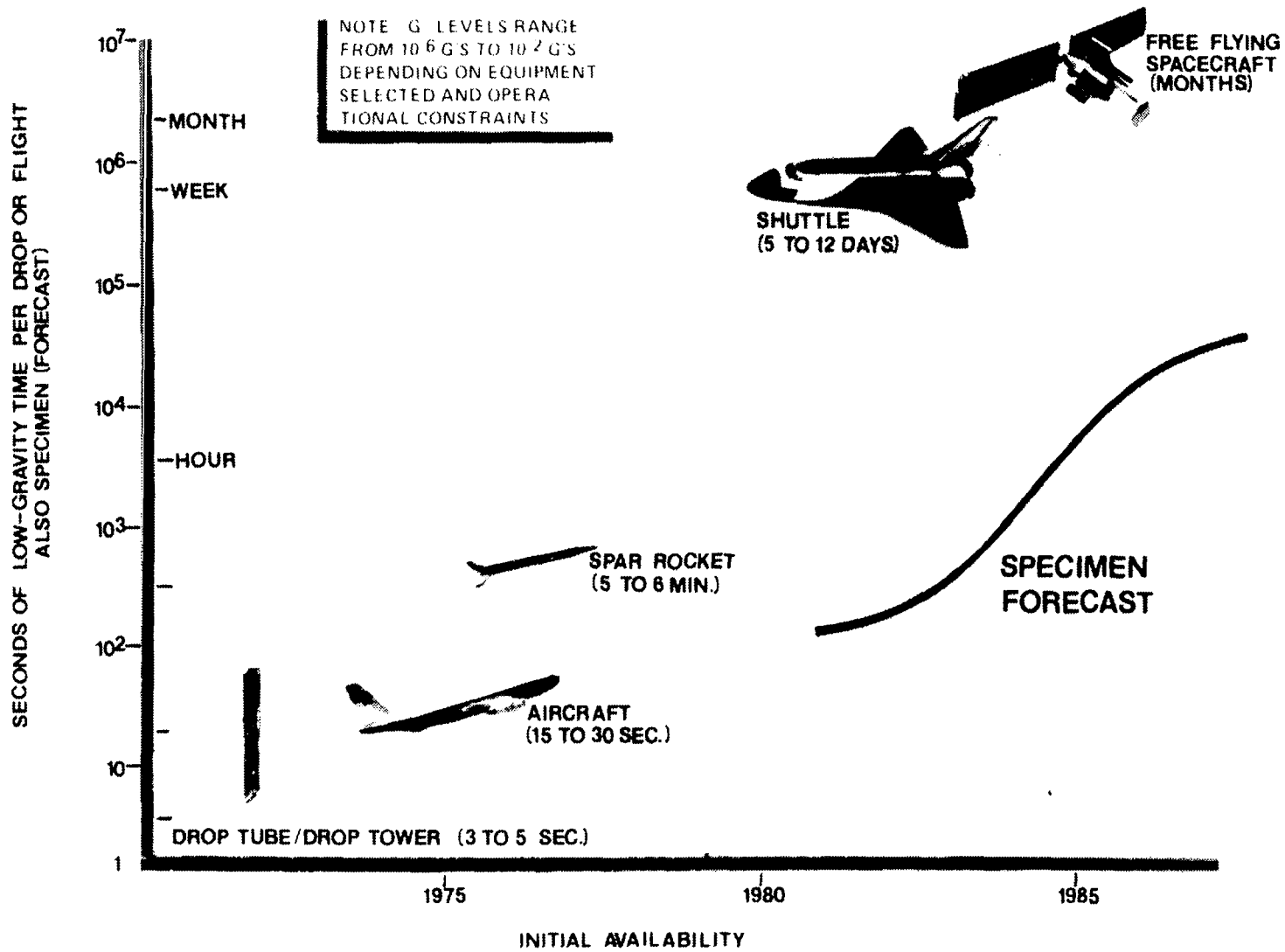
Figure 1. Low-gravity capability.
