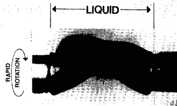
SIMULATED FLOAT ZONE IN 0-g.
