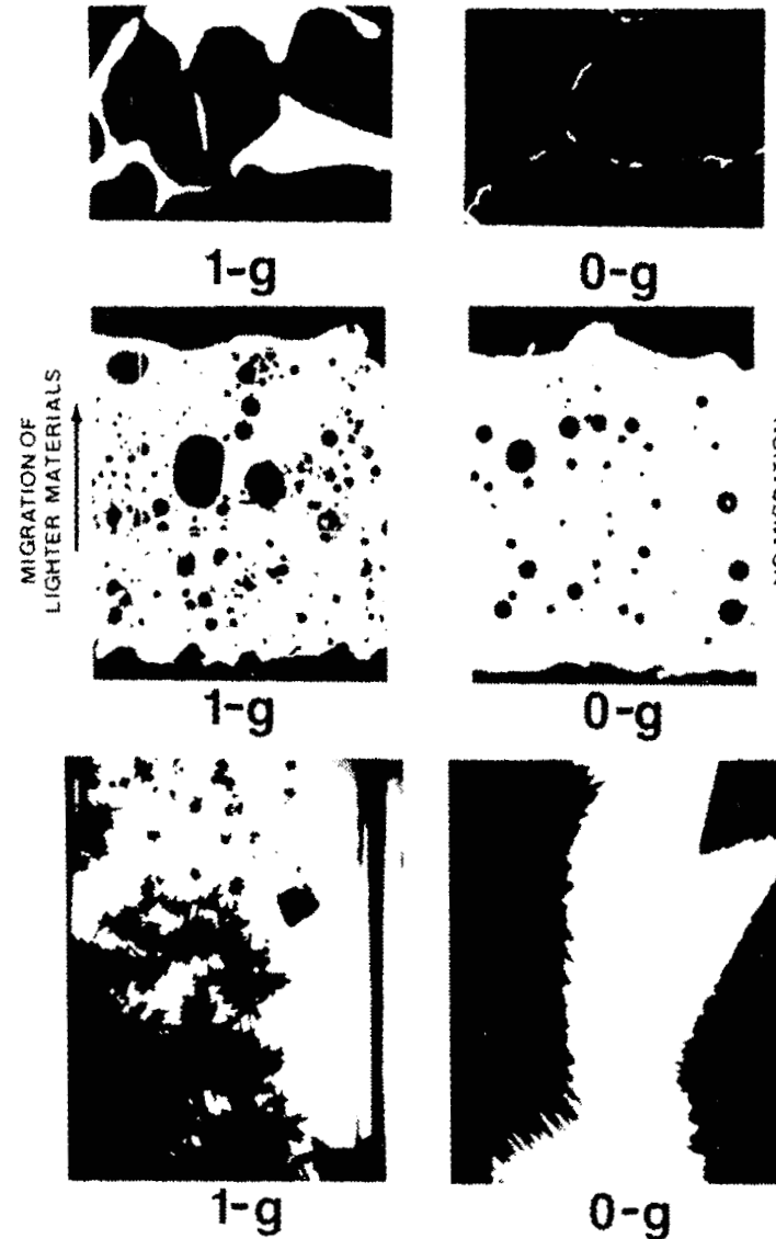
Figure 4. Sedimentation/buoyancy effects.
