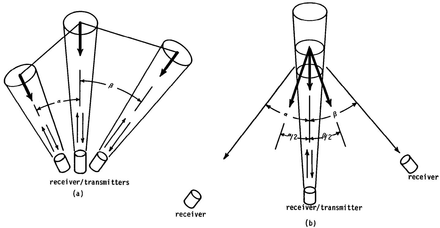
Figure 4-2. Three Dimensional Wind Velocity Acoustic Sounder Systems: a) three monostatic systems and b) monostatic vertical system with two additional receivers to form bistatic systems
