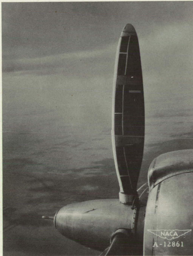
Figure 31.— Ice formation of encounter 12. Camber face. Efficiency loss, 5 percent.
