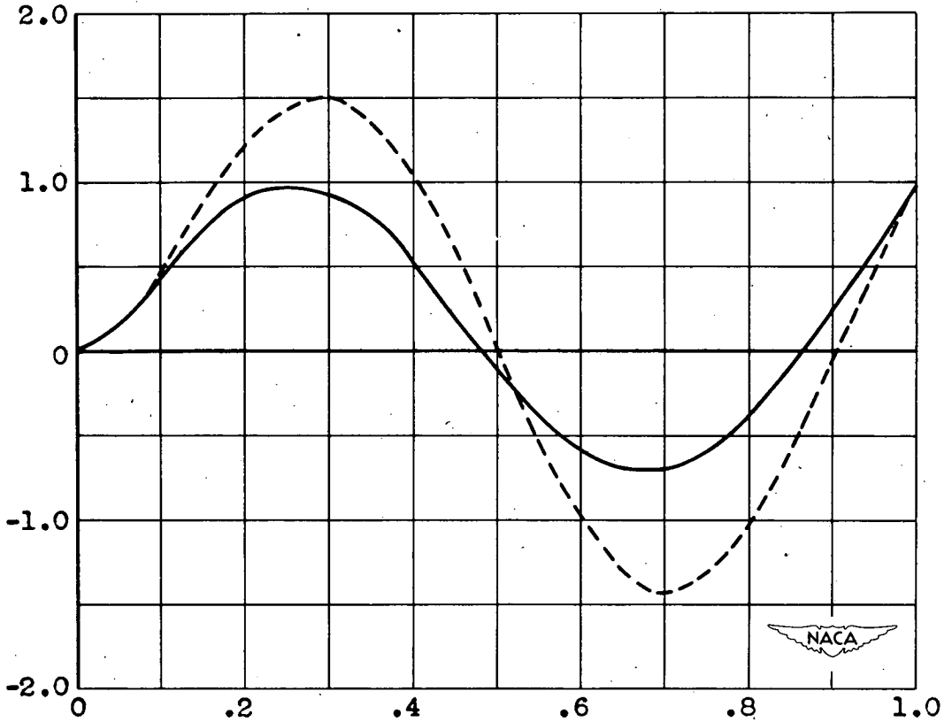
(e) Bending vibrations; second mode, n = 3 .
