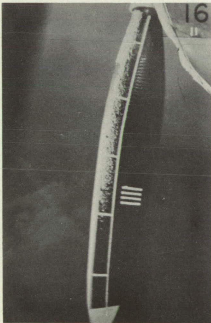
Figure 30.— Ice formation of encounter 11. Thrust face. Efficiency loss, 0 percent.
