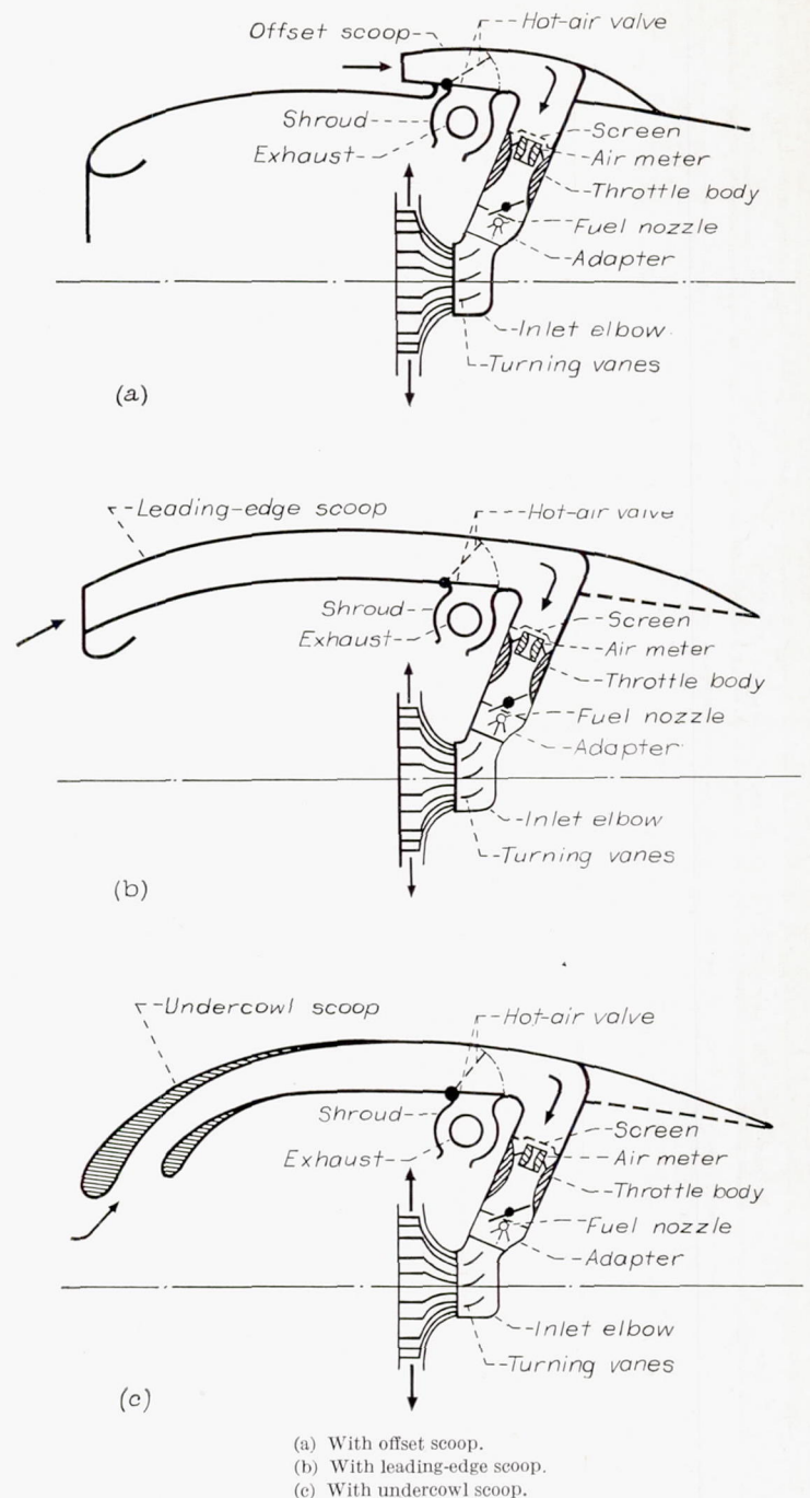
FIGURE 1.—Typical induction system.
