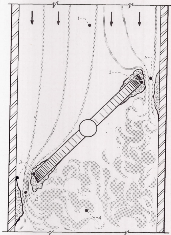
FIGURE 3.—Schematic diagram of throttle and throttle barrel showing air-flow pattern and throttling ice.
