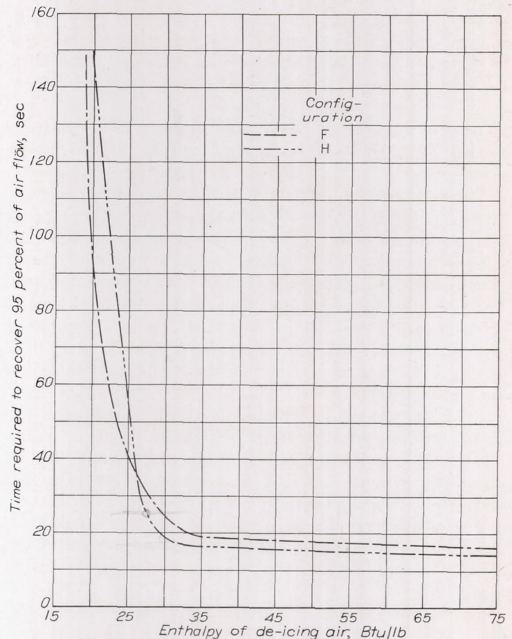
FIGURE 22.—Variation of air-flow recovery time with de-icing air enthalpy for two induction systems at low cruise power with an air-flow loss due to icing of 2000 pounds per hour.
