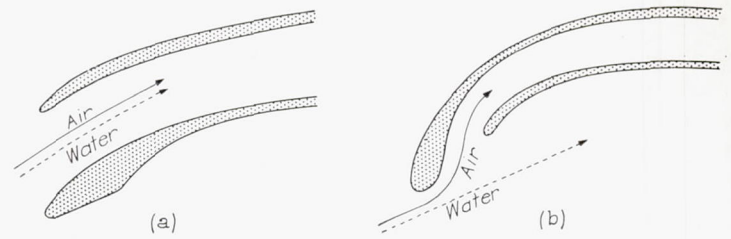
(a) Leading-edge scoop. (b) Undercowl scoop. FIGURE 10.—Air and water-droplet paths for conventional and undercowl scoops.
