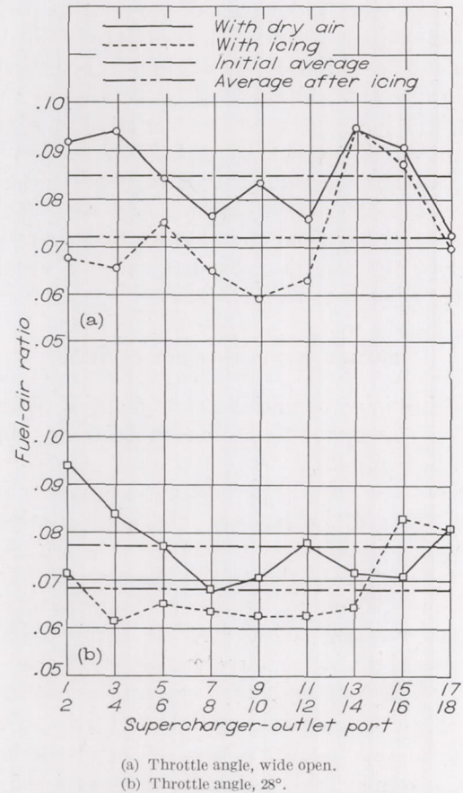
FIGURE 19.—Effect of icing on mixture distribution. Air temperature, 25° F; air flow, 7000 pounds per hour reduced to 6500 pounds per hour by icing.
