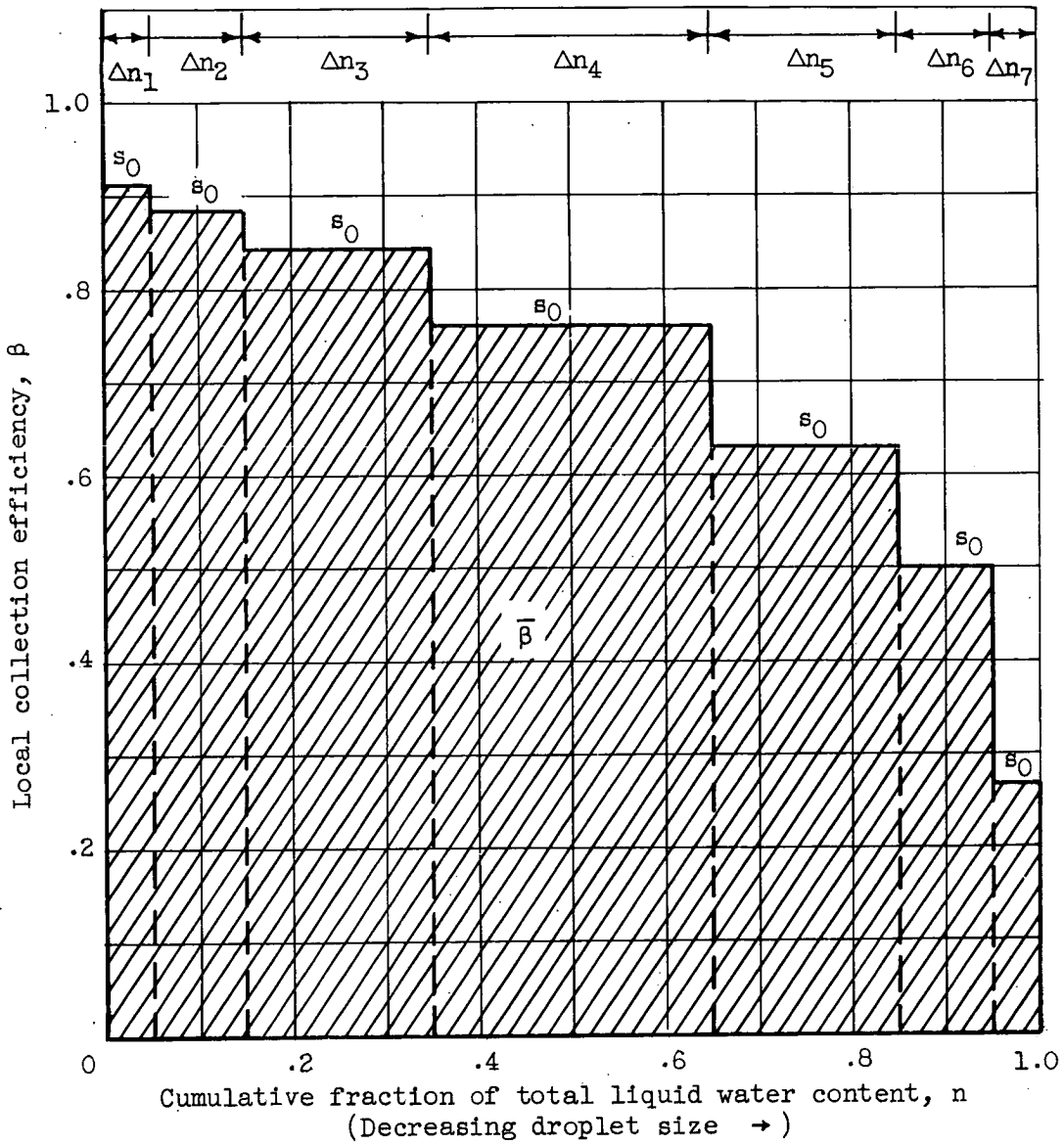
Figure 4. - Typical representation of weighted local collection efficiency \bar{\beta} as summation of contributions by each droplet-size group in distribution for one particular surface location s_0 on two-dimensional body for block-type droplet distribution. Cross-hatched area represents \bar{\beta} at s_0 .
