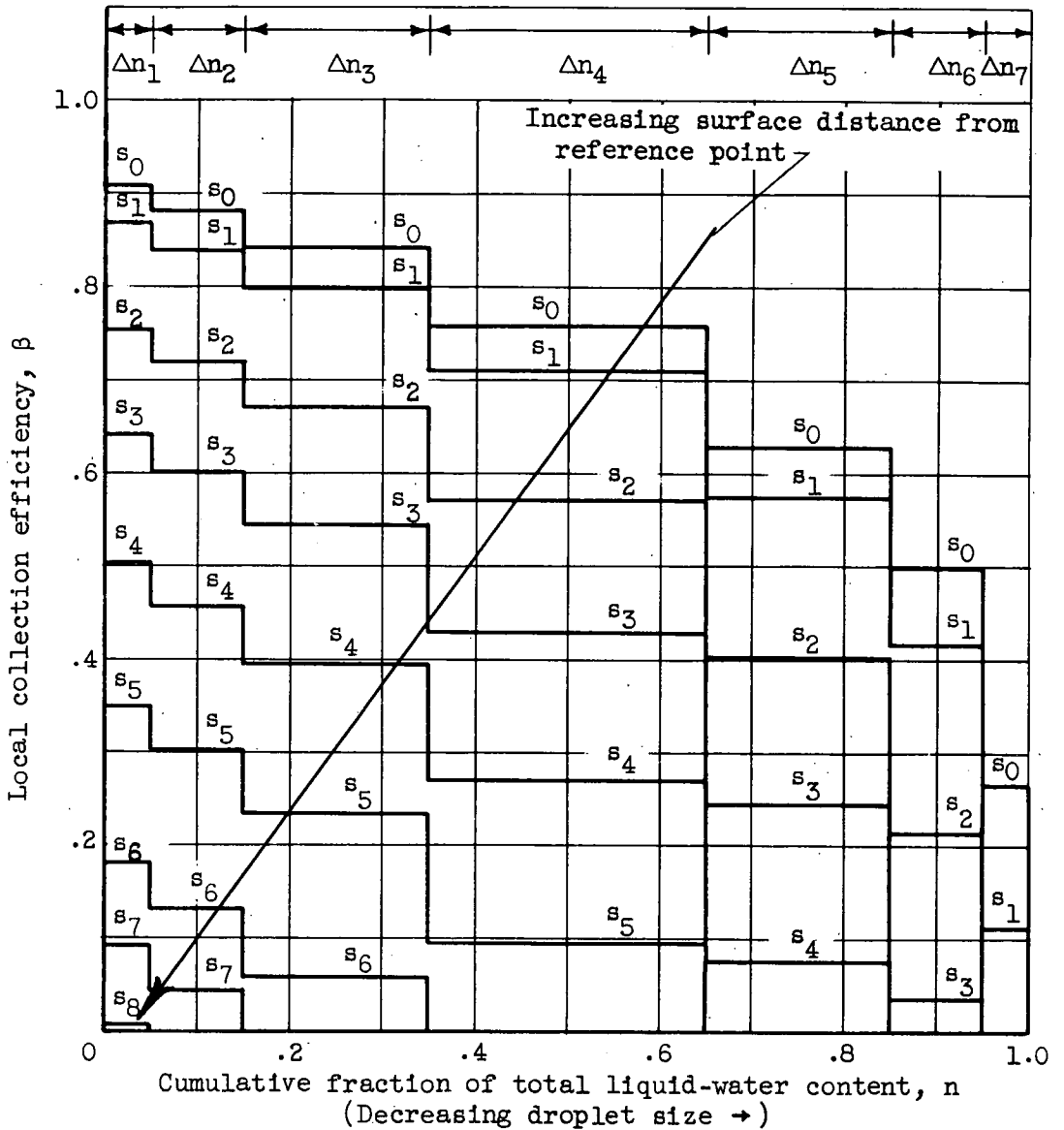
Figure 5. - Typical variation of weighted local collection efficiency \bar{\beta} (represented by area under a particular s_n curve) as function of surface location on two-dimensional body for block-type droplet distribution.
