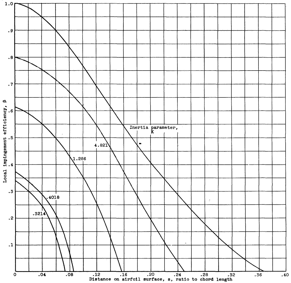
(e) Free-stream Reynolds number, 1024.
