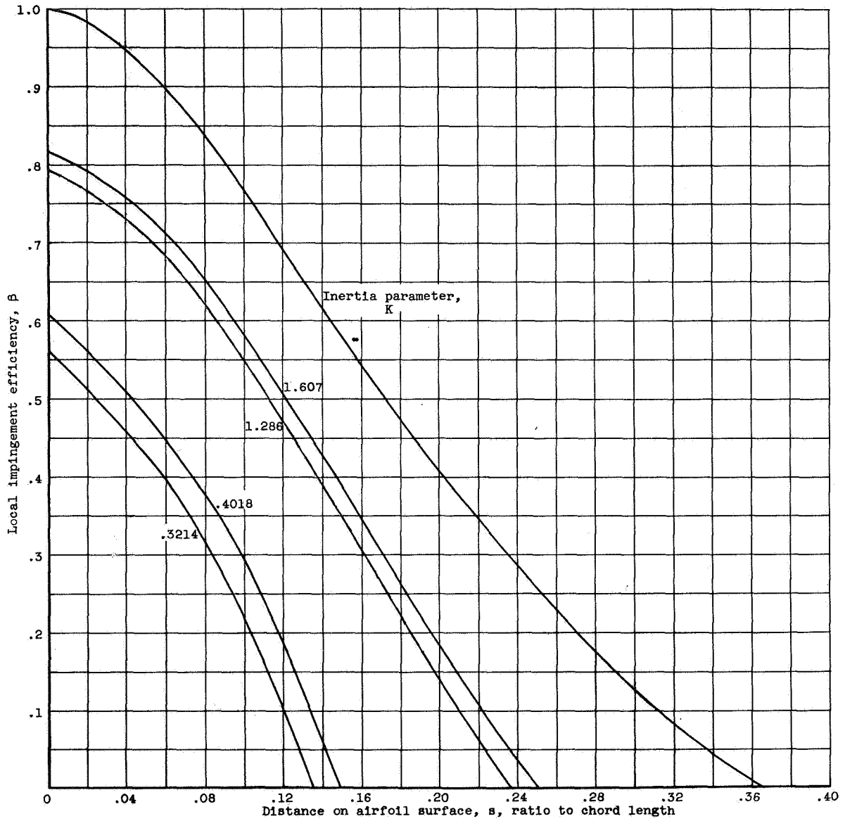
(c) Free-stream Reynolds number, 128.
