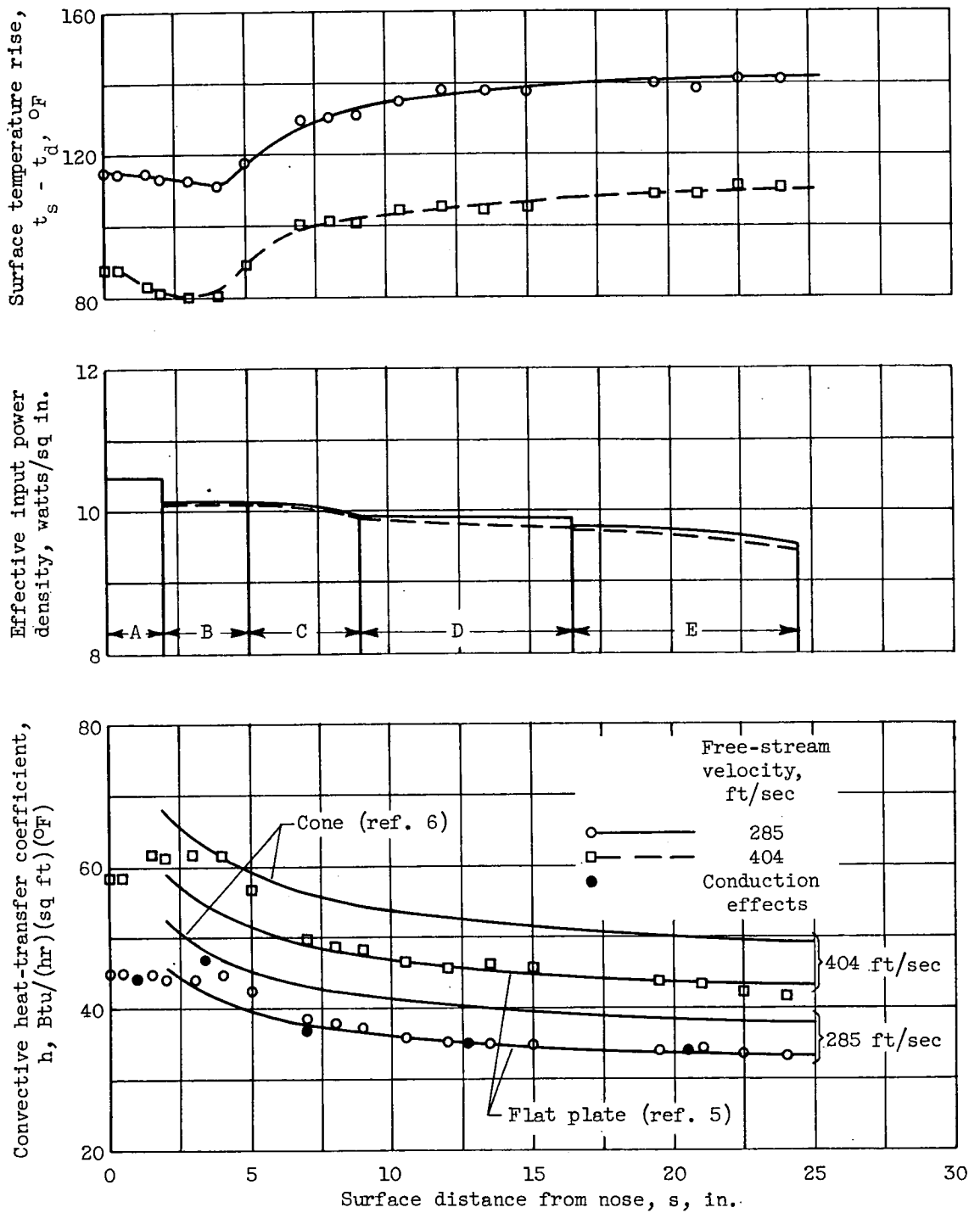
Figure 7. - Effect of free-stream velocity on surface temperature distribution and heat-transfer characteristics of stationary spinner with uniform heat input. Nominal input power density, 10 watts per square inch; angle of attack, 0^\circ ; free-stream total temperature, -2^\circ F.
