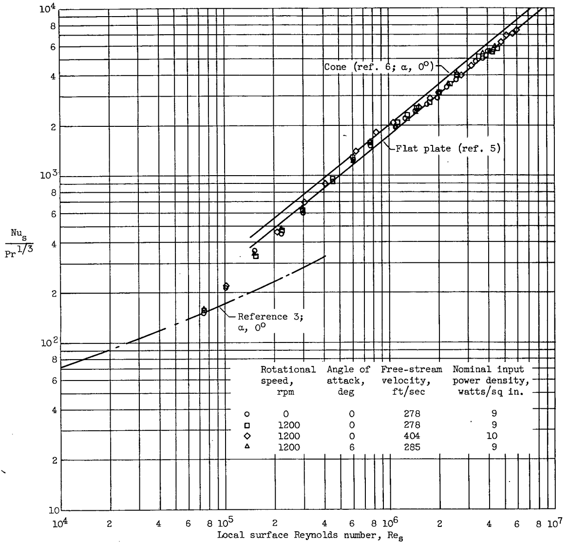
Figure 9. - Comparison of heat-transfer results obtained with stationary and with rotating spinner at various free-stream velocities for 0° and 6° angles of attack. Uniform heat input; average free-stream total temperature, -2° F.
