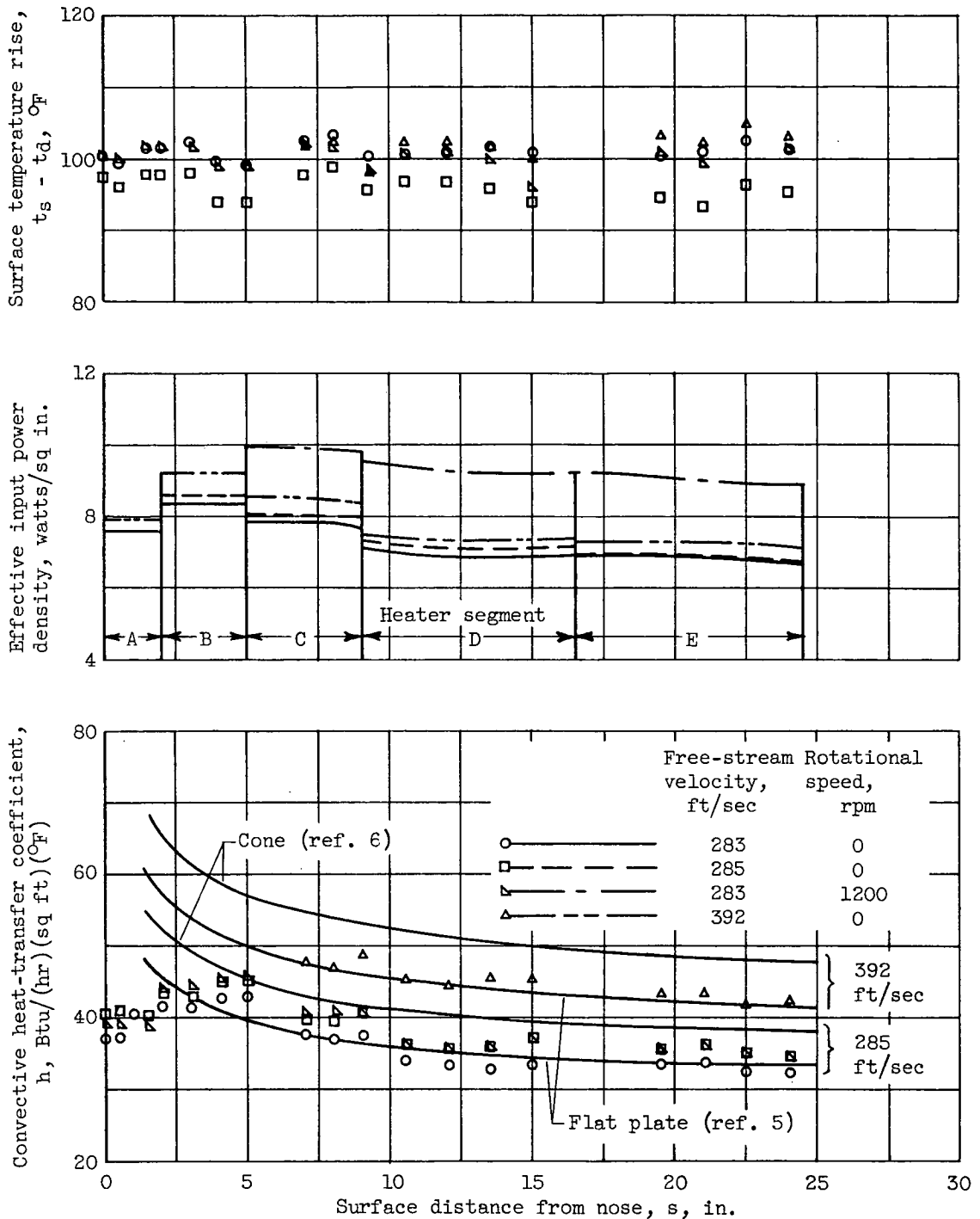
Figure 12. - Experimental results obtained at various free-stream velocities and rotational speeds for spinner with uniform surface temperature. Angle of attack, 0^\circ ; average free-stream total temperature, -1^\circ F.
