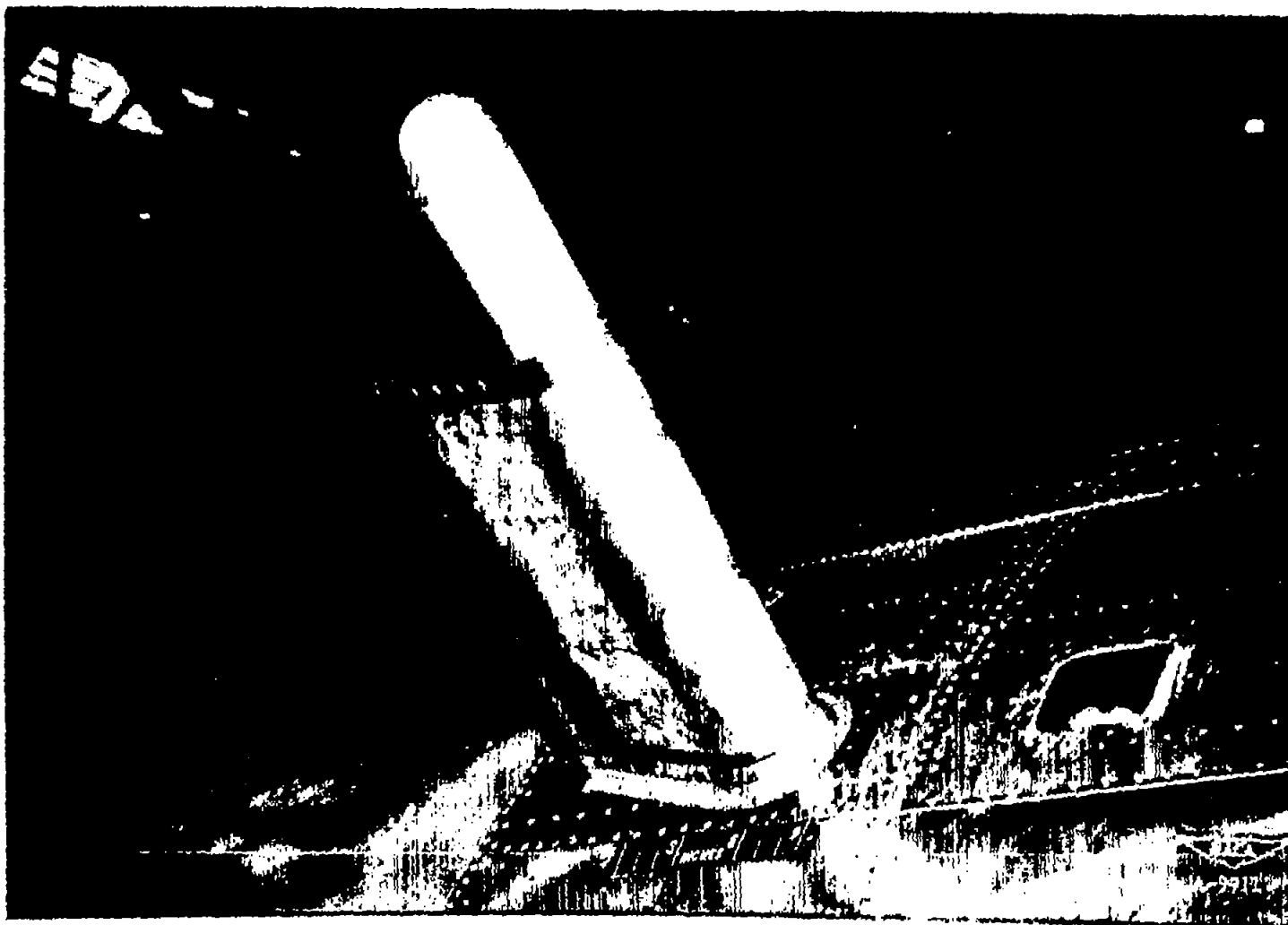
Figure 3.- Nonrotating, blueprint-paper-covered, 4-inch-diameter cylinder for the measurement of maximum drop diameter in clouds.
