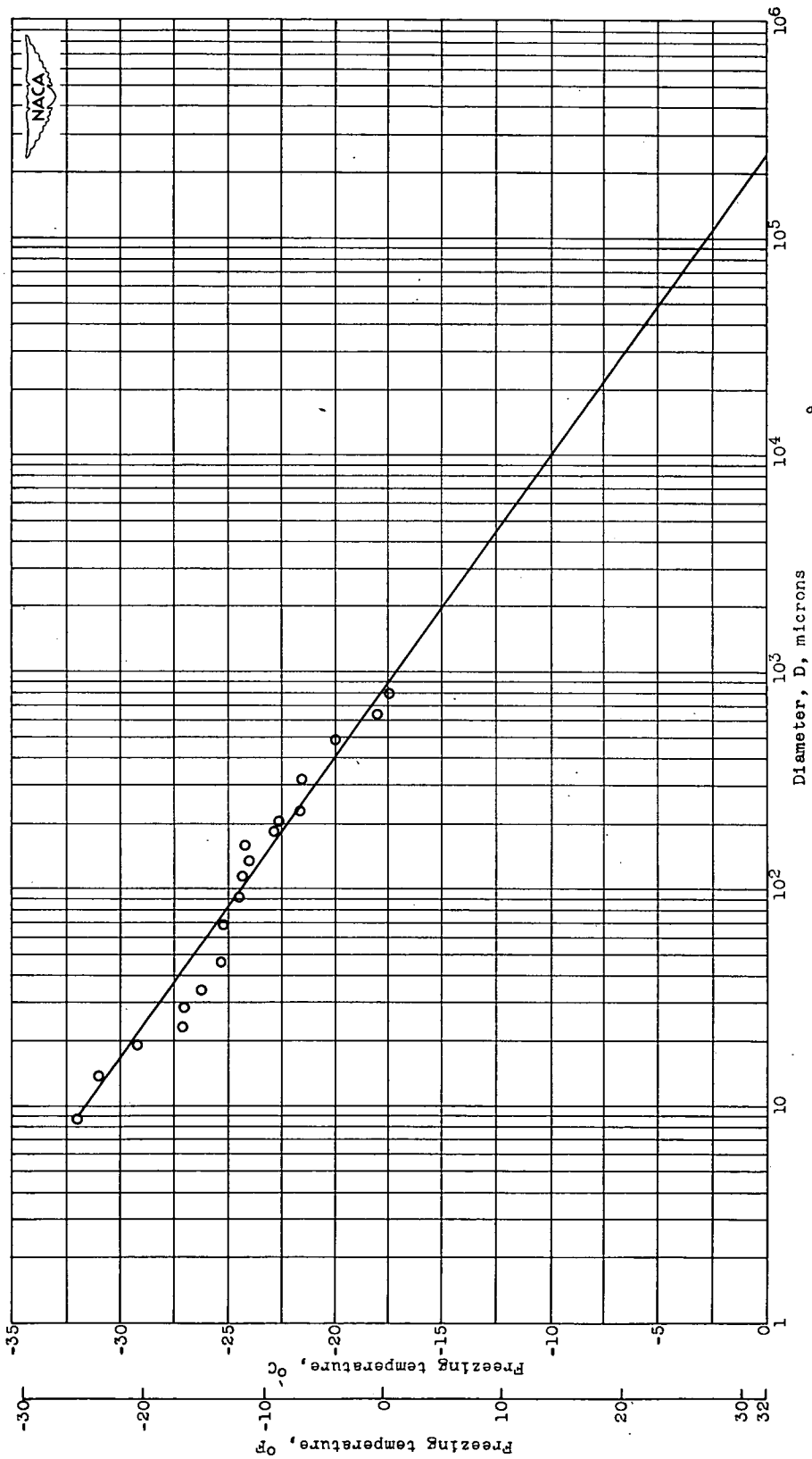
Figure 2. - Straight line fitted to data from reference 2 for diameter D against average freezing temperature.
