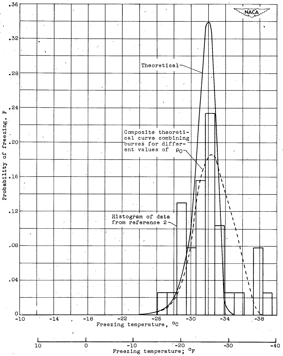
Figure 3. - Concluded. Comparison of theoretical and experimental probability curves.
