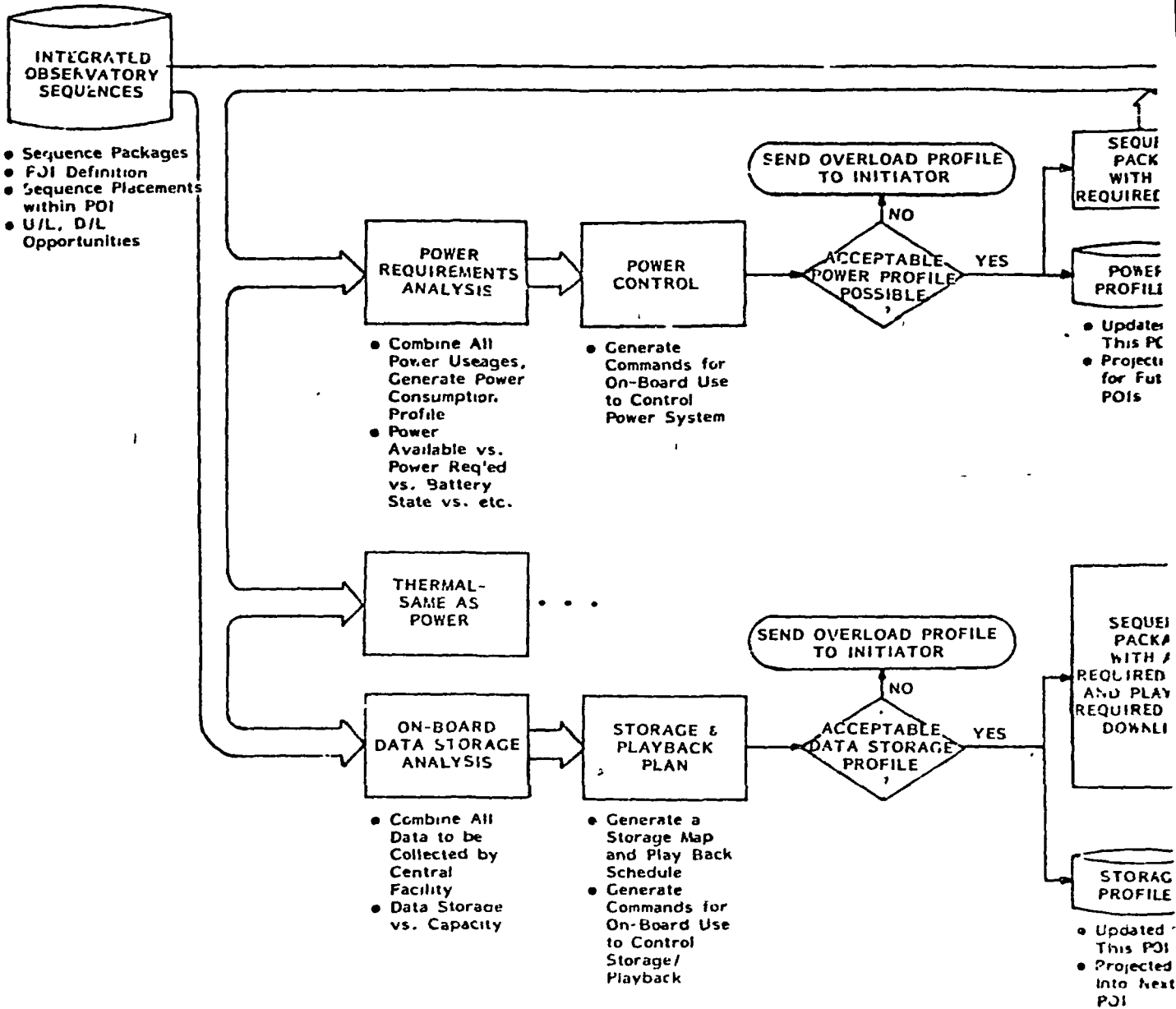
FIGURE 3 4-3 COMMAND GENERATION
