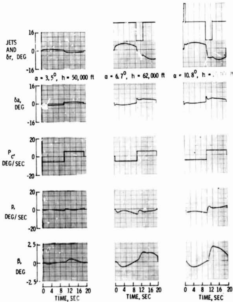
(c) Mach number 1.5 Figure 12.- Continued.
