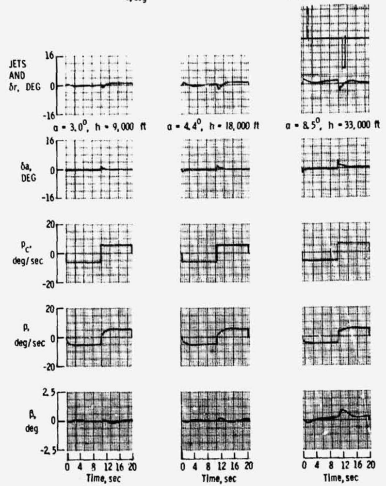
(b) Mach number .7 Figure 9. - Continued.
