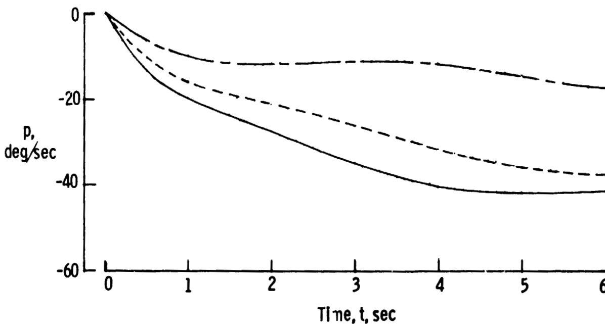
Figure 7.- Response for the unaugmented space shuttle orbiter for a two degree aileron input.
