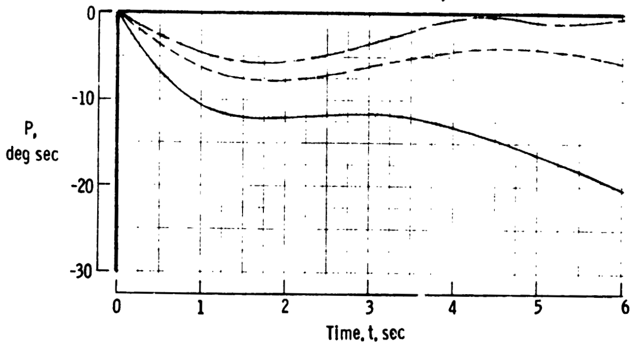
(a) Mach number 1.5
