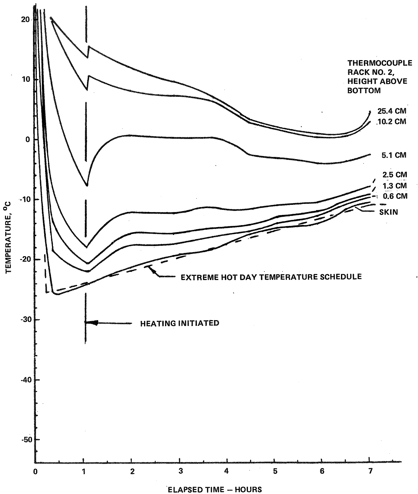
FIGURE 24 - TIME HISTORY, HIGH-POWER HEATING, EXTREME HOT DAY, TEST 143, LFP-13 FUEL
