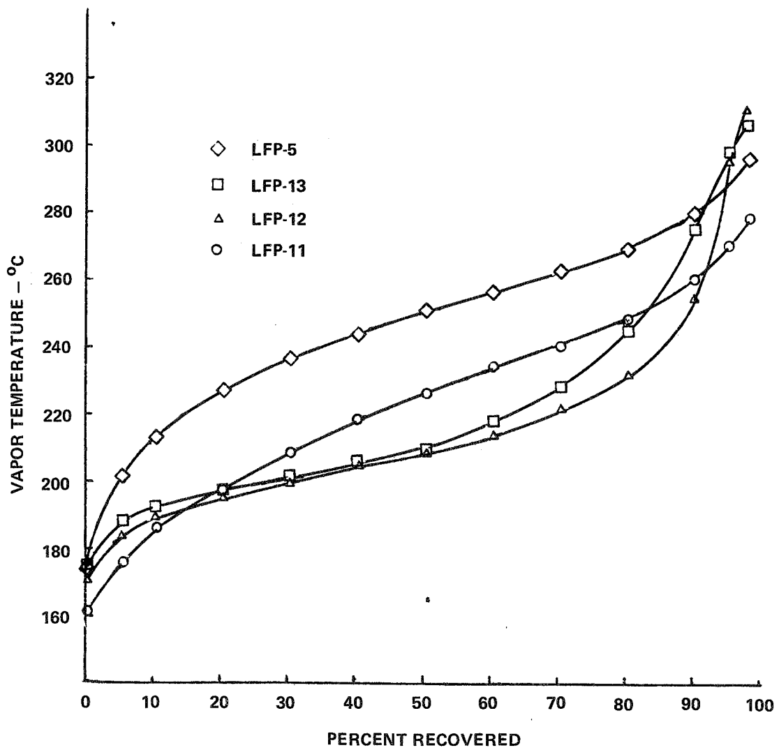
FIGURE 12 - DISTILLATION CHARACTERISTICS OF TEST FUELS, ASTM METHOD D-86 (REF. 7)
