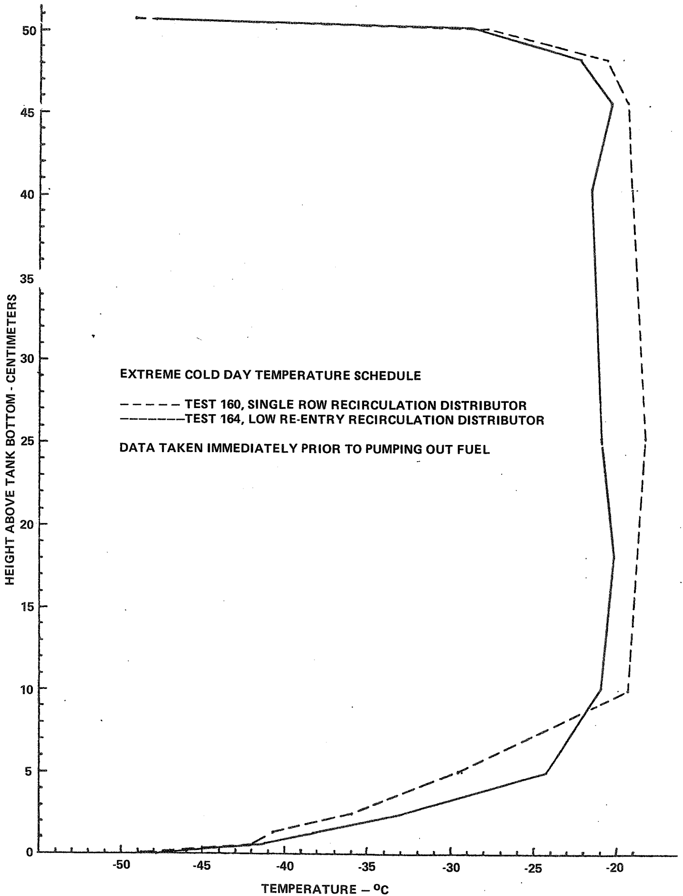
FIGURE 33 - TEMPERATURE PROFILE COMPARISON, LOW RE-ENTRY VS. SINGLE ROW DISTRIBUTOR, TESTS 160 AND 164, LFP-13 FUEL
