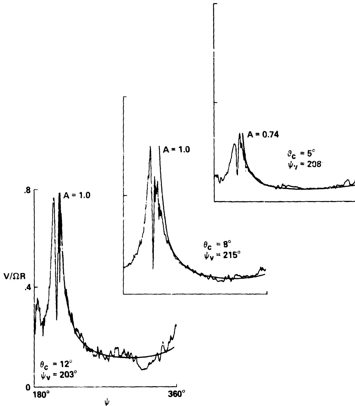
Figure 12.- Typical vortex velocity-time trace and 1/R curve fit for various pitch settings; vortex age = 200^\circ (nominal), \Omega = 1250 rpm.
