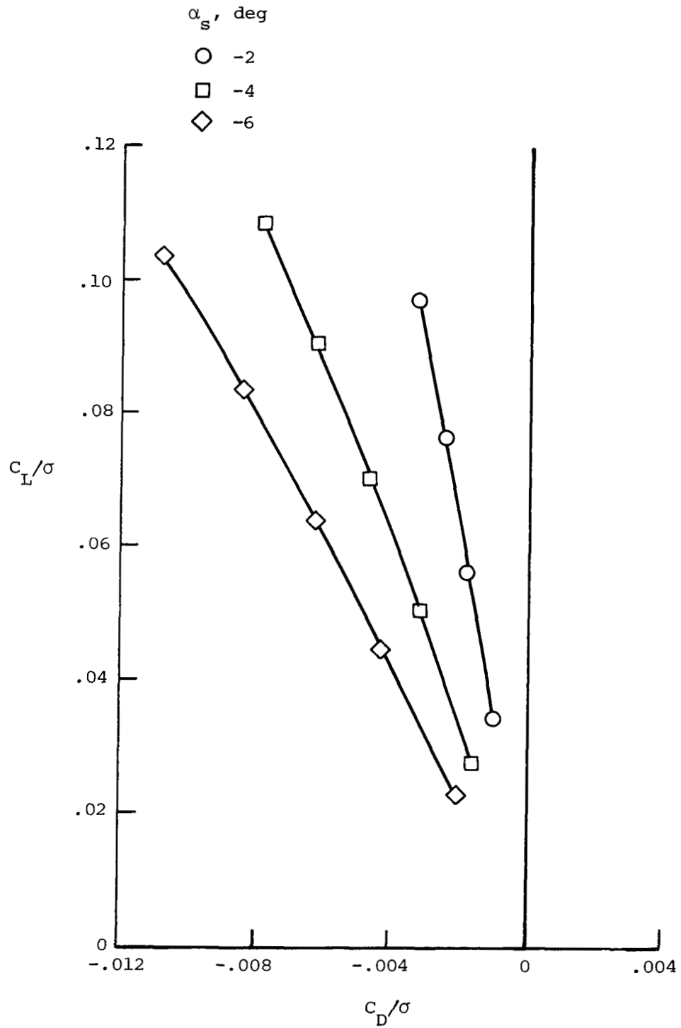
(a) C_L/\sigma versus C_D/\sigma at \mu = 0.20 .
