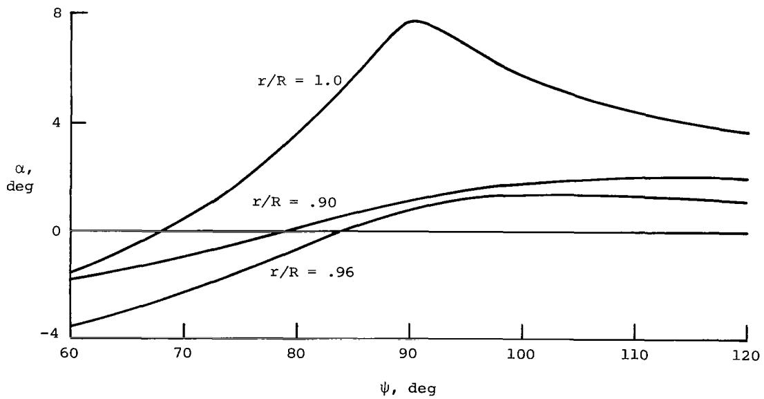
(b) \mu = 0.20 ; C_L/\sigma = 0.08 ; \alpha_s = -4^\circ ; nonuniform inflow.
