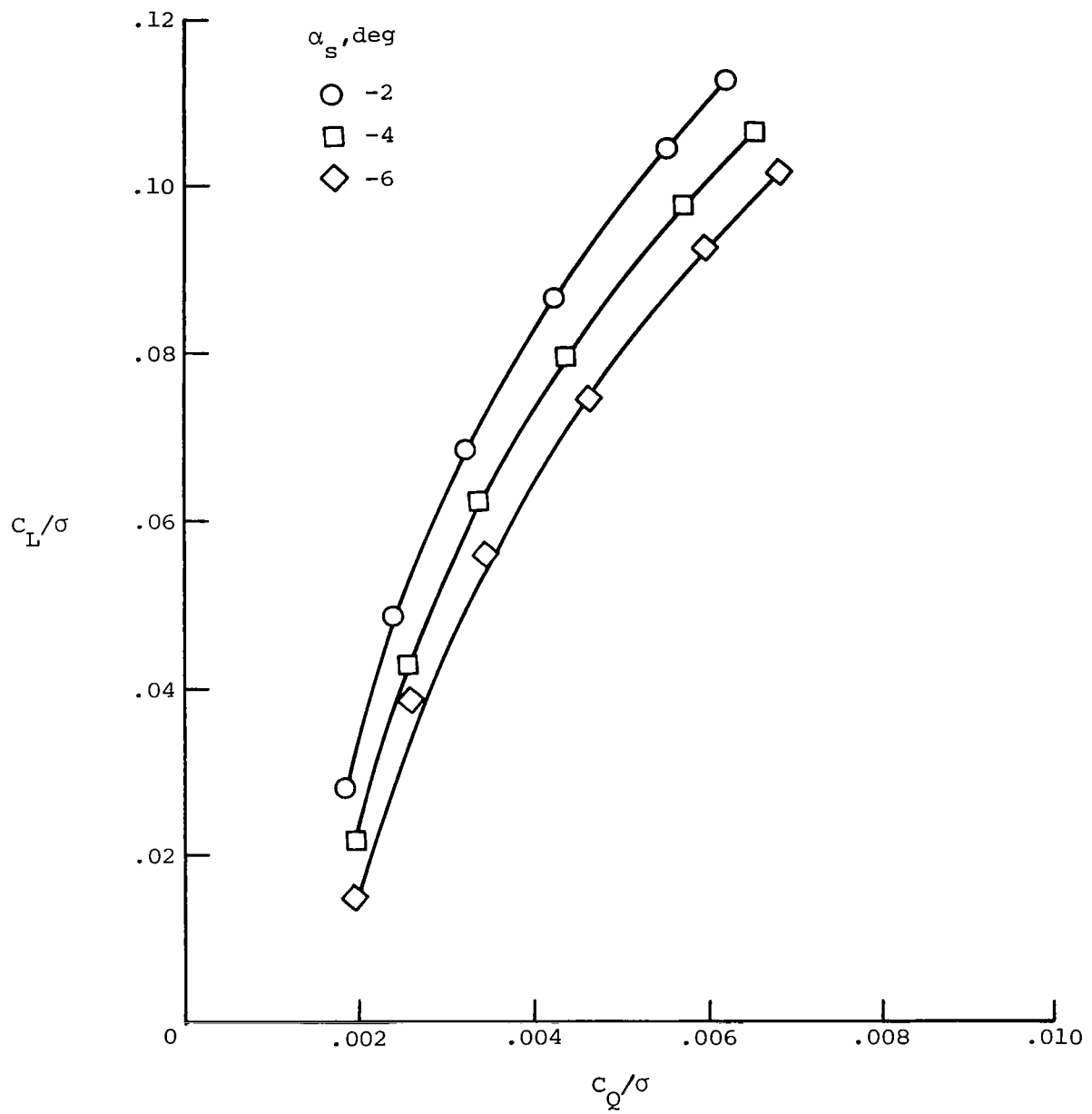
(b) C_L/\sigma versus C_Q/\sigma at \mu = 0.20 .
