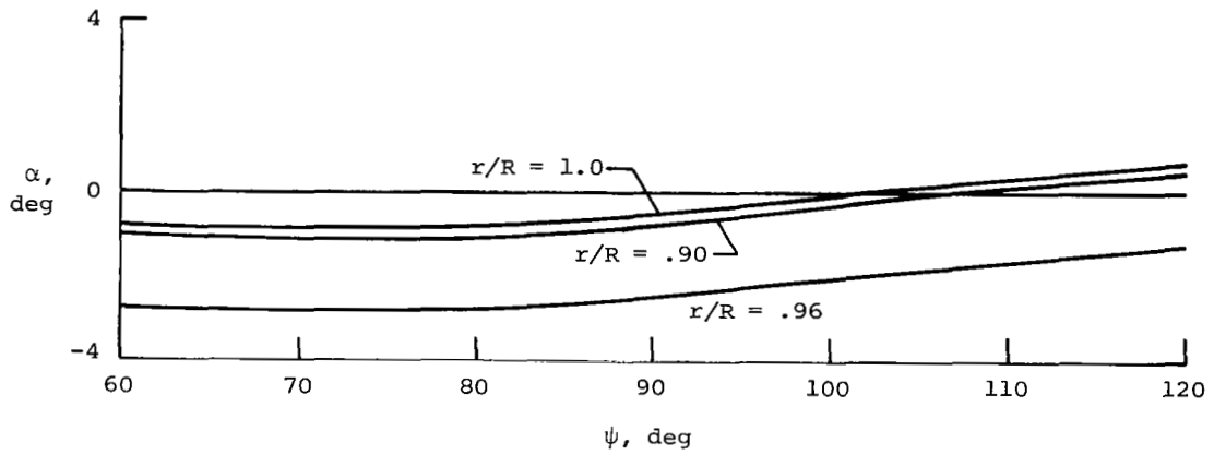
(e) \mu = 0.35 ; C_L/\sigma = 0.08 ; \alpha_s = -6^\circ ; uniform inflow.
