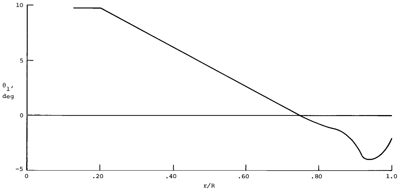
Figure 3.- Rotor blade geometry.
