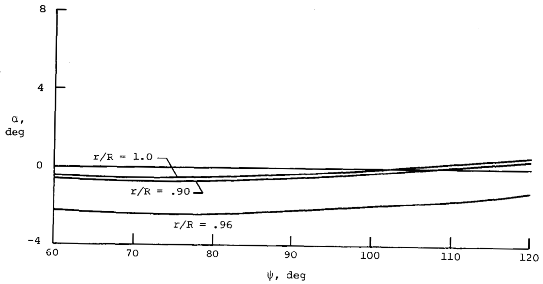
(c) \mu = 0.30 ; C_L/\sigma = 0.08 ; \alpha_s = -4^\circ ; uniform inflow.
