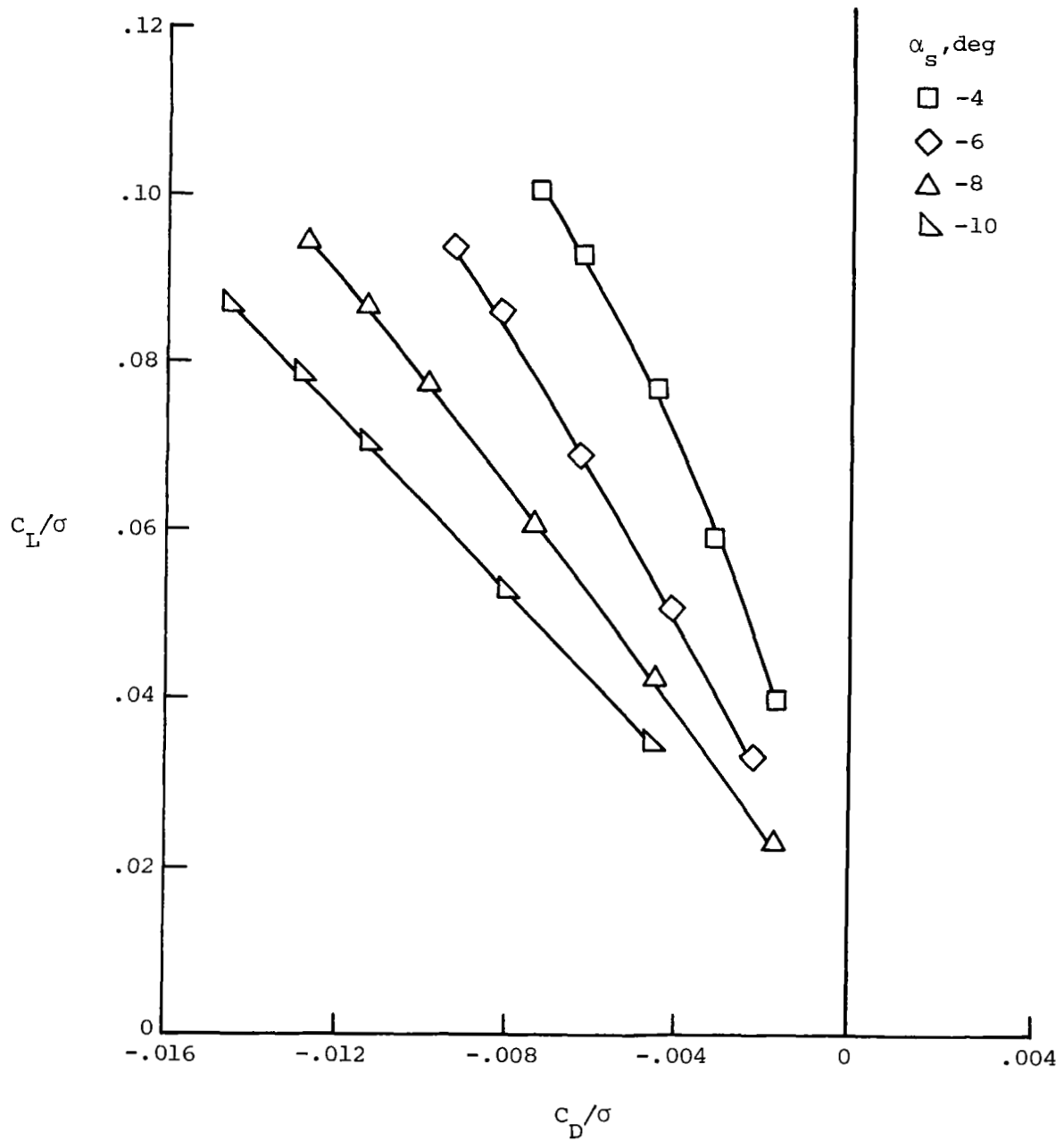
(c) C_L/\sigma versus C_D/\sigma at \mu = 0.30 .
