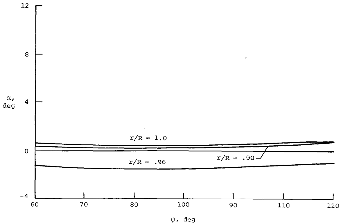
(a) \mu = 0.20 ; C_L/\sigma = 0.08 ; \alpha_s = -4^\circ ; uniform inflow.
