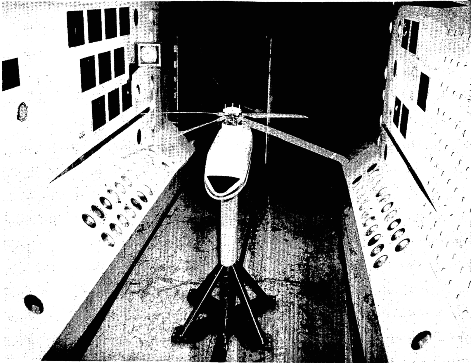
Figure 5.- ARES in TDT.
