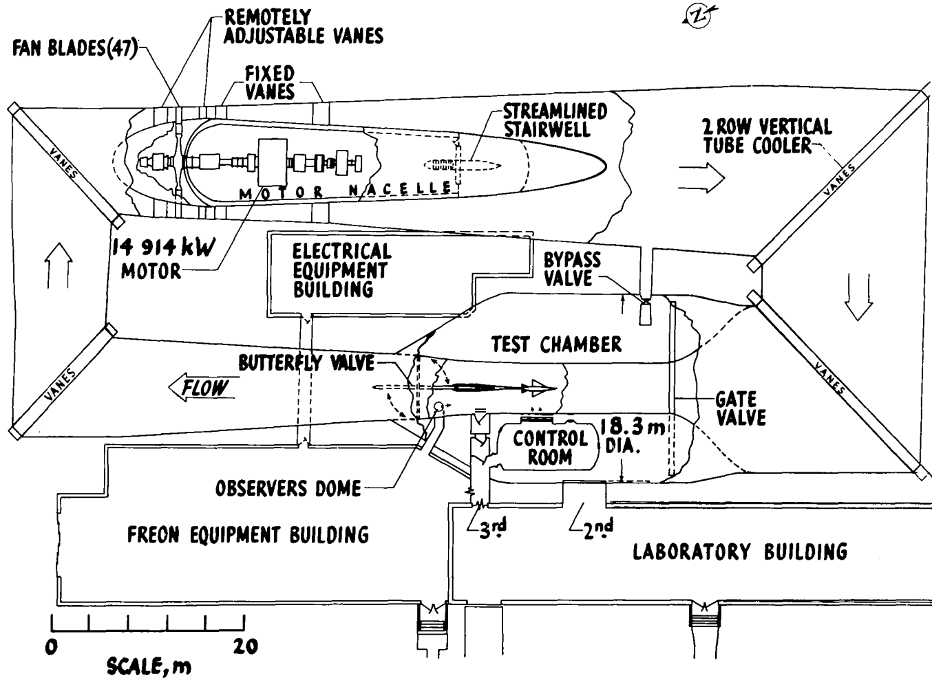
Figure 2.- Langley Transonic Dynamics Tunnel.
