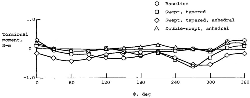
(a) \mu = 0.20 ; C_L/\sigma = 0.08 ; \alpha_S = -4^\circ .
