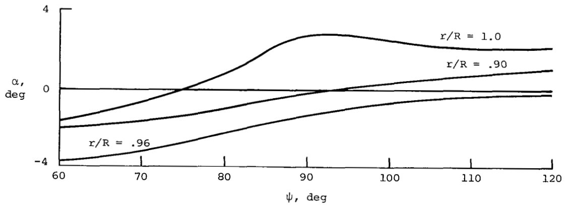
(f) \mu = 0.35 ; C_L/\sigma = 0.08 ; \alpha_s = -6^\circ ; nonuniform inflow.
