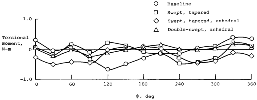
(b) \mu = 0.30 ; C_L/\sigma = 0.08 ; \alpha_S = -4^\circ .
