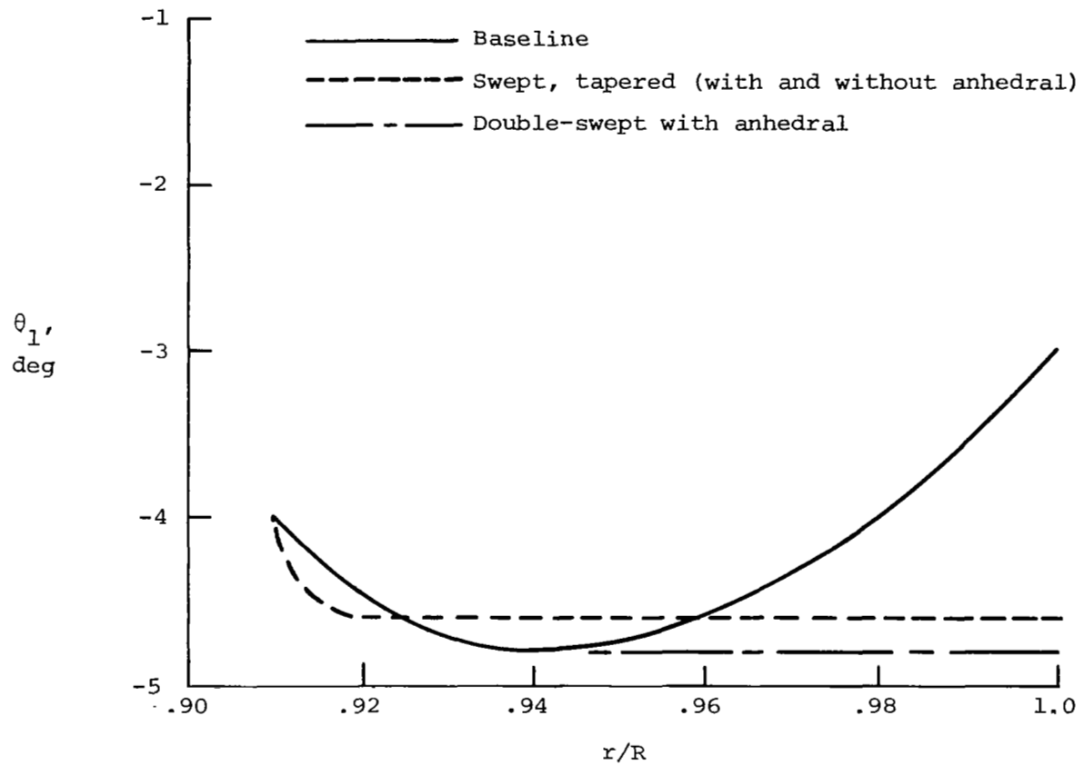
(b) Tip twist distribution (positive nose-up).
