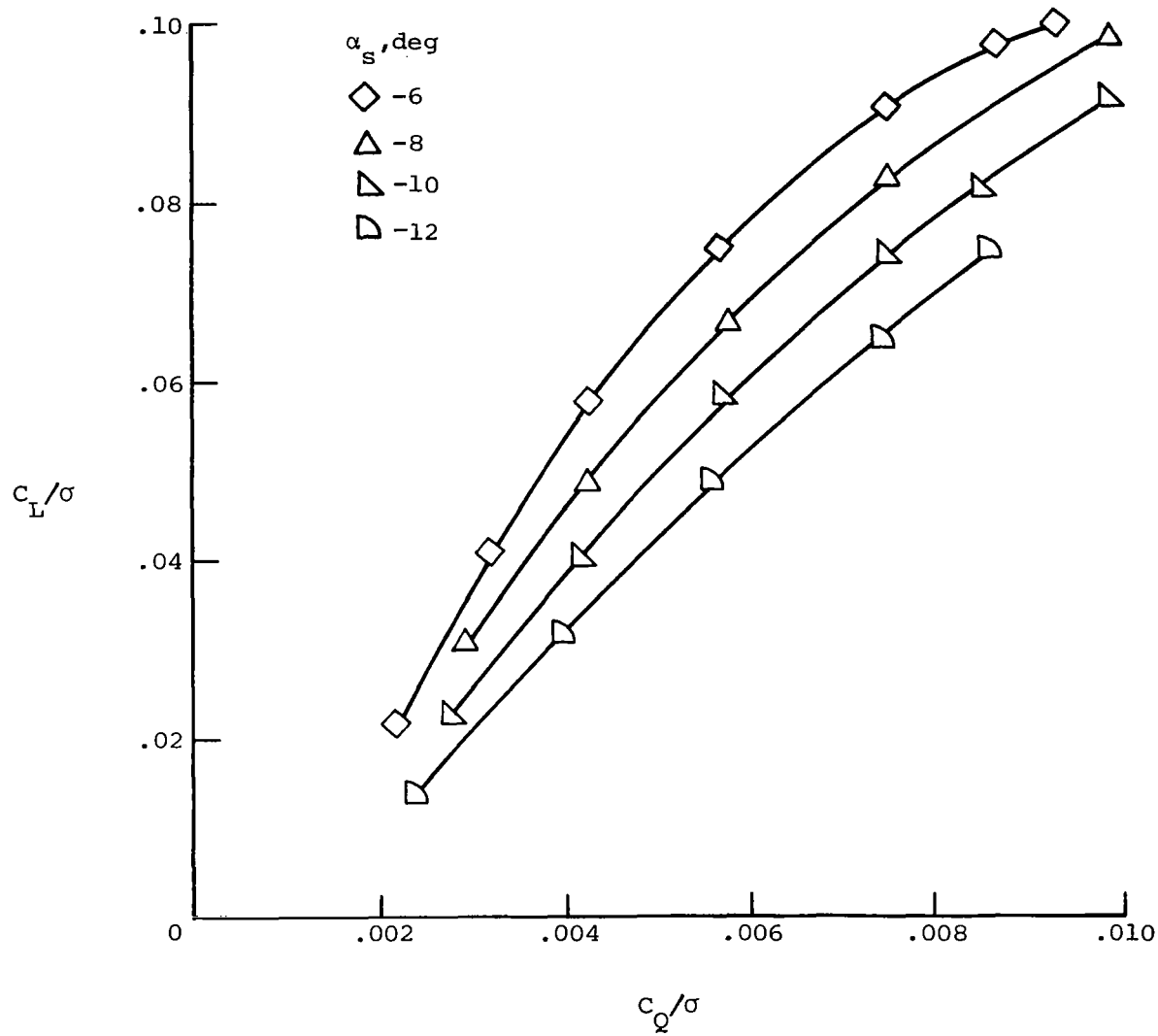
(f) C_L/\sigma versus C_Q/\sigma at \mu = 0.35 .
