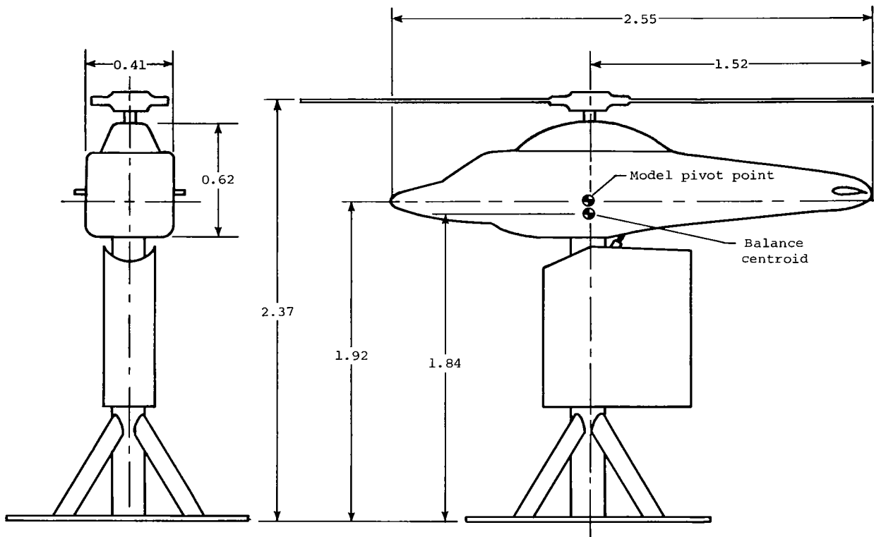
Figure 6.- Schematic diagram of aeroelastic rotor experimental system. All dimensions are given in meters.
