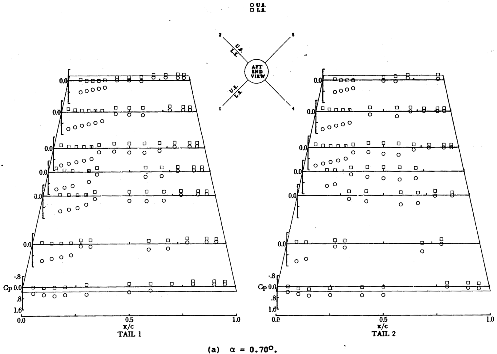
Figure 21.- Pressure coefficients for tail planform A at M = 1.60 , \phi = 45^\circ , and \delta = -15^\circ .
