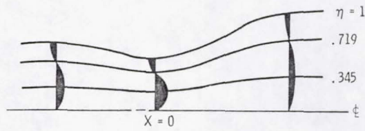
Figure 2. - Coordinate surfaces ( \eta = 0, 0.345, 0.719, 1 ) and transverse shape of (1, 1) mode at various axial locations.
