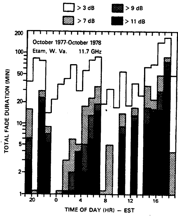
Figure 5.5-4. Diurnal Distribution of Fades Exceeding 3, 7, 9, 11 dB
