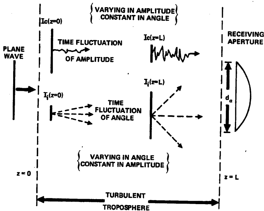
Figure 6.6-1. Decomposition into Coherent and Incoherent Components
