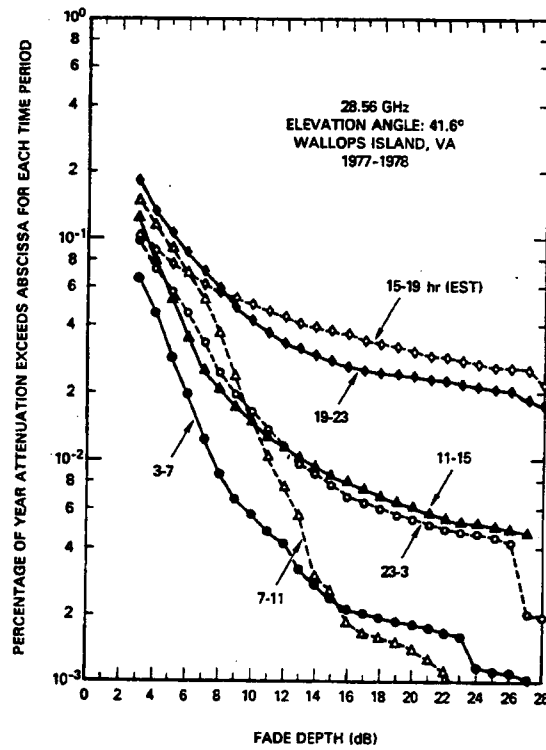
Figure 5.5-3. Cumulative Distributions for Six Contiguous Four-Hour Time Slots of Day
