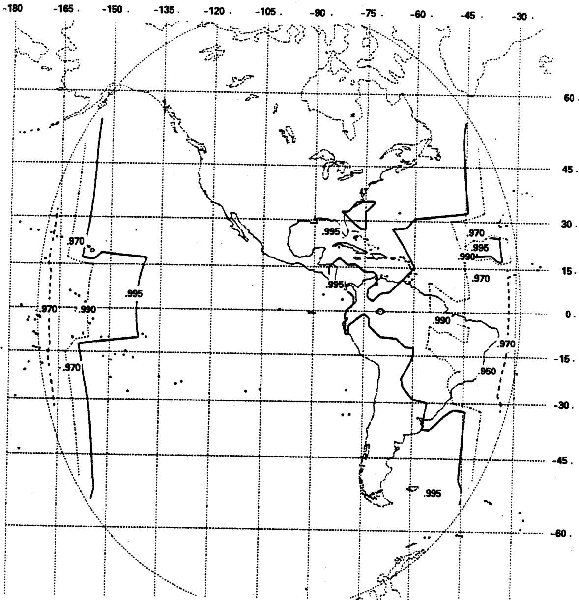
Figure 3.4-8. Availability Contour for Satellite at 100^{\circ}\text{W} With 6 dB Margin Operating at 20 GHz
