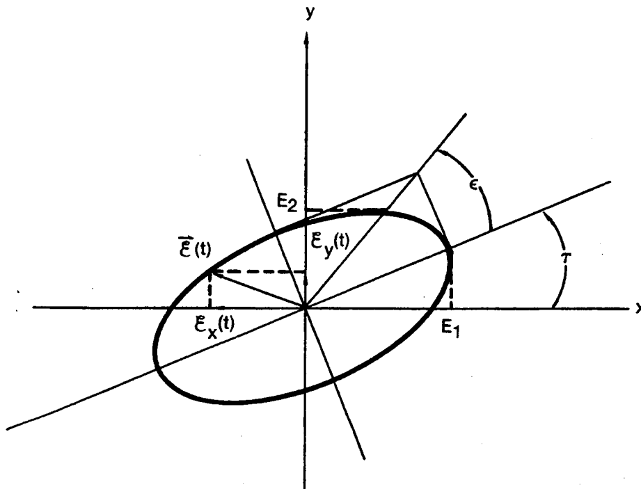
Figure 4.2-1. Polarization Ellipse
