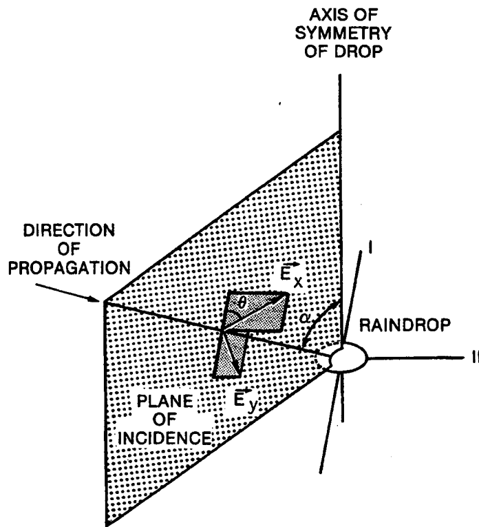
Figure 4.3-1. Geometry for Rain Depolarization Analysis
