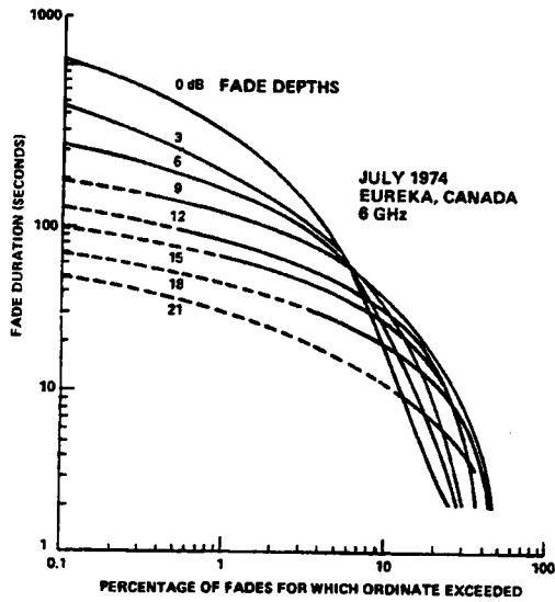
Figure 6.6-9 Cumulative Distributions of Fade Durations at 6 GHz
