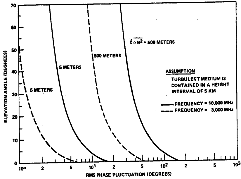
Figure 6.6-11. R.M.S. Phase Fluctuations for an Earth-Space Path
