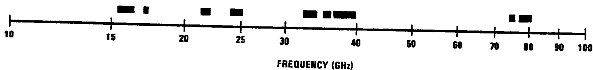
Figure 6.1-1. Frequencies NOT Potentially Available for Earth-Space Transmissions.
