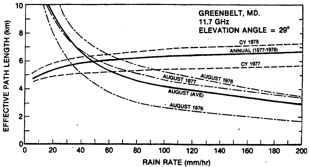
Figure 3.7-2. Effective Path Length for Annual & Worst Month Periods
