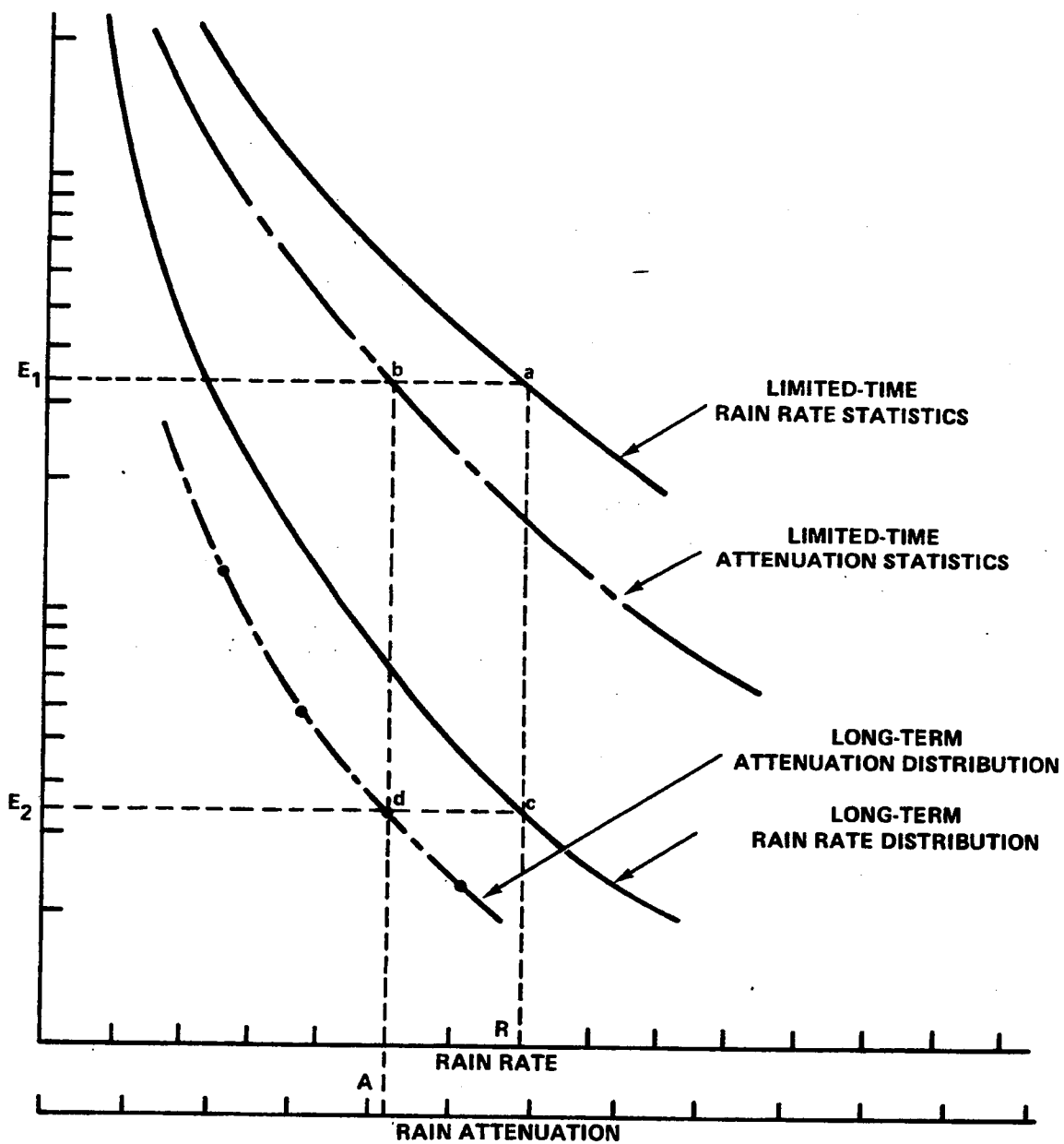
Figure 6.3-9 Construction of Cumulative Attenuation Statistics Using the Distribution Extension Technique
