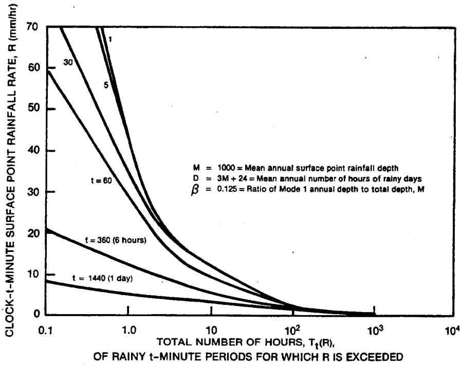
Figure 3.2-1. Average Year Cumulative Time Distributions
