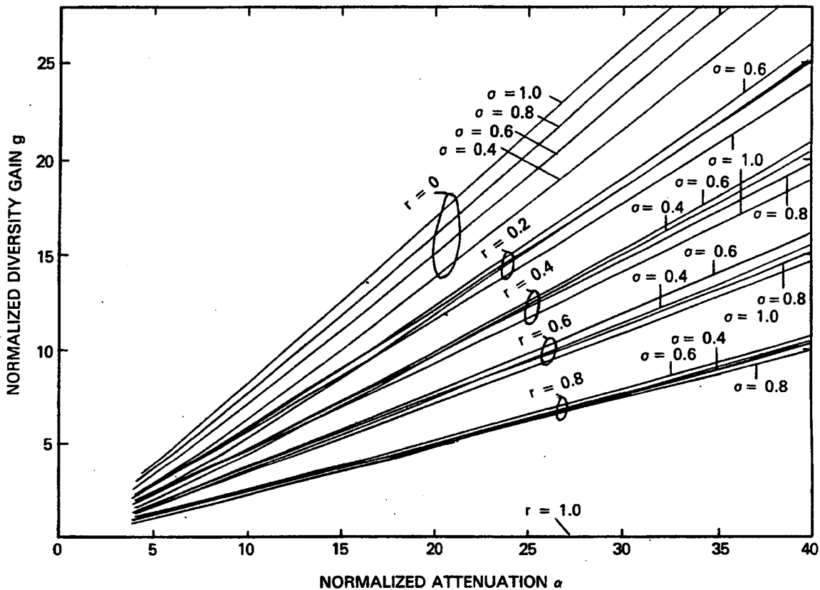
Figure 6.5-11. Diversity Gain versus Attenuation for Varying Distribution Parameters (Normalization is with Respect to Median Attenuation)
