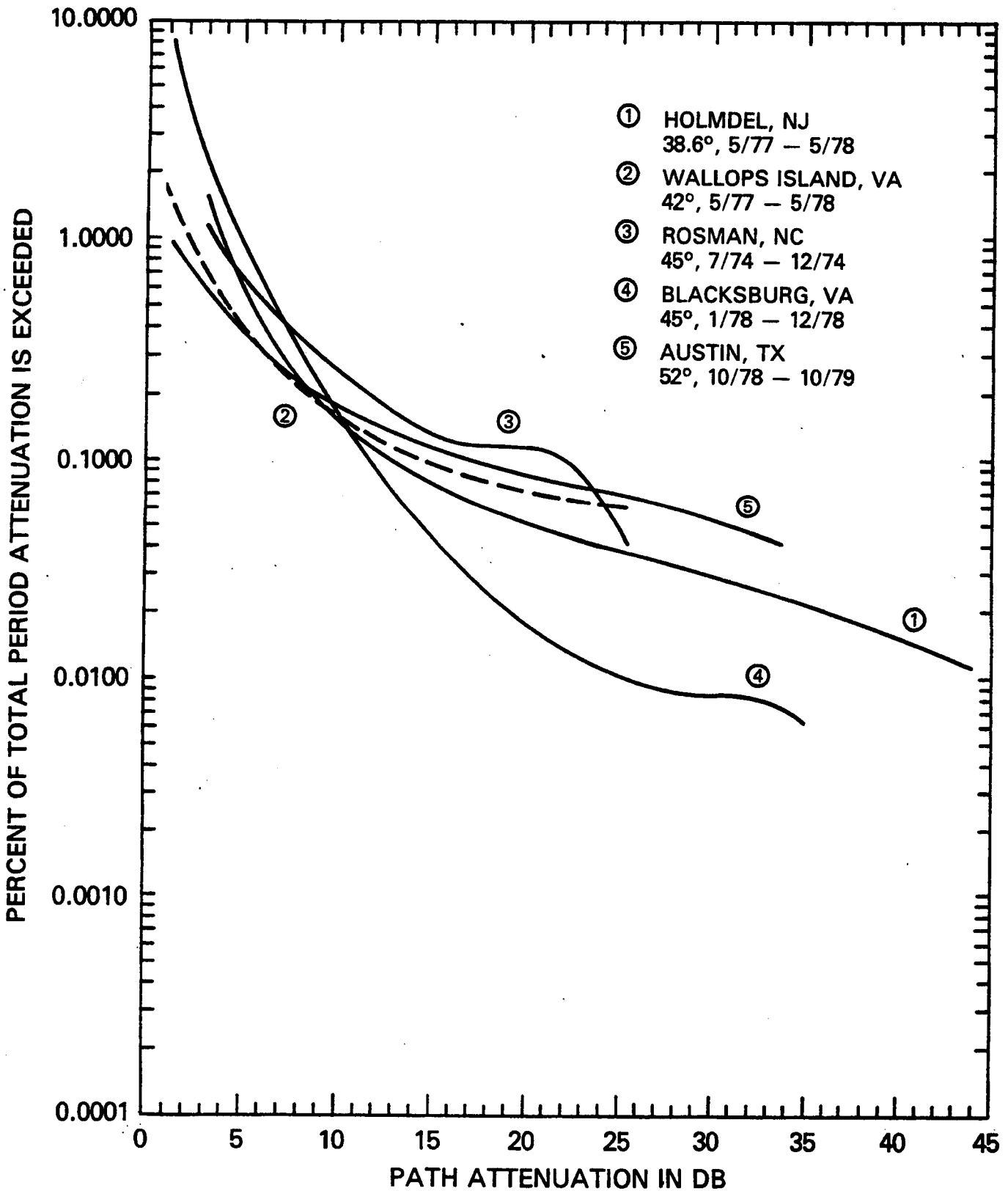
Figure 5.4-13. Summary of 28.56 and 30 GHz Measurements
