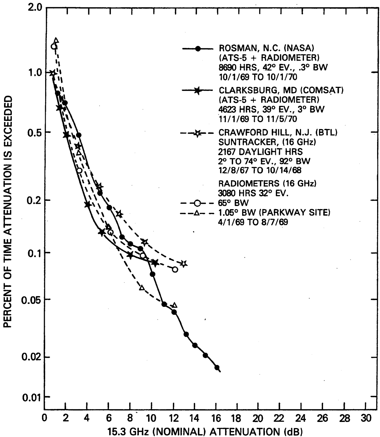
Figure 5.4-10. Summary of 15 GHz Measurements
