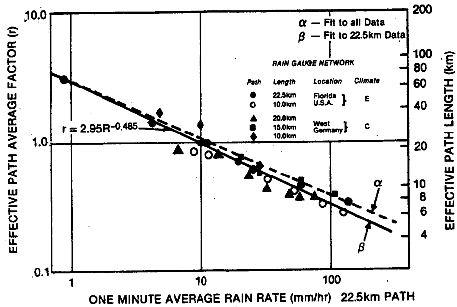
Figure 3.4-11. Effective Path Average Factor Versus Rain Rate
