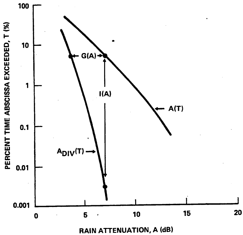
Figure 6.5-2. Definition of Diversity Gain and Diversity Advantage
