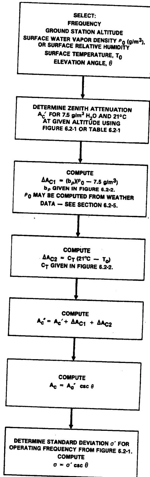
Figure 6.2-3. Technique for Computing Mean Clear Air Attenuation
