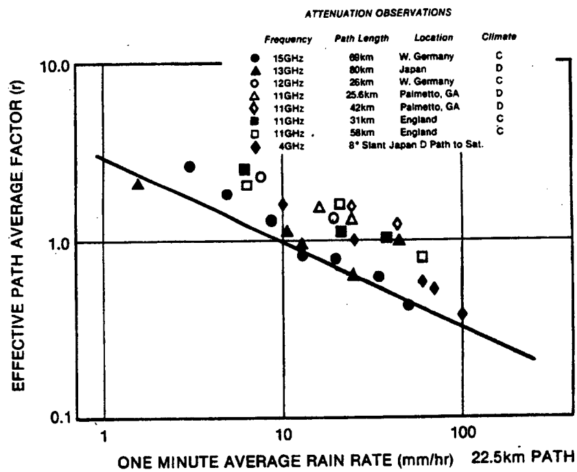
Figure 3.4-12. Effective Path Average Factor Versus Rain Rate Derived from Attenuation Measurements
