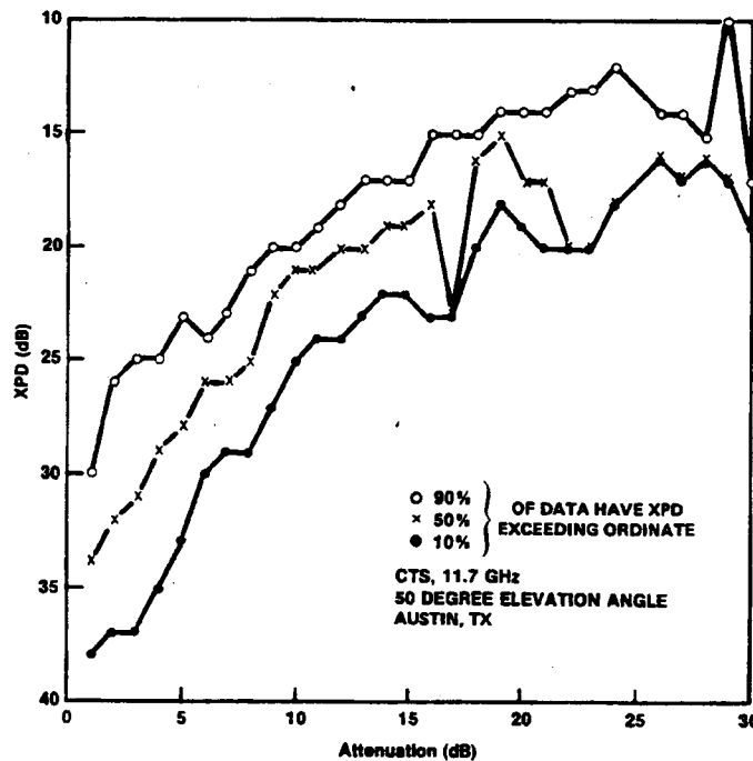
Figure 6.7-2. Twelve Month Isolation Versus Attenuation Data
