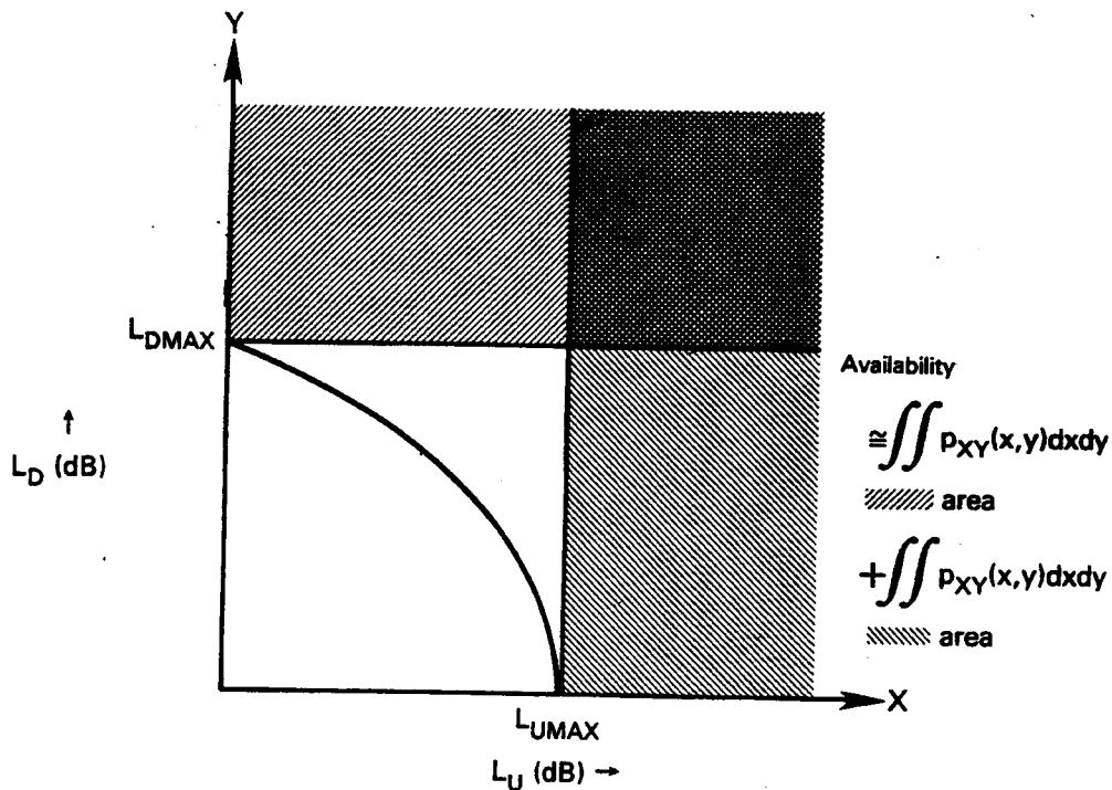
Figure 7.3-8. Approximate Composite Margin Plane Analysis
