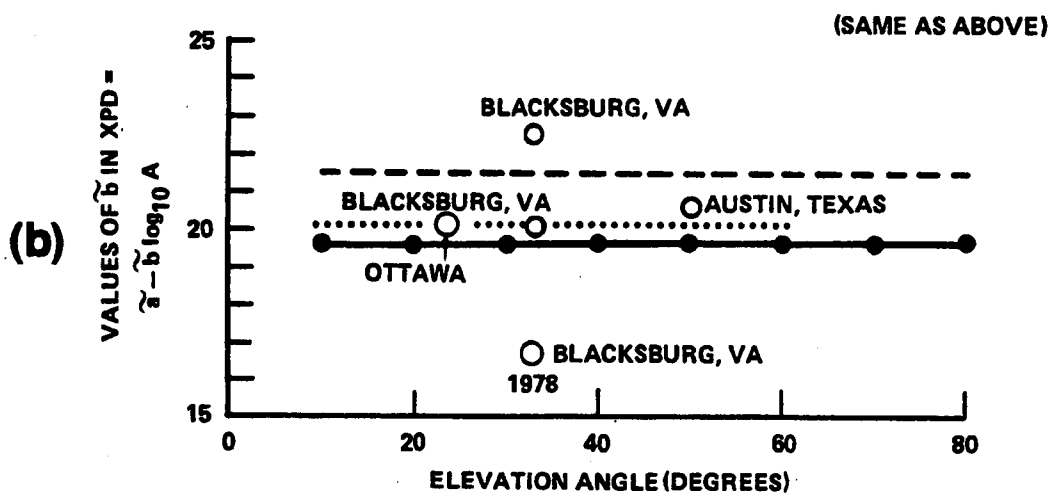
Figure 6.7-4 Elevation Angle Dependence of the Coefficients in the Cross-Polarization Discrimination Relation
