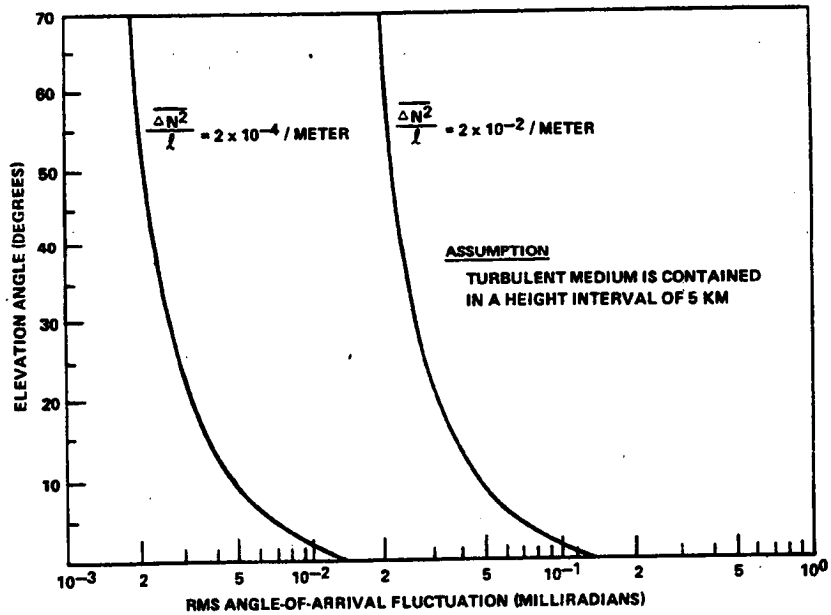
Figure 6.6-12. R.M.S. Angle-of-Arrival Fluctuations for an Earth-Space Path
