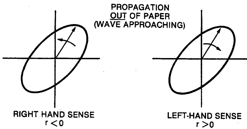
Figure 4.2-2. Definition of Sign of Axial Ratio, r
