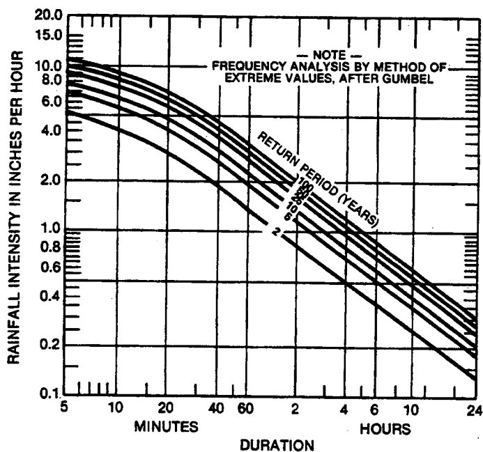
Figure 6.3-11. Typical Rain Rate-Duration-Frequency Curves From U.S. Weather Service, Annual Series
