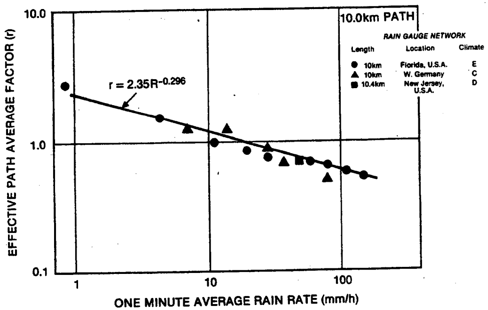
Figure 3.4-10. Effective Path Average Factor Versus Rain Rate, 10 km Path
