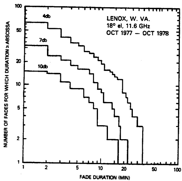
Figure 5.6-1. Histogram of Fade Duration From Radiometer Data
