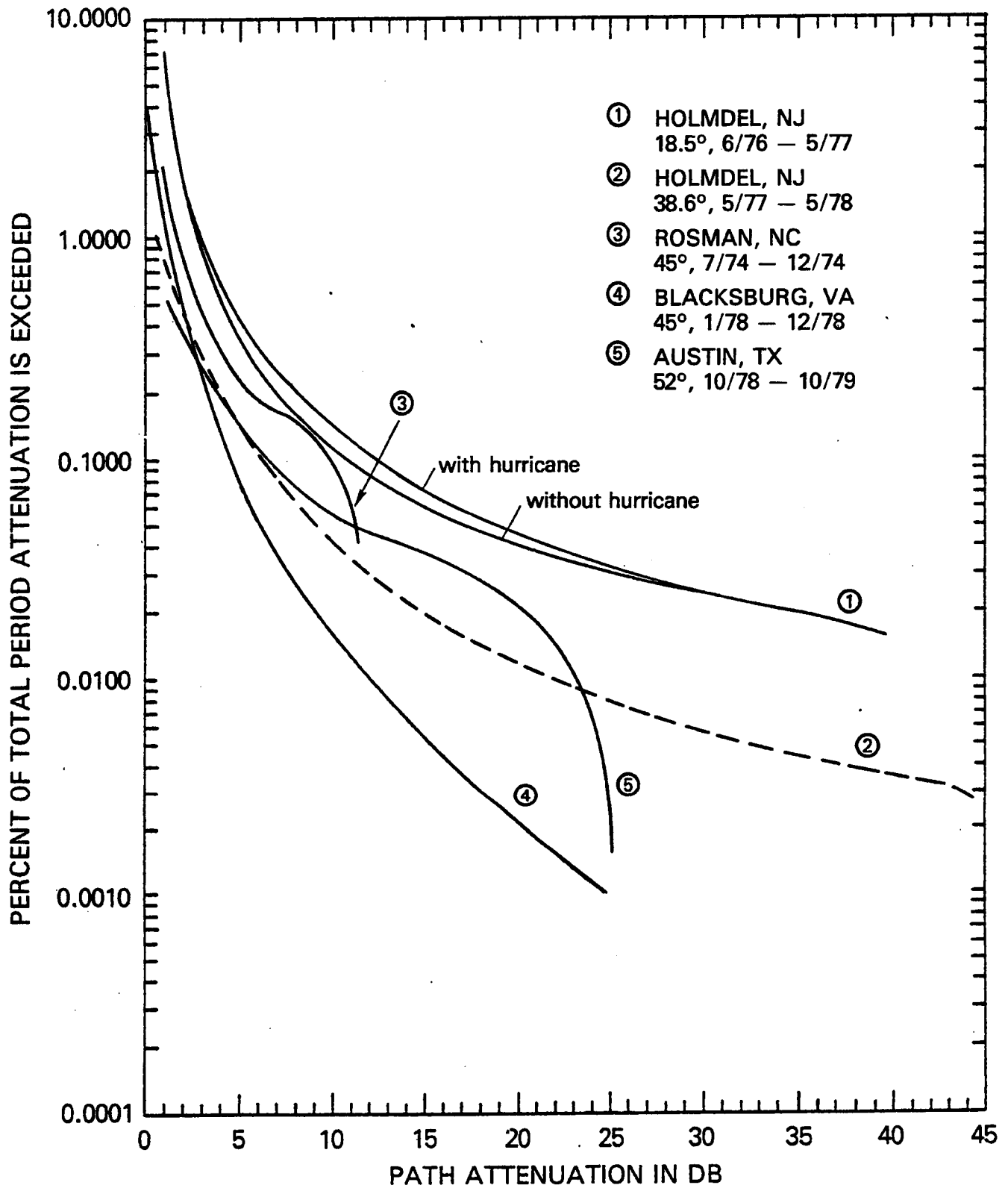
Figure 5.4-11. Summary of 19.04 and 20 GHz Measurements
