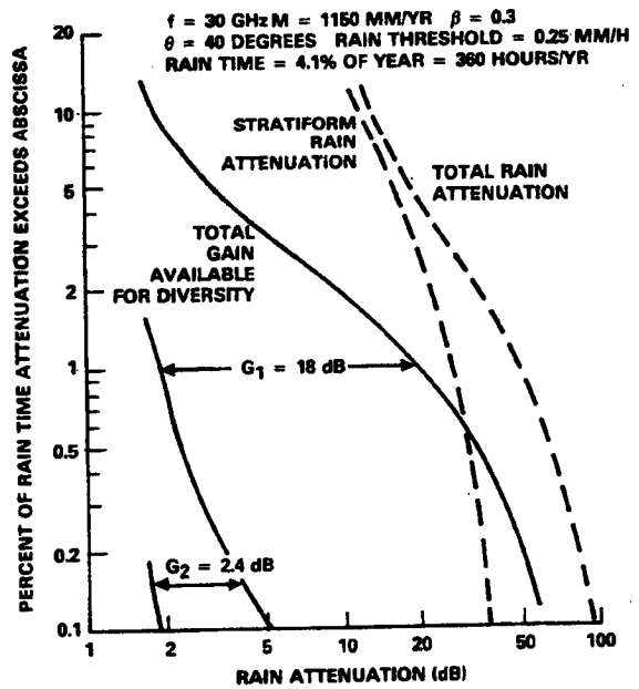
Figure 6.5-7. Cumulative Distribution of Total and Stratiform Rain Attenuation Plus Gain Available for Diversity Systems
