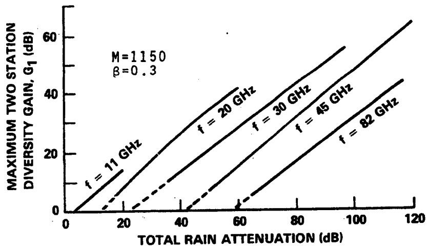
Figure 6.5-9. Maximum Diversity Gain, G_1 Versus Attenuation for Selected Frequencies
