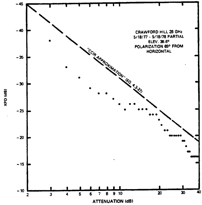
Figure 5.7-3. 28 GHz Crosspolarization Measurements
