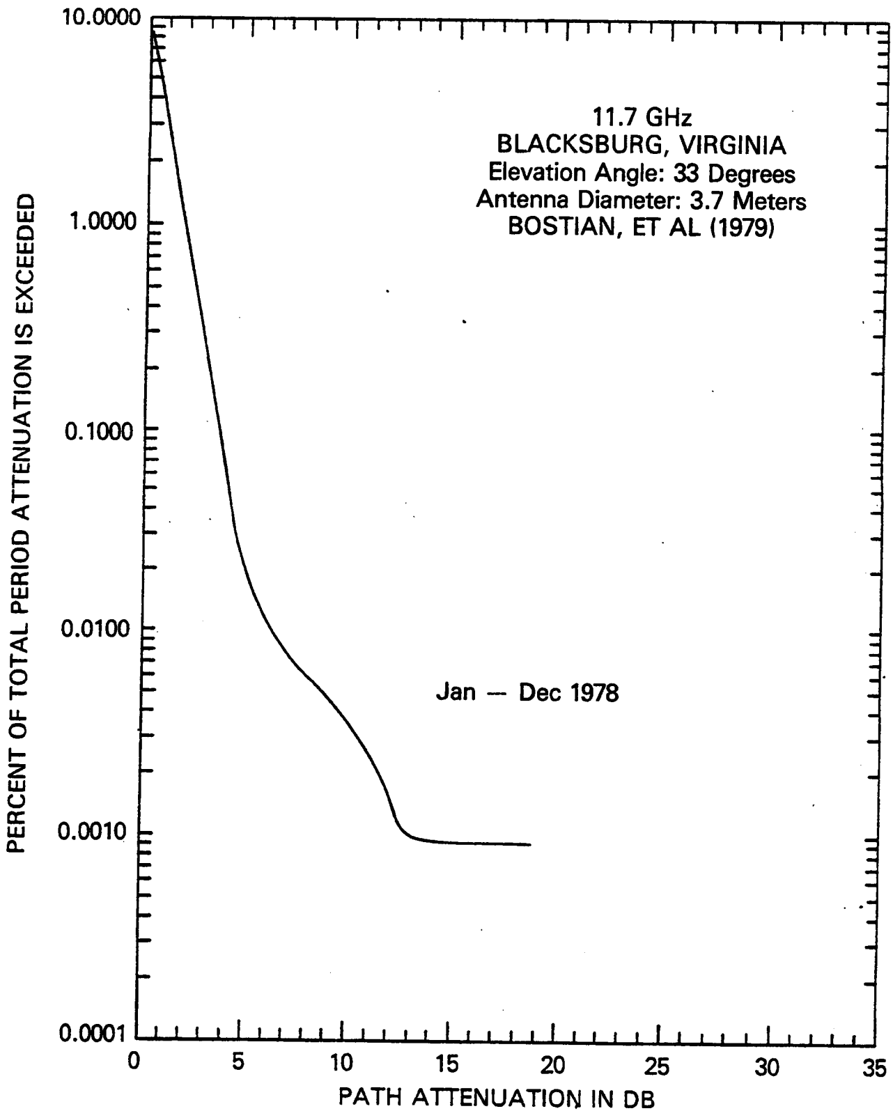
Figure 5.4-4 Annual 11.7 GHz Attenuation Distribution for Blacksburg, Va.
