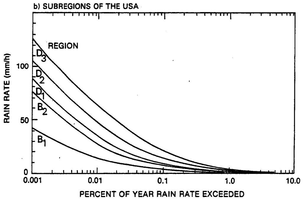
Figure 6.3-3. Point Rain Rate Distributions as a Function of Percent of Year Exceeded
