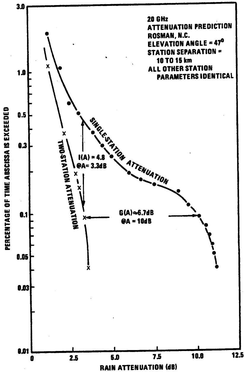
Figure 6.5-10. Path Diversity Gain Statistics for Rosman, N.C.
