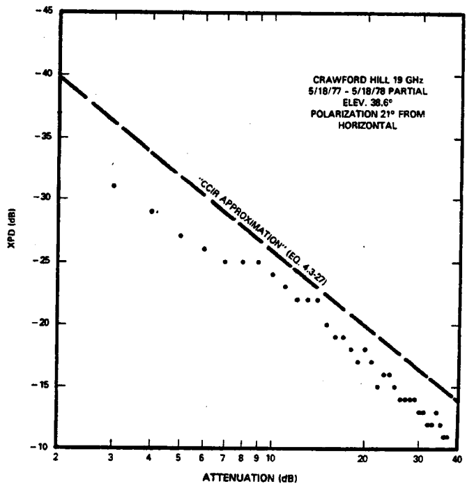
Figure 5.7-2. 19 GHz Cross-Polarization Measurements - Near Horizontal Polarization
