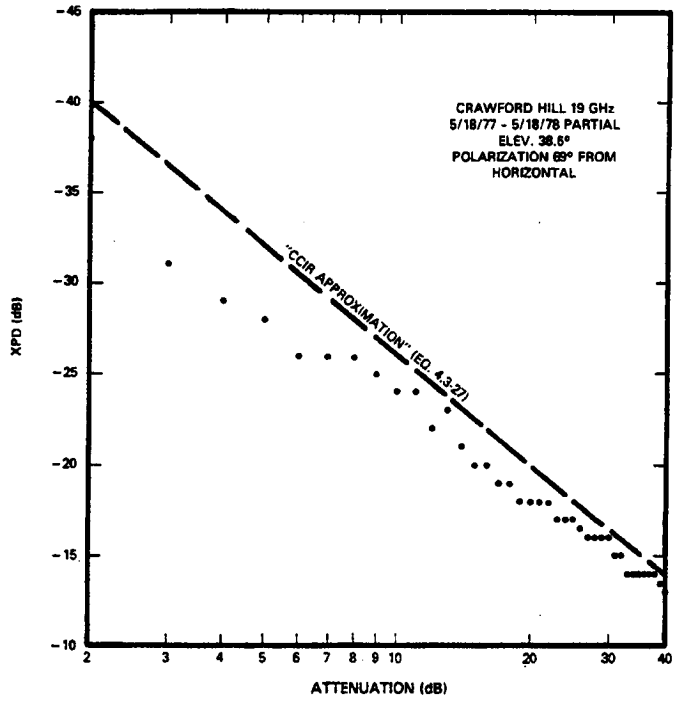
Figure 5.7-1. 19 GHz Cross-Polarization Measurements - Near Vertical Polarization
