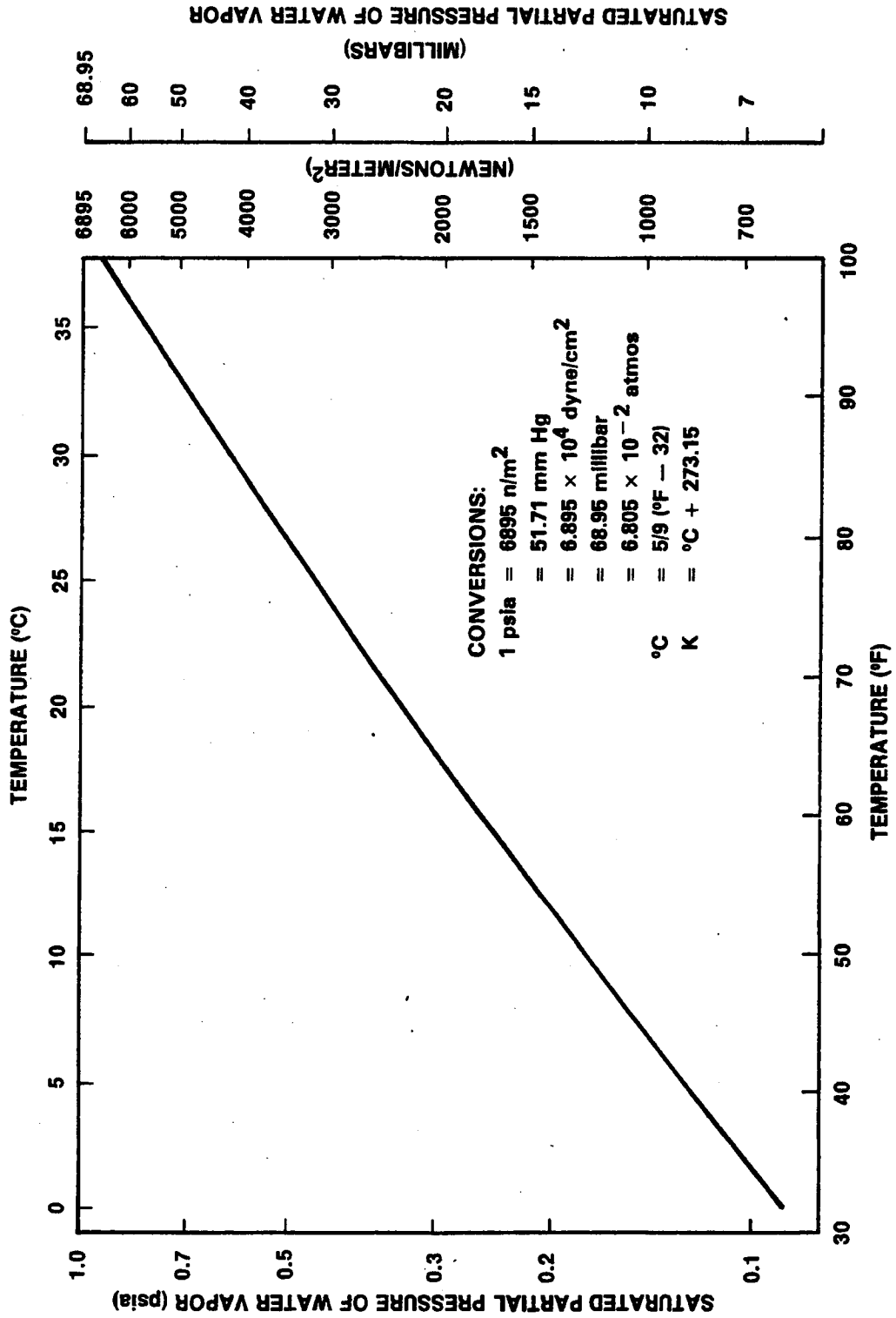
Figure 6.2-4 The Saturated Partial Pressure of Water Vapor Versus Temperature
