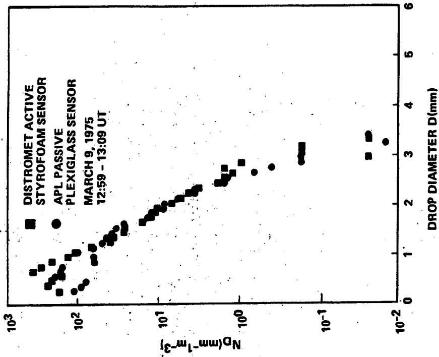
Figure 2.3-2. Raindrop Size Distribution Measured With Two Disdrometers
