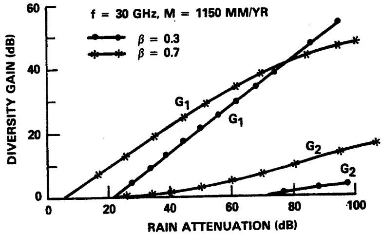
Figure 6.5-8. Maximum Diversity Gains G_1 (Two Stations) and G_2 (Three Stations) Versus Single-Site Attenuation
