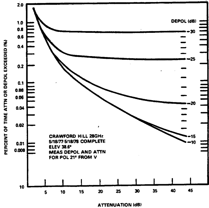
Figure 5.7-4. Joint Attenuation-Depolarization Statistics for 28 GHz Link
