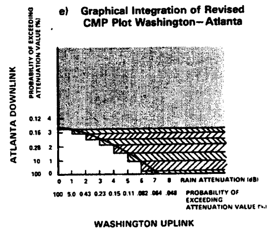
Figure 7.3-7. Composite Margin Plane Availability Analysis (from Kittiver - 1976)
