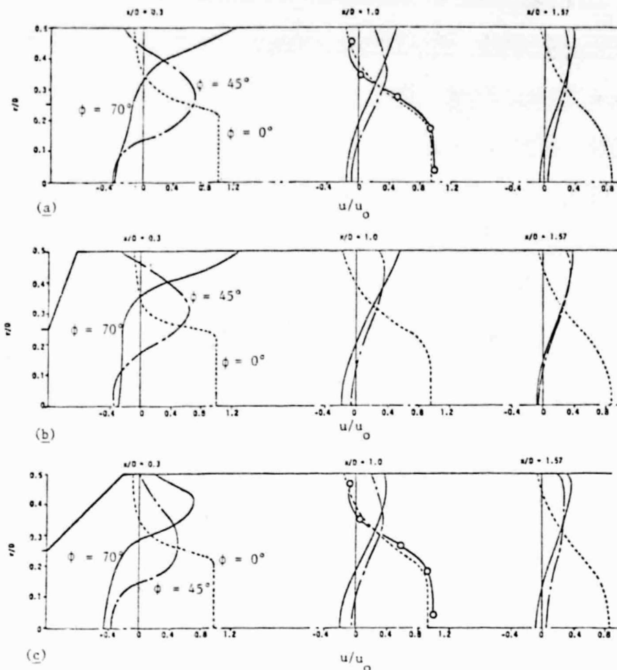
Fig. 5. Predicted axial velocity profiles for Re_d = 1.26 \times 10^5 showing the effect of swirl vane angle \phi for wall expansion angles \alpha : (a) 90^\circ , (b) 70^\circ , and (c) 45^\circ . [ \circ — \circ — \circ Experiment (30) with \phi = 0 and Re_d = 2 \times 10^5 ]
