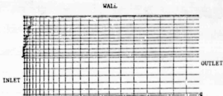
Fig. 3. An example of a coarse grid system being employed to fit the flow domain.
