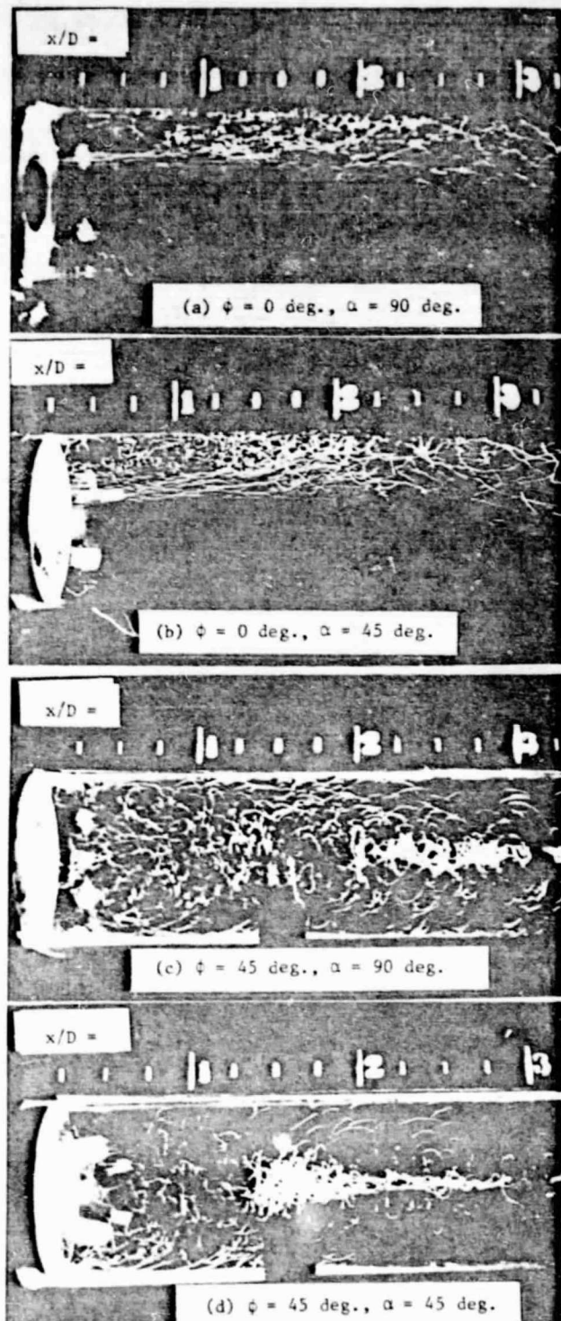
Fig. 10. Flow visualization of pathlines produced by helium-filled soap bubbles for various swirl angles \phi and expansion angles \alpha .
