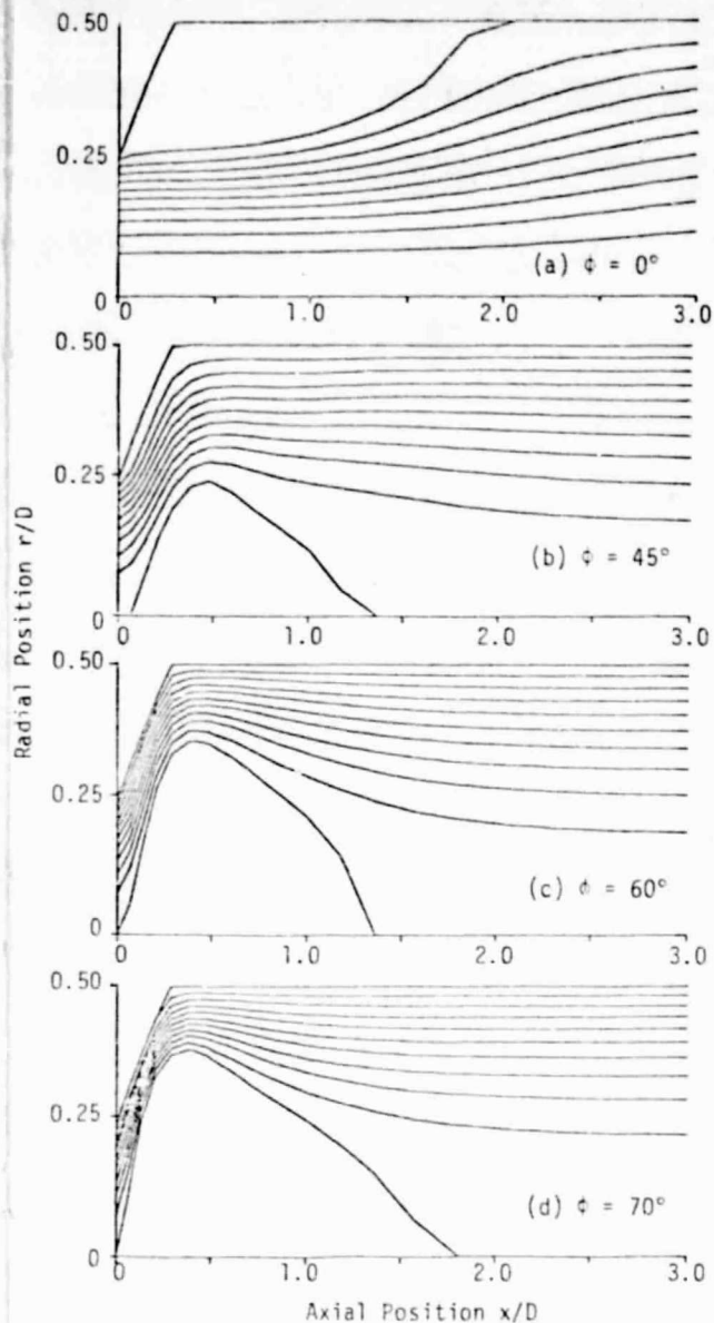
Fig. 9. Predicted streamline plots for a wall expansion angle \alpha = 45^\circ and Re_d = 1.26 \times 10^5 for various swirl vane angles \phi .
