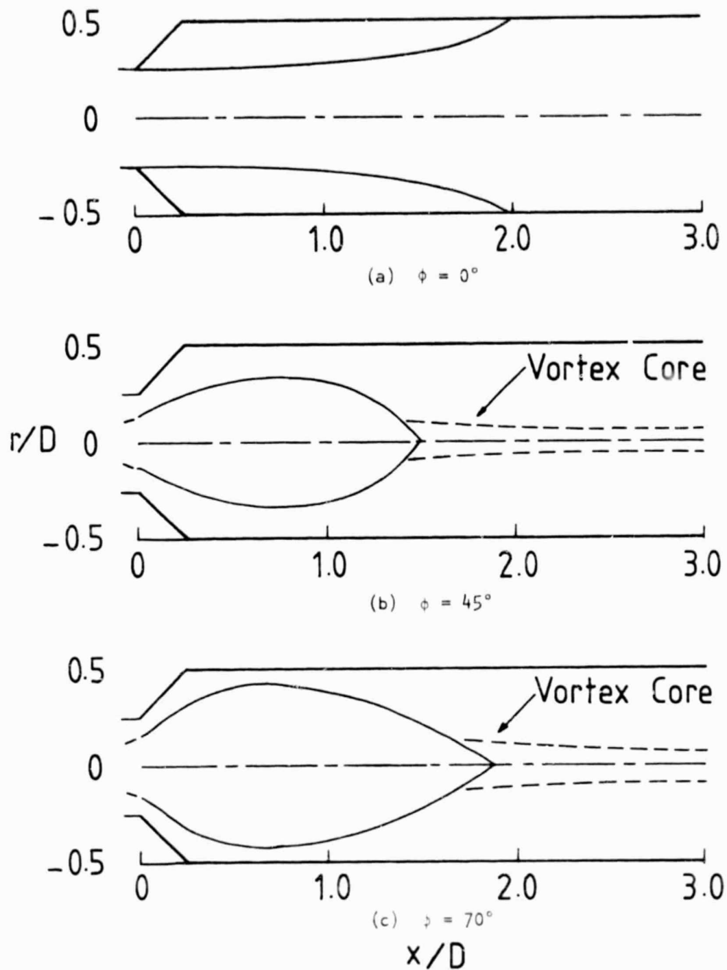
Figure 21. Artistic Impressions of Dividing Streamlines With Wall Expansion Angle \alpha = 45^\circ for Swirl Vane Angles: (a) \phi = 0^\circ , (b) \phi = 45^\circ , and (c) \phi = 70^\circ
