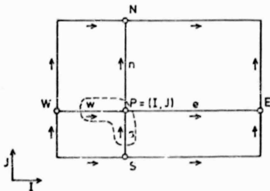
Fig. 2. Staggered grid system and notation.
