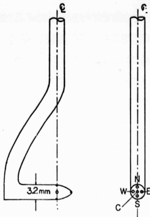
Fig. 3 Five-hole pitot probe.
