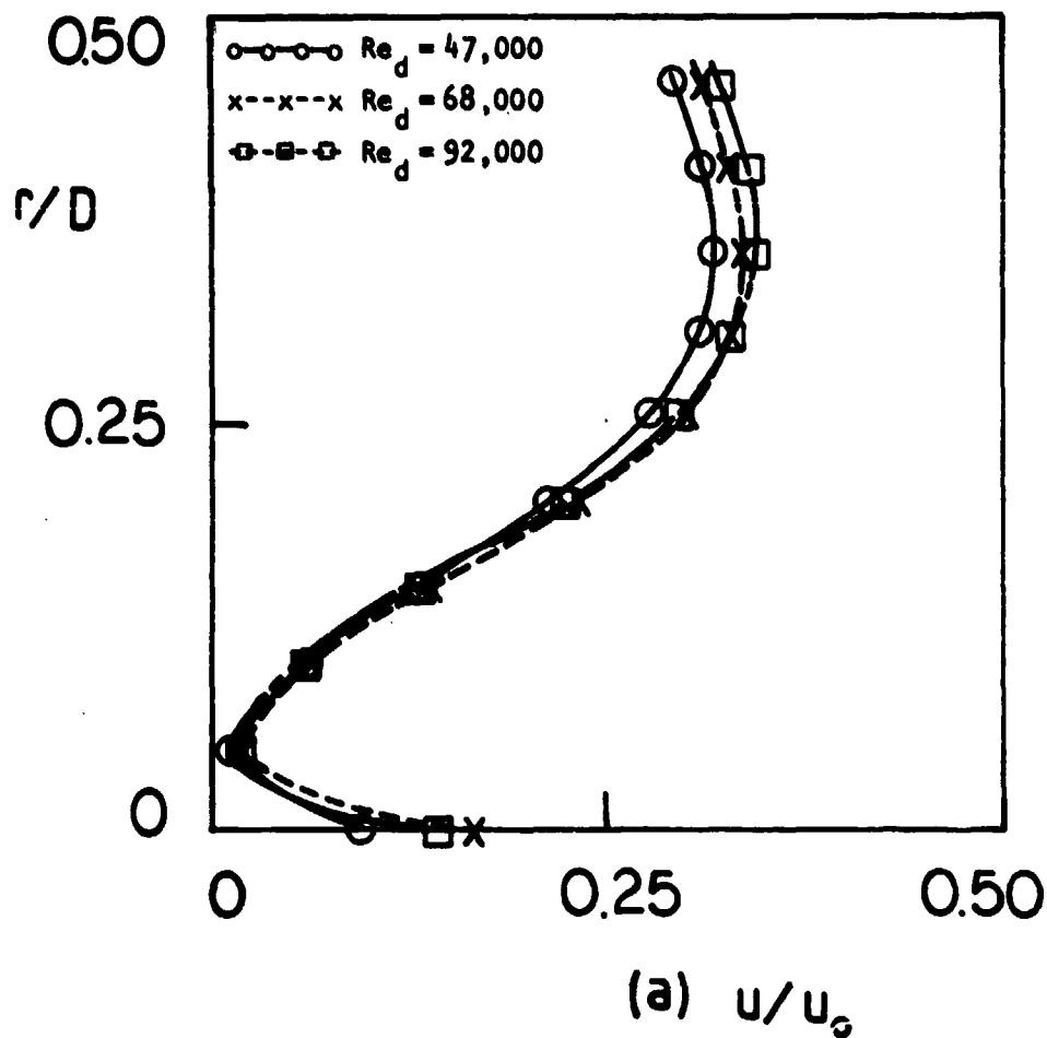
Figure 49. Effect of Inlet Reynolds Number on Measured Velocity Profiles With Wall Expansion Angle \alpha = 90^\circ and Swirl Vane Angle \phi = 45^\circ at Axial Station x/D = 2.5 for (a) Axial Velocity and (b) Swirl Velocity
