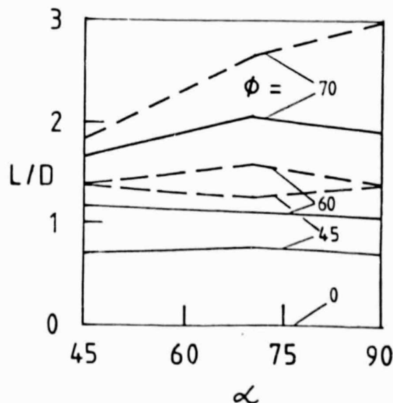
Fig. 13. Predicted effect of sidewall angle \alpha and swirl vane angle \phi on central toroidal recirculation zone CTRZ length. [--- nonreacting, — reacting]
