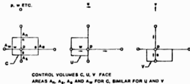
Fig. 3 The three control volumes associated with points of the three grids.
