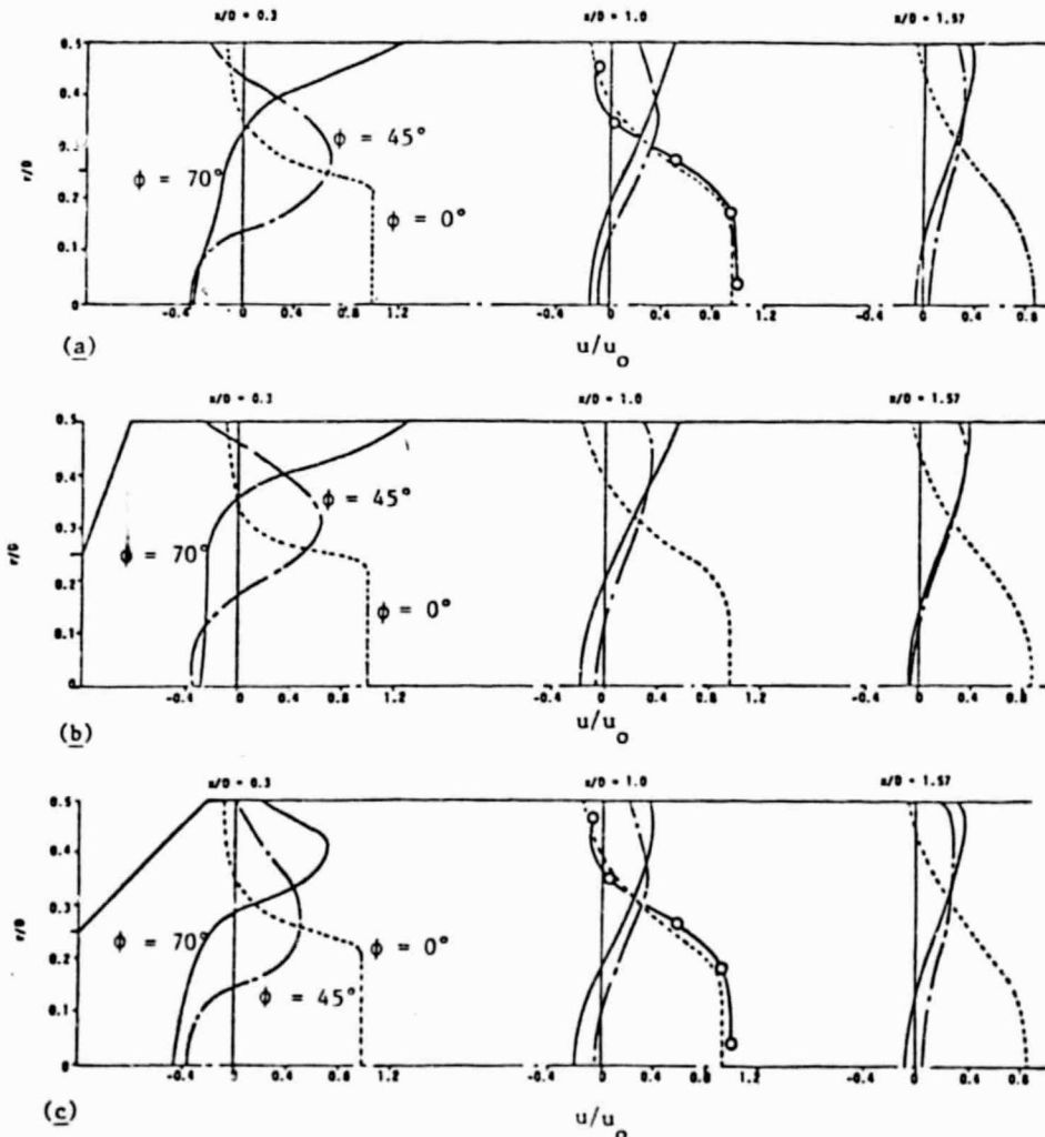
Fig. 7. Predicted axial velocity profiles showing the effect of swirl vane angle \phi for wall expansion angles \alpha : (a) 90^\circ , (b) 70^\circ , and (c) 45^\circ , nonreacting flowfield [o—o—o Experiment 31 with \phi = 0 ]
