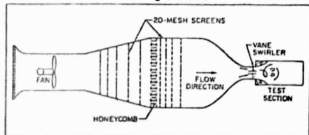
Fig. 2 Schematic of overall flow facility.
