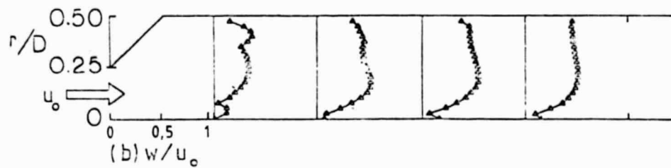
Fig. 16 Measured velocity profiles for wall expansion angle \alpha = 45^\circ and swirl vane angle \phi = 45^\circ .
