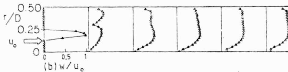
Fig. 13 Measured velocity profiles for wall expansion angle \alpha = 90^\circ and swirl vane angle \phi = 45^\circ .
