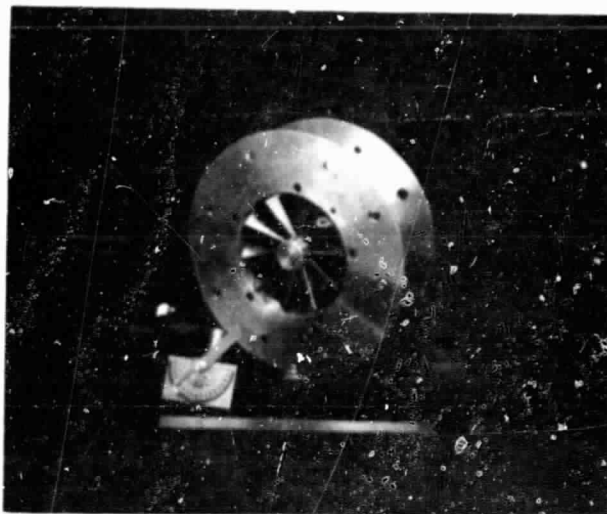
Figure 8. View of the Swirl Vane Assembly From Downstream With the In- strument for Measuring the Vane Angle
