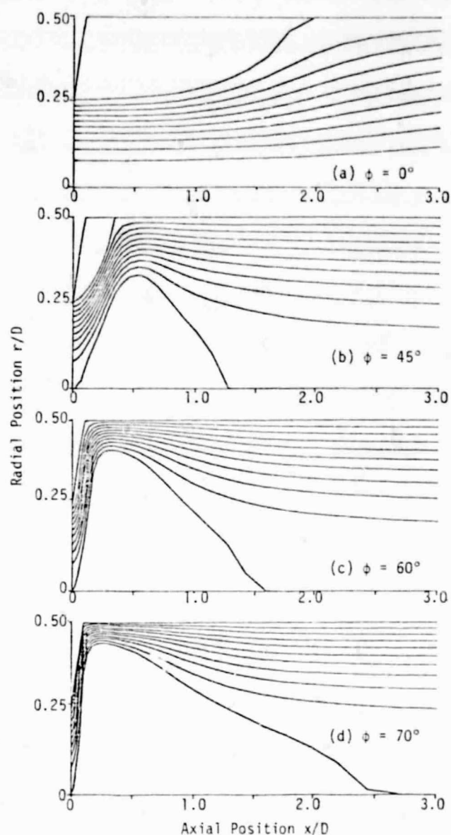
Fig. 8. Predicted streamline plots for a wall expansion angle \alpha = 70^\circ and Re_d = 1.26 \times 10^5 for various swirl vane angles \phi .
