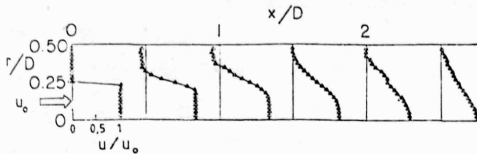
Fig. 12 Measured velocity profiles for wall expansion angle \alpha = 90^\circ and swirl vane angle \phi = 0^\circ .
