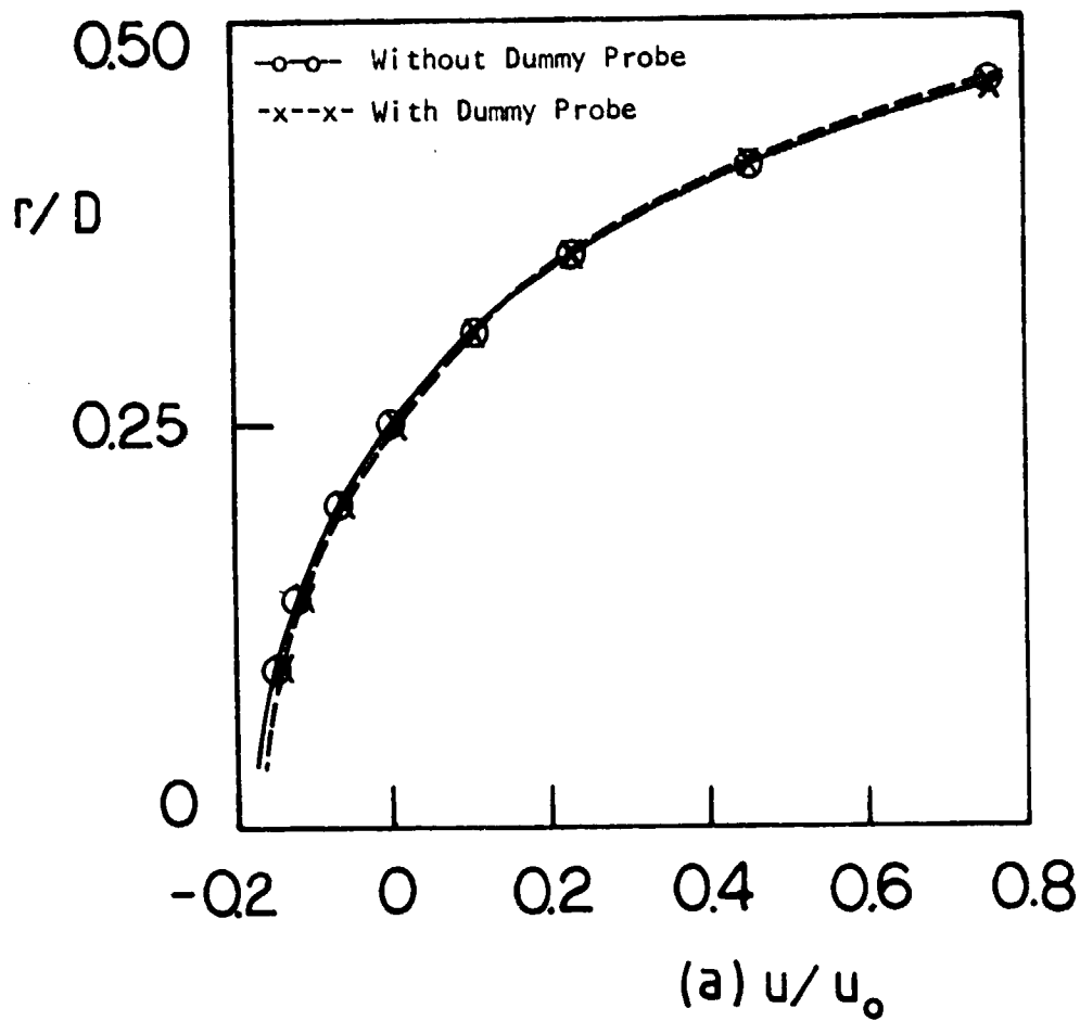
Figure 47. Probe Interference Effect on Measured Velocity Profiles With Wall Expansion Angle \alpha = 90^\circ and Swirl Vane Angle \phi = 45^\circ at Axial Station x/D = 1.0 for (a) Axial Velocity and (b) Swirl Velocity
