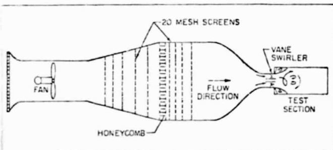
Fig. 4. Schematic of flow facility.
