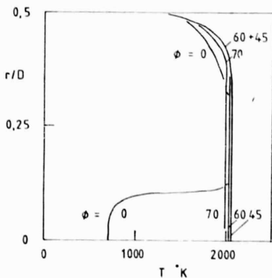
Fig. 11. Temperature profiles at x/D = 0.75 .
