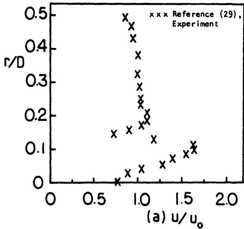
Figure 56. Inlet Velocity Profiles at x/D = 0.01375 ( x = 0.2 cm) for the Coswirling Coannular Pipe Flow Test Case (a) Axial Velocity and (b) Swirl Velocity
