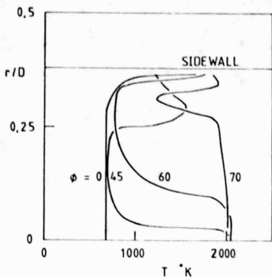
Fig. 10. Temperature profiles at x/D = 0.1 .
