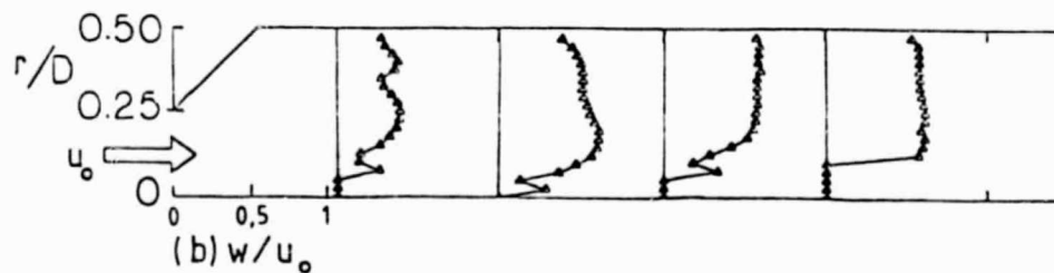
Fig. 17 Measured velocity profiles for wall expansion angle \alpha = 45^\circ and swirl vane angle \phi = 70^\circ .
