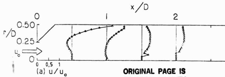
Fig. 16 Measured velocity profiles for wall expansion angle \alpha = 45^\circ and swirl vane angle \phi = 45^\circ .
