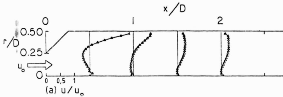
Fig. 15 Measured velocity profiles for wall expansion angle \alpha = 45^\circ and swirl vane angle \phi = 0^\circ .
