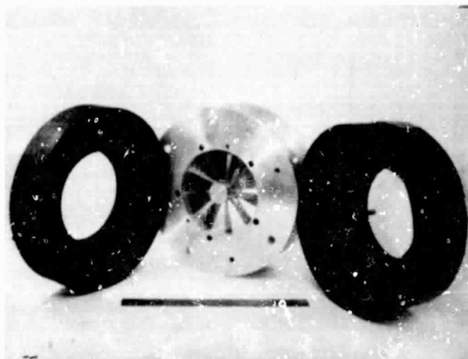
Figure 9. View of Swirler With 70° and 45° Expansion Blocks
