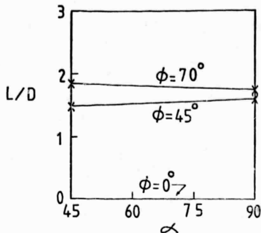
Fig. 11 Experimental effect of wall expansion angle \alpha and swirl vane angle \phi on the central toroidal recirculation zone length.
