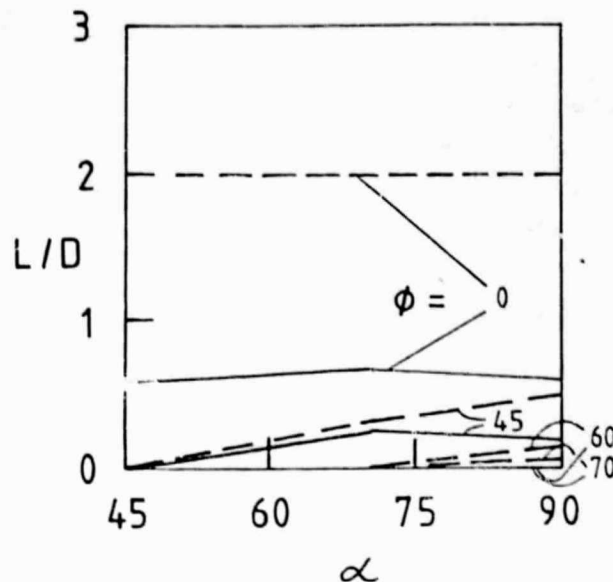
Fig. 12. Predicted effect of sidewall angle \alpha and swirl vane angle \phi on corner recirculation zone CRZ length. [--- nonreacting, — reacting]
