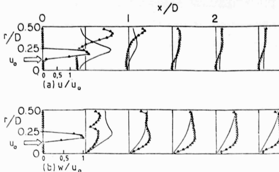
Fig. 18 Predicted and measured velocity profiles for a specific test case with wall expansion angle \alpha = 90^\circ and swirl vane angle \phi = 45^\circ . [— predictions, \Delta - \Delta - \Delta measurements]
