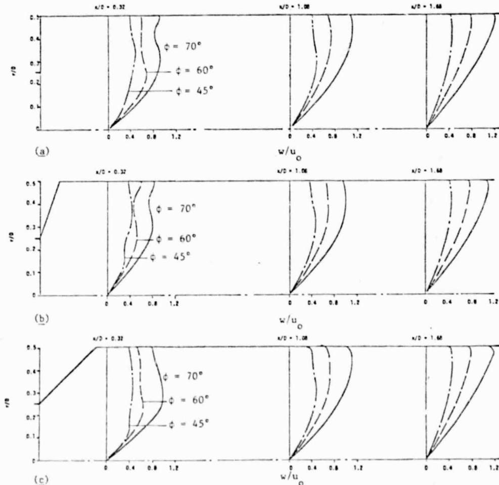
Fig. 6. Predicted swirl velocity profiles for Re_d = 1.26 \times 10^5 showing the effect of swirl vane angle \phi for wall expansion angles \alpha : (a) 90^\circ , (b) 70^\circ , and (c) 45^\circ
