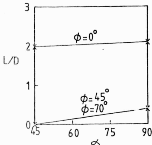
Fig. 10 Experimental effect of wall expansion angle \alpha and swirl vane angle \phi on corner recirculation zone length.
