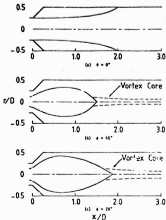
Fig. 6 Artistic impressions of dividing streamlines with wall expansion angle \alpha = 45^\circ for swirl vane angles: (a) \phi = 0^\circ , (b) \phi = 45^\circ , and (c) \phi = 70^\circ .
