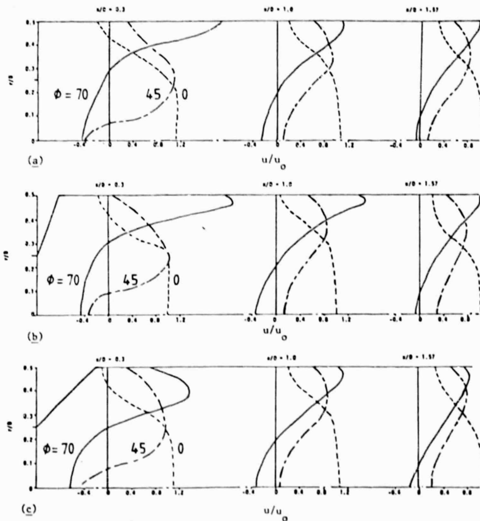
Figure 9. Predicted axial velocity profiles showing the effect of swirl vane angle \phi for wall expansion angles \alpha : (a) 90^\circ , (b) 70^\circ , and (c) 45^\circ , reacting flowfield.
