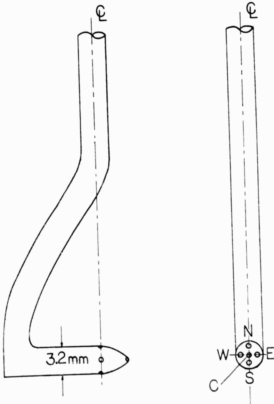
Figure 13. Five-Hole Pitot Probe
