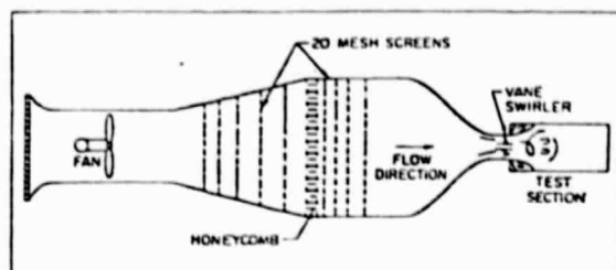
Fig. 2 Schematic of flow facility.
