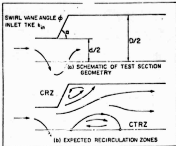
Fig. 1. The flowfield being investigated.
