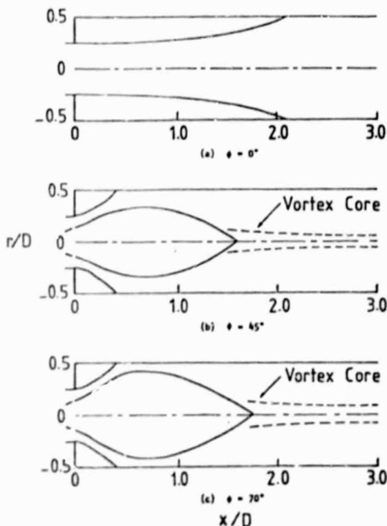
Fig. 5 Artistic impressions of dividing streamlines with wall expansion angle \alpha = 90^\circ for swirl vane angles: (a) \phi = 0^\circ , (b) \phi = 45^\circ , and (c) \phi = 70^\circ .
