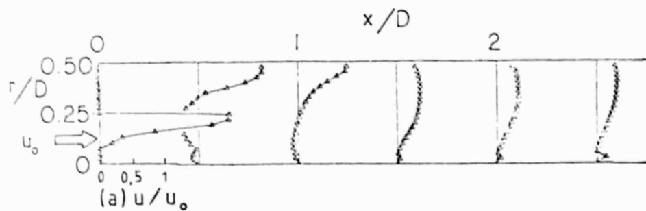
Fig. 13 Measured velocity profiles for wall expansion angle \alpha = 90^\circ and swirl vane angle \phi = 45^\circ .
