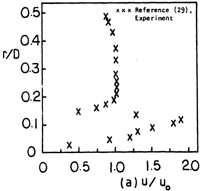
Figure 52. Inlet Velocity Profiles at x/D = 0.01375 ( x = 0.002 m) for the Counterswirling Coannular Pipe Flow Test Case (a) Axial Velocity and (b) Swirl Velocity
