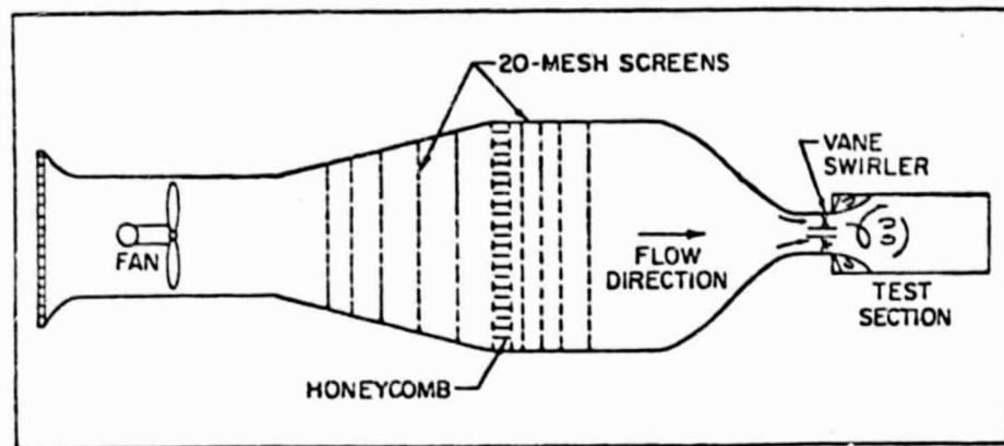
Figure 3. Schematic of Overall Flow Facility
