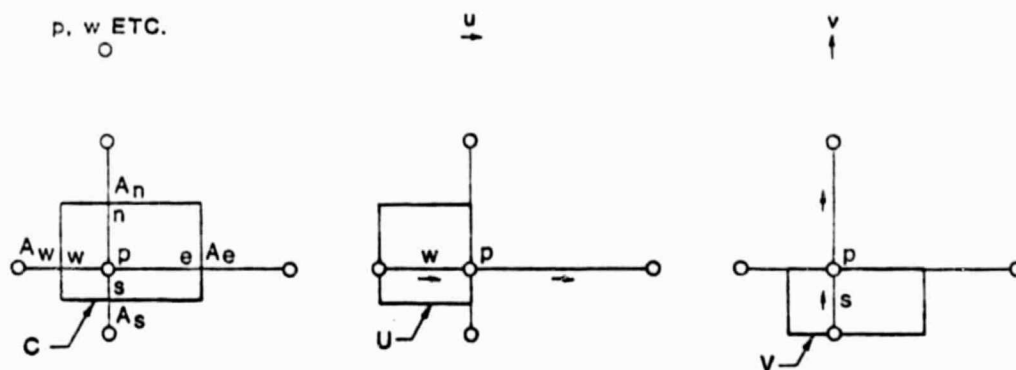
CONTROL VOLUMES C, U, V FACE AREAS A_n , A_s , A_e AND A_w FOR C, SIMILAR FOR U AND V
