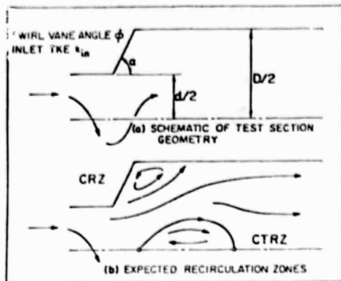
Fig. 1. The flowfield being investigated.
