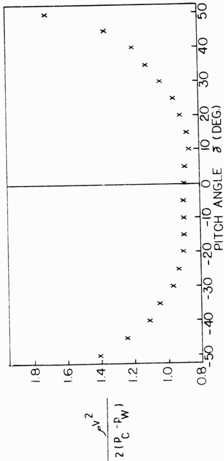
Figure 17. Velocity Coefficient Calibration Characteristic for the Five-Hole Pitot Probe
