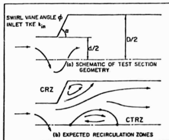
Fig. 1 The flowfield being investigated.
