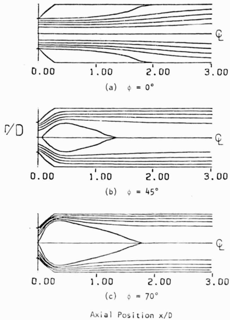
Figure 31. Predicted Streamline Plots With Wall Expansion Angle \alpha = 45^\circ for Swirl Vane Angles: (a) \phi = 0^\circ , (b) \phi = 45^\circ , and (c) \phi = 70^\circ
