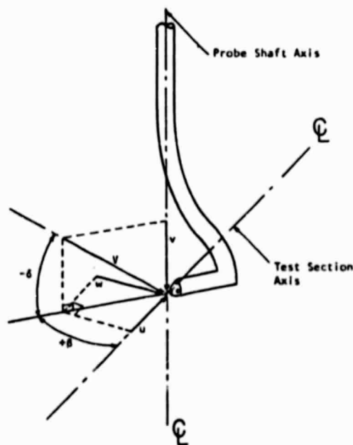
Fig. 4 Velocity components and flow direction angles associated with five-hole pitot measurements (yaw angle \beta in the horizontal plane and pitch angle \delta in the vertical plane).
