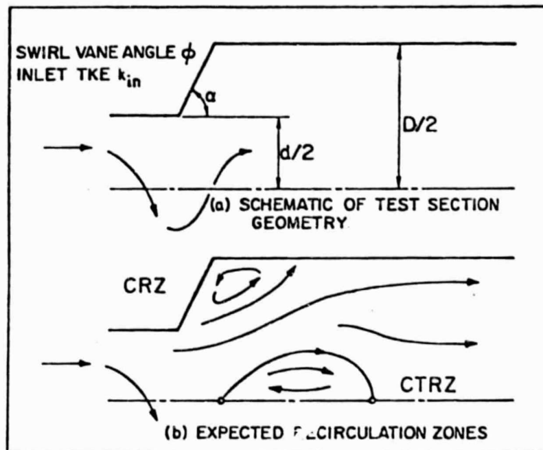
Figure 2. The Flowfield Being Investigated
