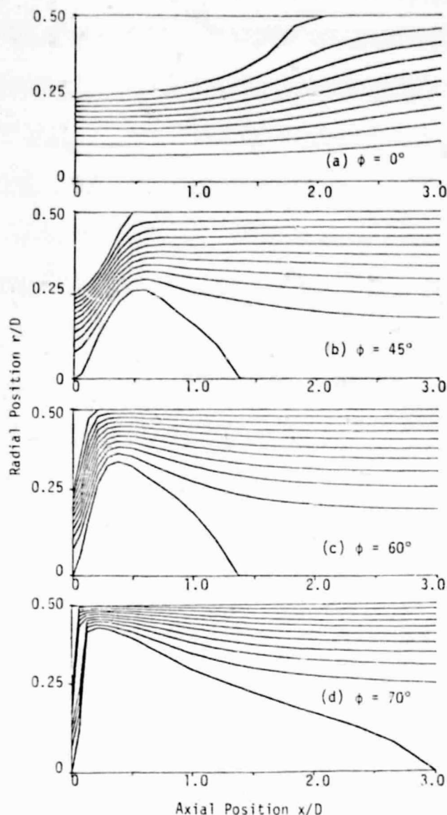
Fig. 7. Predicted streamline plots for a wall expansion angle \alpha = 90^\circ and Re_d = 1.26 \times 10^5 for various swirl vane angles \phi .
