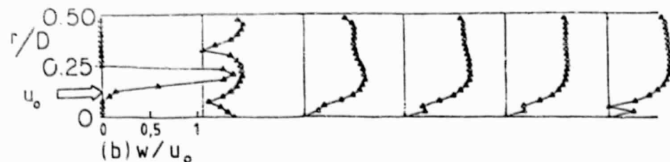
Fig. 14 Measured velocity profiles for wall expansion angle \alpha = 90^\circ and swirl vane angle \phi = 70^\circ .
