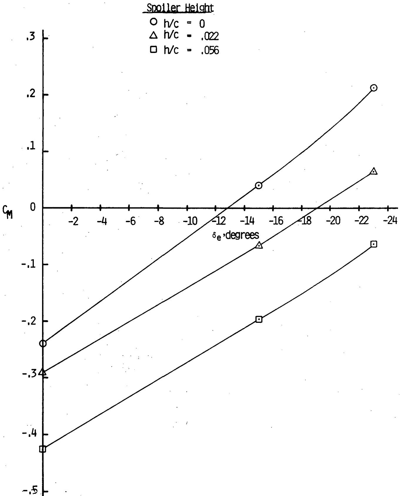
Figure 23. Variation of Pitching Moment Coefficient with Elevator Deflection; 77 hhp, 30° Flaps, \alpha = 10^\circ
