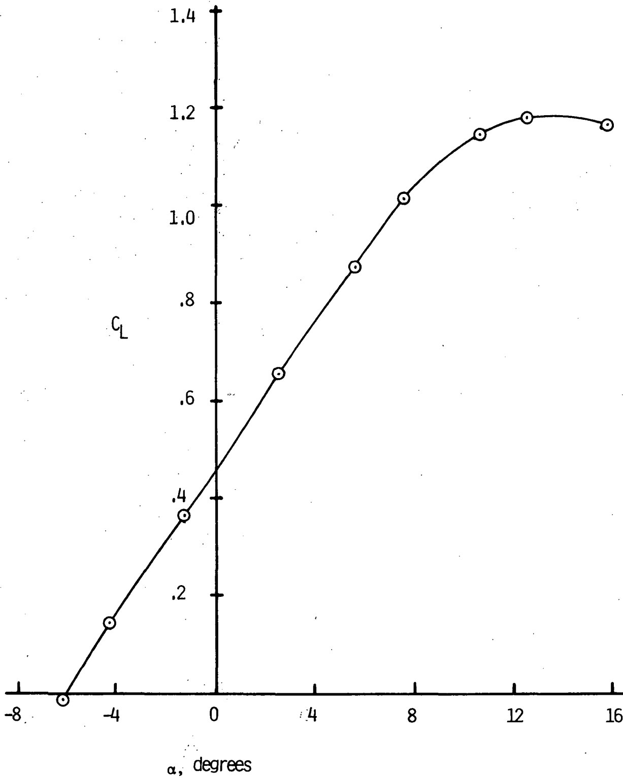
Figure 17. Variation of Lift Coefficient with Angle of Attack; Power off, Wing-Body
