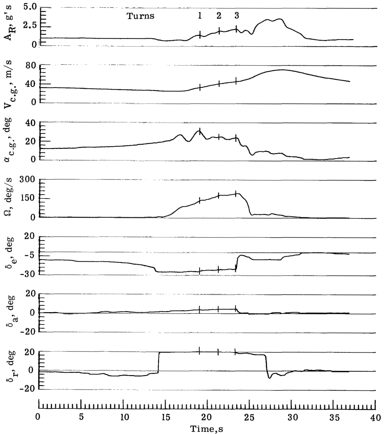
Figure 20.- Elevator-only recovery from 3-turn left spin with PLF @ V_i = 29 m/s.
