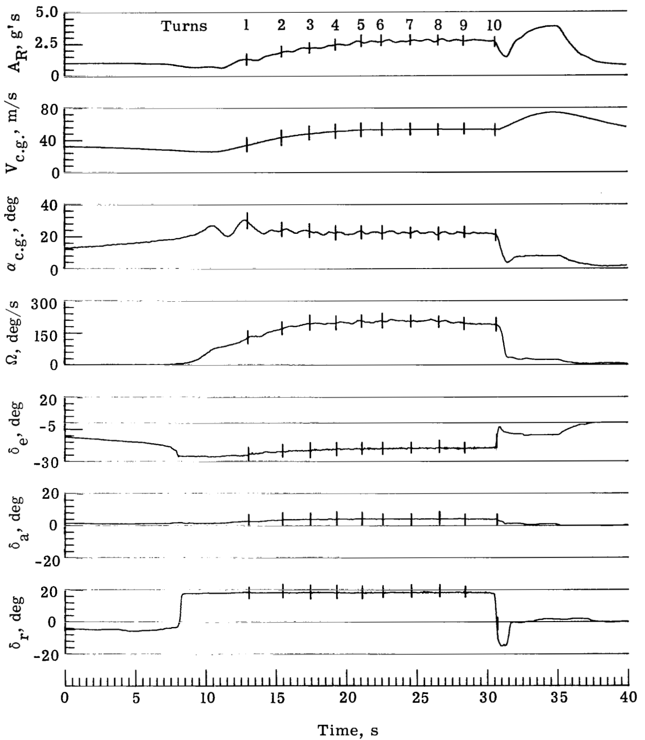
Figure 12.- Ten-turn left spin with PLF @ V_i = 29 m/s.
