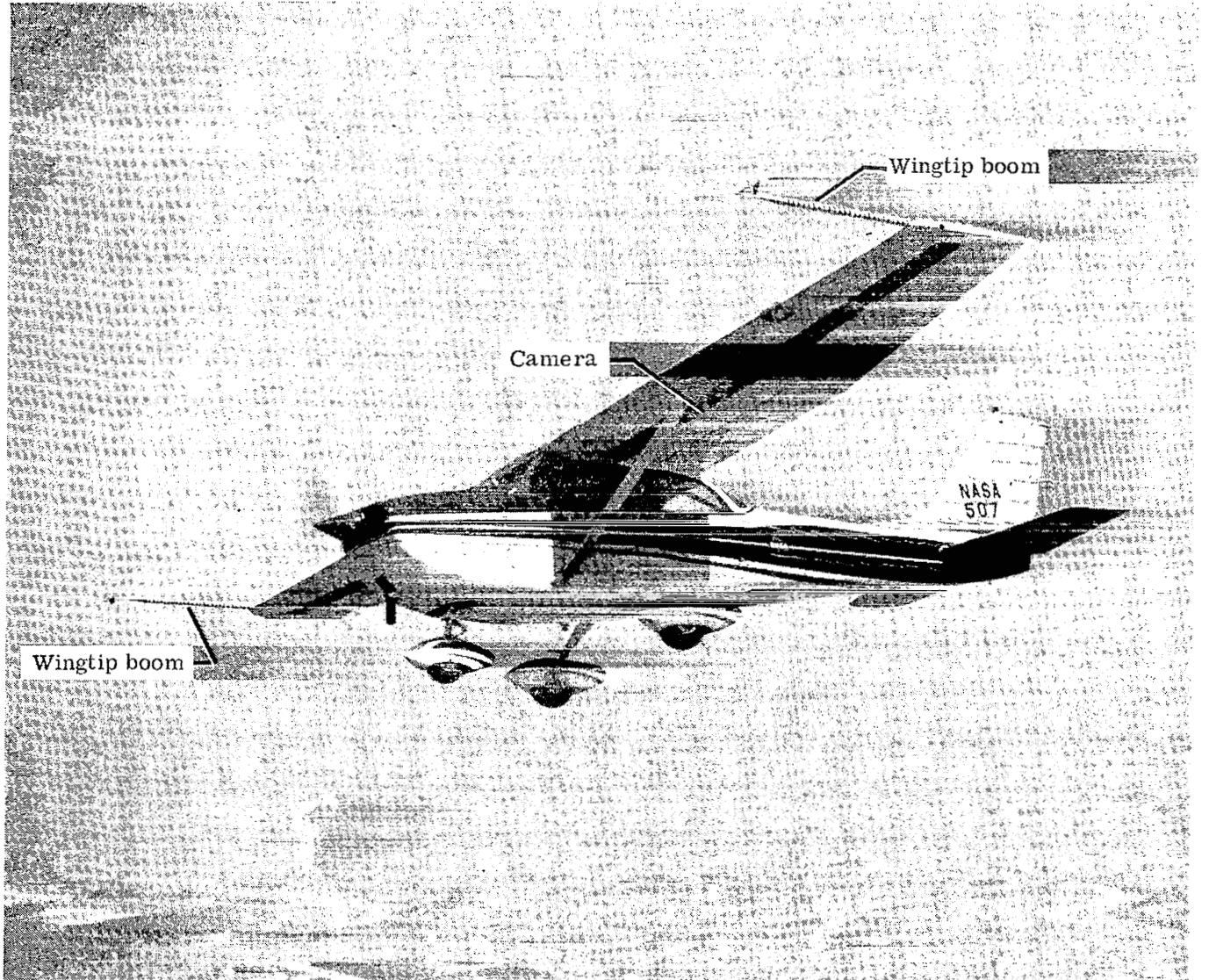
Figure 2.- Test airplane.
