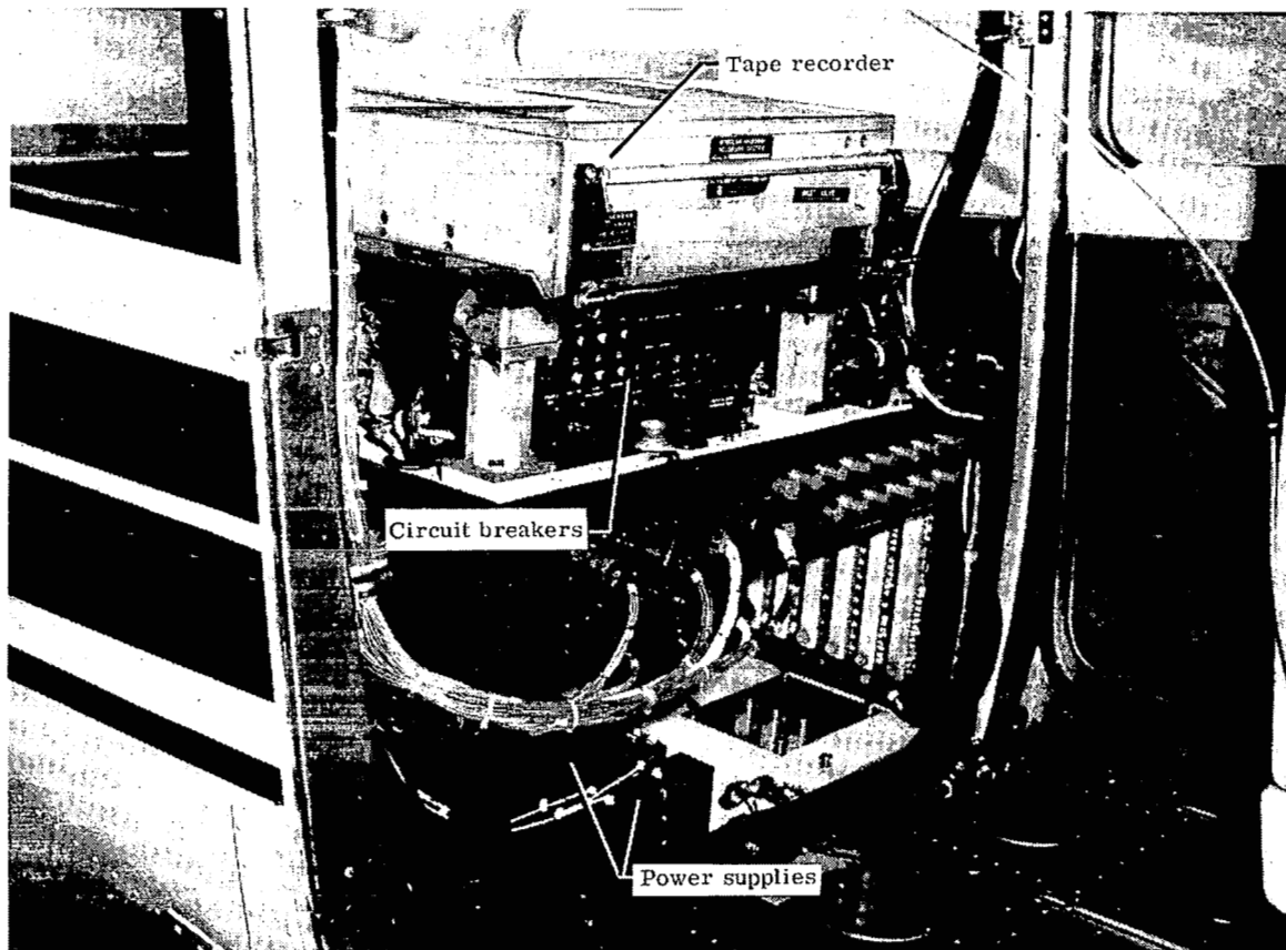
Figure 3.- Instrumentation pallet.
