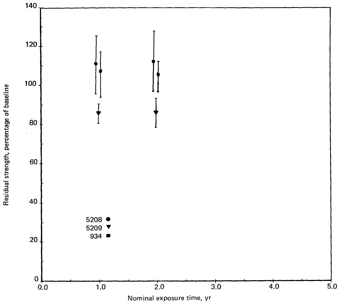
Figure 43. \pm 45 -deg Tension— 82^{\circ}\text{C} ( 180^{\circ}\text{F} )
