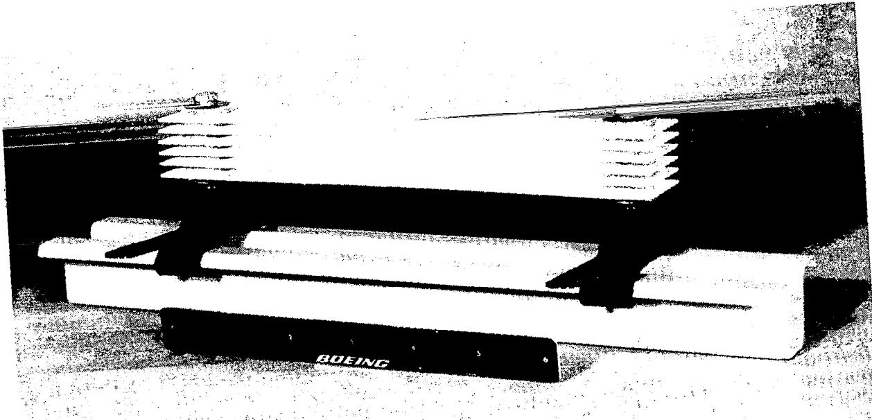
Figure 21. Interior Aircraft Tension Specimen Fixture
