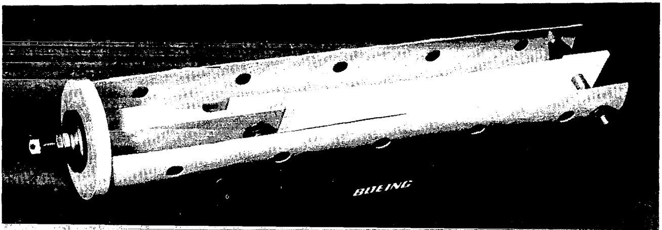
Figure 15. Cutaway of Stressed Tension Specimen Fixture
