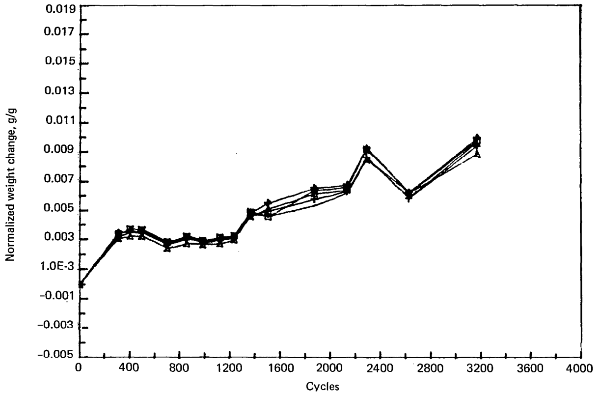
Figure 62. Weight Change of Unpainted 934 as a Function of Ground-Air-Ground Cycles
