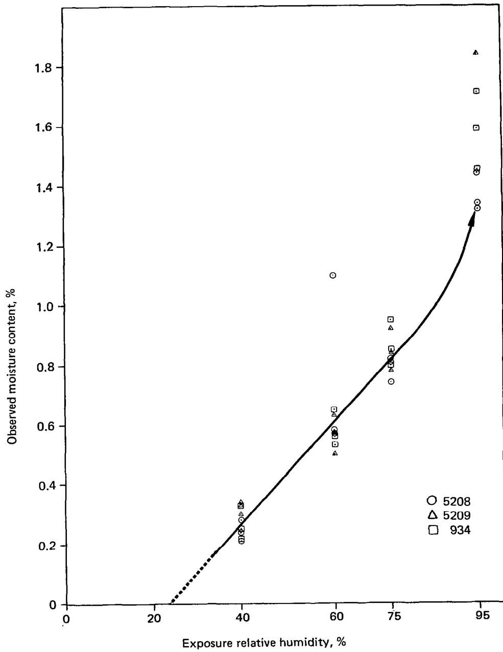
Figure 55. Moisture Content as a Function of Humidity
