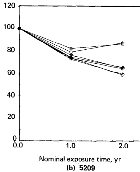
Figure 36. Individual Results, Short Beam Shear—Room Temperature
