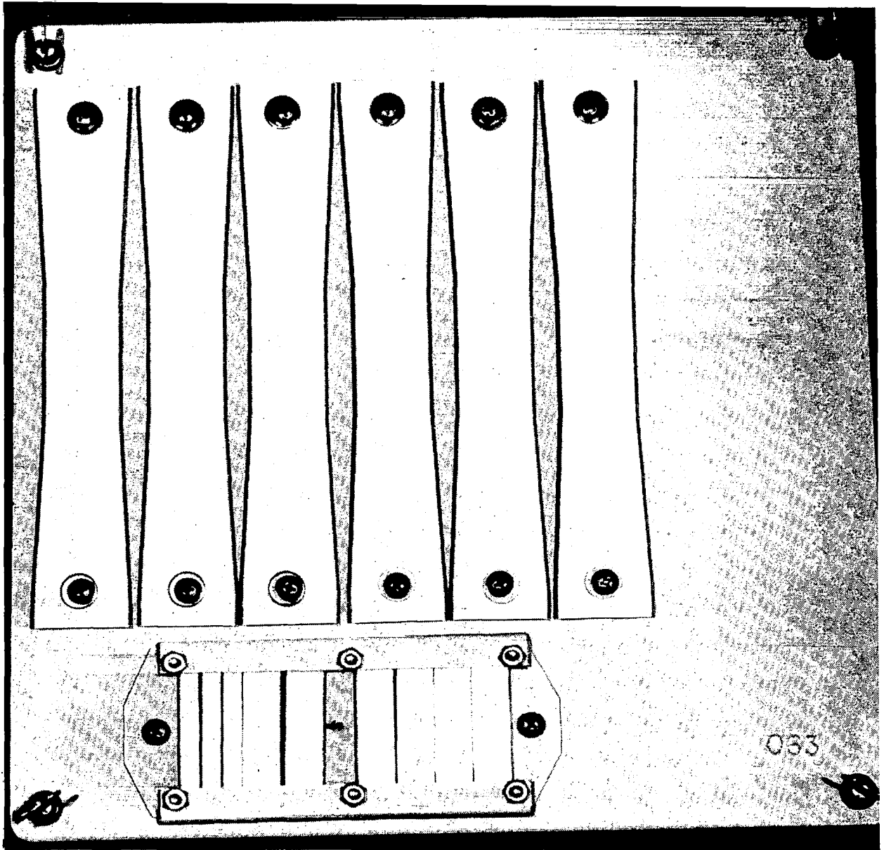
Figure 23. Solar Ground Exposure Insert Panel
