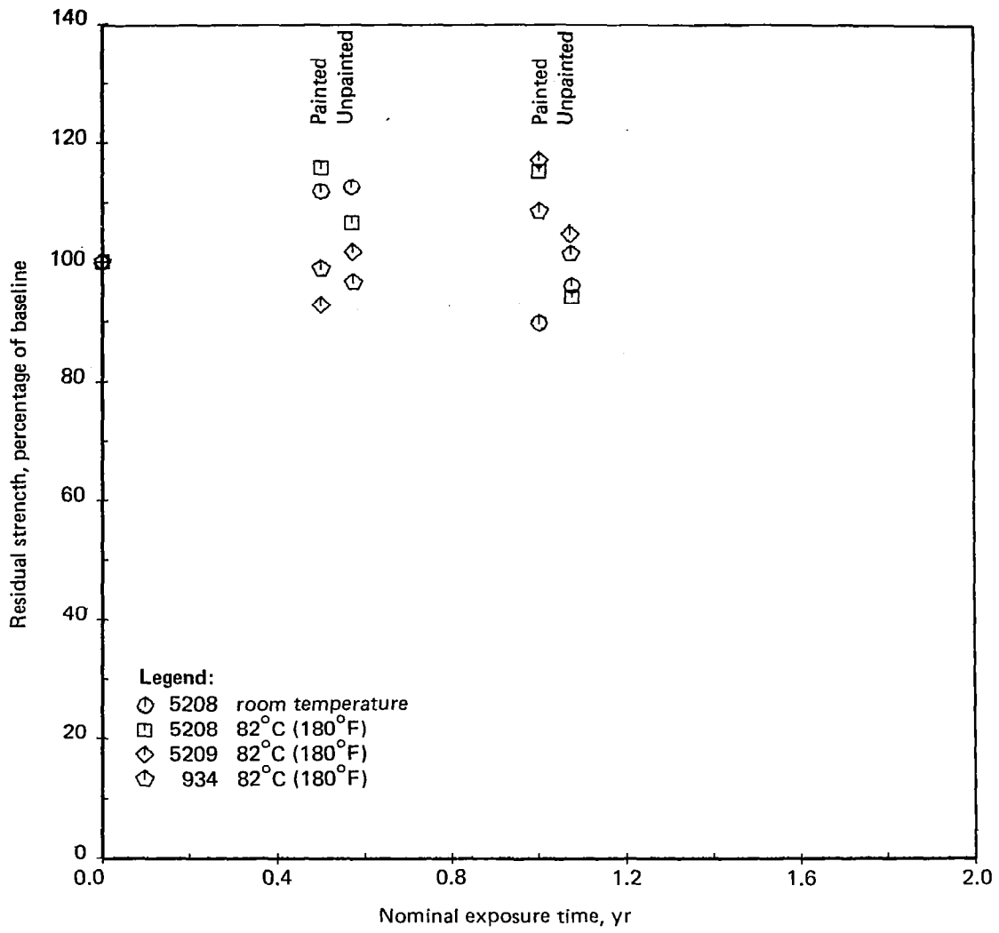
Figure 59. Weatherometer Flexure Strength Results
