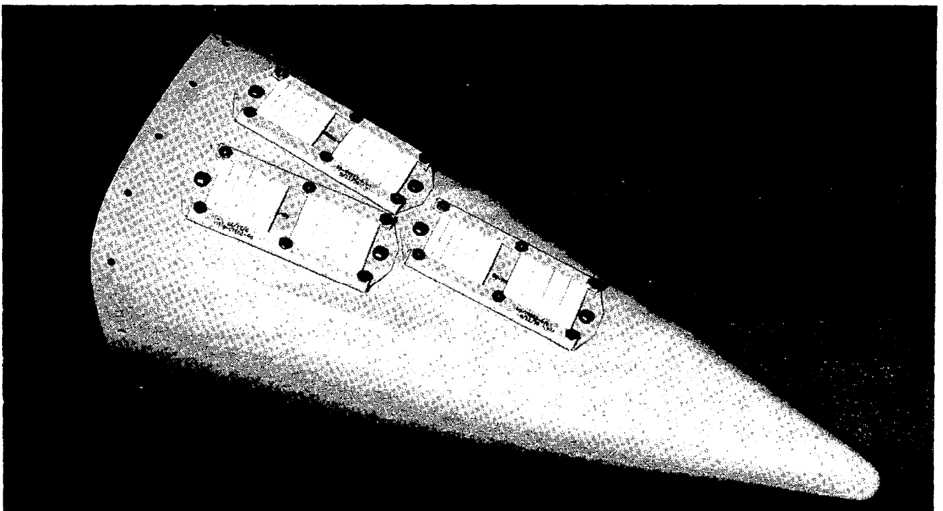
Figure 17. Tailcone With Shear and Flexure Specimen Fixtures Attached
