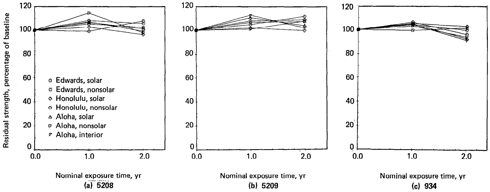
Figure 40. Individual Results, Flexure—Room Temperature
