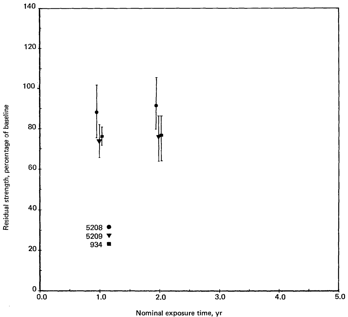
Figure 35. Short Beam Shear—82°C (180°F)
