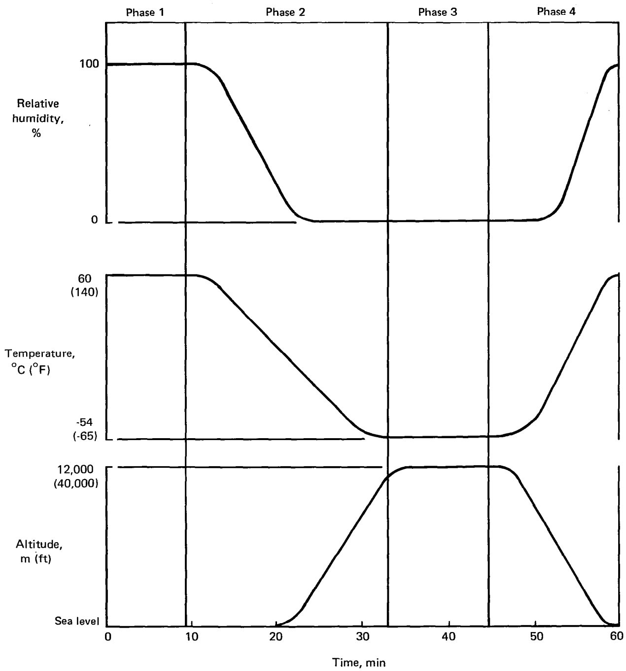
Figure 33. Webber Chamber and Ground-Air-Ground Cycle Detail
