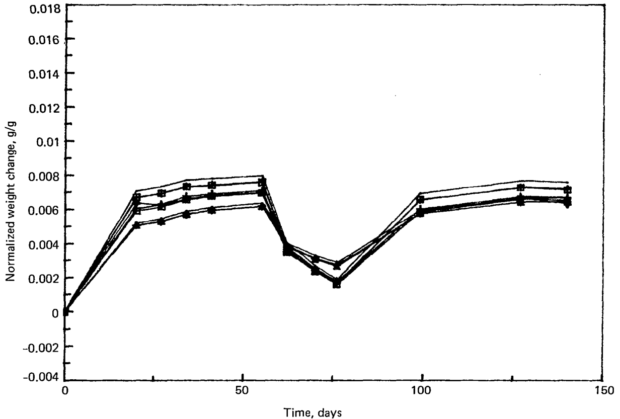
Figure 52. Normalized Weight Change for 75% Relative Humidity Exposure
