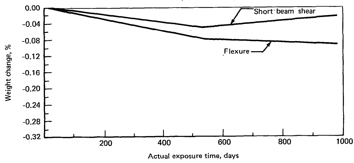
Figure 50. Time Alone Weight Change Results
