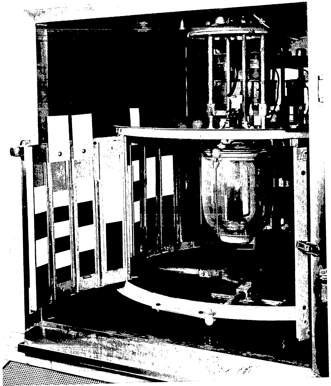
Figure 30. Interior of Weatherometer Exposure Chamber
