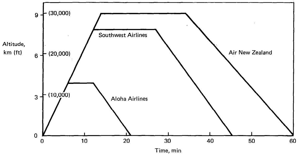
Figure 12. Typical Flight Profiles
