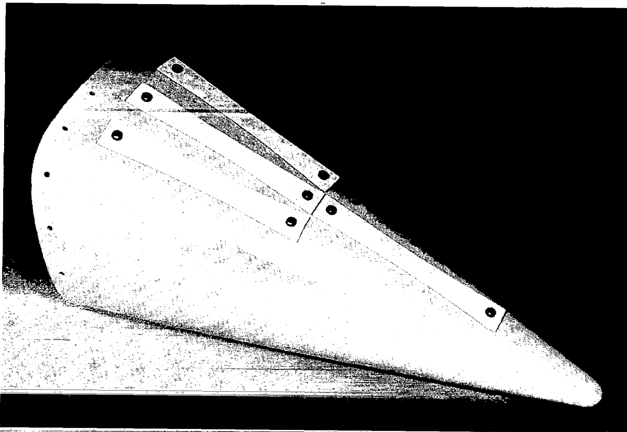
Figure 18. Tailcone With \pm 45 Tension Specimens Attached
