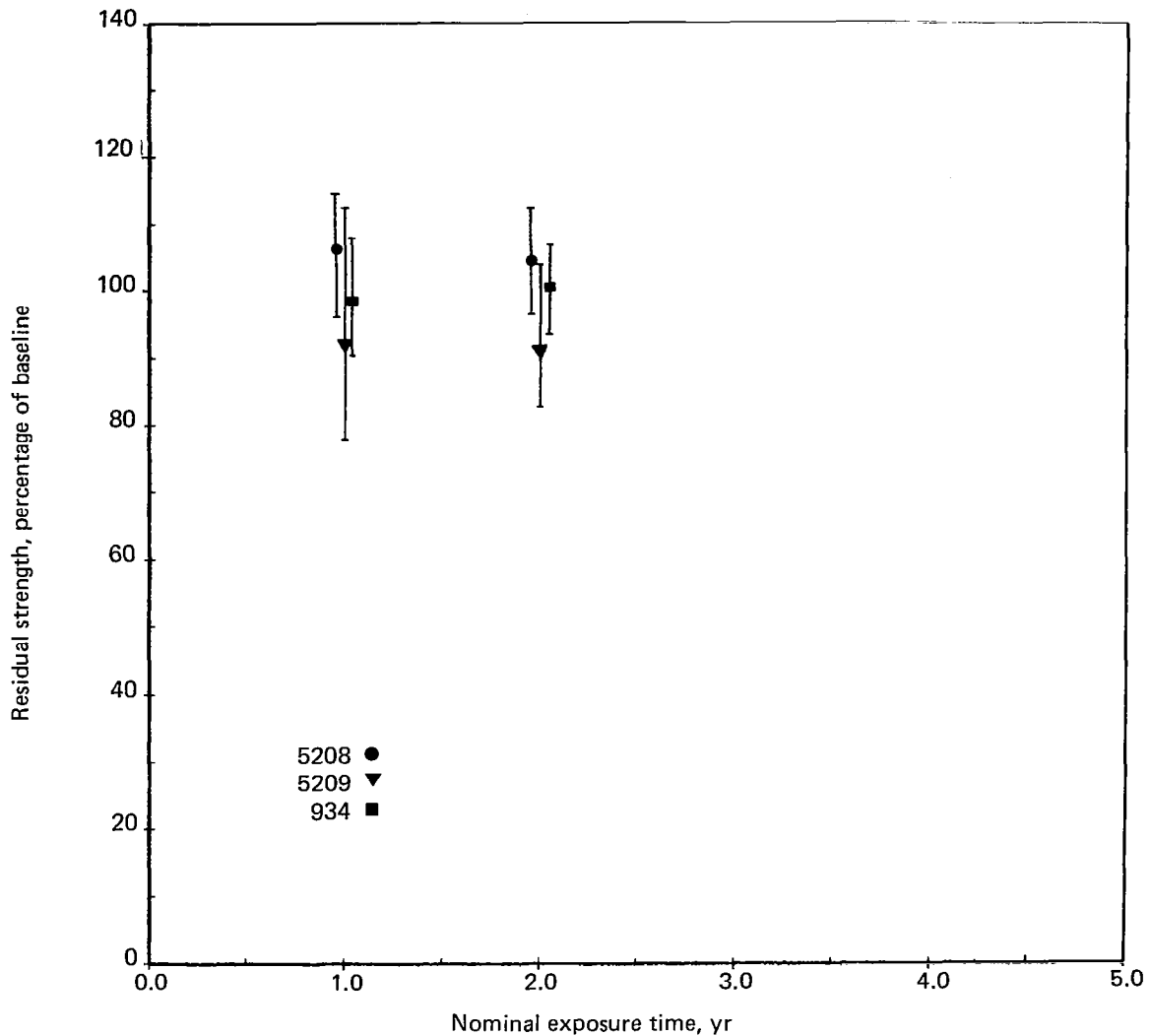
Figure 39. Flexure-82°C (180°F)
