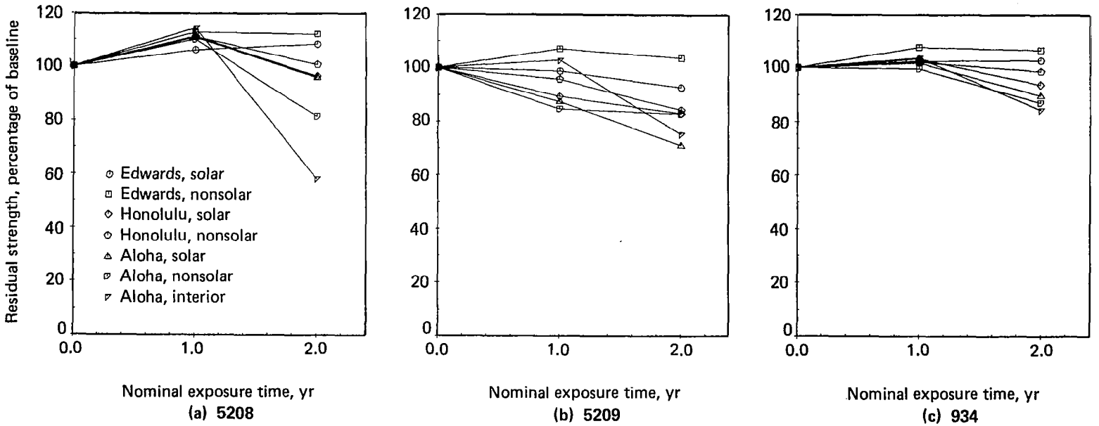
Figure 41. Individual Results, Flexure—82°C (180°F)
