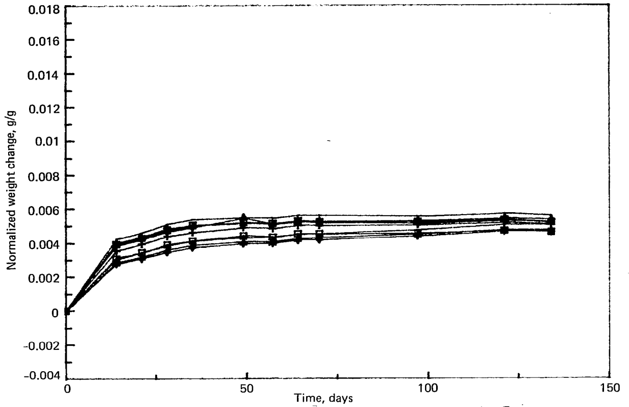
Figure 53. Normalized Weight Change for 60% Relative Humidity Exposure
