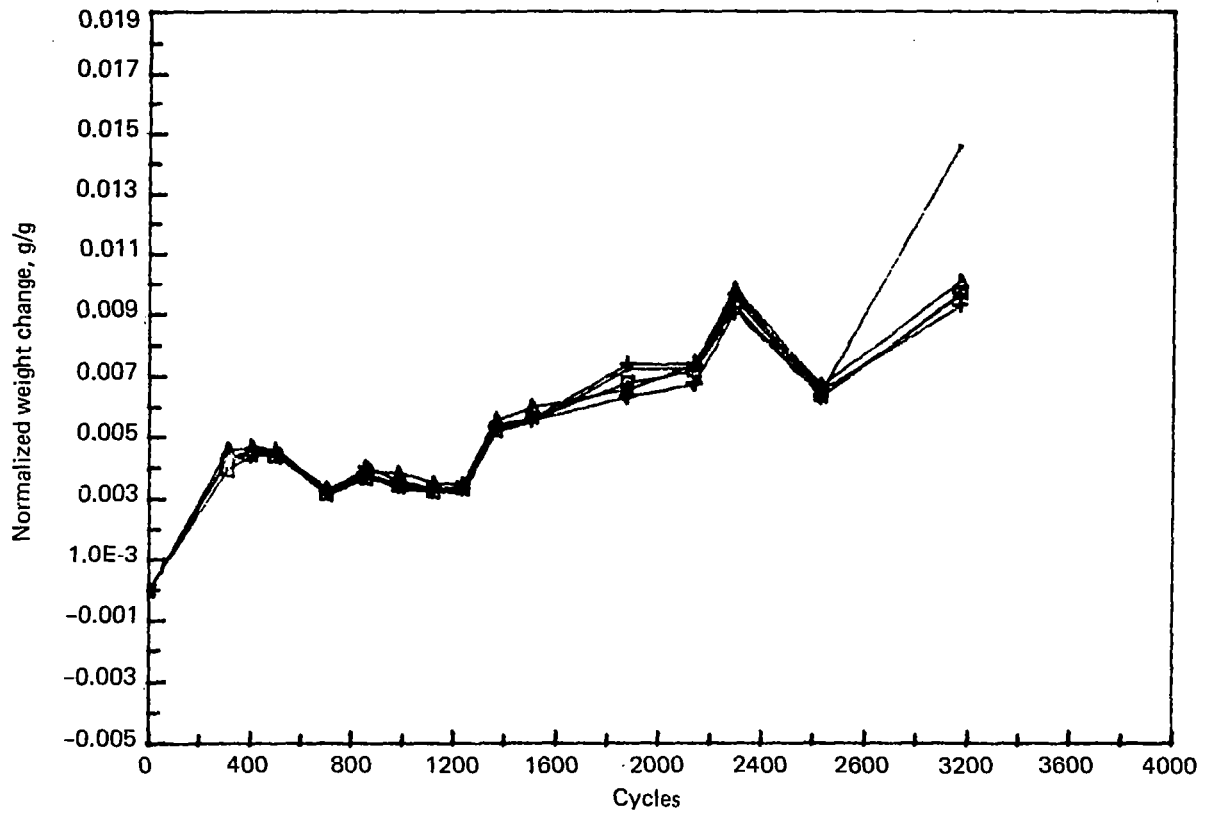
Figure 60. Weight Change of Unpainted 5208 as a Function of Ground-Air-Ground Cycles
