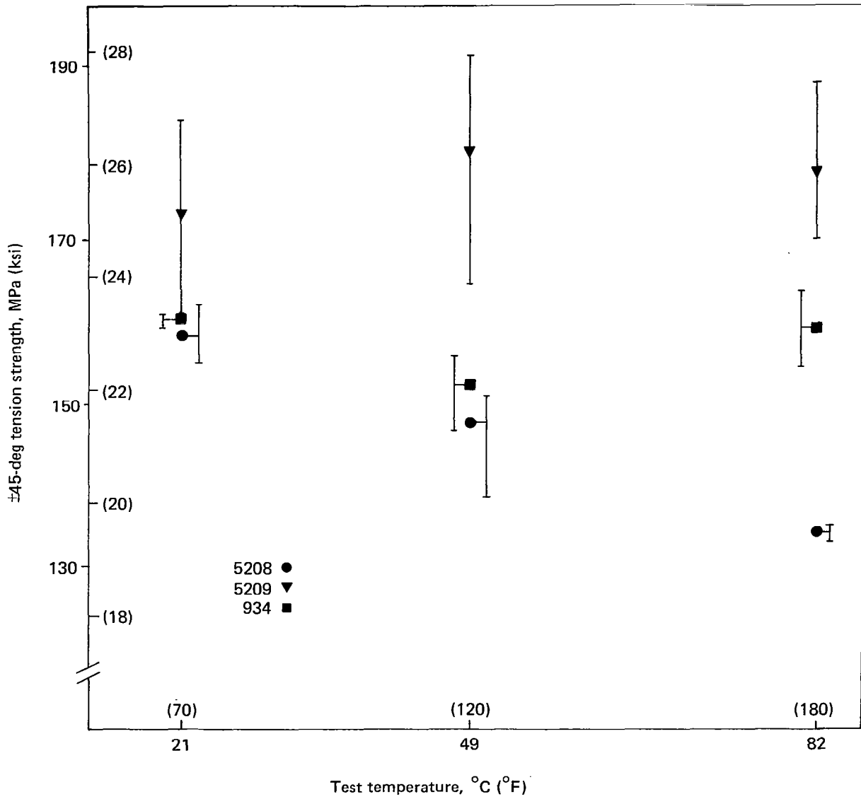
Figure 48. Baseline ±45-deg Tension Strength Results
