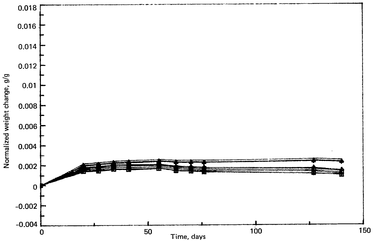
Figure 54. Normalized Weight Change for 40% Relative Humidity Exposure
