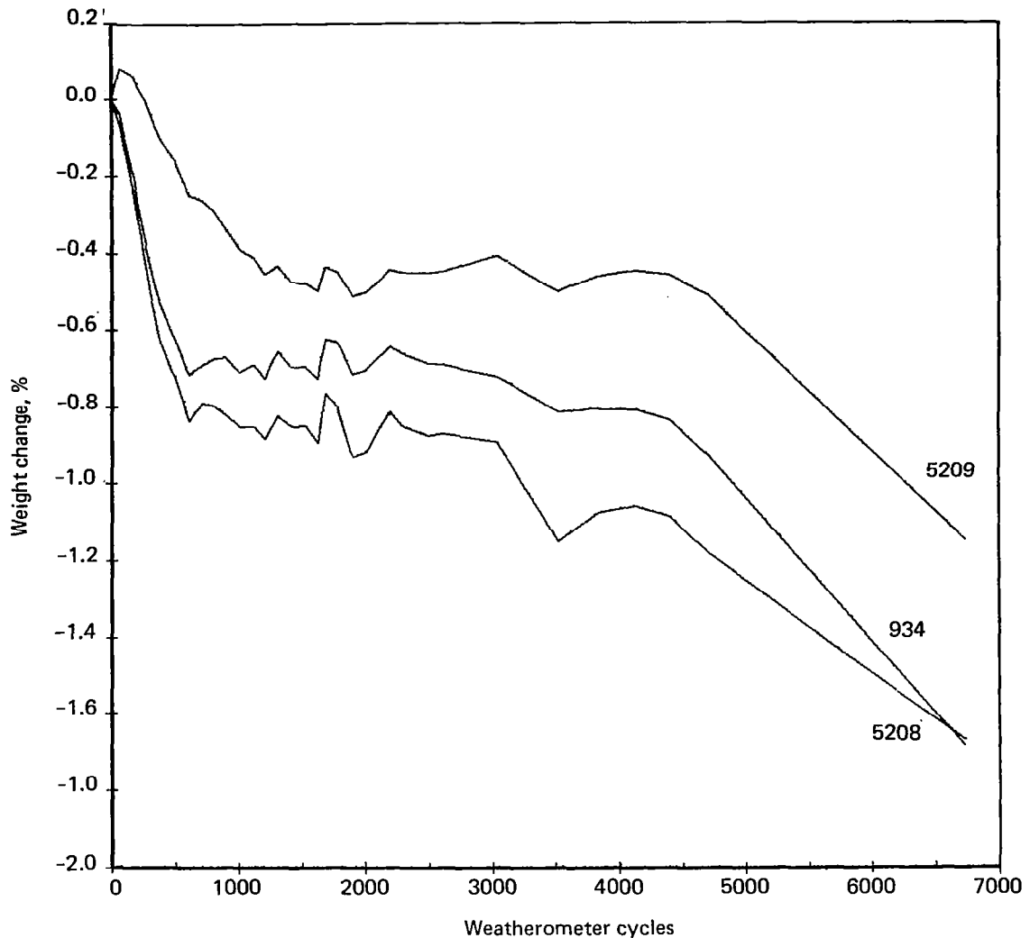
Figure 56. Weights of Unpainted Weatherometer Specimens
