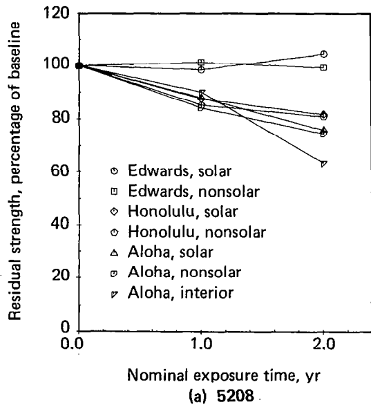
Figure 36. Individual Results, Short Beam Shear—Room Temperature
