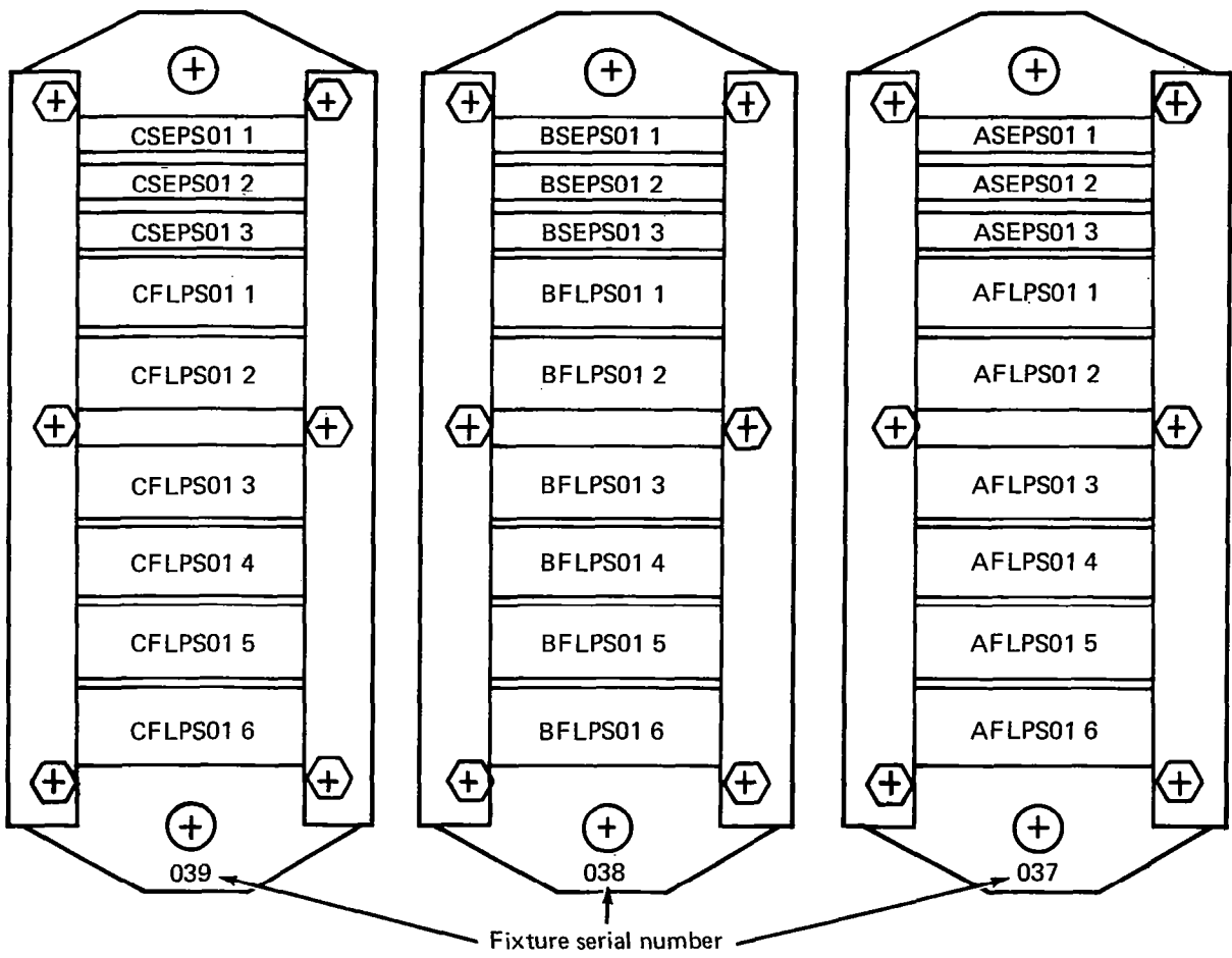
Figure 27. Sample Load Map
