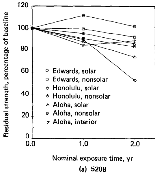
Figure 36. Individual Results, Short Beam Shear—Room Temperature
