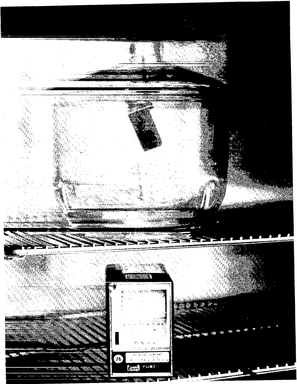
Figure 29. Rustrak Checkout of Humidity Environment
