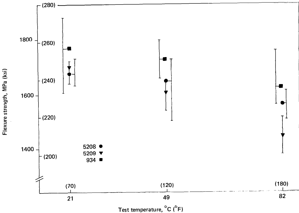
Figure 47. Baseline Flexure Strength Results
