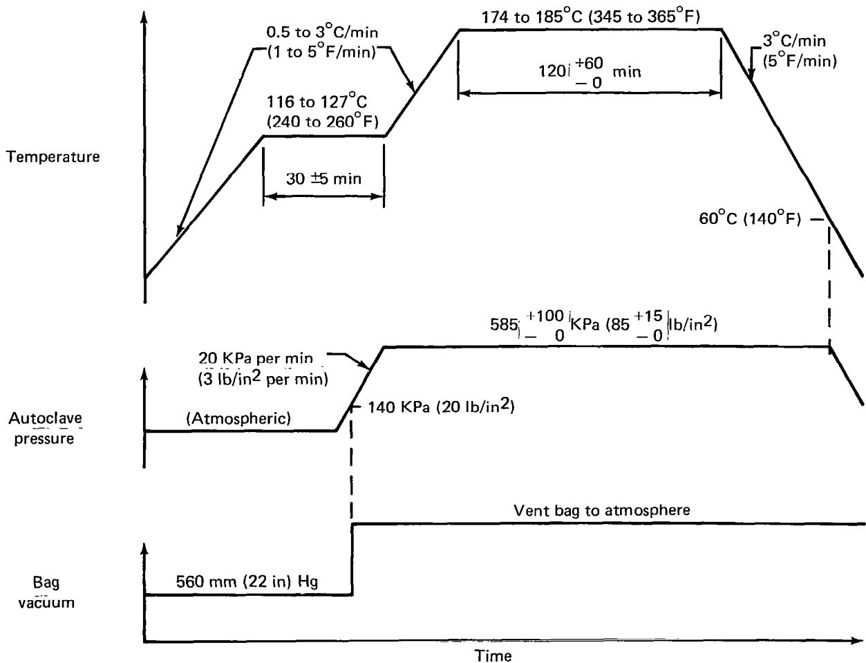
Figure 3. Cure Cycle for 177°C (350°F) Graphite-Epoxy Laminates
