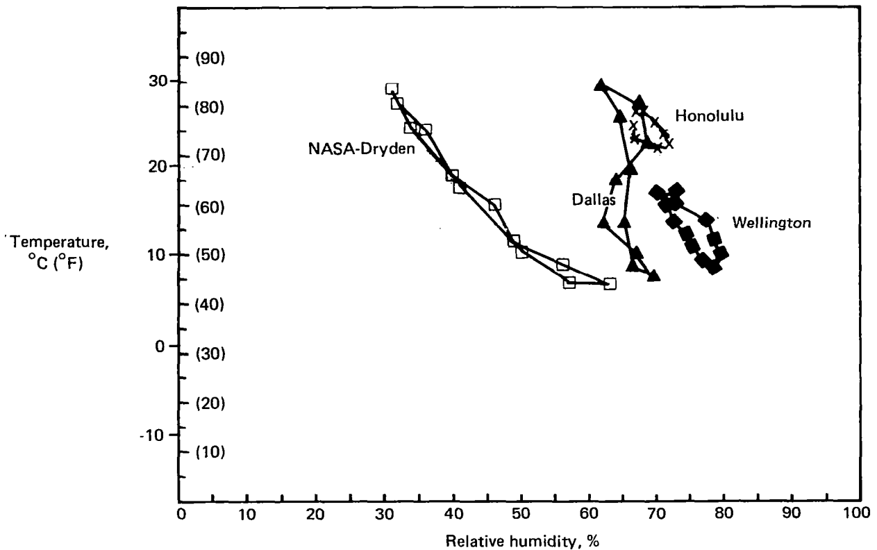
Figure 11. Ground Rack Climatic Data
