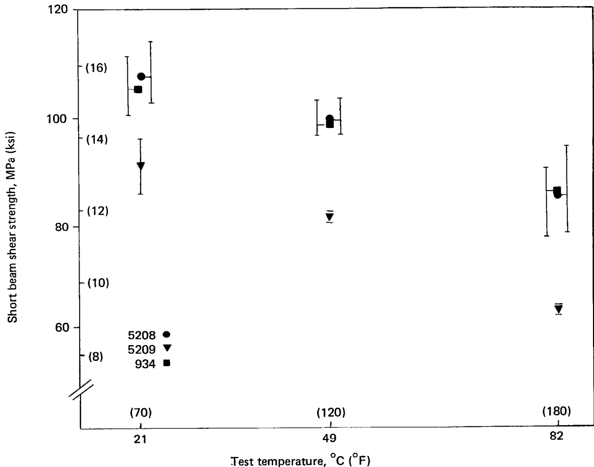
Figure 46. Baseline Short Beam Shear Strength Results
