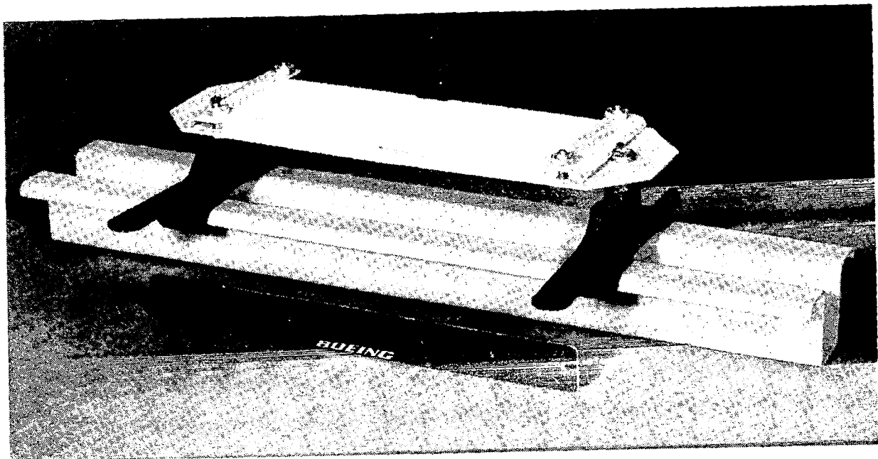
Figure 20. Interior Aircraft Compression Specimen Fixture
