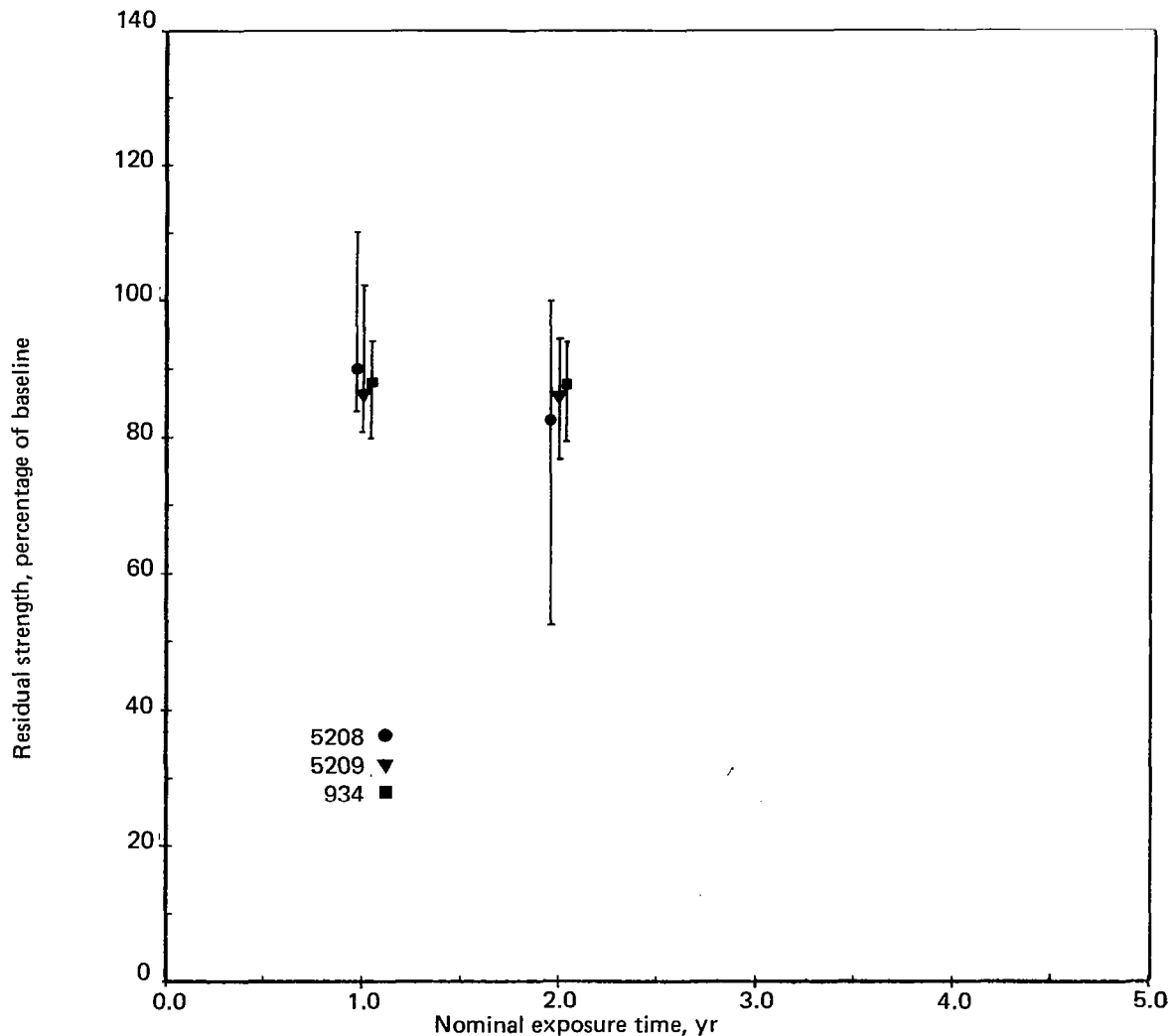
Figure 34. Short Beam Shear—Room Temperature
