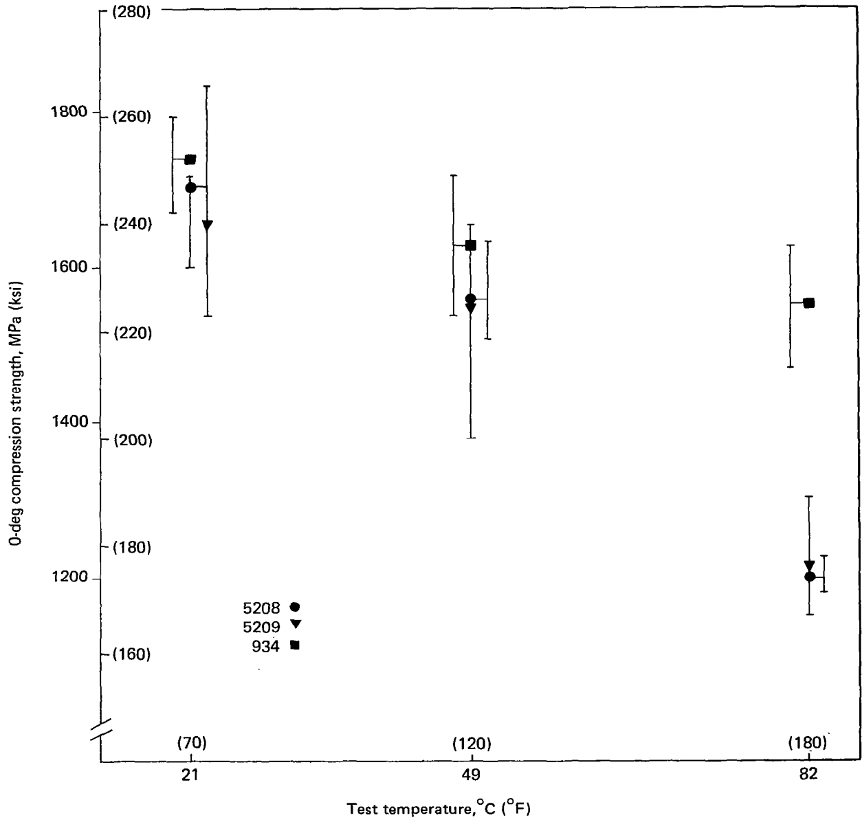
Figure 49. Baseline 0-deg Compression Strength Results
