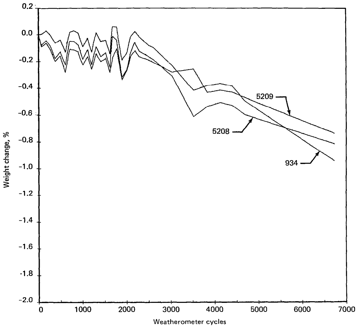
Figure 58. Weights of Painted Weatherometer Specimens
