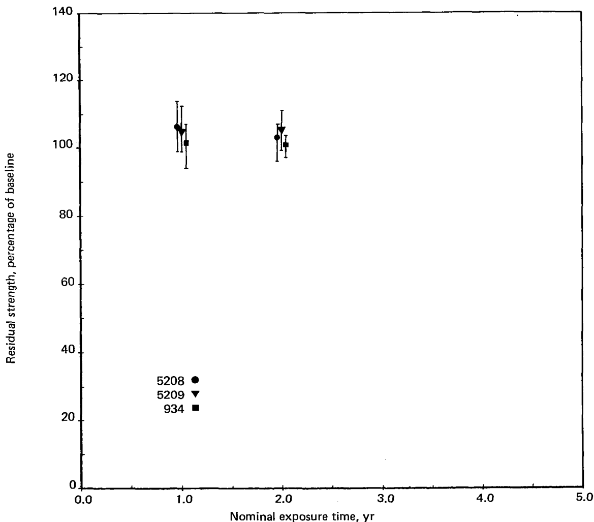
Figure 38. Flexure—Room Temperature
