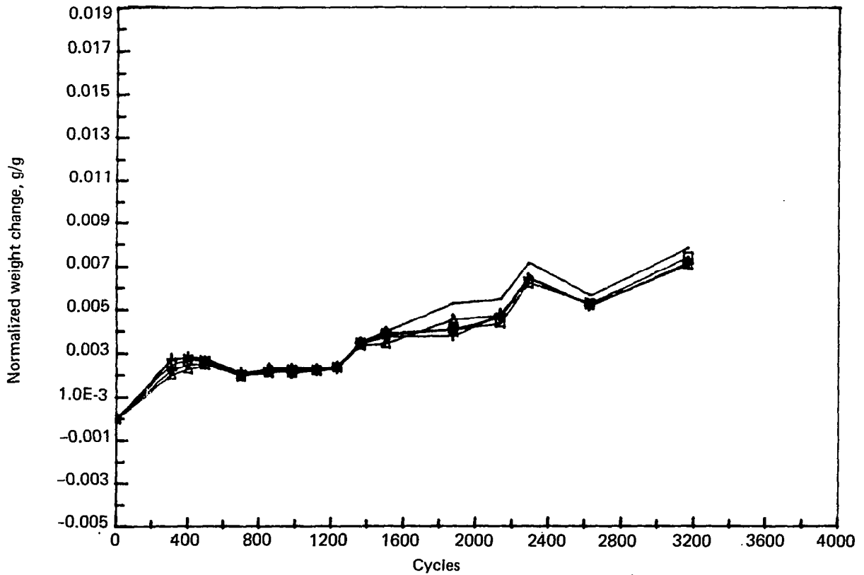
Figure 61. Weight Change of Unpainted 5209 as a Function of Ground-Air-Ground Cycles
