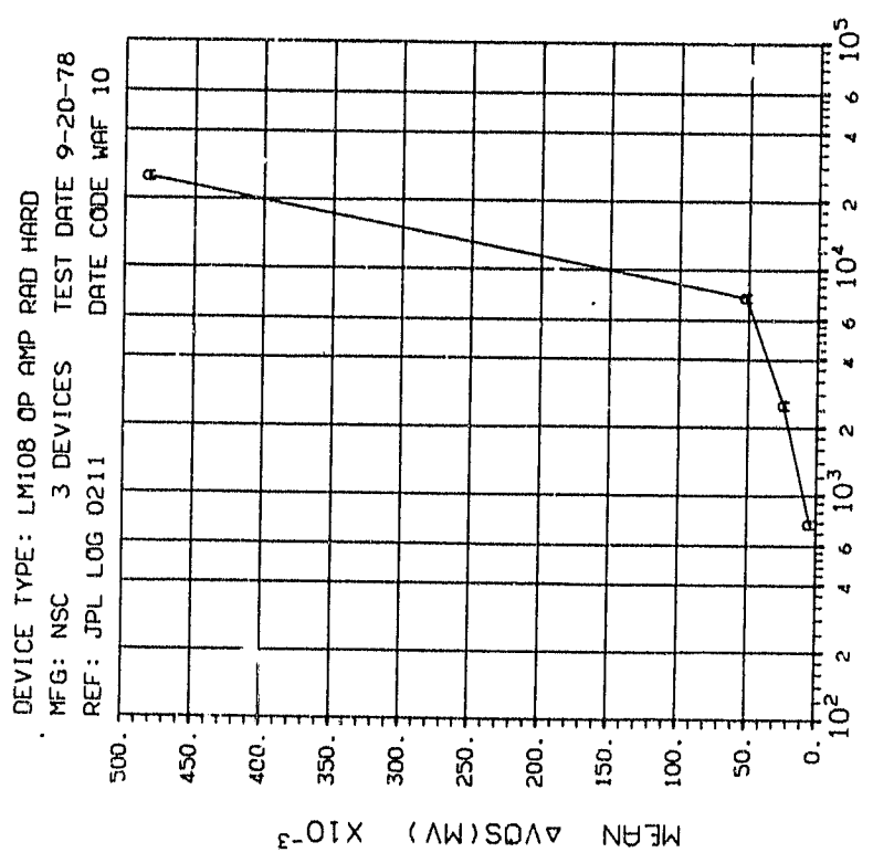
DOSE, Gy(Si) Co 60 Gammas (1) VDS ON MV VS DOSE
