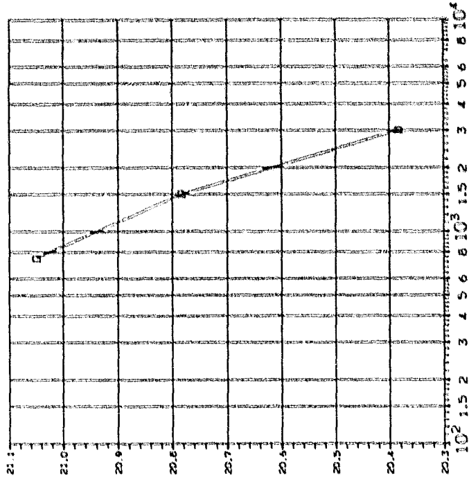
DOSE, Gy(Si) 2.5 MeV electrons (14) I SINK IN MA VS DOSE
