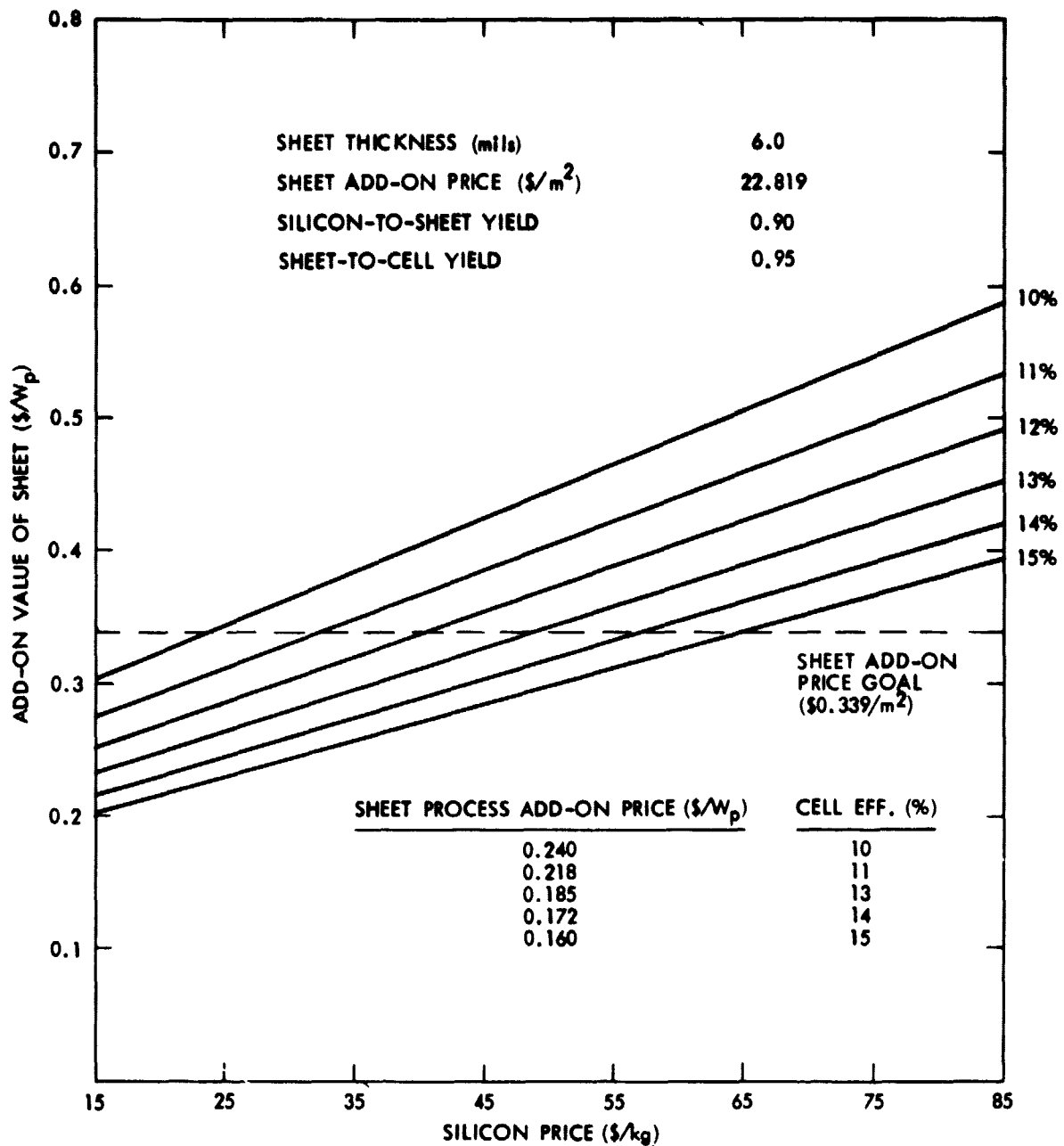
Figure 7c. Add-on Price vs Silicon Price for Sheet Using Web Process for Sheet Thickness of 6 mils
