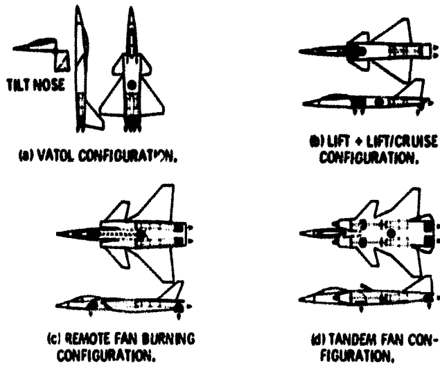
Figure 1. - Supersonic V/STOL airplane types.
