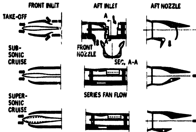
Figure 7. - Inlets and nozzles for tandem fan propulsion systems.
