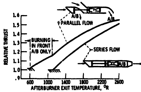
Figure 5. - Effect of afterburner temperature for parallel and series operating modes (FPR) DES = 1.4.
