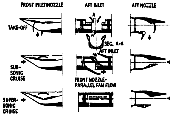
Figure 8. - Inlets and nozzles for reverse flow fan propulsion system.
