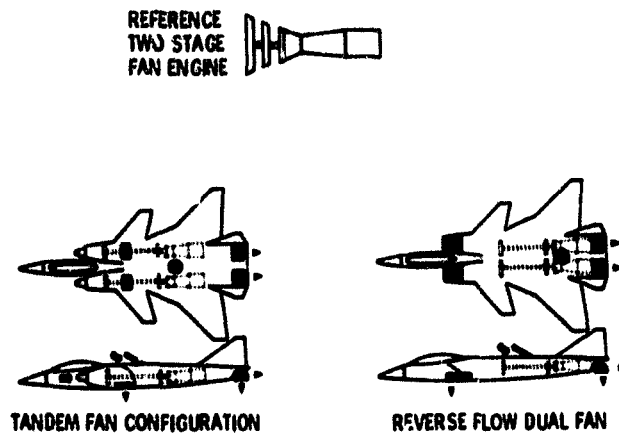
Figure 2. - Airplane variations.
