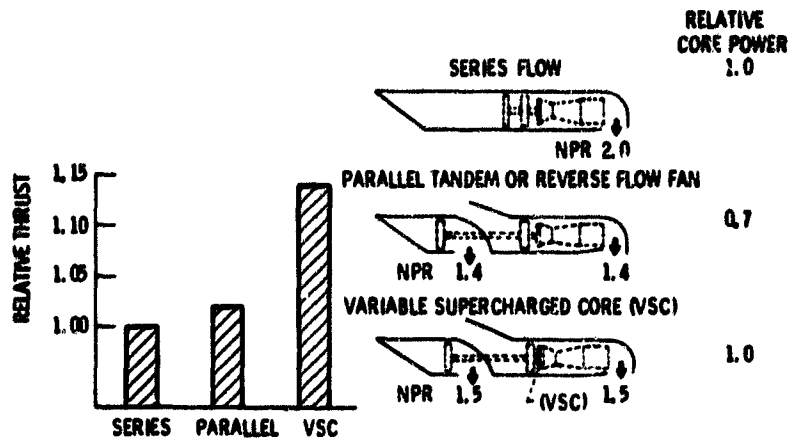
Figure 4. - Takeoff engine performance.
