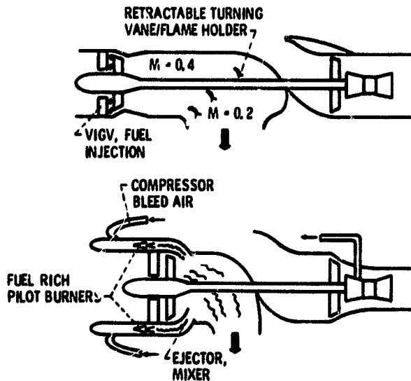
Figure 11. - Fan air burners.
