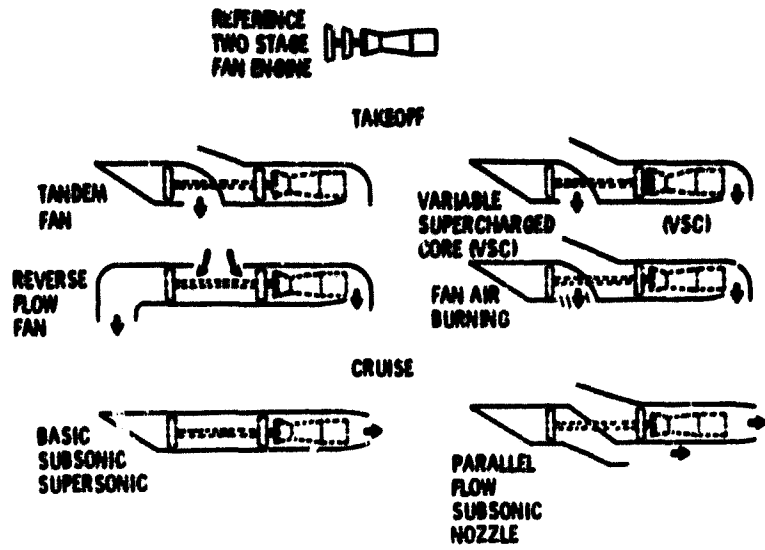
Figure 3. - Engine cycle variations.
