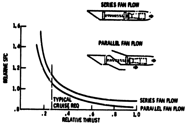
Figure 6. - Subsonic cruise specific fuel consumption M_0 = 0.8 WPR_{DES} = 1.4
