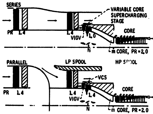
Figure 10. - Variable core supercharger.
