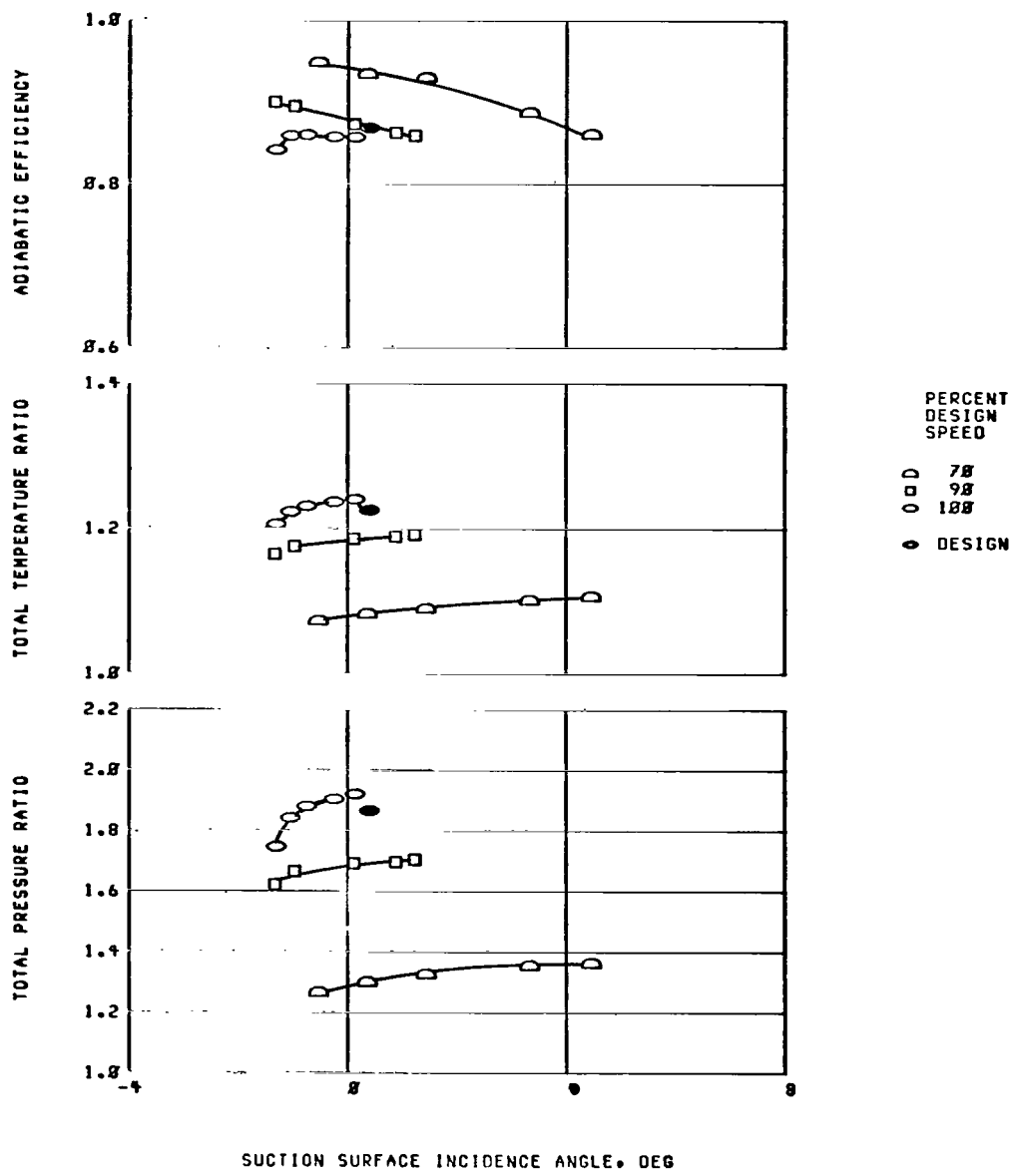
Figure 11. - Continued. Blade-element performance for rotor 36.
