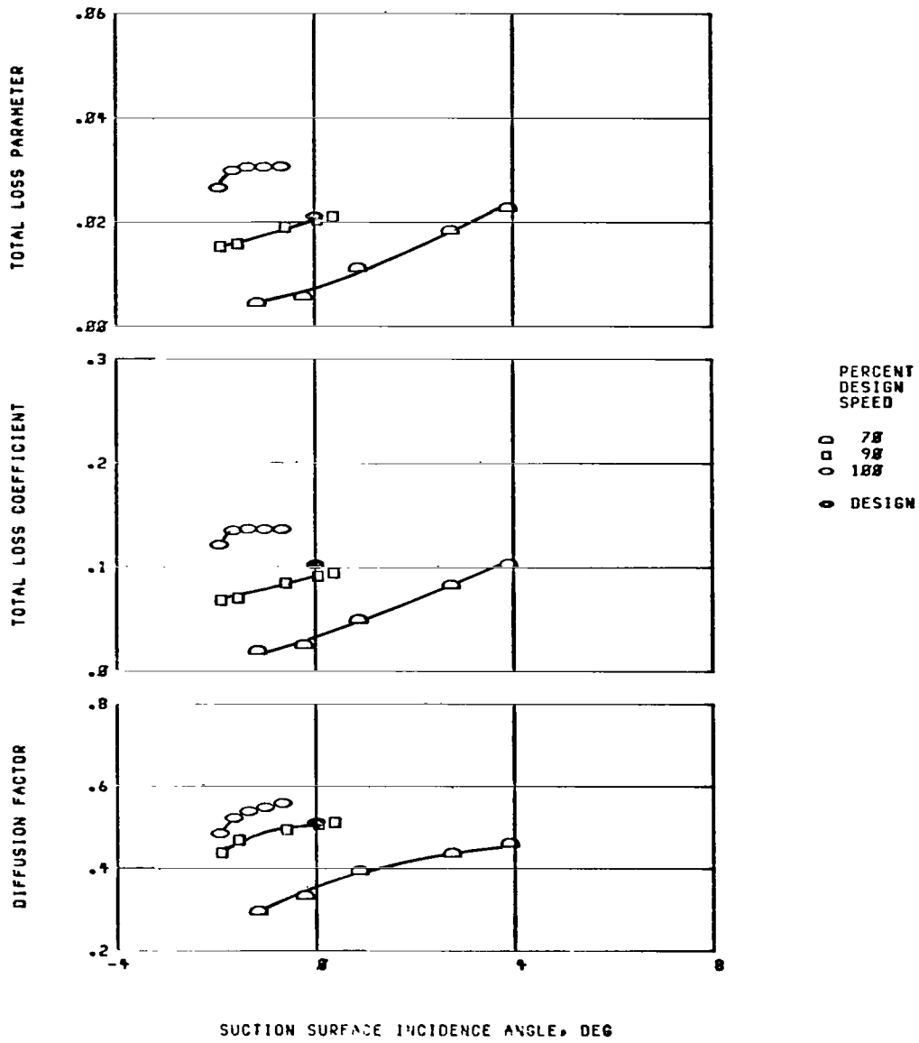
(f) Continued. Location, 70 percent of span. Figure 11. - Continued. Blade-element performance for rotor 36.
