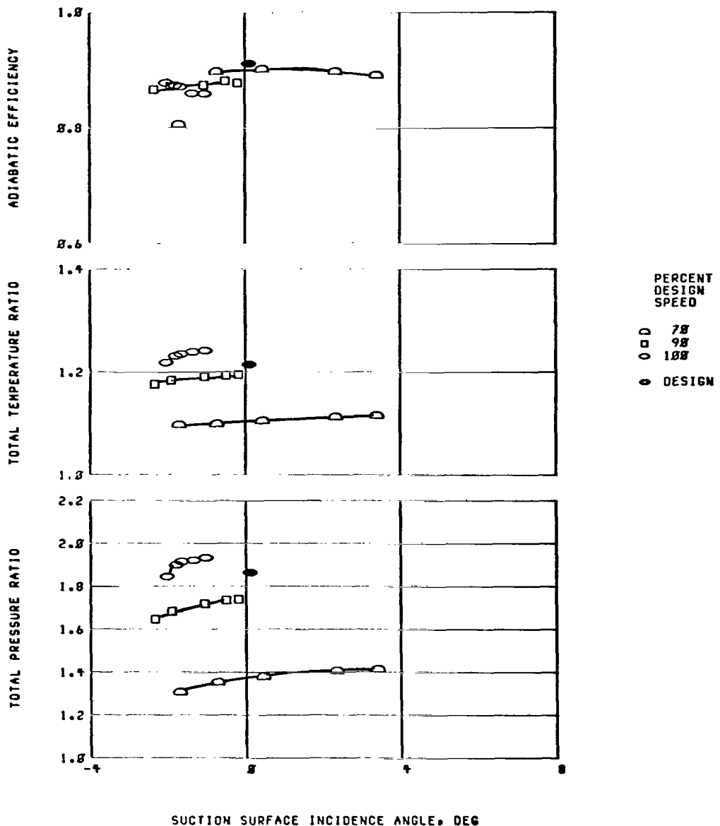
(i) Concluded. Location, 95 percent of span. Figure 11. - Concluded. Blade-element performance for rotor 36.
