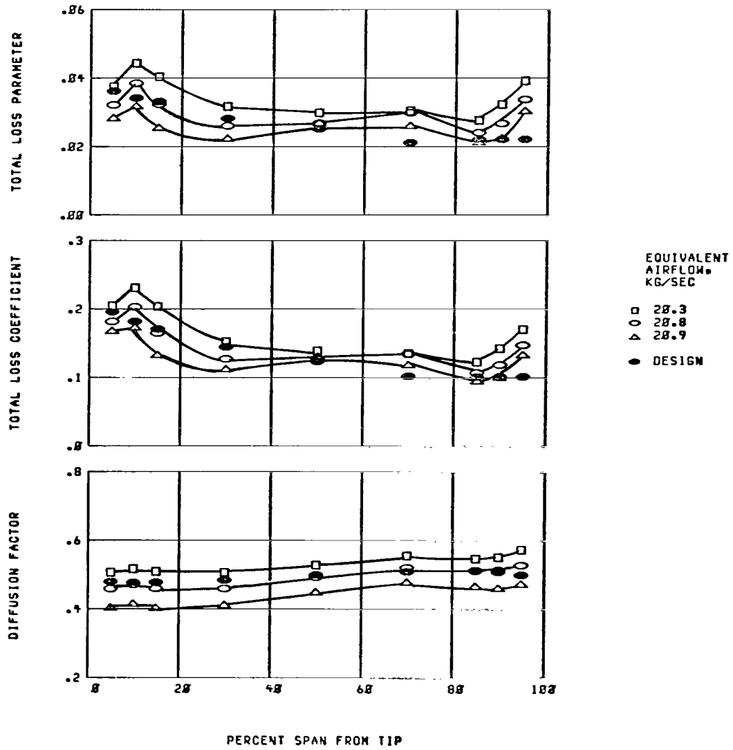
Figure 8. - Continued. Radial distribution of performance for rotor 36. 100 Percent of design speed.
