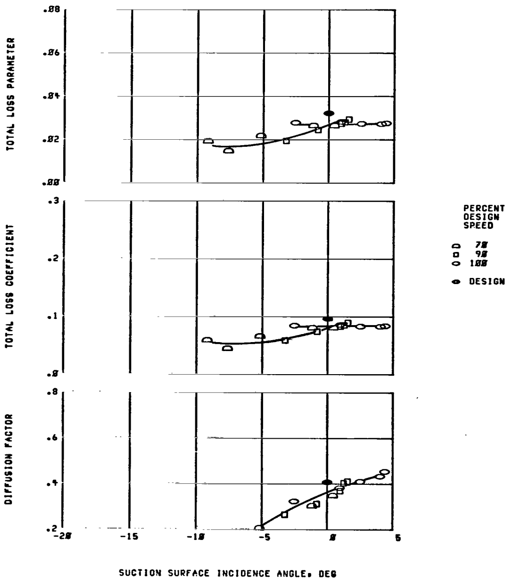
(i) Concluded. Location, 95 percent of span. Figure 12. - Concluded. Blade-element performance for stator 36.
