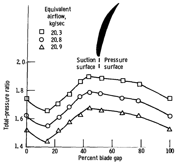
Figure 10. - Circumferential distribution of total-pressure ratio at station 3. 100 Percent of design speed; location, 5 percent of span.
