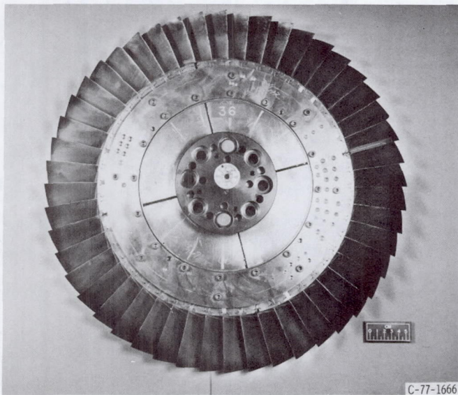
(a) Rotor.
