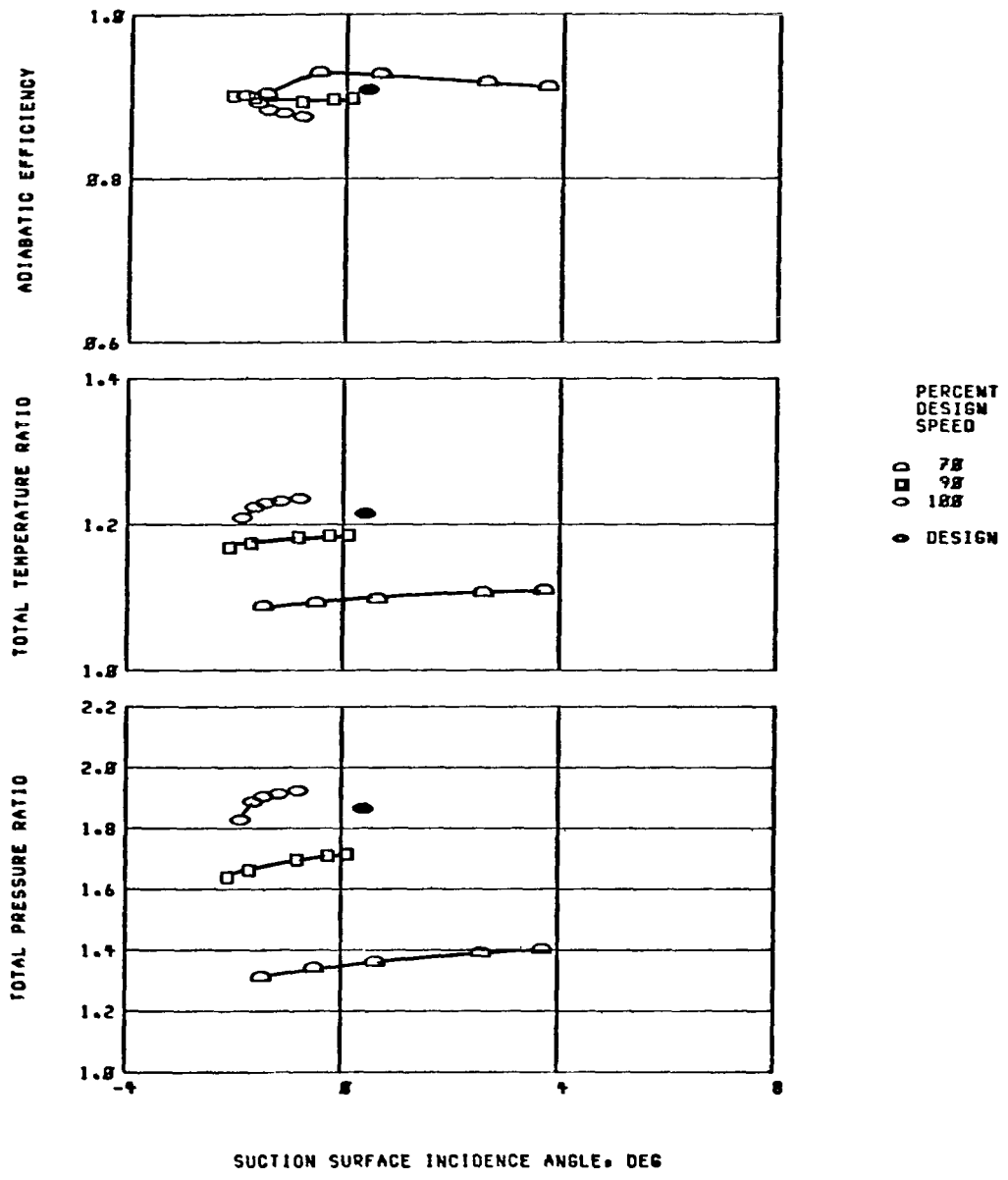
(h) Concluded. Location, 90 percent of span. Figure 11. - Continued. Blade-element performance for rotor 36.
