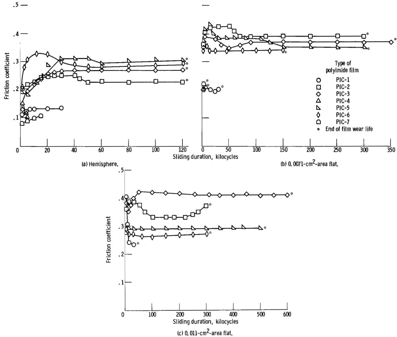
Figure 4. - Average friction coefficient as a function of sliding duration for a hemisphere, a 0.0071-cm 2 -area flat, and a 0.011-cm 2 -area flat sliding on films applied to 440C HT stainless steel substrates. Experimental conditions: ambient temperature, 25 o C; sliding speed, 1000 rpm (2.6 m/sec); load, 1 kg (9.8 N); moist air atmosphere (50 percent relative humidity).
