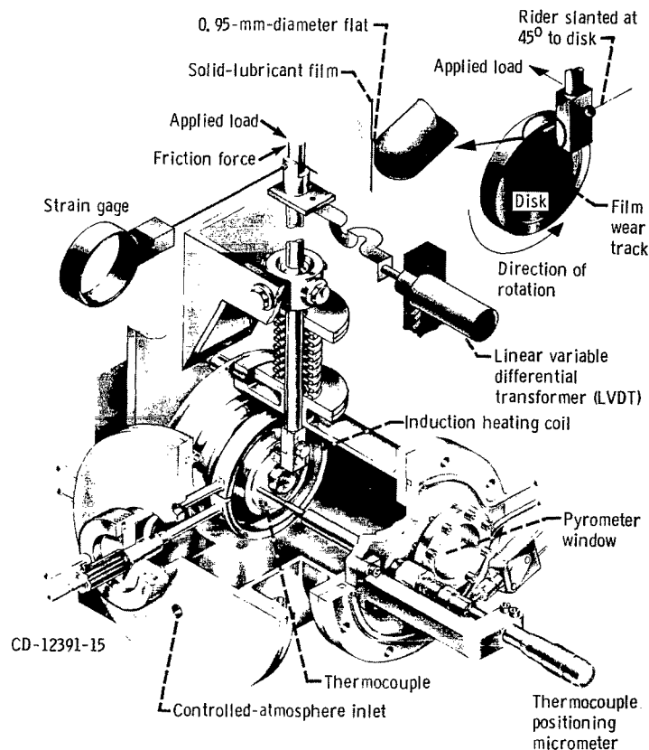
Figure 2. - Friction and wear apparatus.
