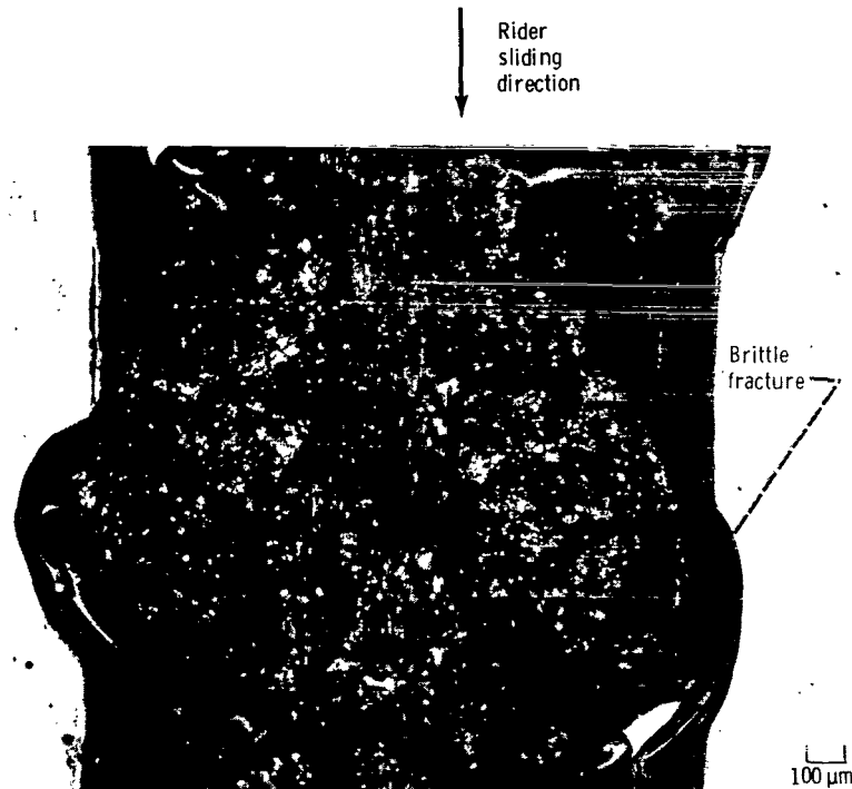
Figure 9. - Photomicrograph of PIC-7 film wear track after 15 kilocycles of a sliding hemisphere on the film. (This photomicrograph also typifies what happened when the flat areas slid against the film and also what happened to the PIC-4 films for all three contact areas.)
