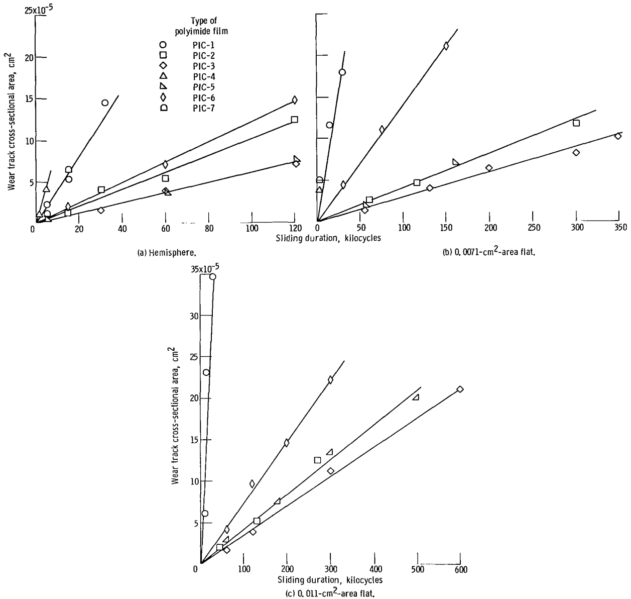
Figure 5. - Wear of seven polyimide films as a function of sliding duration for a hemisphere, a 0.0071- \text{cm}^2 -area flat, and a 0.011- \text{cm}^2 -area flat sliding on films applied to 440C HT stainless steel substrates. Experimental conditions: ambient temperature, 25 ^{\circ} C; sliding speed, 1000 rpm (2.6 m/sec); load, 1 kg (9.8 N); moist air atmosphere (50 percent relative humidity).
