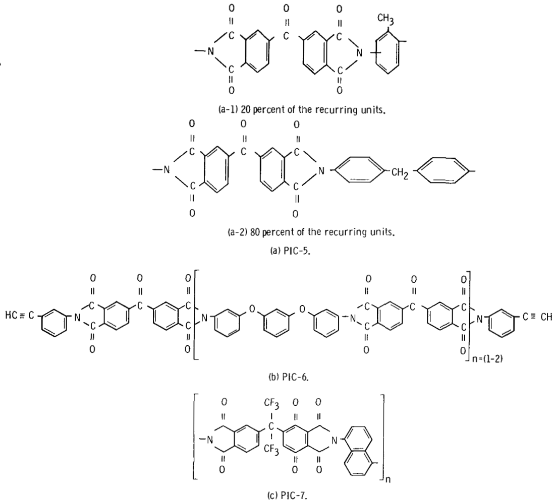
Figure 1. - Structure of polyimide types PIC-5, PIC-6, and PIC-7.
