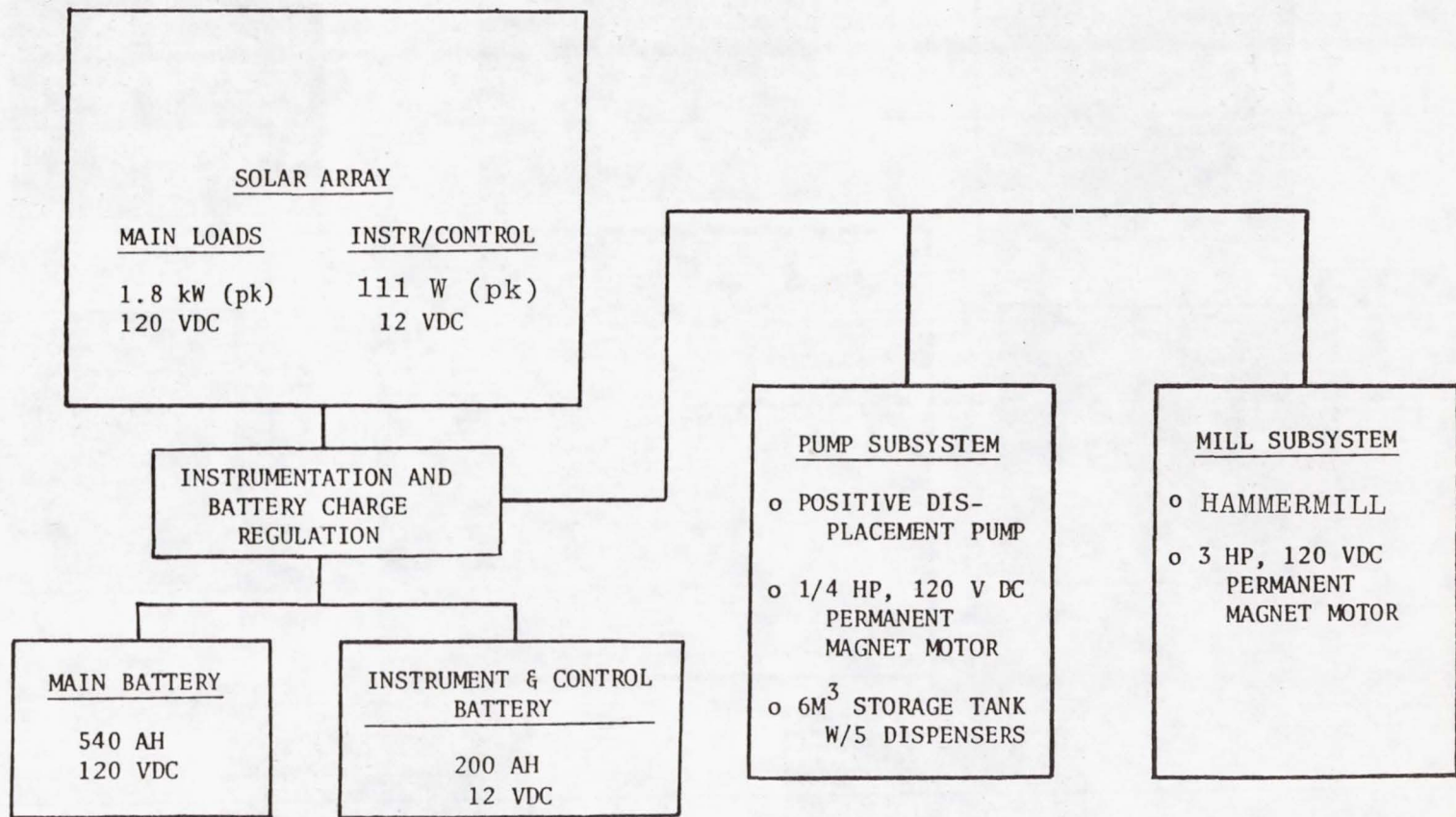
FIGURE 1 - SYSTEM DIAGRAM: PHOTOVOLTAIC-POWERED PUMPING/MILLING SYSTEM, TANGAYE, UPPER VOLTA
