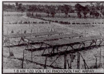
TANGAYE VILLAGE SOLAR ELECTRIC SYSTEM
