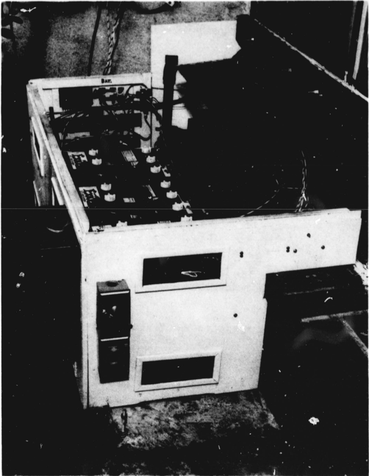
Figure 26. Batteries, Inverter, and Breaker Switch Box
