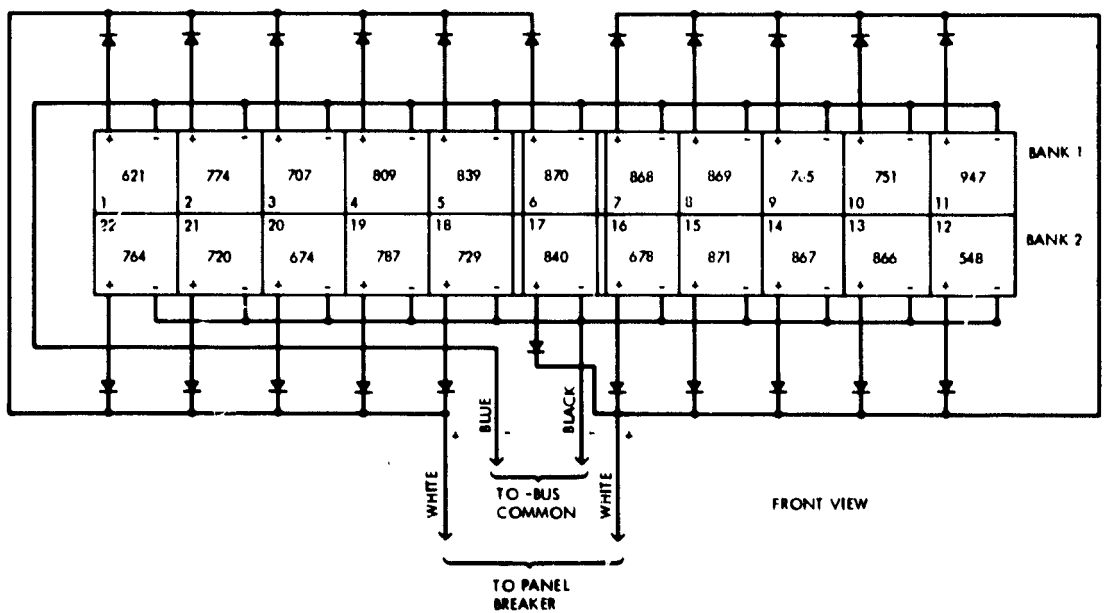
Figure 6. Schematic Diagram of a PV Array Configuration
