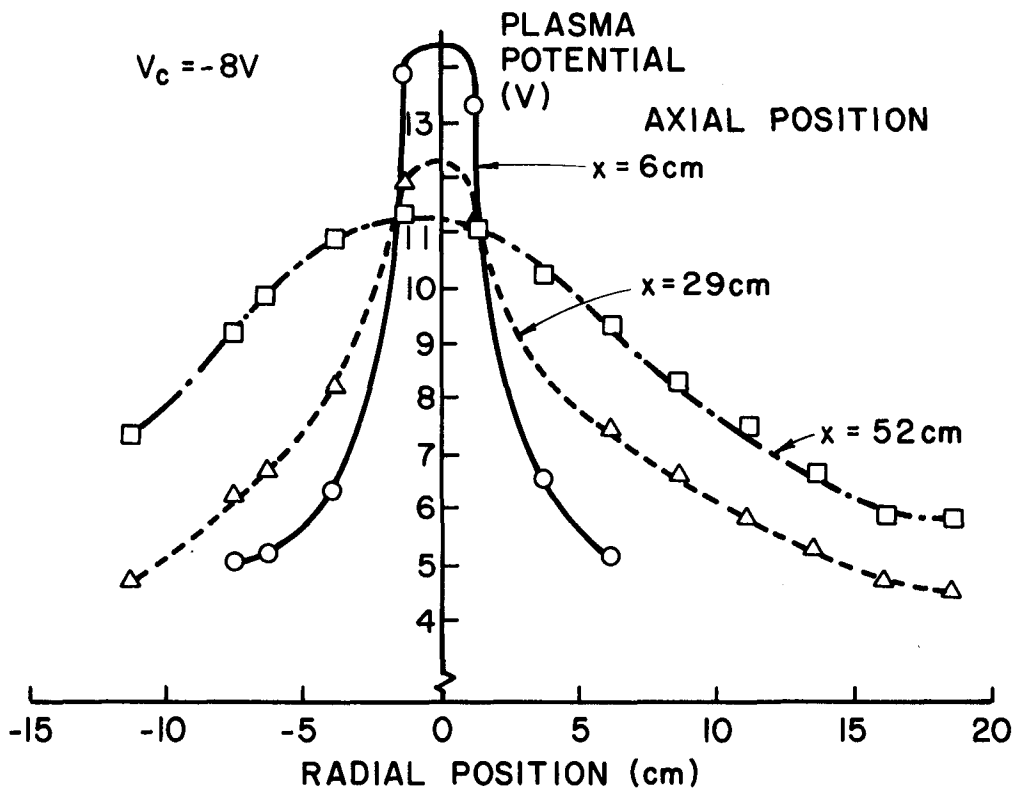
a. NEUTRALIZER ON FIELD LINE MISSING BEAM \mathcal{Q} BY \sim 30 cm
