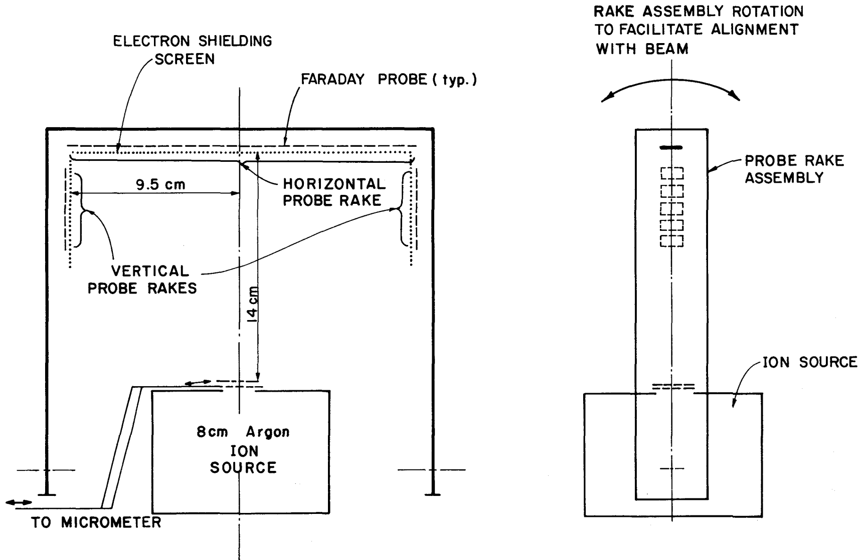
Figure 15. Deflecting Beamlet Test Apparatus.
