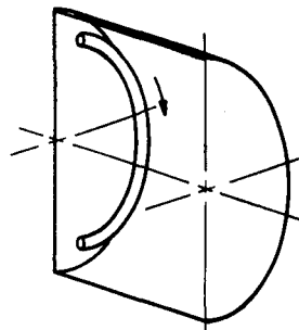
b. SINGLE UPSTREAM TORUS
