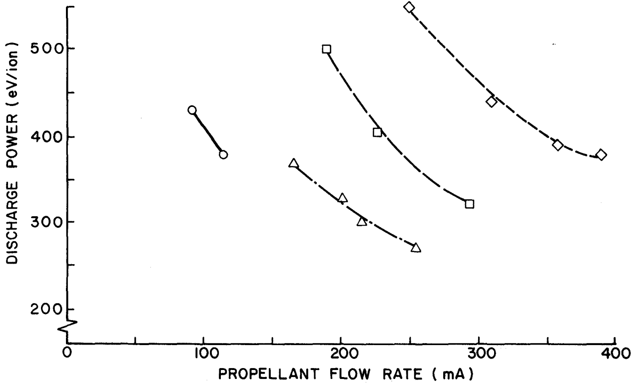
Figure 42. SIT 8 Performance at High Powers
