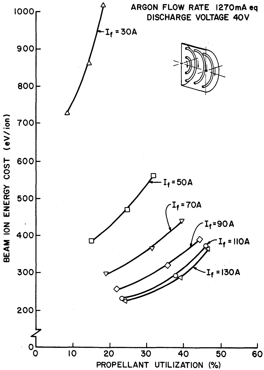
Figure 37. Effect of Field Current on Performance.
