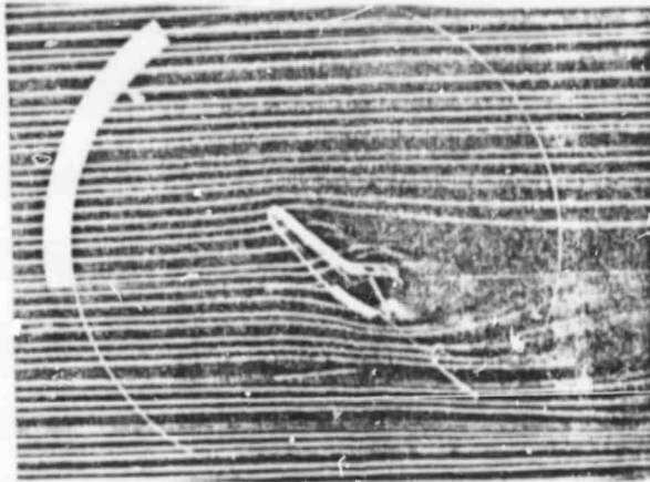
Model of BUMERANG in Smoke Wind Tunnel.
