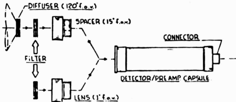
Figure 7. Optical/electronic module of multiband radiometer.
