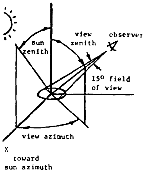
Figure 2. Coordinate system used for analysis.
