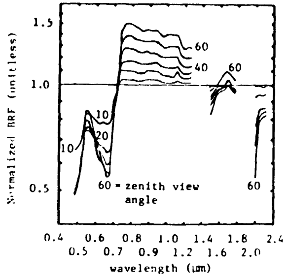
Figure 3. Normalized BRF for wheat 21 June 1976 three hours before noon with view azimuth 90^\circ to sun azimuth. Sun (zenith, azimuth) = (43^\circ, 109^\circ) .
