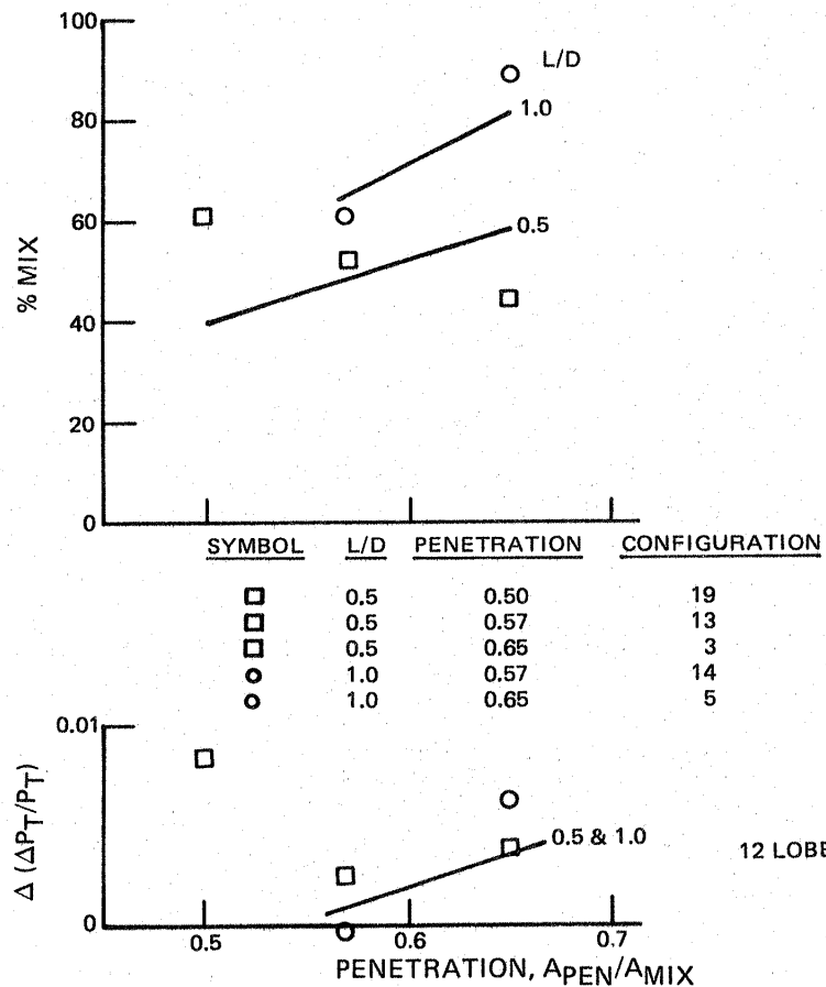
Figure 49 Percent Mixing and Excess Pressure Loss Variation with Penetration
