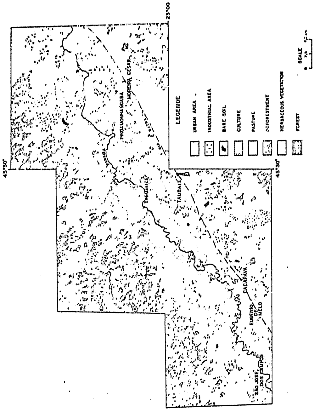
Fig. III.9 - Land-use map of test-site Taubaté (1977).
