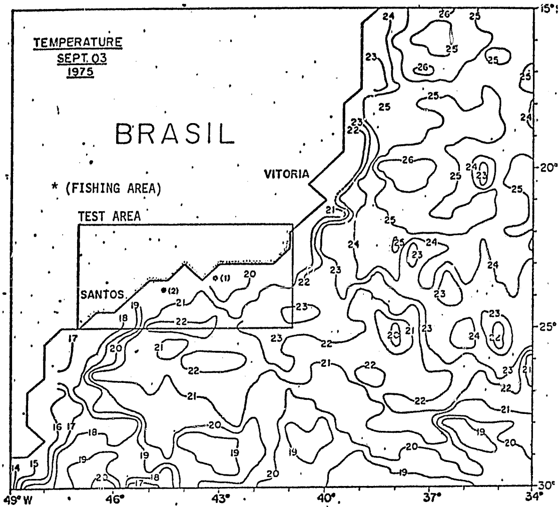
Fig. III.6 - Isotherms obtained through the GOSSTCOMP Project.
