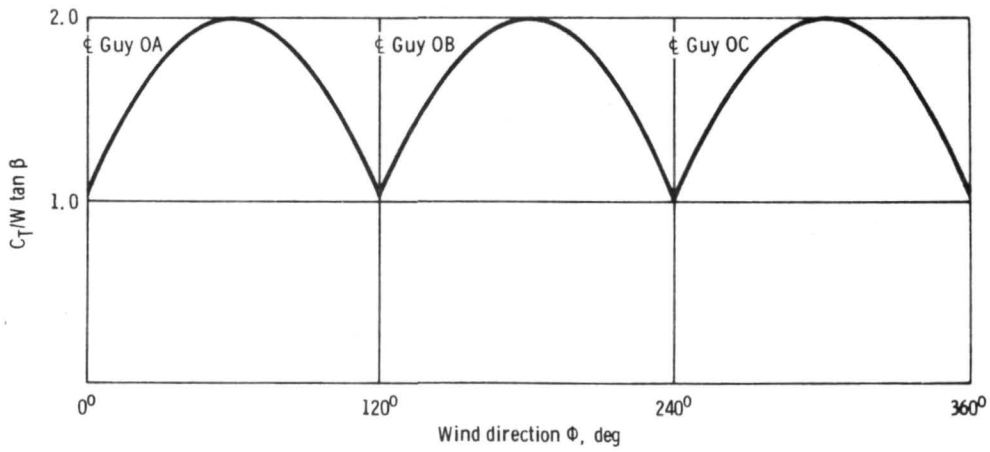
Figure A-5. - Compressive force in tower due to tension in guy rods.
