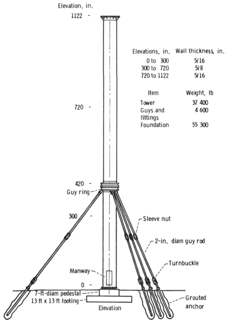
(a) Tower and foundation design - Configuration 1.
