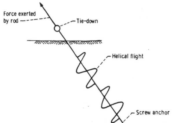
Figure 4. - Schematic of screw anchor.
