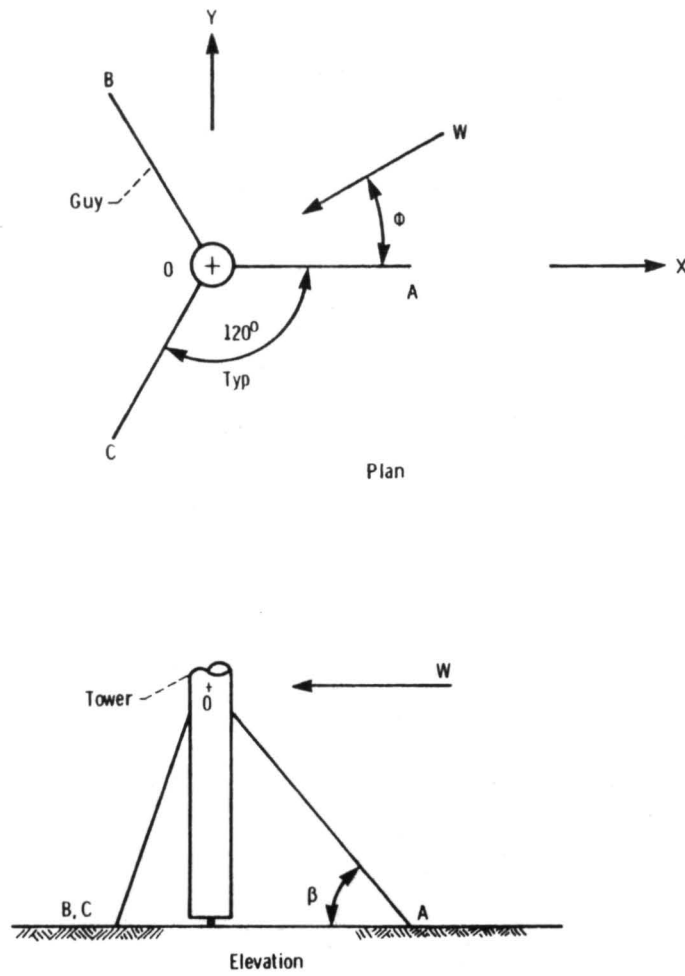
Figure A-1. - Coordinate system for guy rod force analysis.
