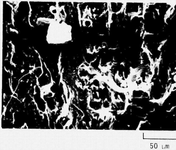
(a) 3.6 kPa H 2 O vapor. \Delta K = 23 \text{ MN/m}^{3/2} .
