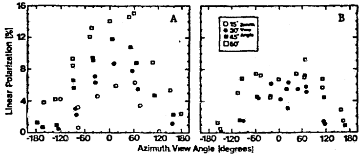
Fig. 3. Linear polarization (%) for view directions of wheat on 19 June 1976 (A) and 17 July 1976 (B). 0° azimuth is toward sun azimuth.
