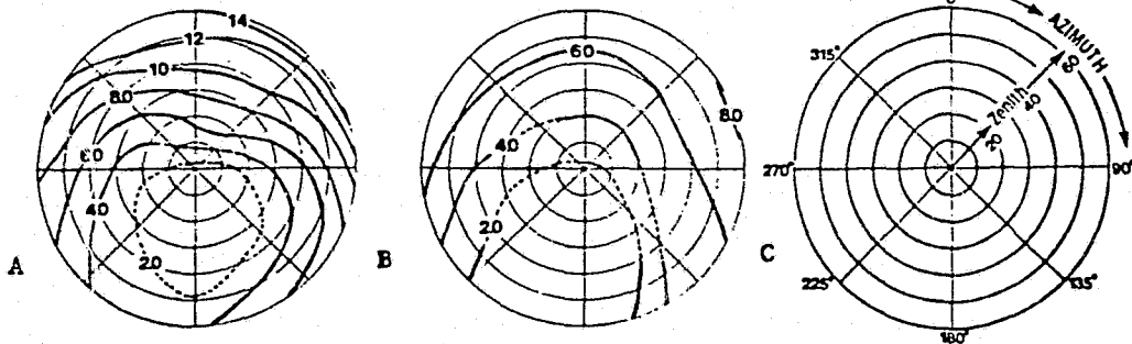
Fig. 4. Linear polarization (%) for view direction (C) of wheat on 19 June 1976 (A) and 17 July 1976 (B). 0° azimuth is toward sun azimuth.
