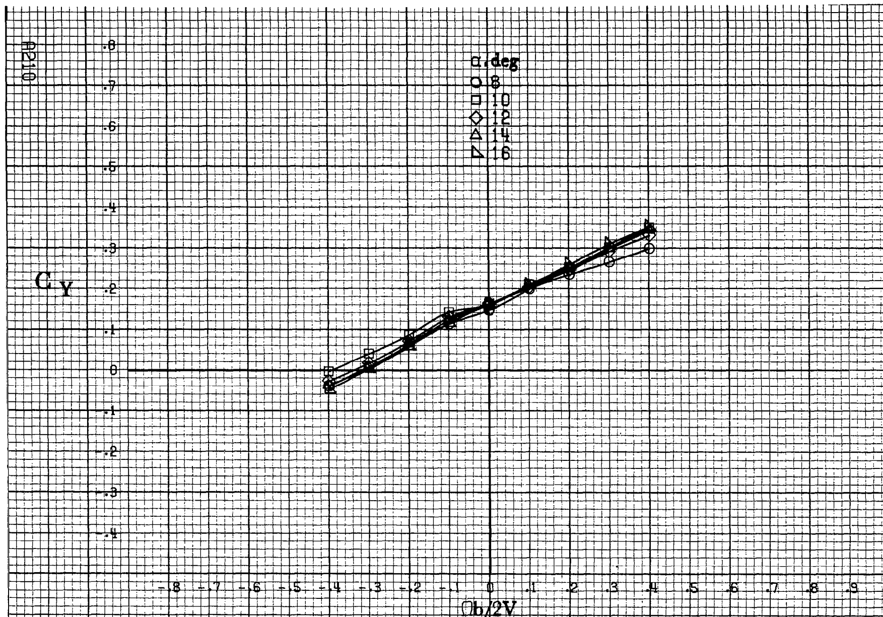
Figure A59 - Effect of rotation rate and angle of attack on side-force coefficient for basic configuration. \delta_e=0^\circ , \delta_a=0^\circ , \delta_d=16^\circ , \delta_r=0^\circ , \beta=0^\circ .
