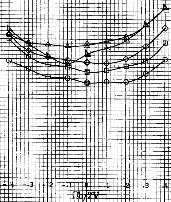
(c) \alpha = 30 to 50 deg, SR = 0 . Figure A 76.-Continued.
