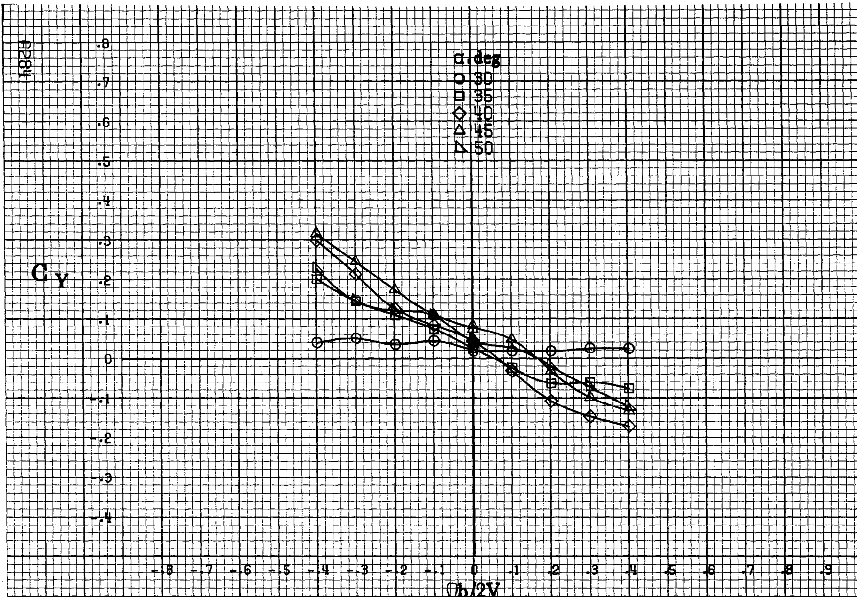
(c) \alpha=30 to 50 deg, SR=0 . Figure A77.-Continued.
