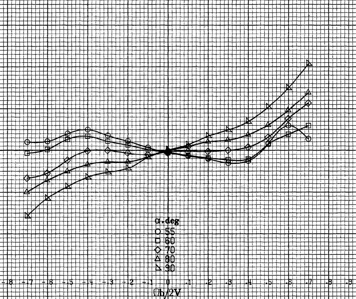
(d) \alpha = 55 to 90 deg, SR = 0 . Figure A14.-Concluded.
