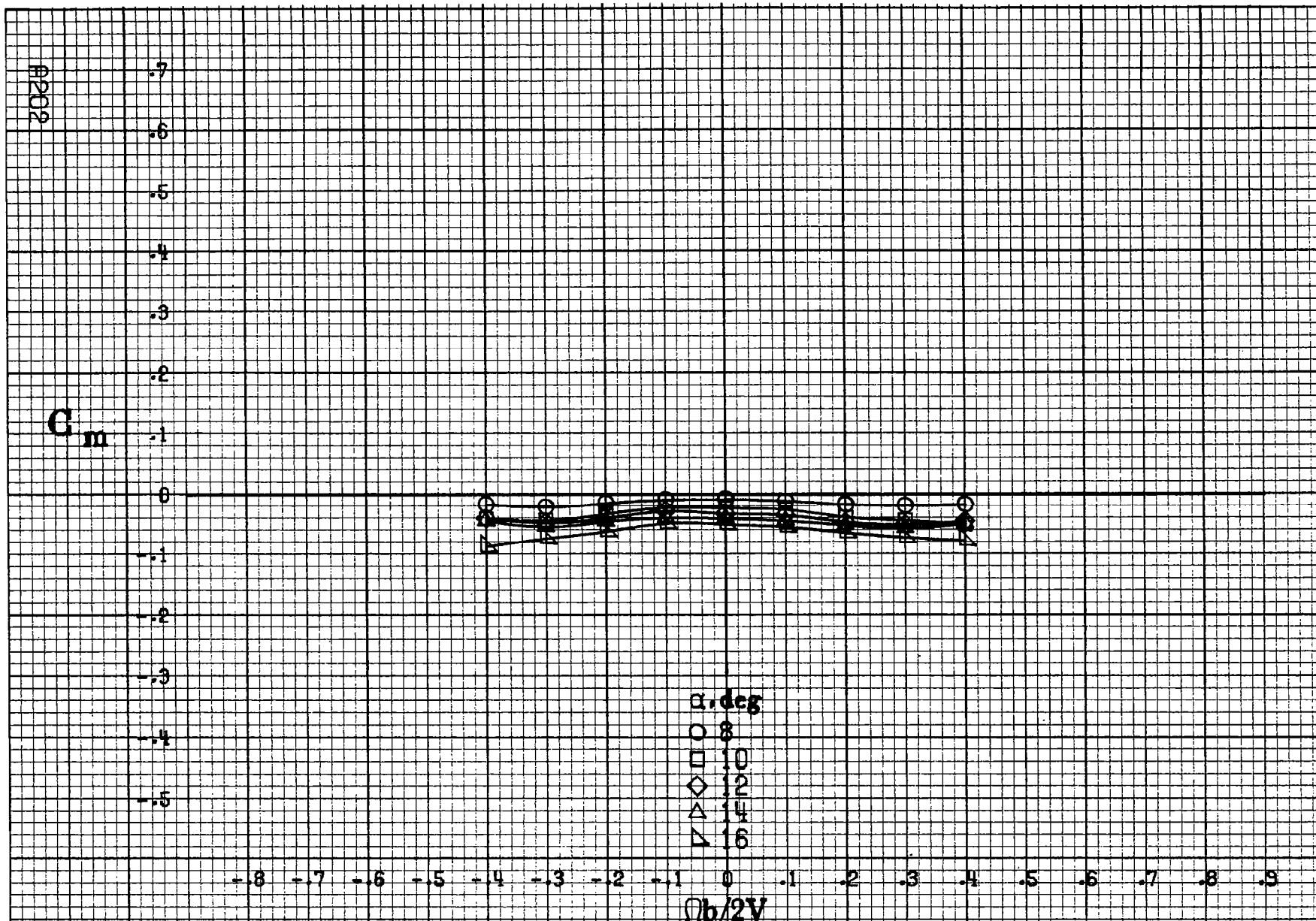
Figure A57.- Effect of rotation rate and angle of attack on pitching-moment coefficient for basic configuration. \delta_e = 0^\circ , \delta_a = 0^\circ , \delta_d = 6^\circ , \delta_r = 0^\circ , \beta = 0^\circ .
