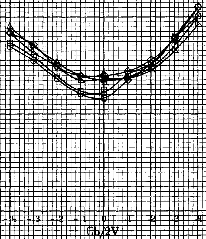
(b) \alpha=55 to 90 deg, SR=0 . Figure A88.- Concluded.
