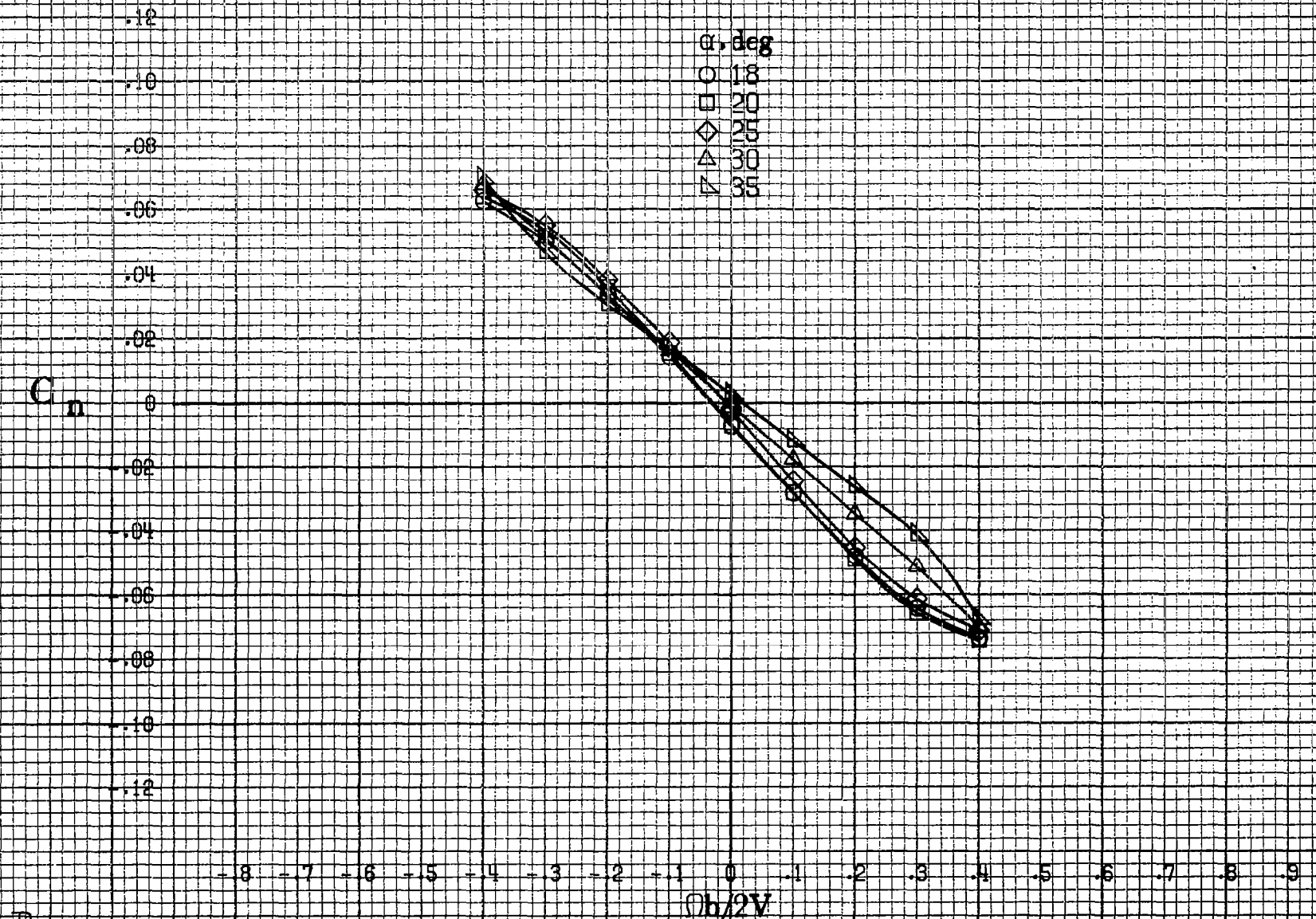
(b) \alpha = 18 to 35 deg. SR = 182.9 cm (72 in). Figure A25.-Continued.
