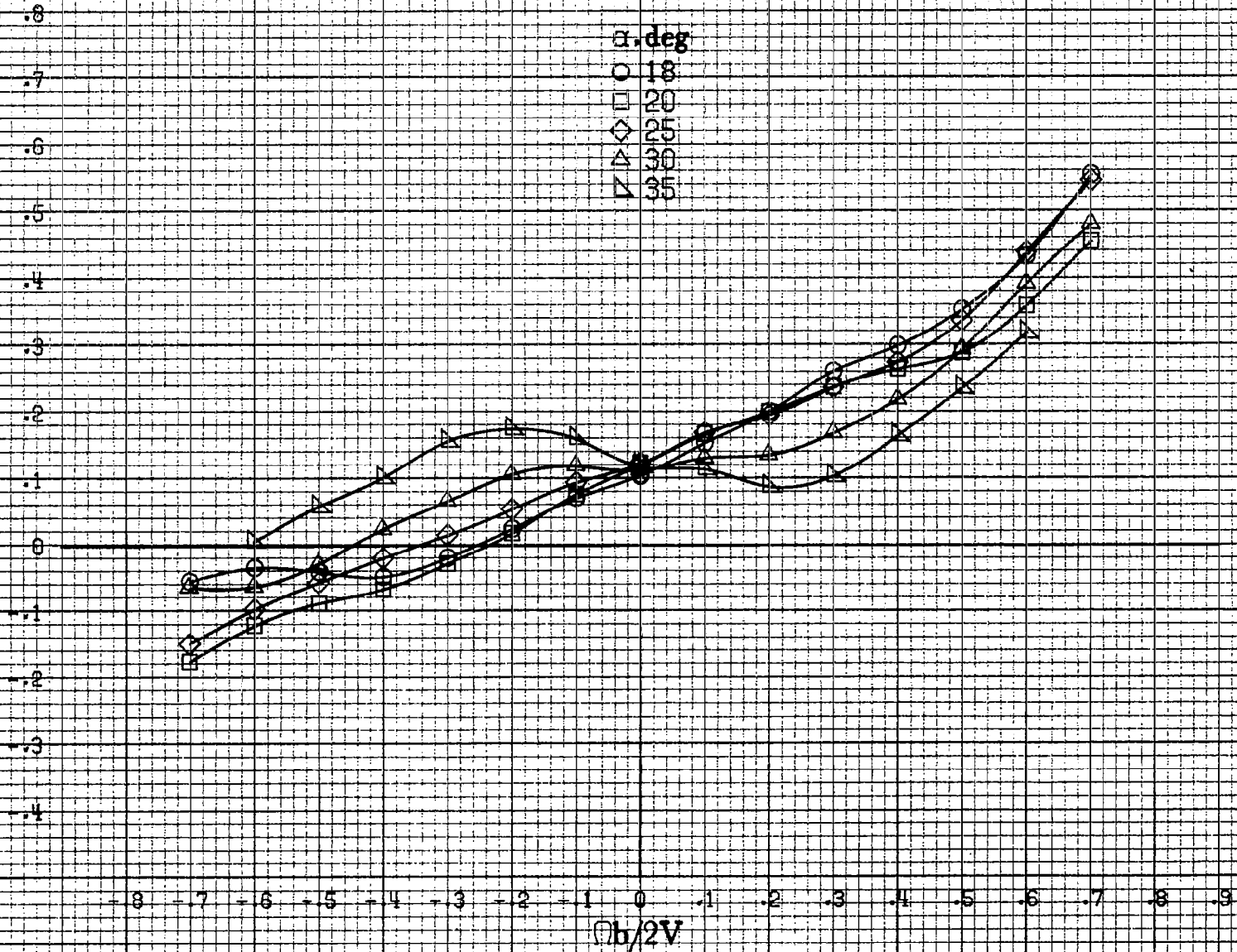
(b) \alpha = 18 to 35 deg, SR = 182.9 cm (72 in). Figure A17.-Continued.
