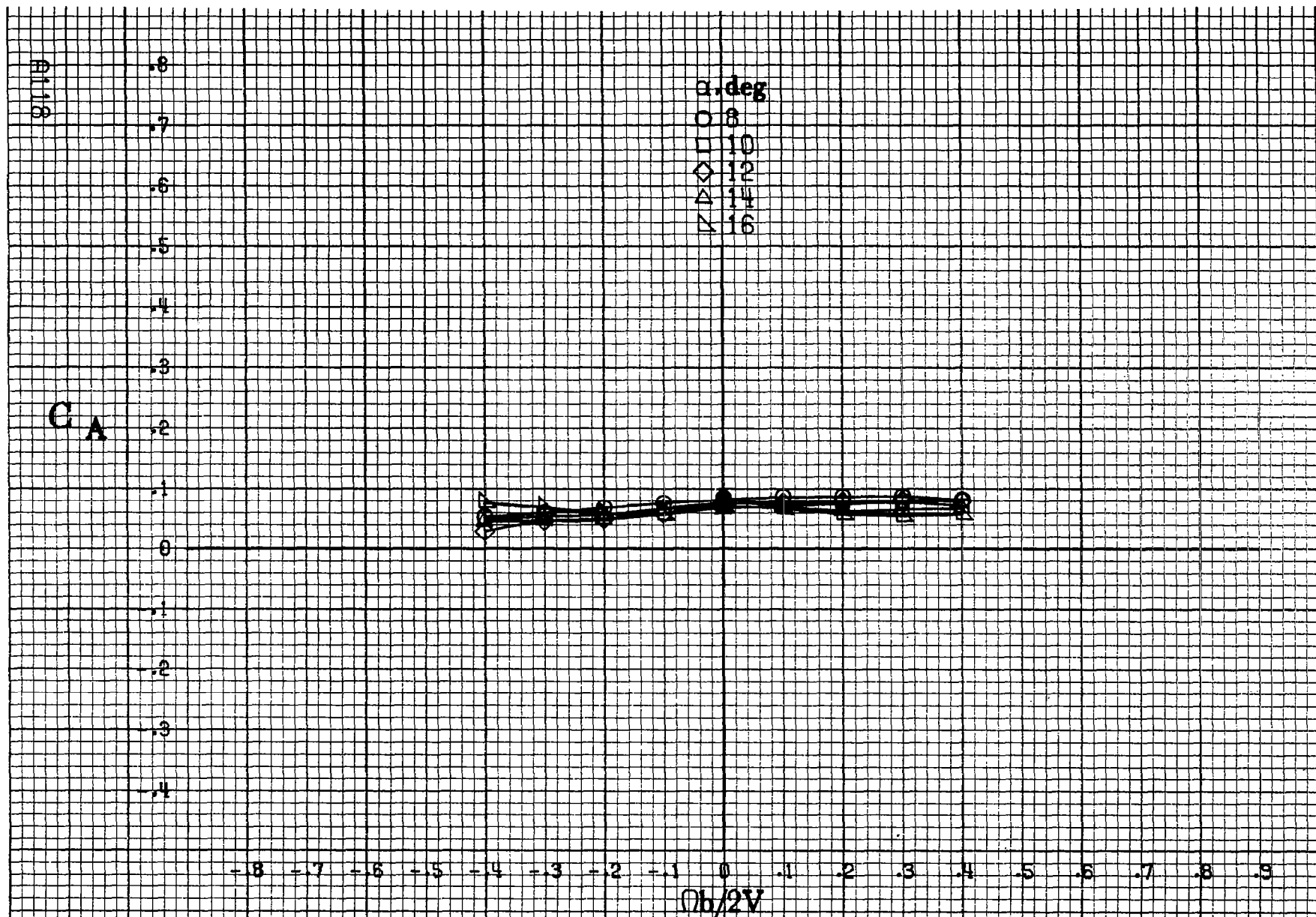
Figure A.30 - Effect of rotation rate and angle of attack on axial-force coefficient for basic configuration. \delta_e = 0^\circ , \delta_a = 0^\circ , \delta_d = 0^\circ , \delta_r = 0^\circ , \beta = 0^\circ .
