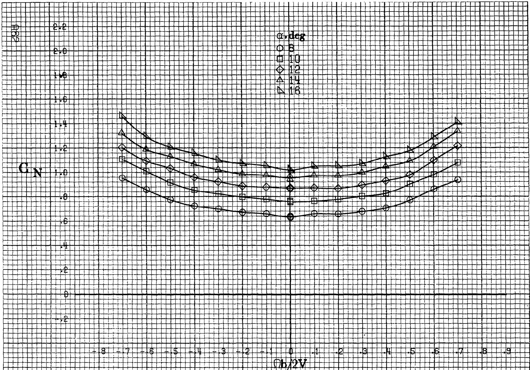
Figure A16.-Effect of rotation rate and angle of attack on normal-force coefficient for body wing vertical tail configuration \delta_e = 0^\circ , \delta_s = 0^\circ , \delta_r = 0^\circ , \delta = 0^\circ .
