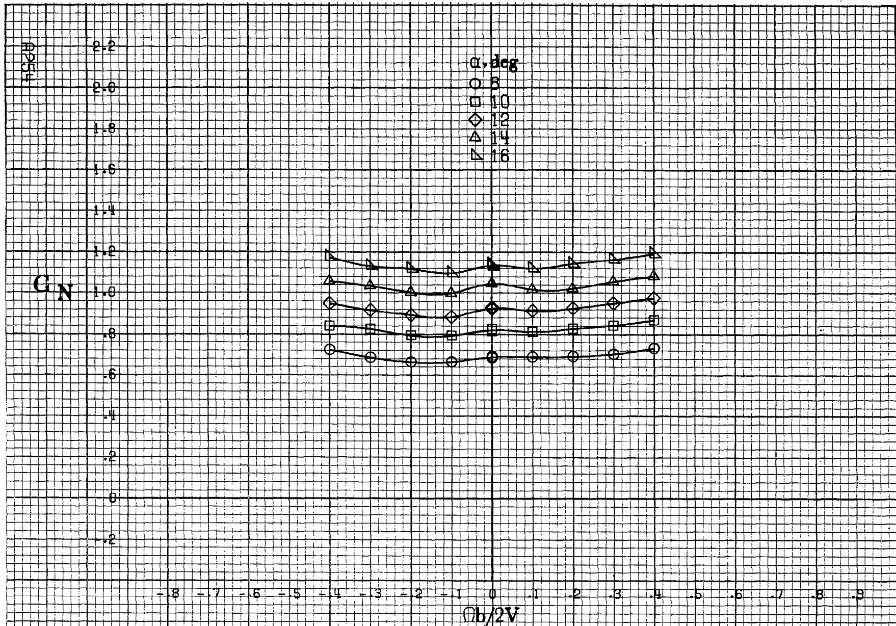
Figure A70.- Effect of rotation rate and angle of attack on normal-force coefficient for basic configuration. \delta_r = 0^\circ , \delta_a = 0^\circ , \delta_a = 11^\circ , \delta_r = 0^\circ , \beta = 0^\circ .
