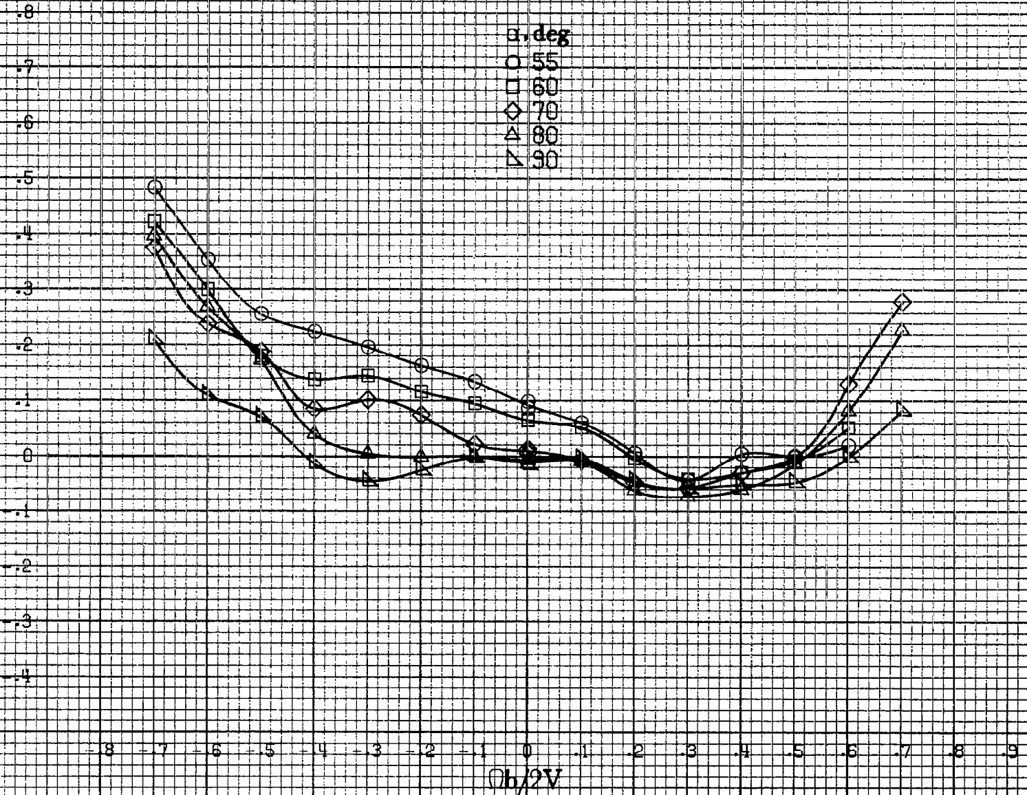
(d) \alpha = 55 to 90 deg, SR = 0 . Figure A 35.- Concluded.
