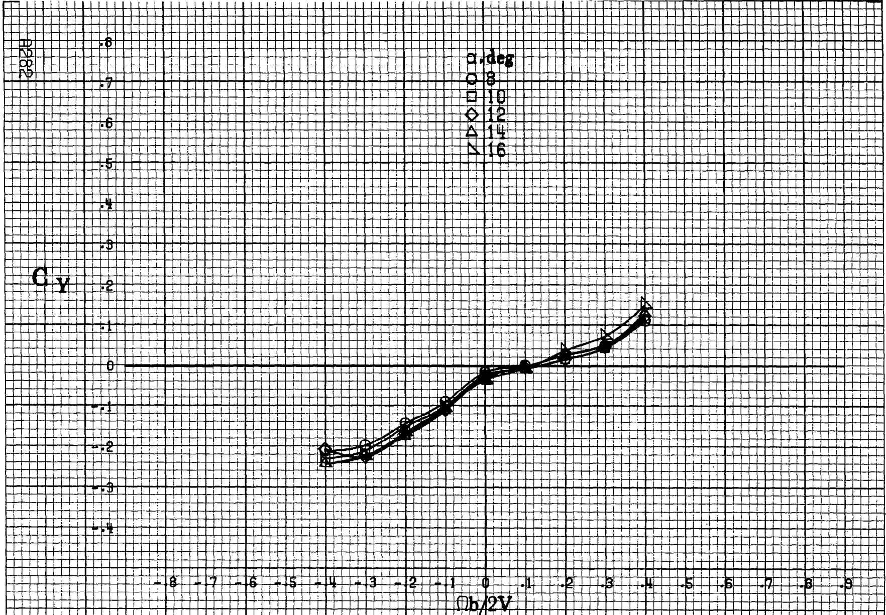
Figure A77.- Effect of rotation rate and angle of attack on side-force coefficient for basic configuration. \delta_e=0^\circ , \delta_a=0^\circ , \delta_A=11^\circ , \delta_r=0^\circ , B=10^\circ .
