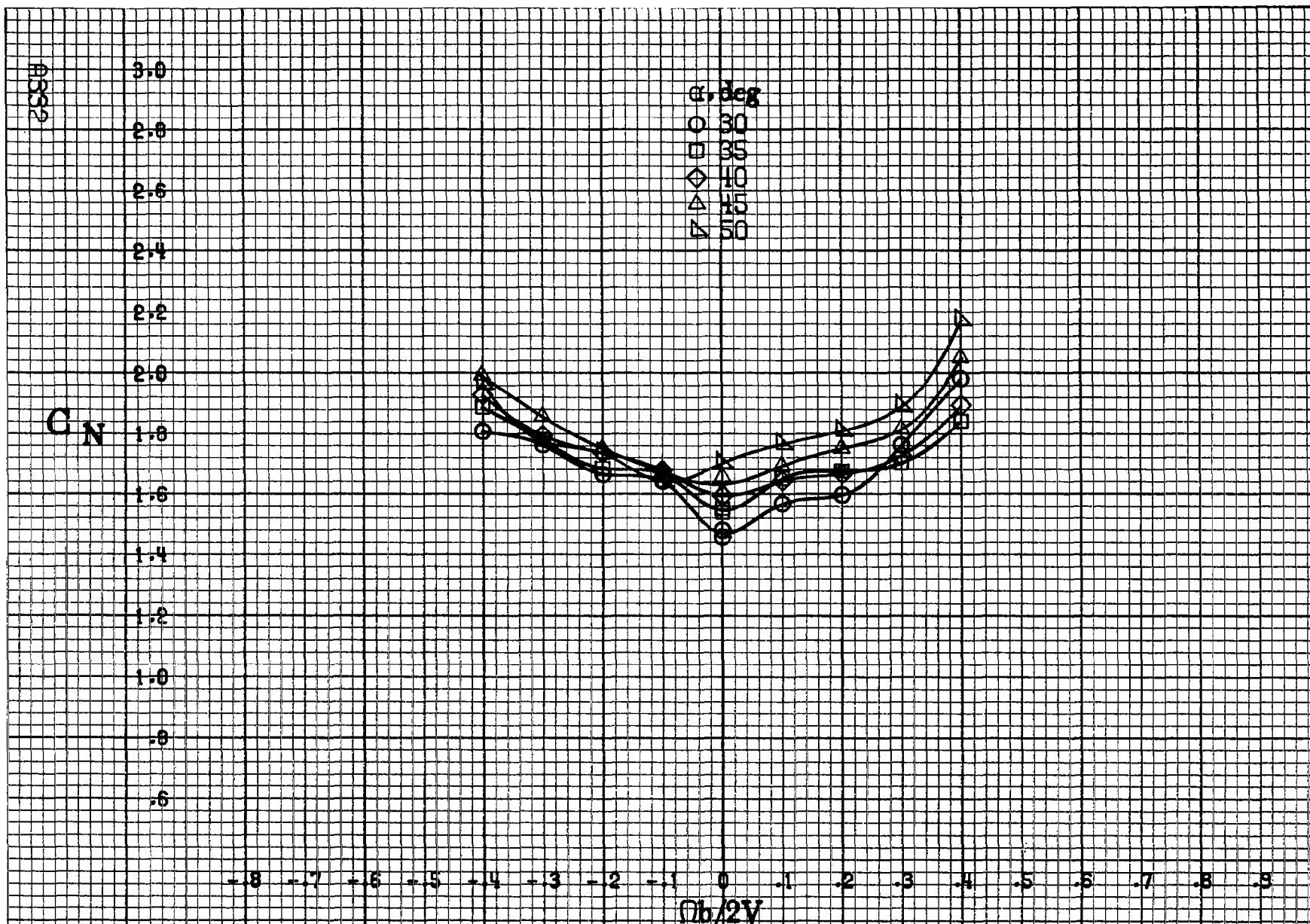
Figure A100.-Effect of rotation rate and angle of attack on normal-force coefficient for basic configuration. \delta_c = 0^\circ , \delta_a = 20.0^\circ , \delta_d = 6^\circ , \delta_r = -15^\circ , \beta = 10^\circ .
