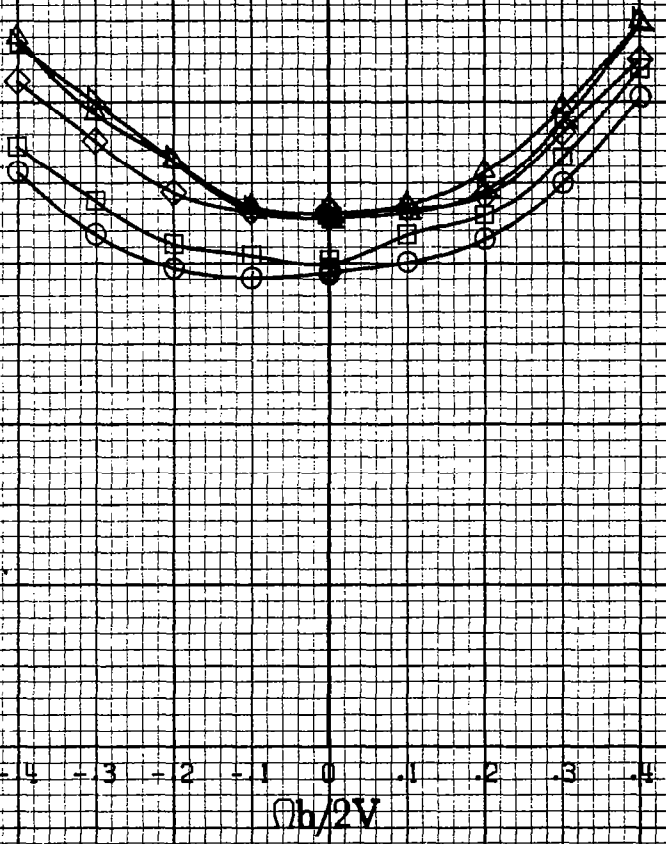
(b) \alpha=55 to 90 deg, SR=0 . Figure A52.- Concluded.
