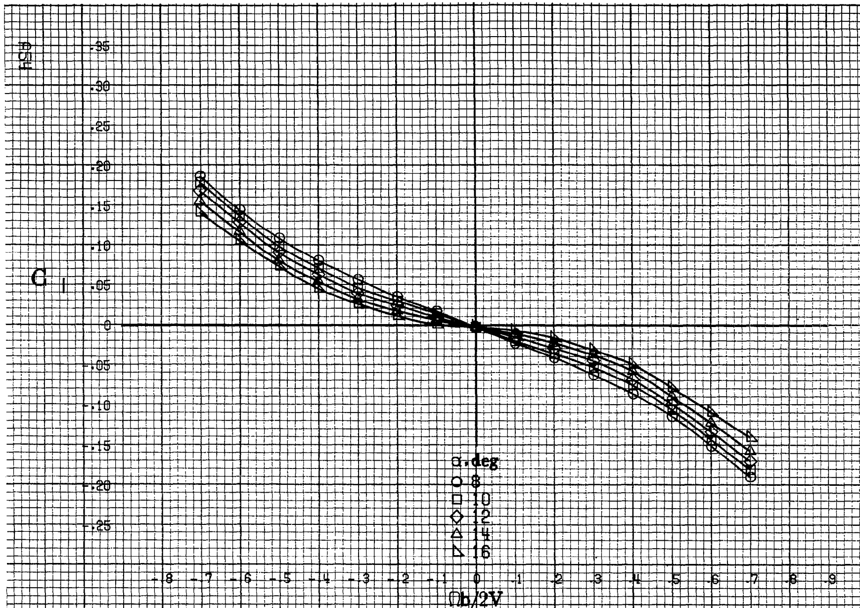
Figure A14. Effect of rotation rate and angle of attack on rolling-moment coefficient for body wing vertical tail configuration \delta_a = 0^\circ , \delta_s = 0^\circ , \delta_r = 0^\circ , \delta = 0^\circ .
