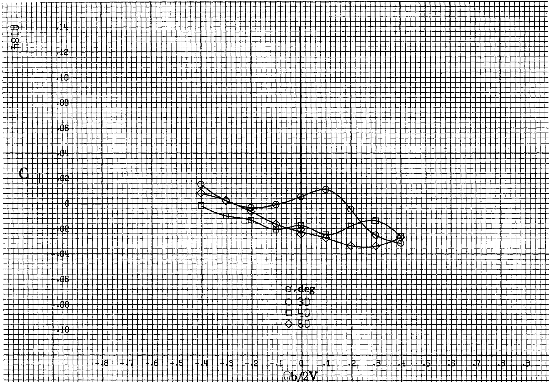
Figure A 50 - Effect of rotation rate and angle of attack on rolling-moment coefficient for basic configuration. \delta_c = 25^\circ , \delta_a = 0^\circ , \delta_d = 0^\circ , \delta_r = 0^\circ , \delta = 10^\circ .
