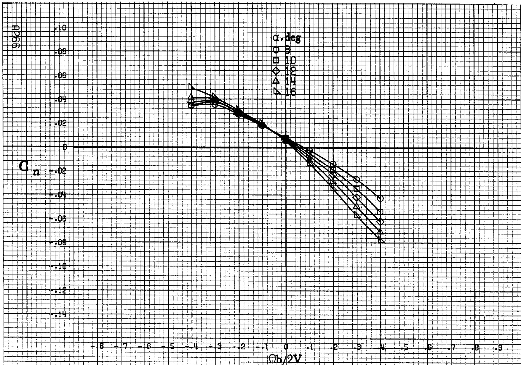
Figure A73.-Effect of rotation rate and angle of attack on yawing-moment coefficient for basic configuration. \delta_e = 0^\circ , \delta_a = 0^\circ , \delta_d = 11^\circ , \delta_r = 0^\circ , \beta = 10^\circ .
