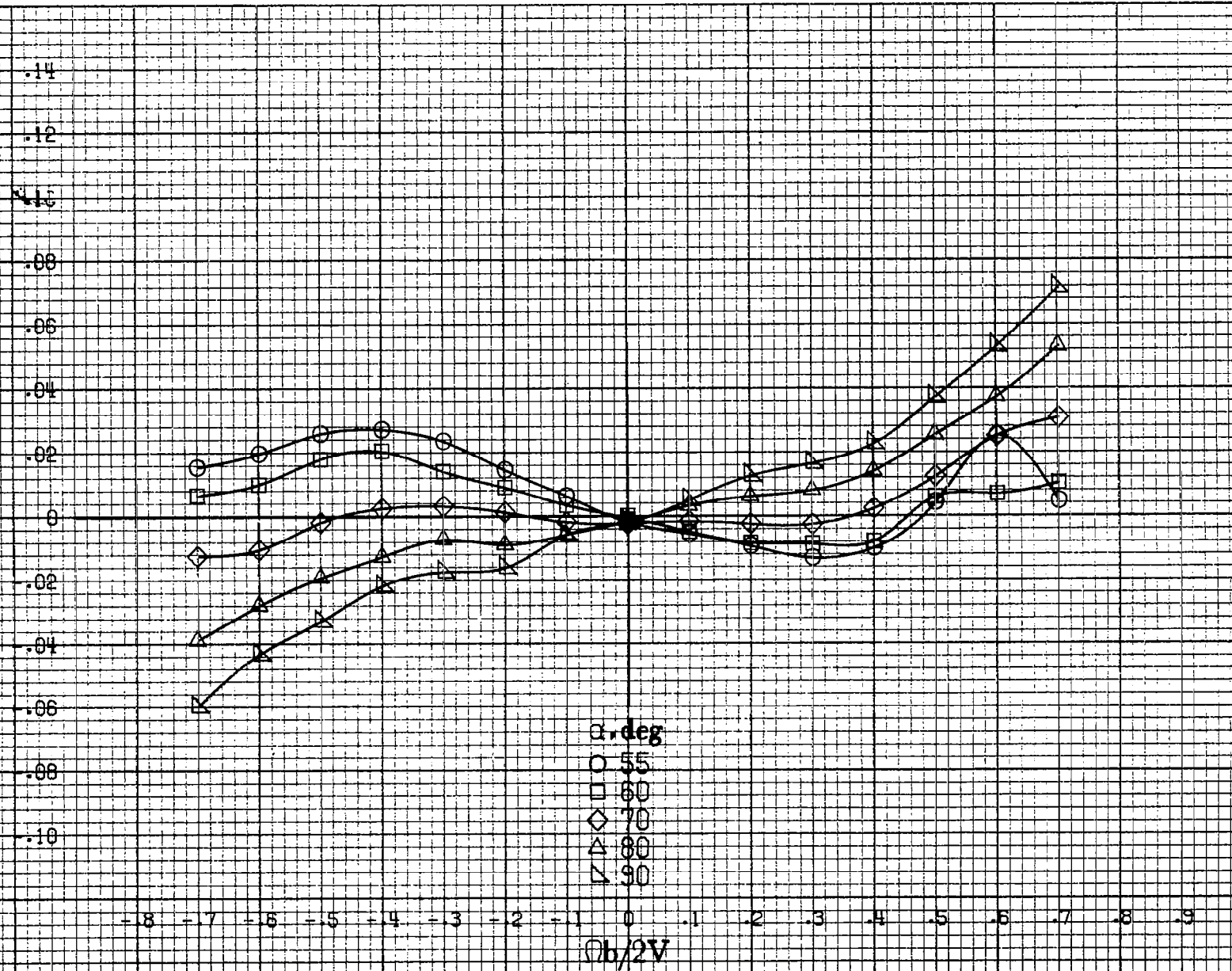
(d) \alpha=55 to 90 deg, SR=0 . Figure A8.- Concluded.
