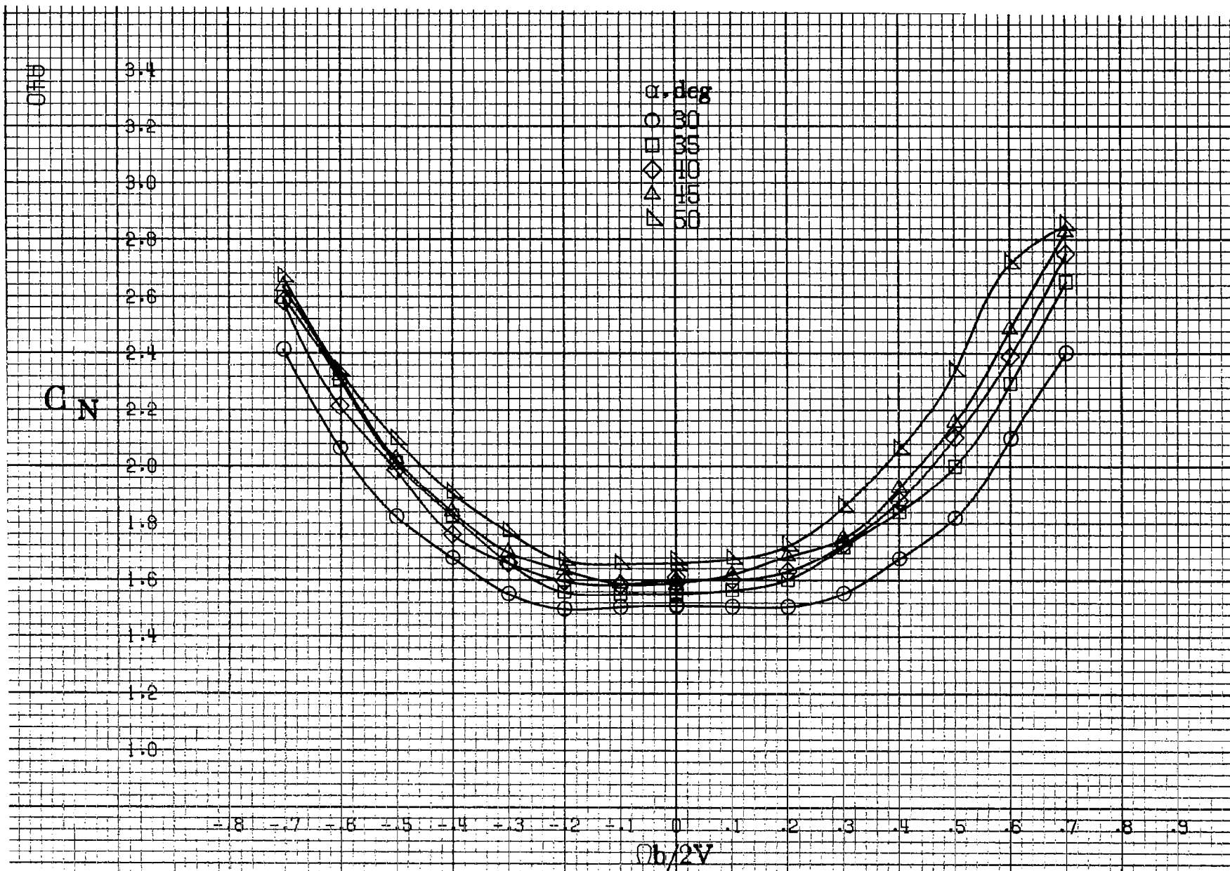
(c) \alpha = 30 to 50 deg, SR = 0 . Figure A-10.-Continued.
