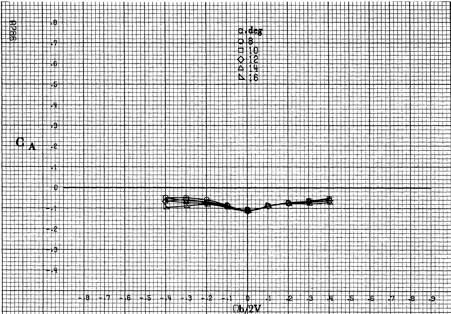
Figure A78.-Effect of rotation rate and angle of attack on axial-force coefficient for basic configuration. \delta_c = 0^\circ , \delta_s = 0^\circ , \delta_a = 11^\circ , \delta_r = 0^\circ , B = 10^\circ .
