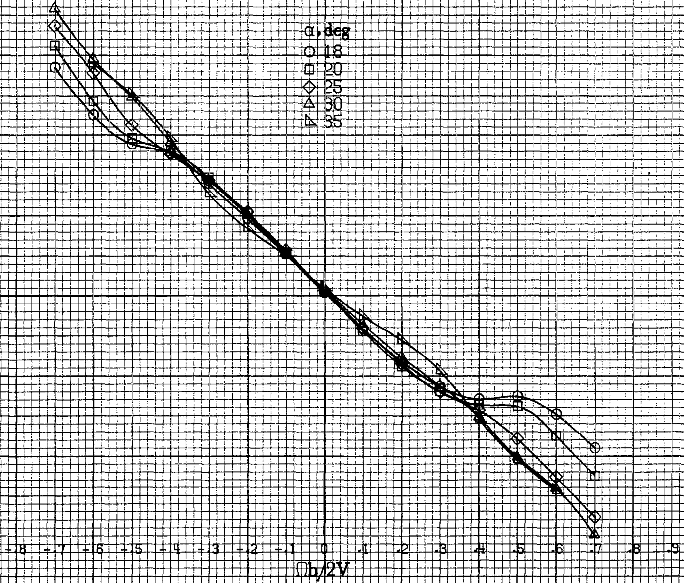
(b) \alpha=18 to 35 deg, SR = 182.9 cm (72 in). Figure A13.-Continued.
