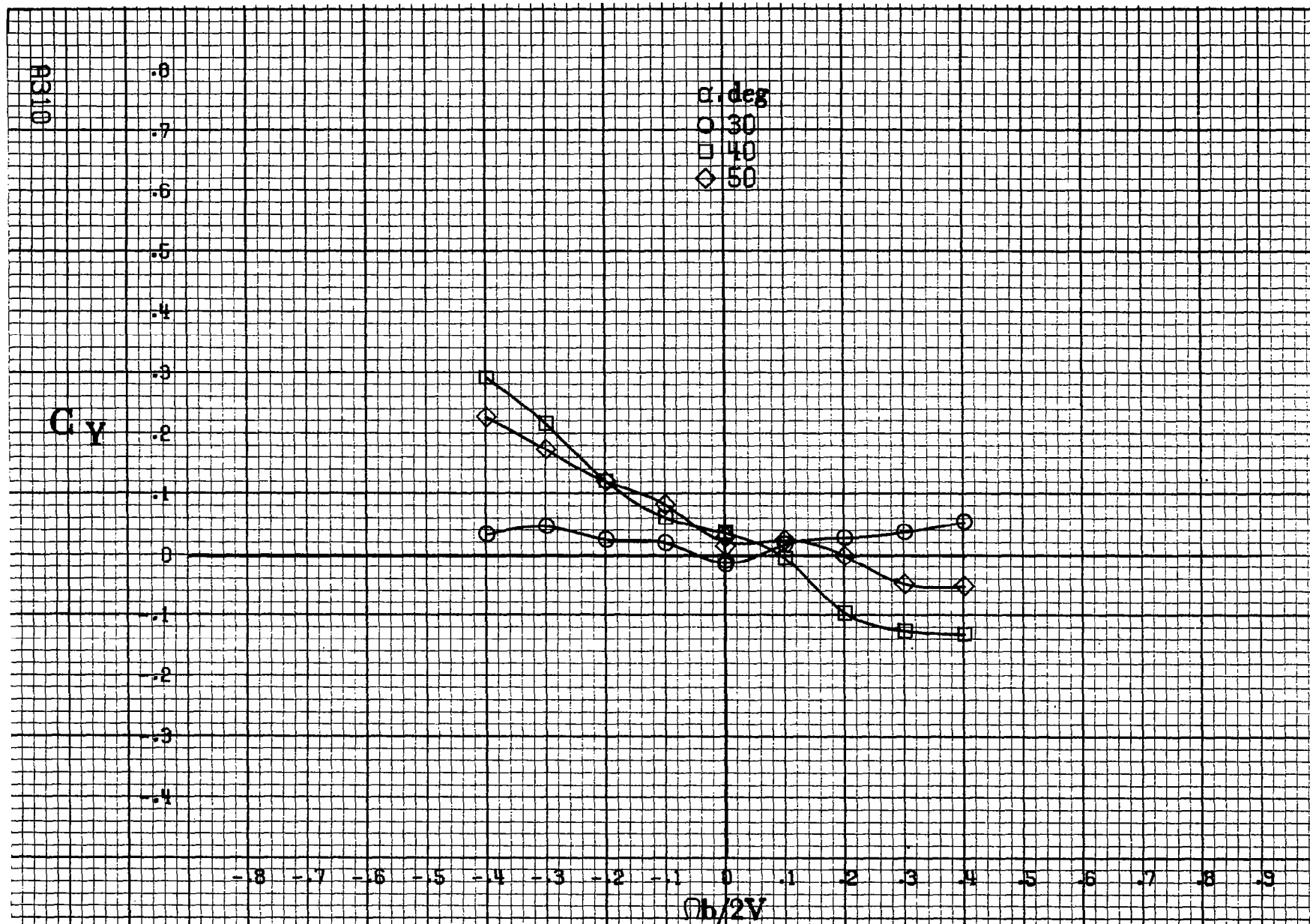
Figure A 89.- Effect of rotation rate and angle of attack on side-force coefficient for basic configuration. \delta_e = 0^\circ , \delta_a = 20.0^\circ , \delta_{\dot{a}} = 6^\circ , \delta_r = 0^\circ , \beta = 10^\circ .
