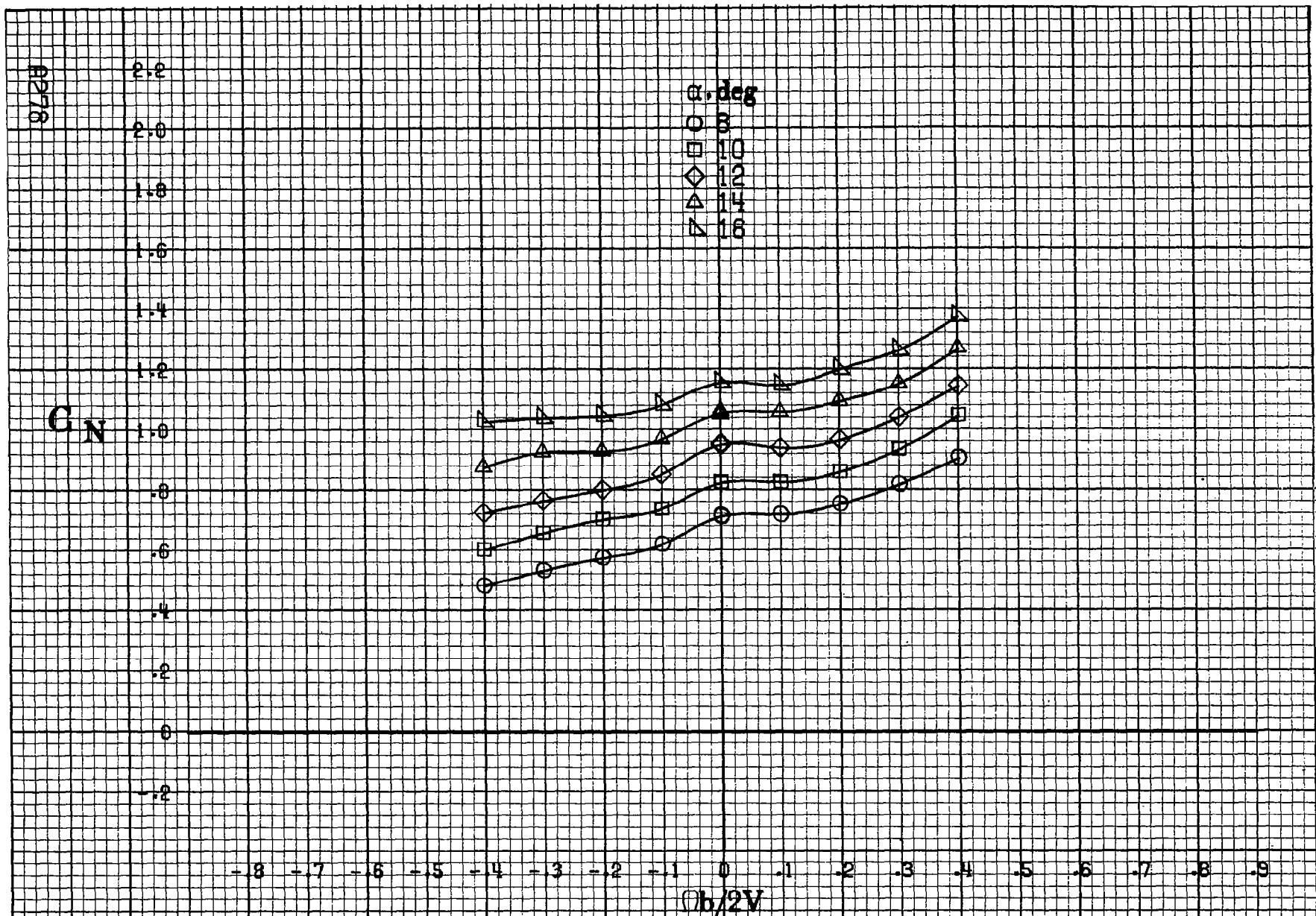
Figure A 76.-Effect of rotation rate and angle of attack on normal-force coefficient for basic configuration. \delta_e = 0^\circ , \delta_a = 0^\circ , \delta_{\alpha} = 11^\circ , \delta_r = 0^\circ , \beta = 10^\circ .
