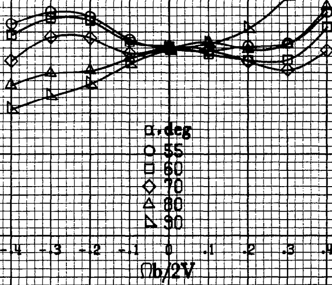
(d) \alpha = 55 to 90 deg, SR = 0 . Figure A74.- Concluded.
