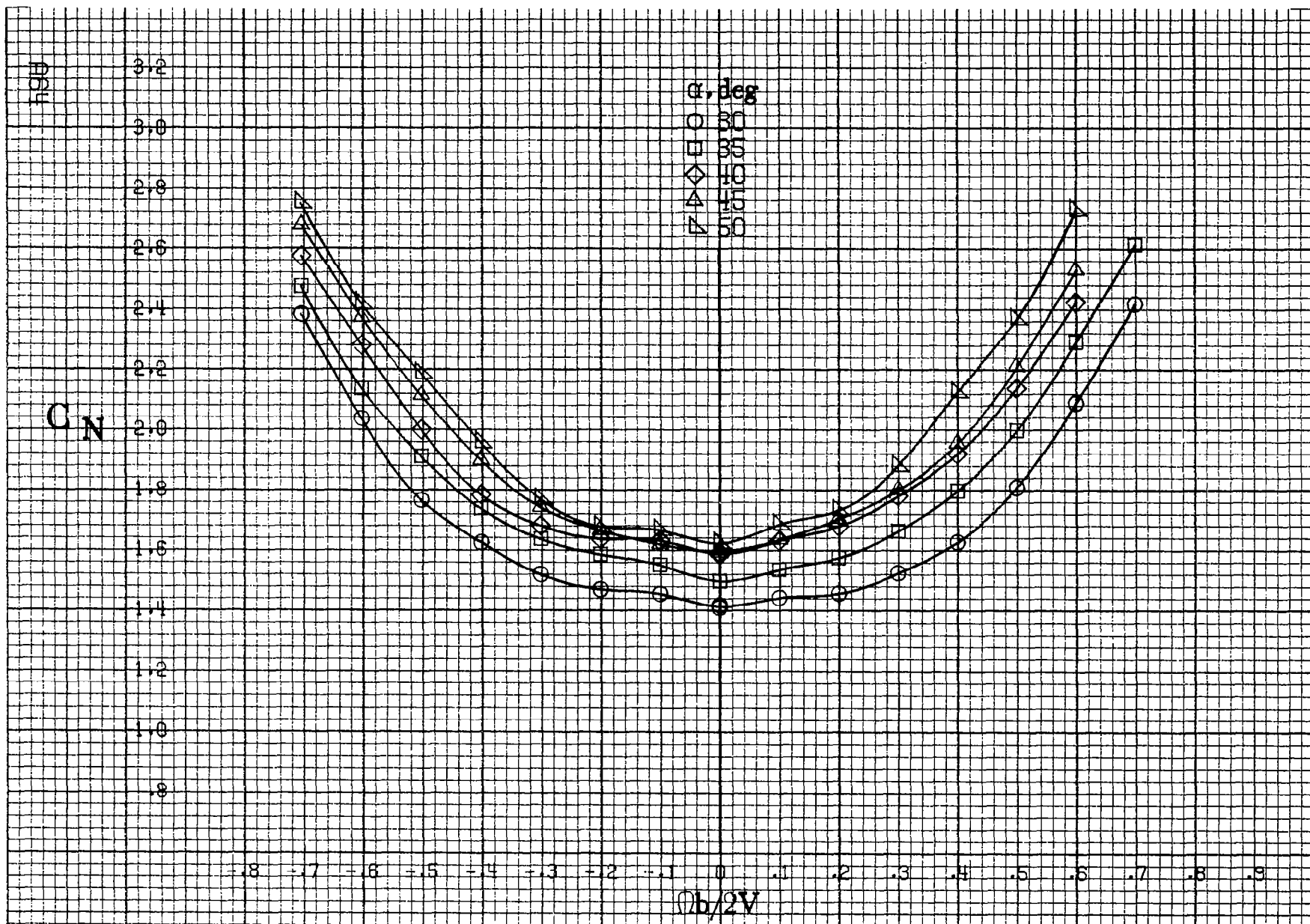
(c) \alpha = 30 to 50 deg, SR = 0 . Figure A16.-Continued.
