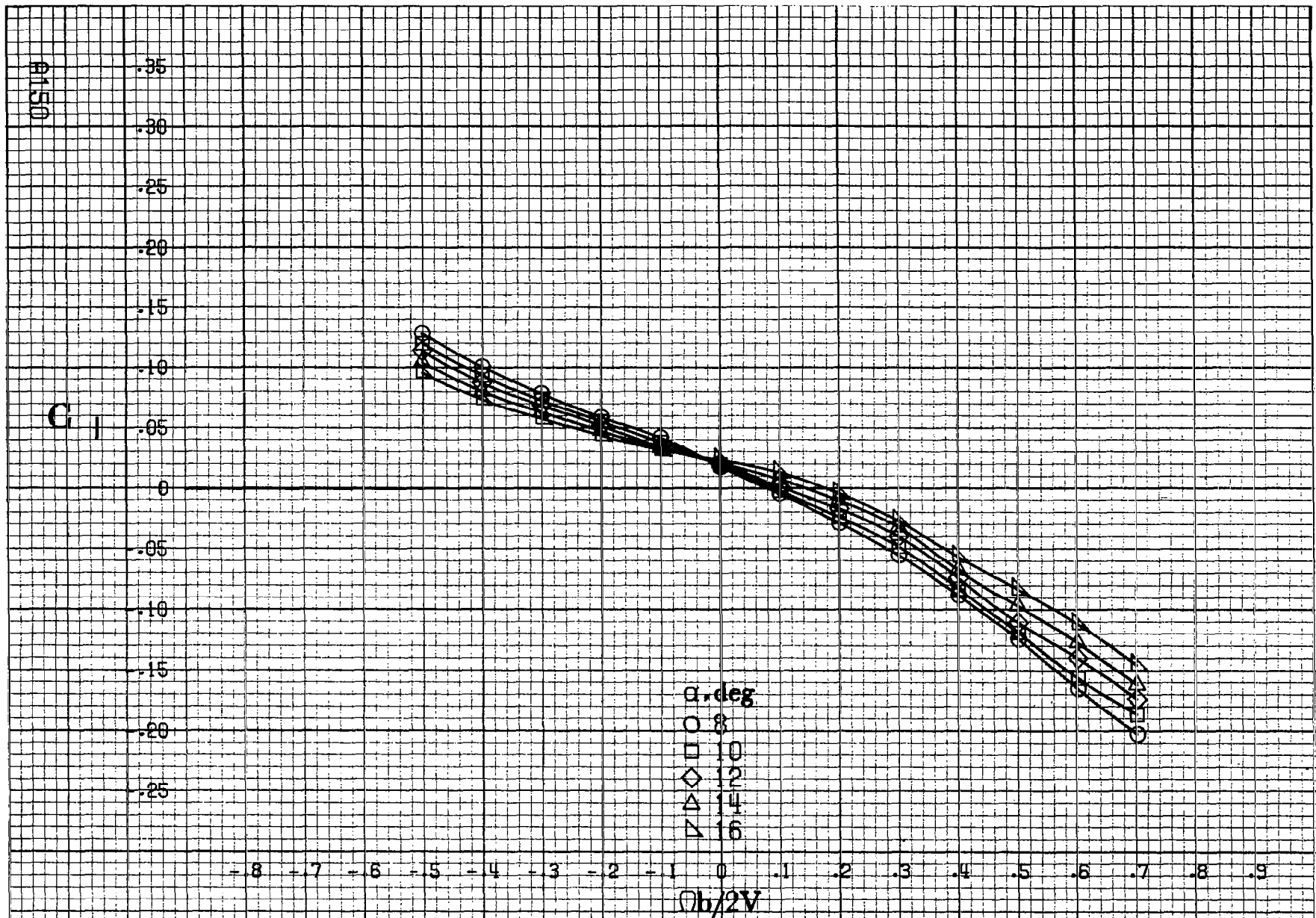
Figure A38.-Effect of rotation rate and angle of attack on rolling-moment coefficient for basic configuration. \delta_e = 0^\circ , \delta_a = 0^\circ , \delta_{\dot{a}} = 0^\circ , \delta_r = 0^\circ , B = -10^\circ .
