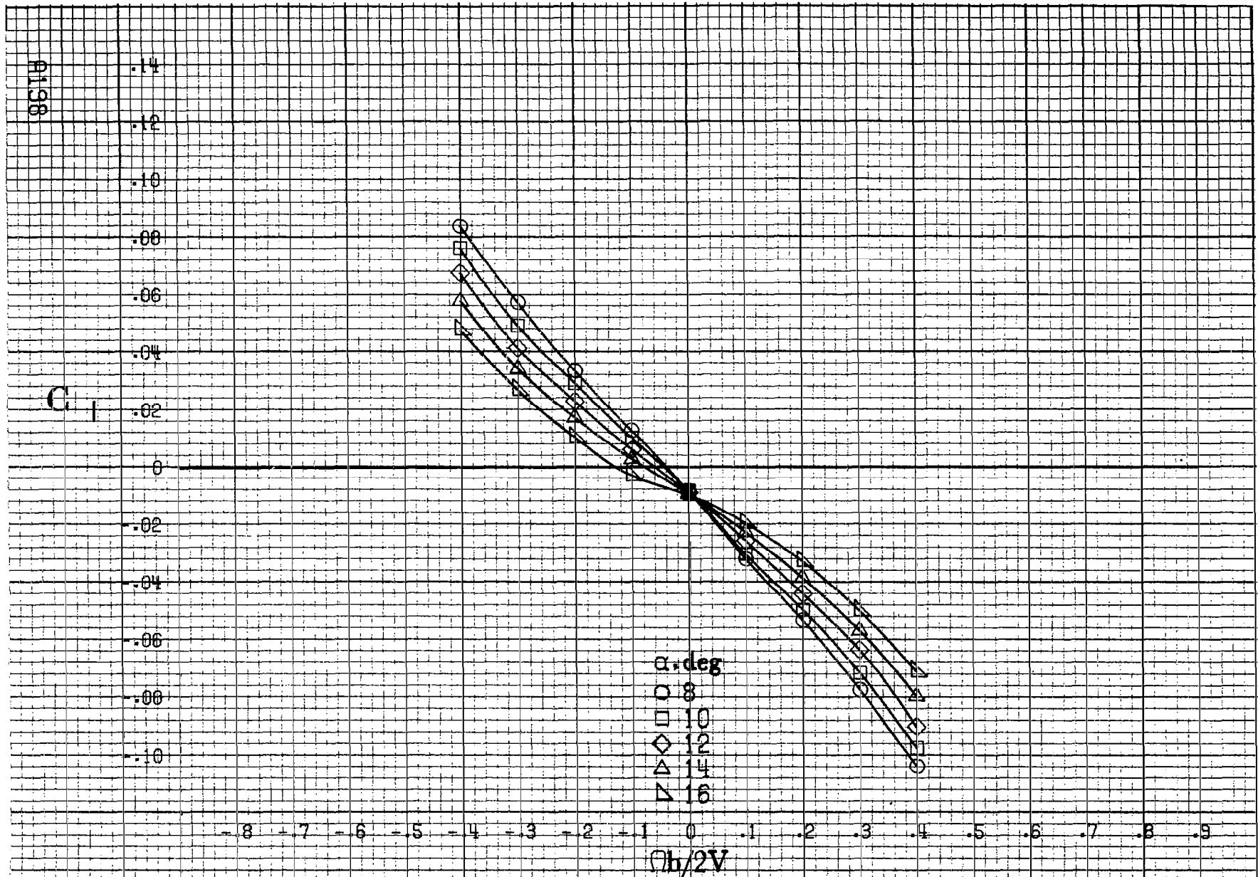
(a) \alpha = 8 to 16 deg, SR = 182.9 em (72 in).
