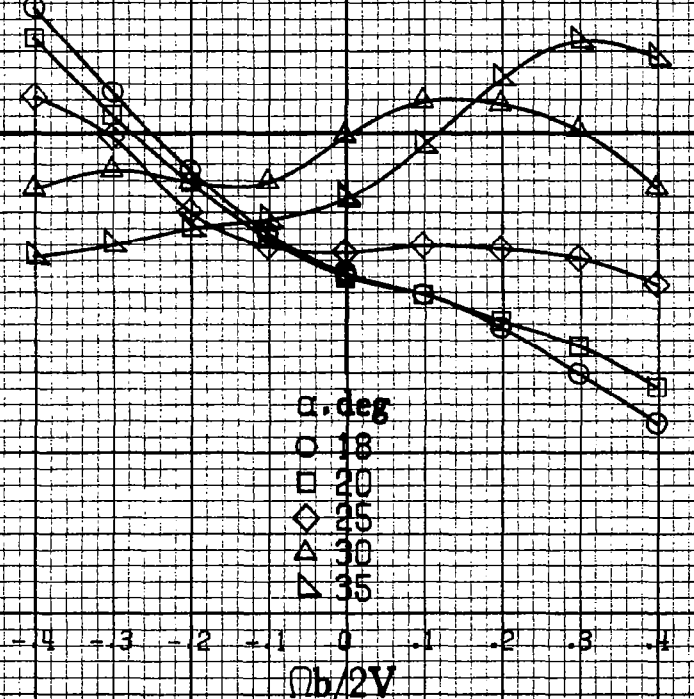
(b) \alpha = 18 to 35 deg, SR = 182.9 cm (72 in). Figure A 62.-Continued.
