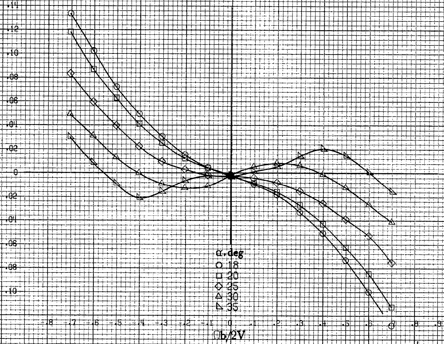
(b) α = 18 to 35 deg. SR = 182.9 cm (72 in). Figure A 20.-Continued.
