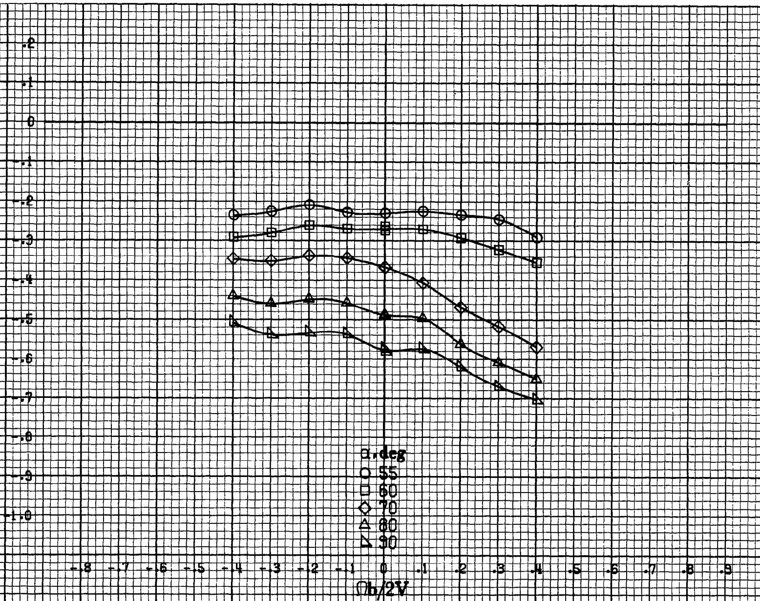
(d) \alpha = 55 to 90 deg, SR = 0 . Figure A 75.-Concluded.
