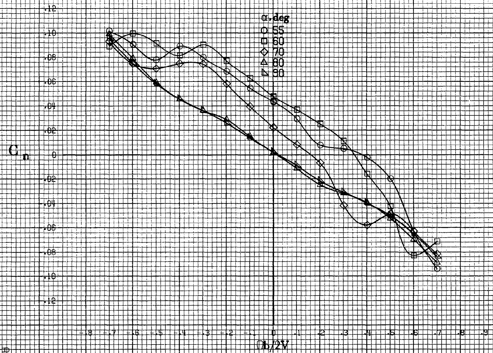
(d) \alpha = 55 to 90 deg, SR = 0 . Figure A1.-Concluded.
