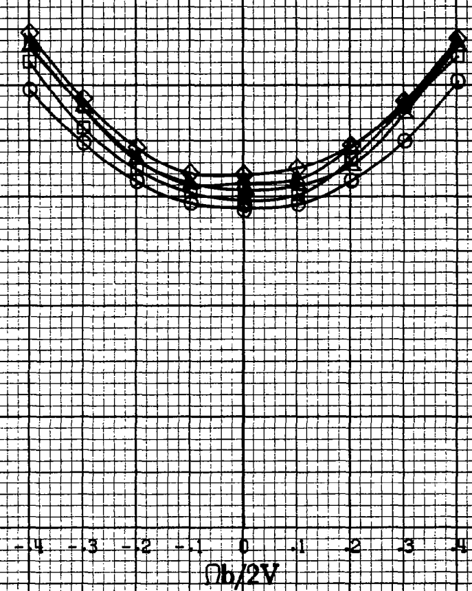
(d) \alpha=55\text{to}90\text{deg} , SR=0 . Figure A58.-Concluded.
