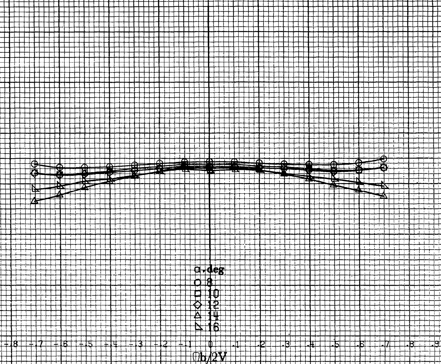
(a) \alpha = 8 to 16 deg, SR = 132.9 cm (72 in).
