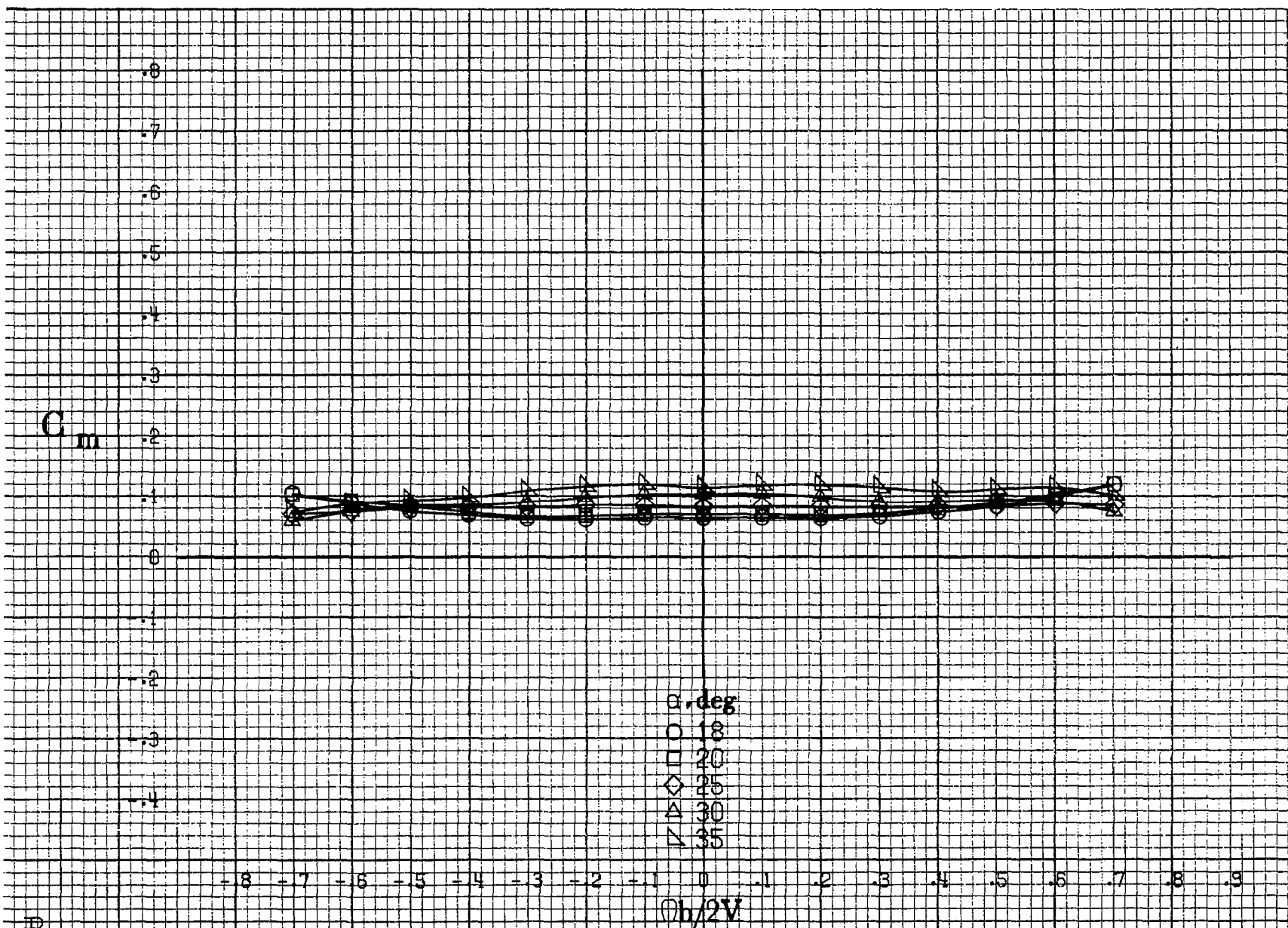
(b) \alpha = 18 to 35 deg, SR = 182.9 cm (72 in). Figure A9.-Continued.
