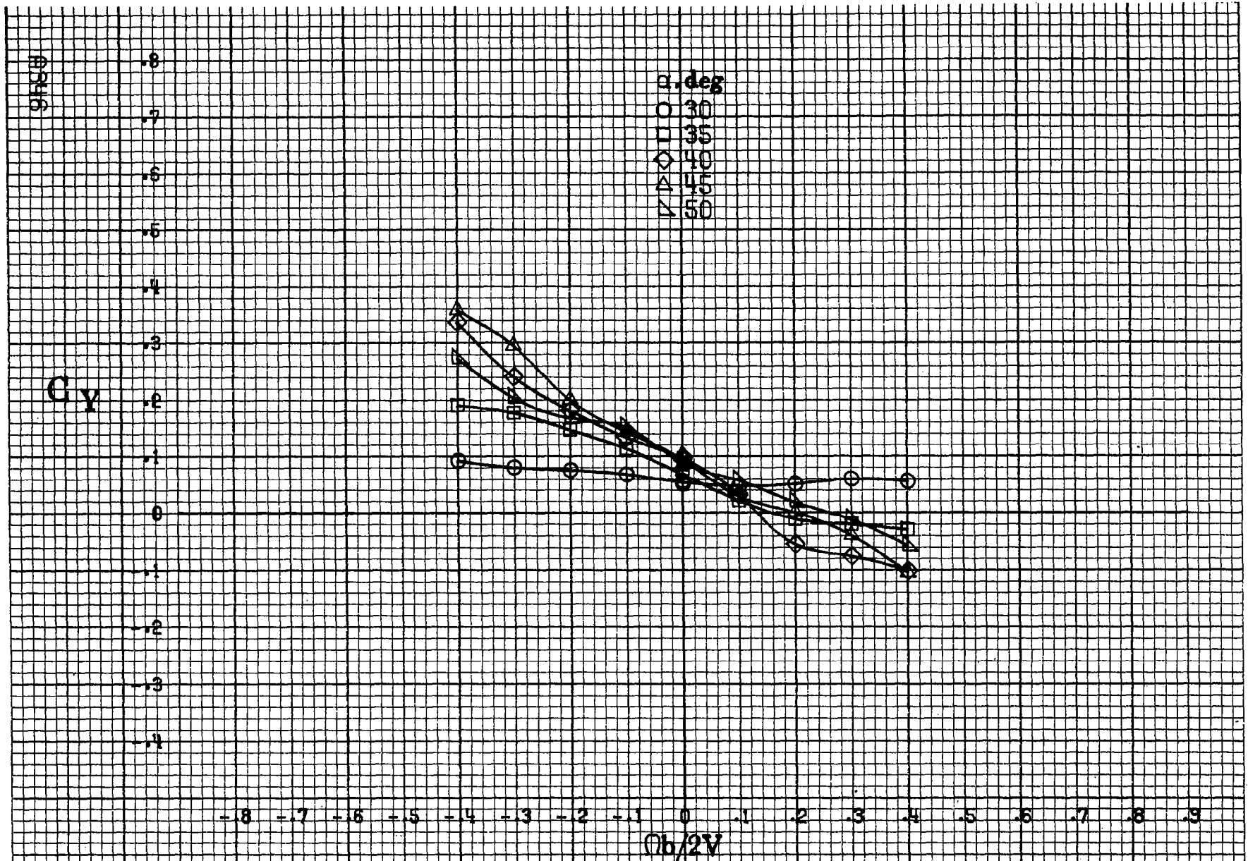
Figure A107.-Effect of rotation rate and angle of attack on side-force coefficient for basic configuration. \delta_r = 0^\circ , \delta_a = -20.0^\circ , \delta_a = -6^\circ , \delta_r = 30^\circ , \beta = 0^\circ .
