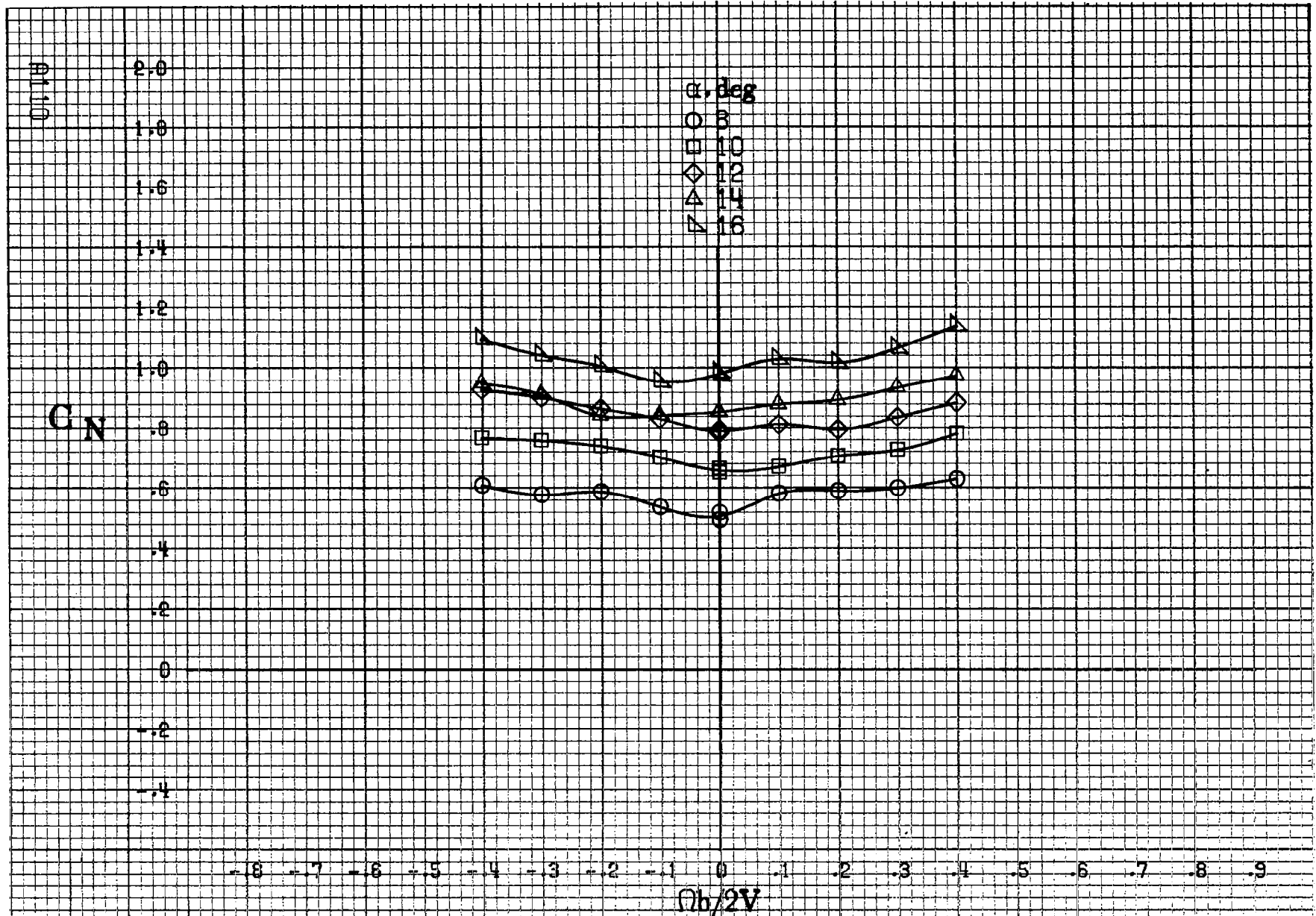
Figure A-28.-Effect of rotation rate and angle of attack on normal-force coefficient for basic configuration. \delta_a = 0^\circ , \delta_s = 0^\circ , \delta_{sa} = 0^\circ , \delta_r = 0^\circ , \beta = 0^\circ .
