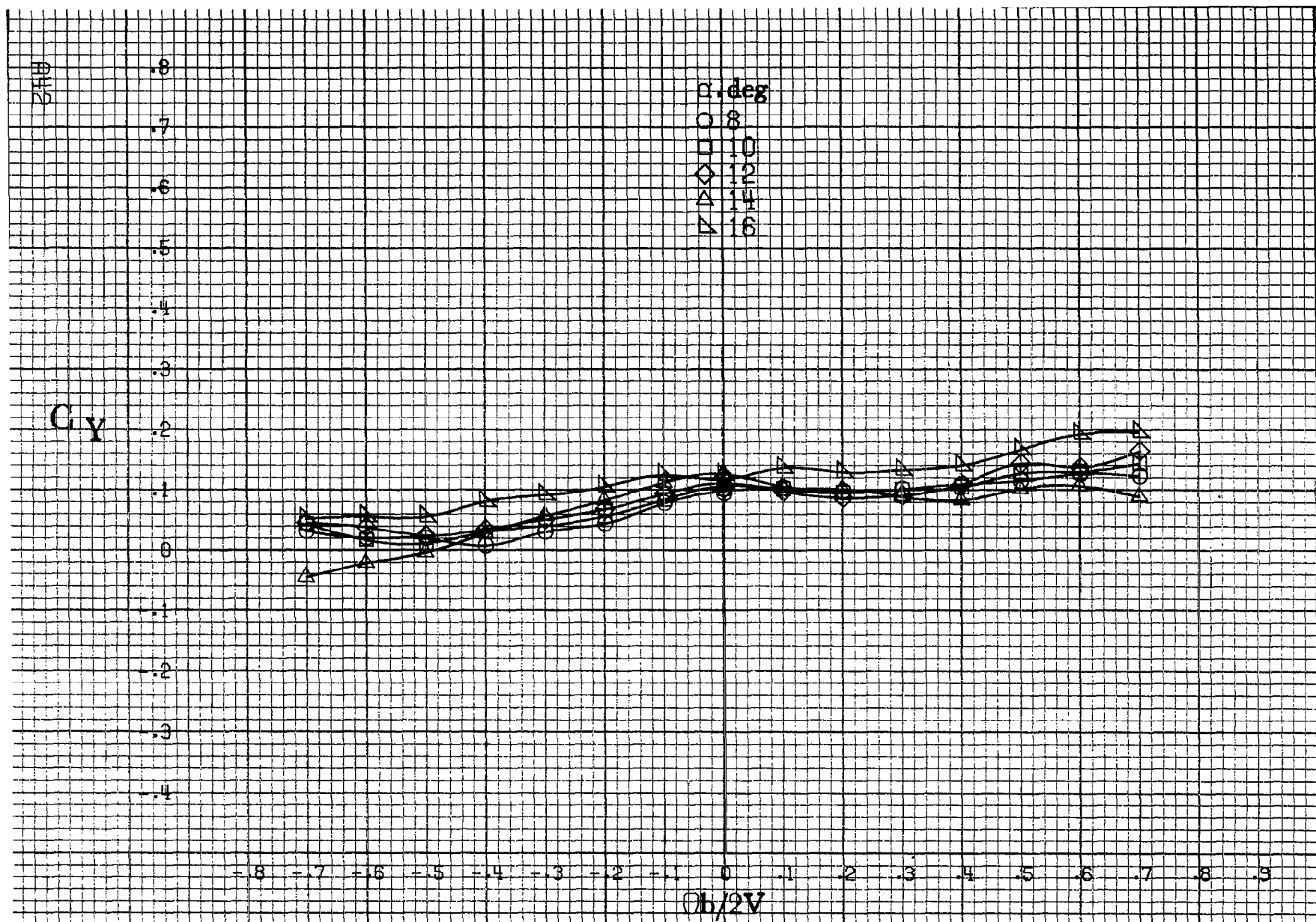
Figure A11.-Effect of rotation rate and angle of attack on side-force coefficient for body wing configuration. \delta_e = 0^\circ , \delta_s = 0^\circ , \delta_r = 0^\circ , \beta = 0^\circ .
