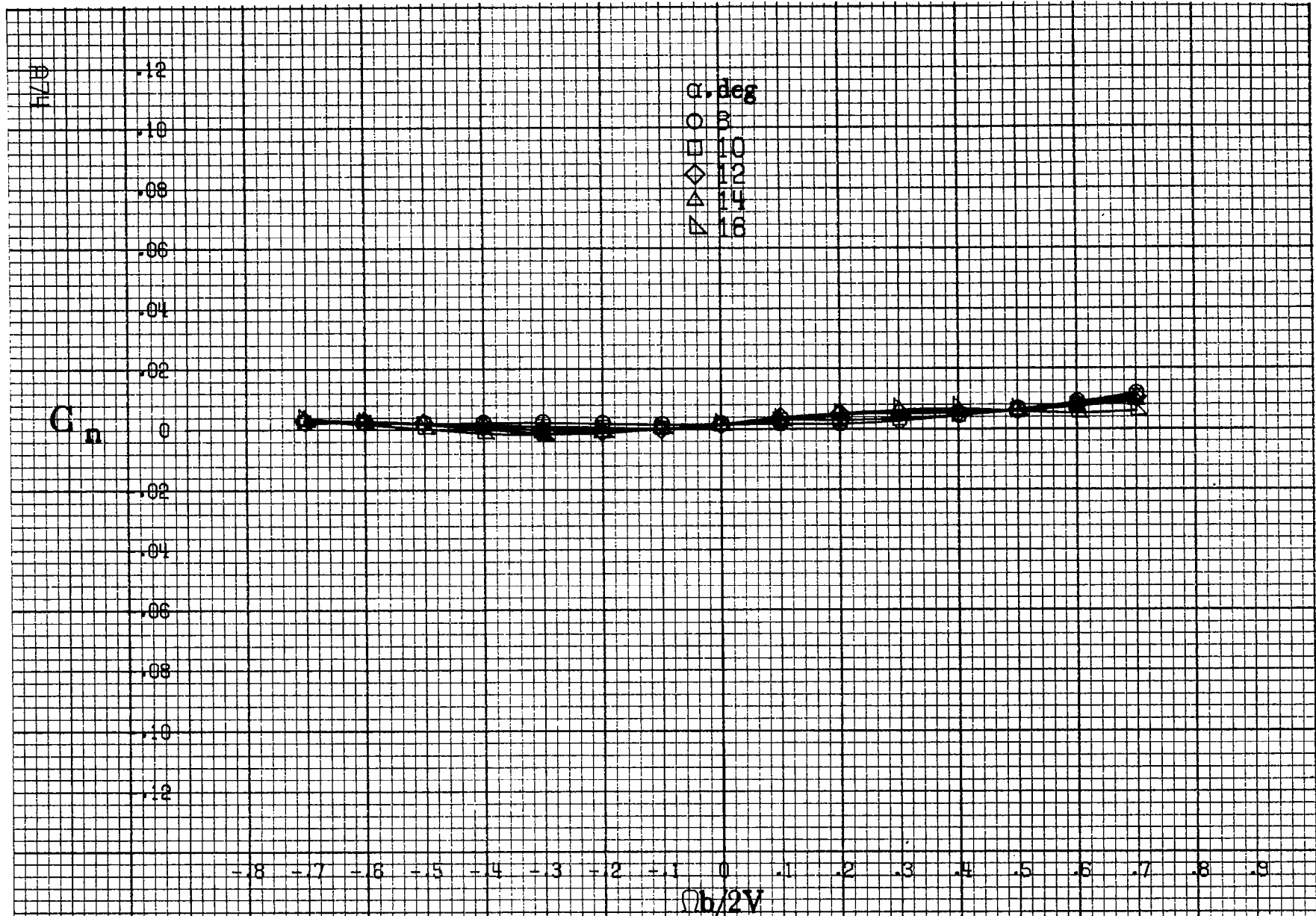
Figure A19 - Effect of rotation rate and angle of attack on yawing-moment coefficient for body wing horizontal tail configuration \delta_e = 0^\circ , \delta_s = 0^\circ , \delta_r = 0^\circ , \beta = 0^\circ .
