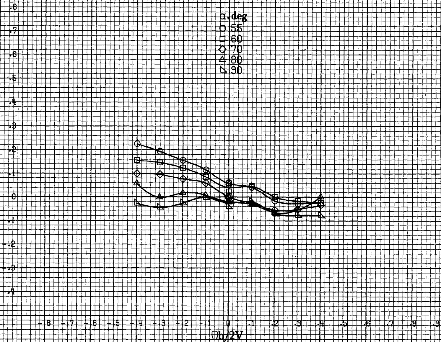
(b) \alpha = 55 to 90 deg, SR = 0 . Figure A 89.-Concluded.
