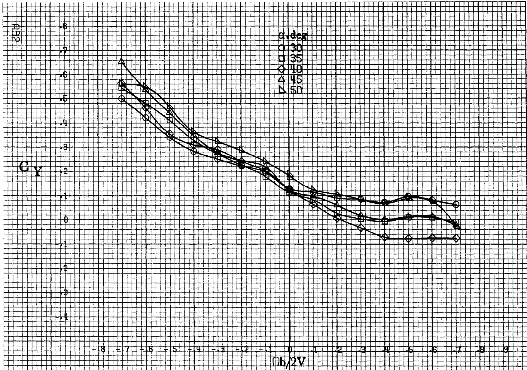
(c) \alpha=30 to 50 deg, SR=0 . Figure A23.-Continued.
