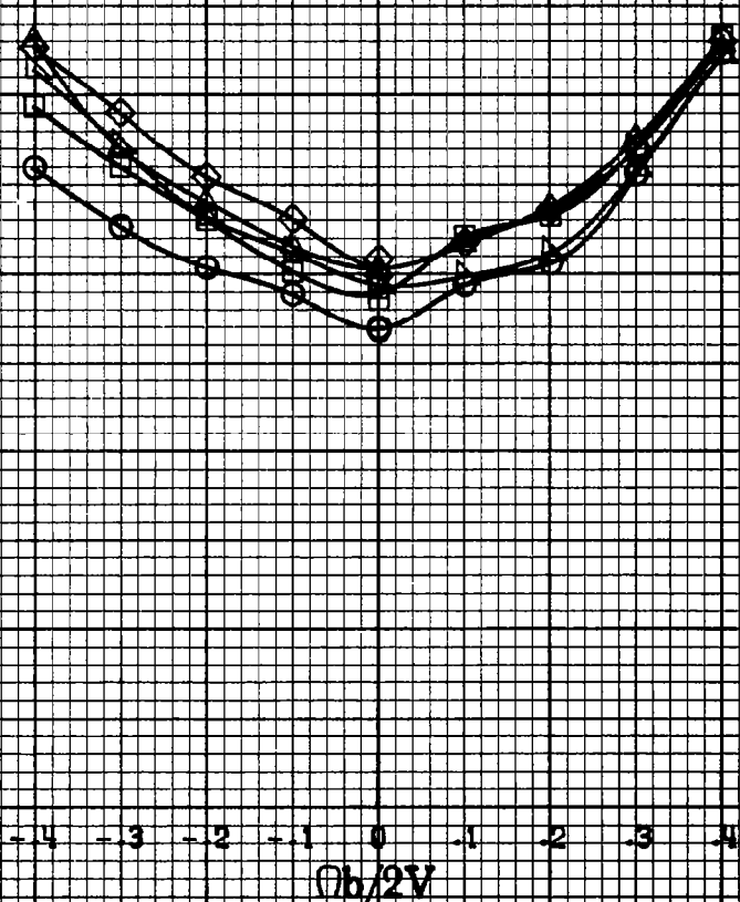
(b) \alpha = 55 to 90 deg, SR = 0 . Figure A100.-Concluded.
