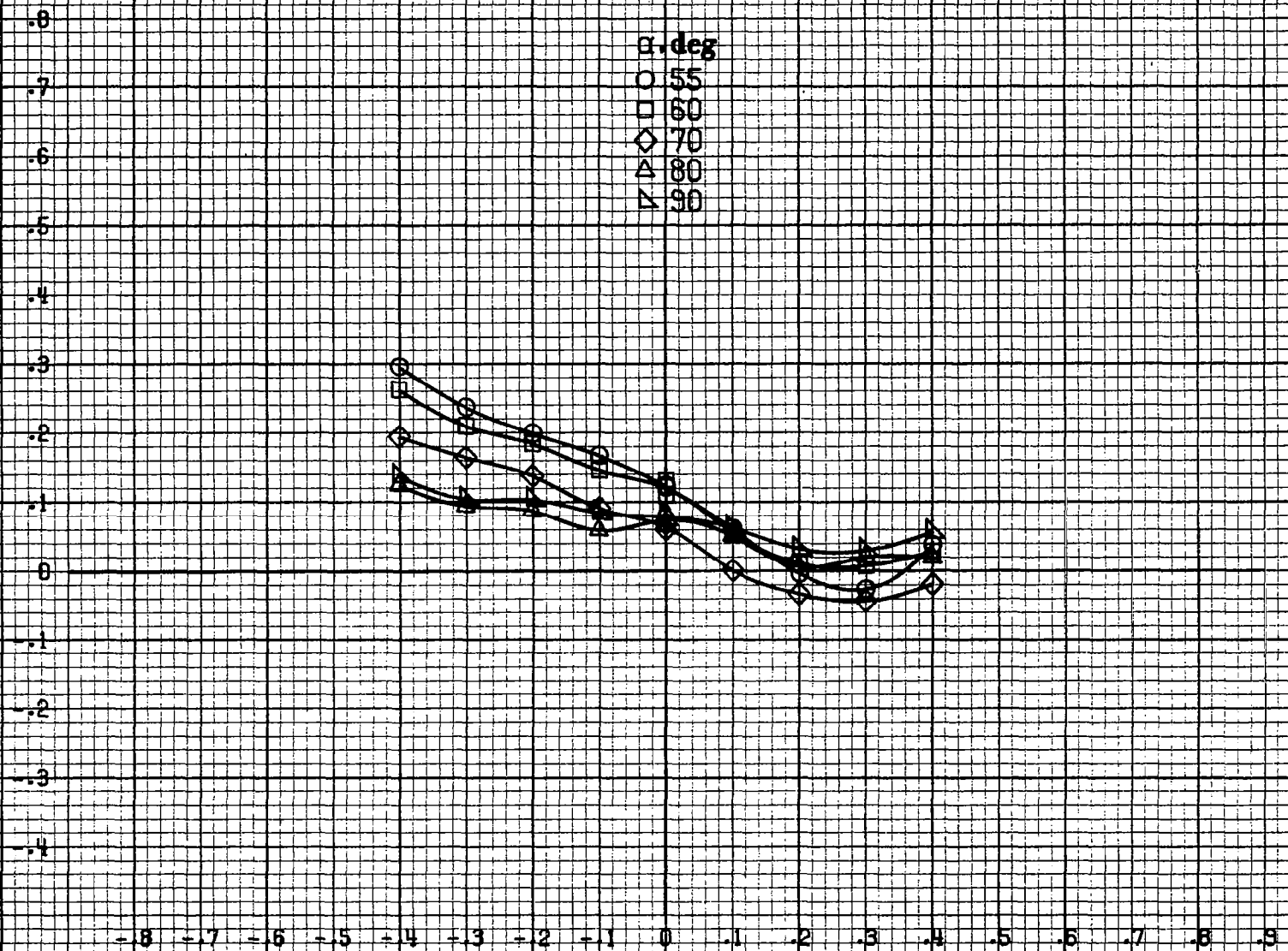
(d) \alpha=55\text{to}90\text{deg} , SR=0 . Figure A59.-Concluded.
