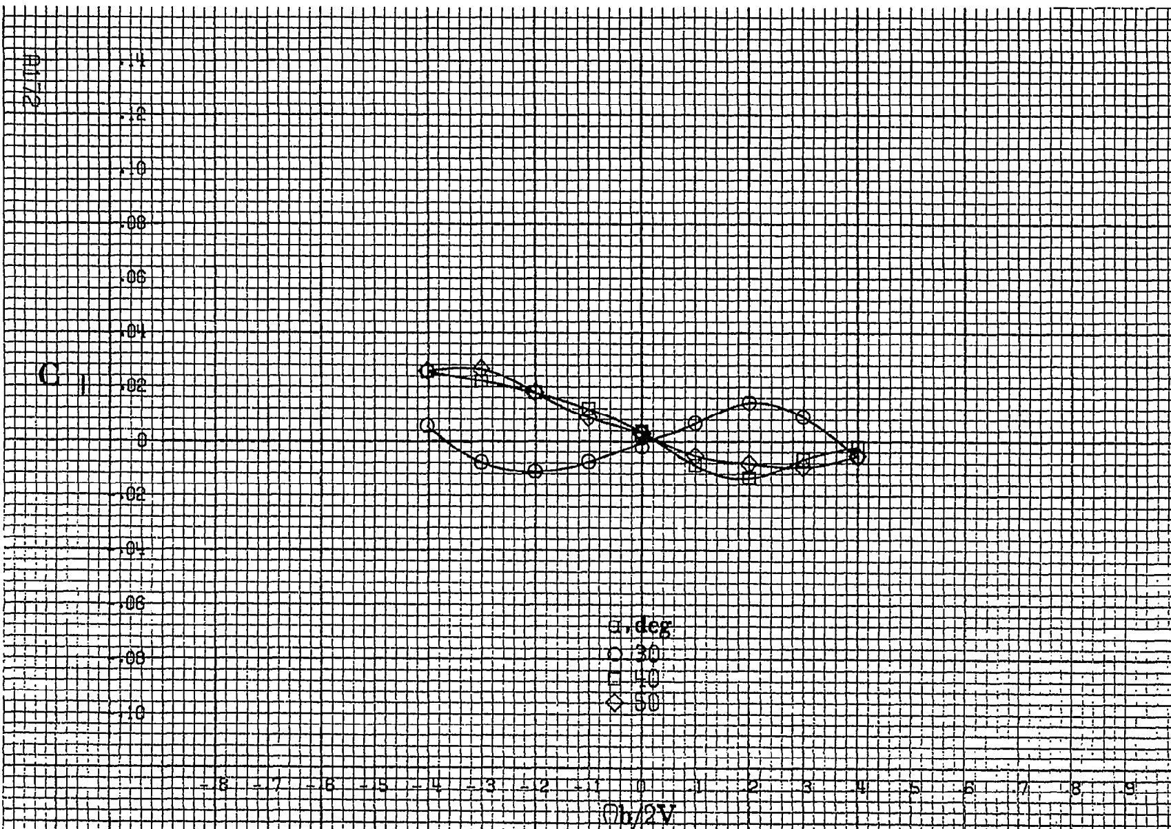
Figure A44. Effect of rotation rate and angle of attack on rolling-moment coefficient for basic configuration. \delta_2 = 25^\circ , \delta_3 = 0^\circ , \delta_4 = 0^\circ , \delta_5 = 0^\circ , \delta_6 = 0^\circ .
