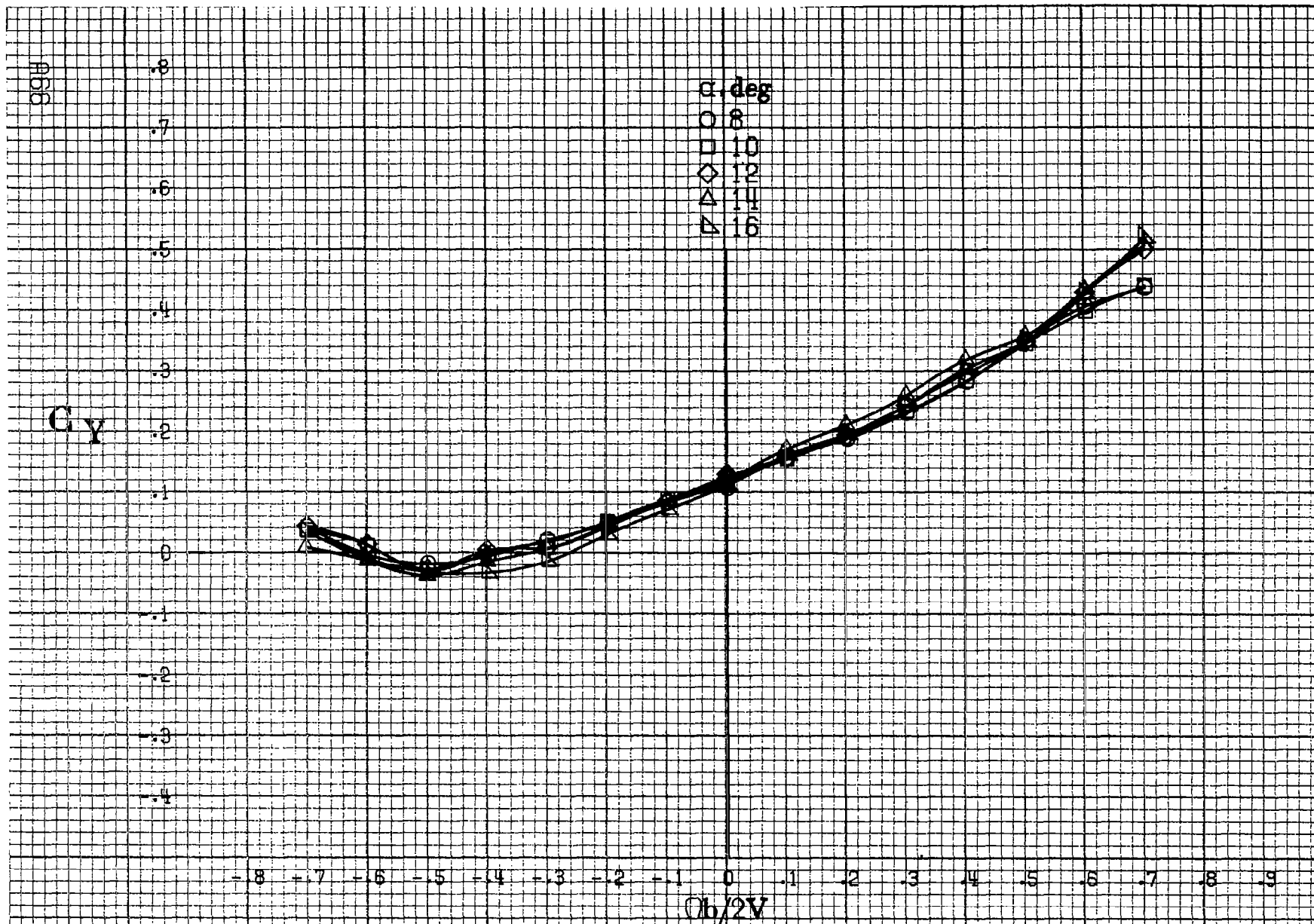
Figure A17 - Effect of rotation rate and angle of attack on side-force coefficient for body wing vertical tail configuration \delta_e = 0^\circ , \delta_a = 0^\circ , \delta_r = 0^\circ , \delta = 0^\circ .
