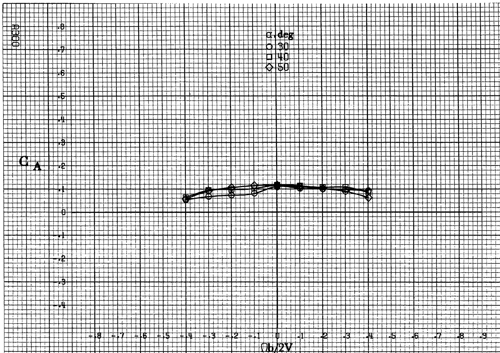
Figure A 84 - Effect of rotation rate and angle of attack on axial-force coefficient for basic configuration. \delta_c = 0^\circ , \delta_a = 20.0^\circ , \delta_d = 6^\circ , \delta_r = 0^\circ , \beta = 0^\circ .
