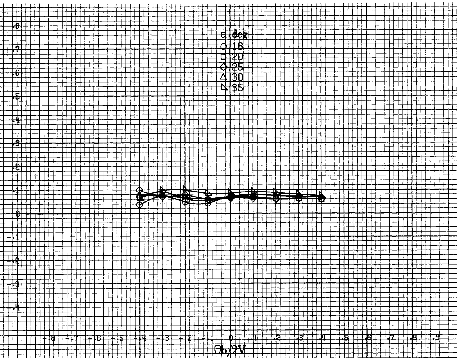
(b) \alpha = 18 to 35 deg. SR = 182.9 cm (72 in). Figure A 80.-Continued.
