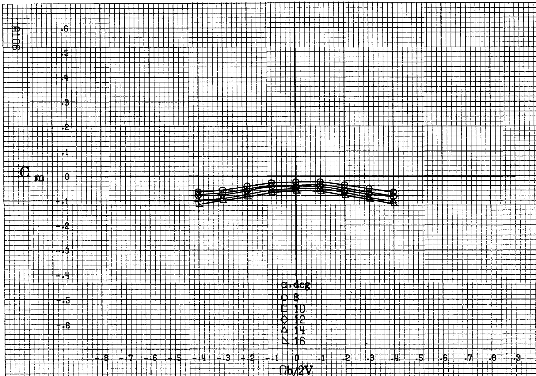
Figure A27.- Effect of rotation rate and angle of attack on pitching-moment coefficient for basic configuration. \delta_e = 0^\circ , \delta_a = 0^\circ , \delta_d = 0^\circ , \delta_r = 0^\circ , B = 0^\circ .
