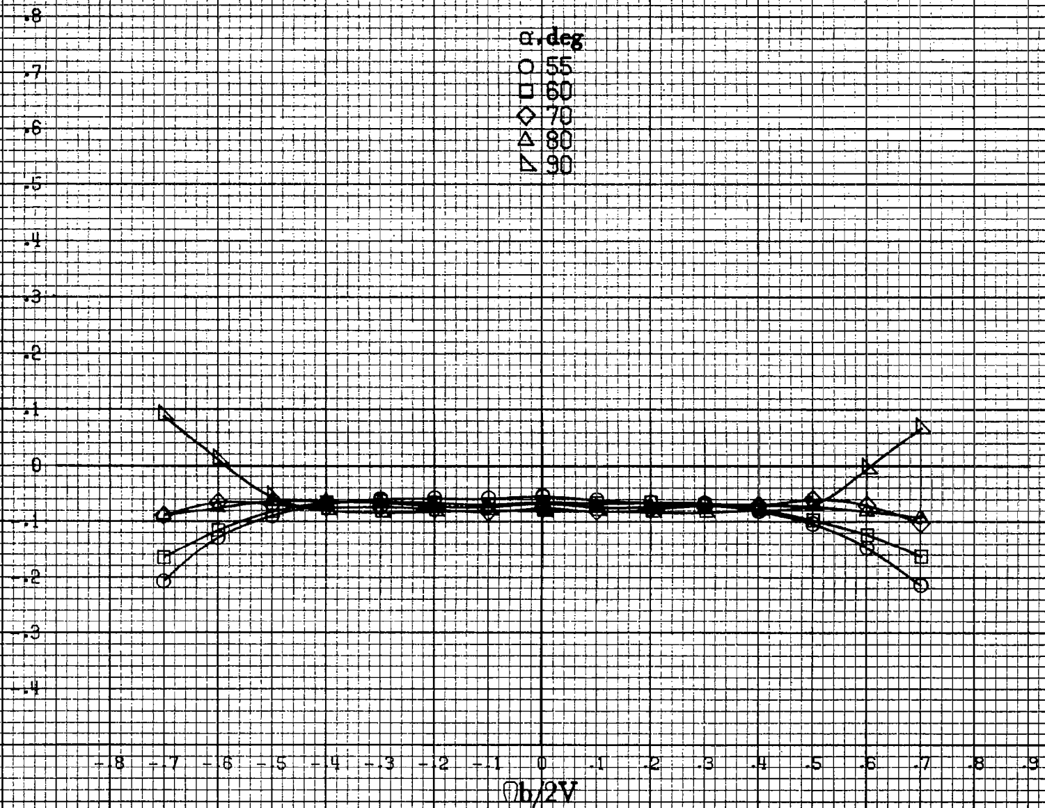
(d) \alpha = 55 to 90 deg, SR = 0 . Figure A6.-Concluded.
