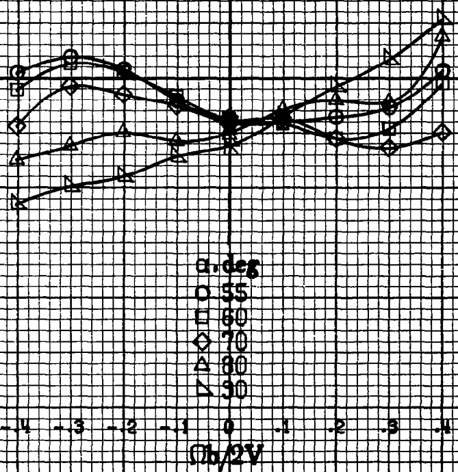
(b) \alpha = 55 to 90 deg, SR = 0 . Figure A104.-Concluded.
