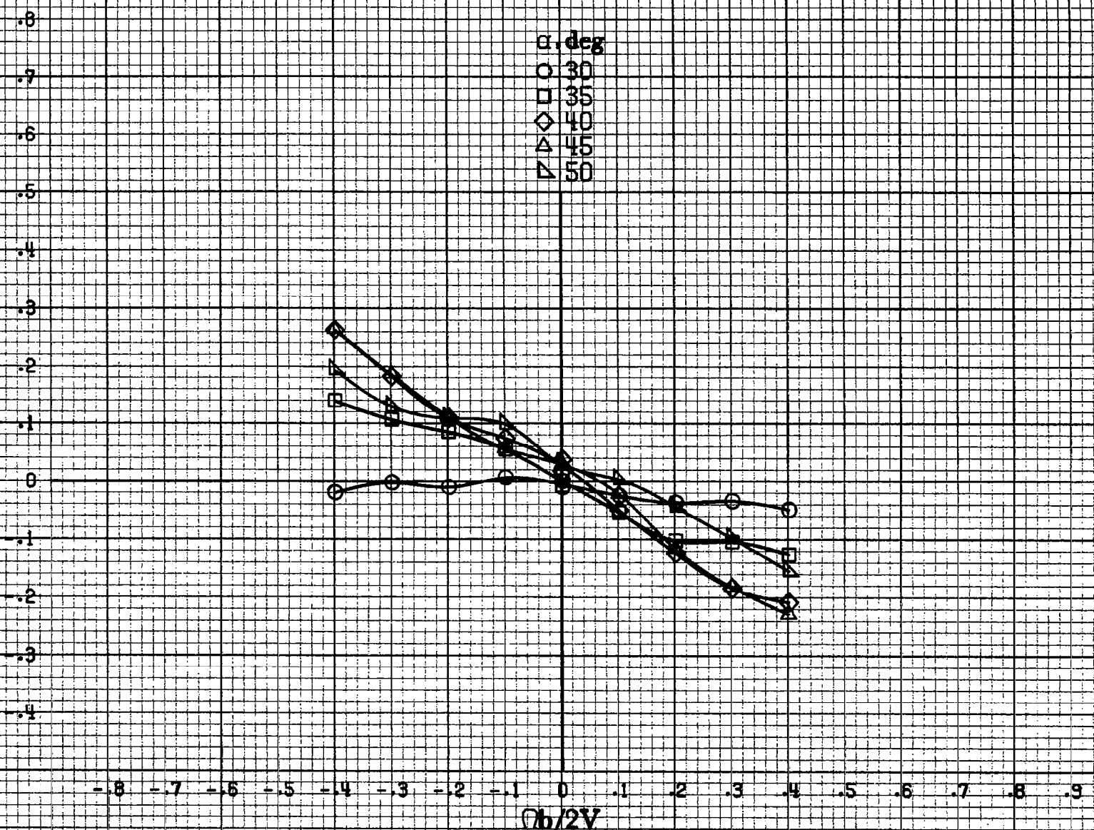
(c) \alpha=30 to 50 deg, SR=0 . Figure A 65.-Continued.
