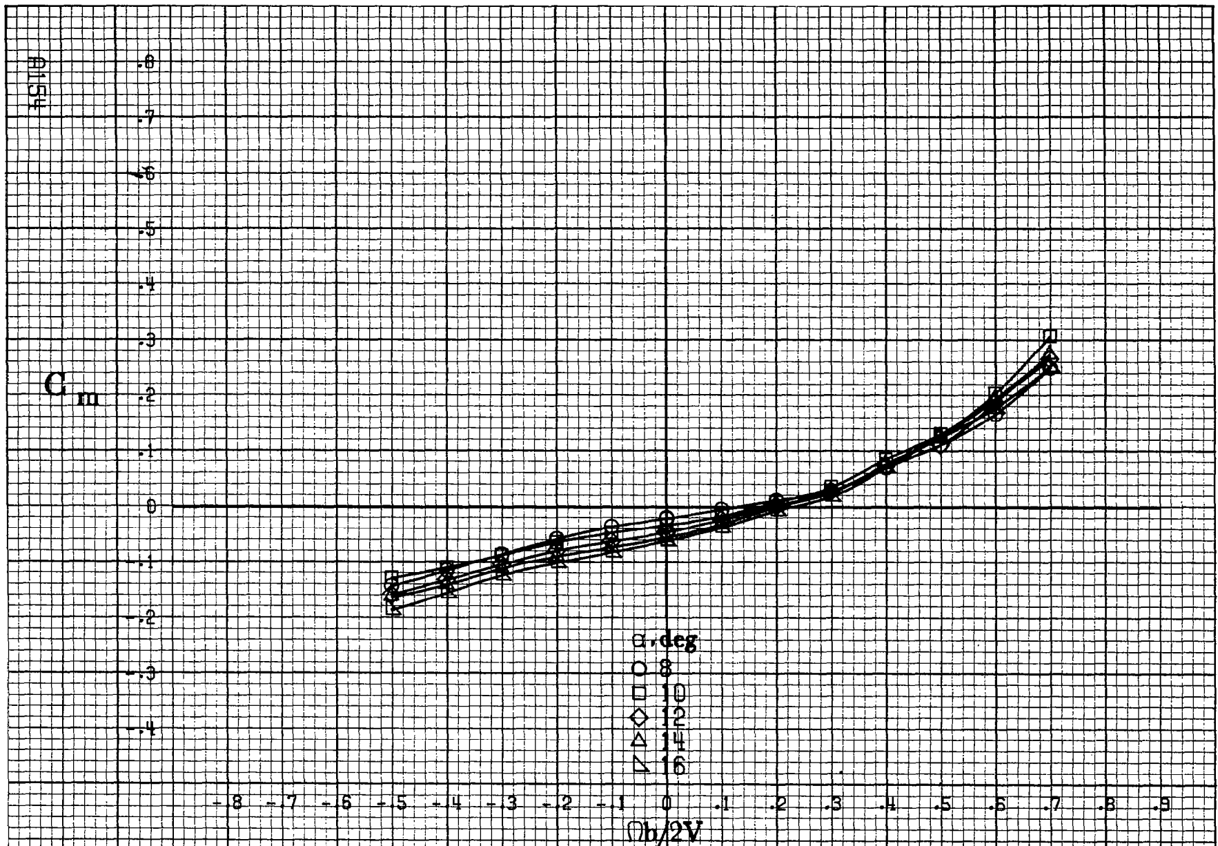
(a) \alpha = 8 to 16 deg, SR = 182.9 cm (72 in). Figure A39. - Effect of rotation rate and angle of attack on pitching-moment coefficient for basic configuration. \delta_c = 0^\circ , \delta_a = 0^\circ , \delta_d = 0^\circ , \delta_e = 0^\circ , \beta = 10^\circ .
