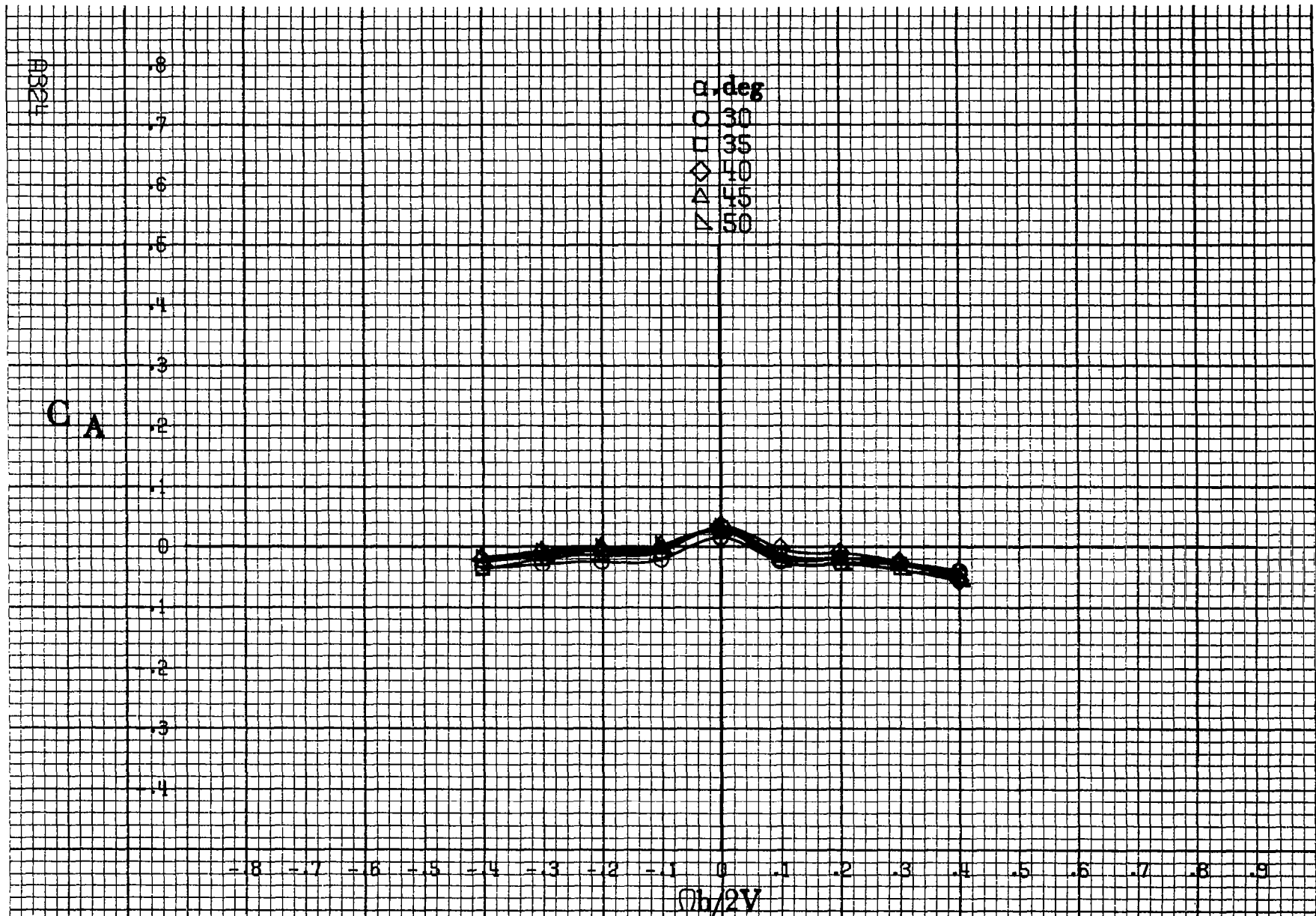
Figure A96 - Effect of rotation rate and angle of attack on axial-force coefficient for basic configuration. \delta_e = 0^\circ , \delta_s = 20.0^\circ , \delta_d = 6^\circ , \delta_r = -15^\circ , \beta = 0^\circ .
