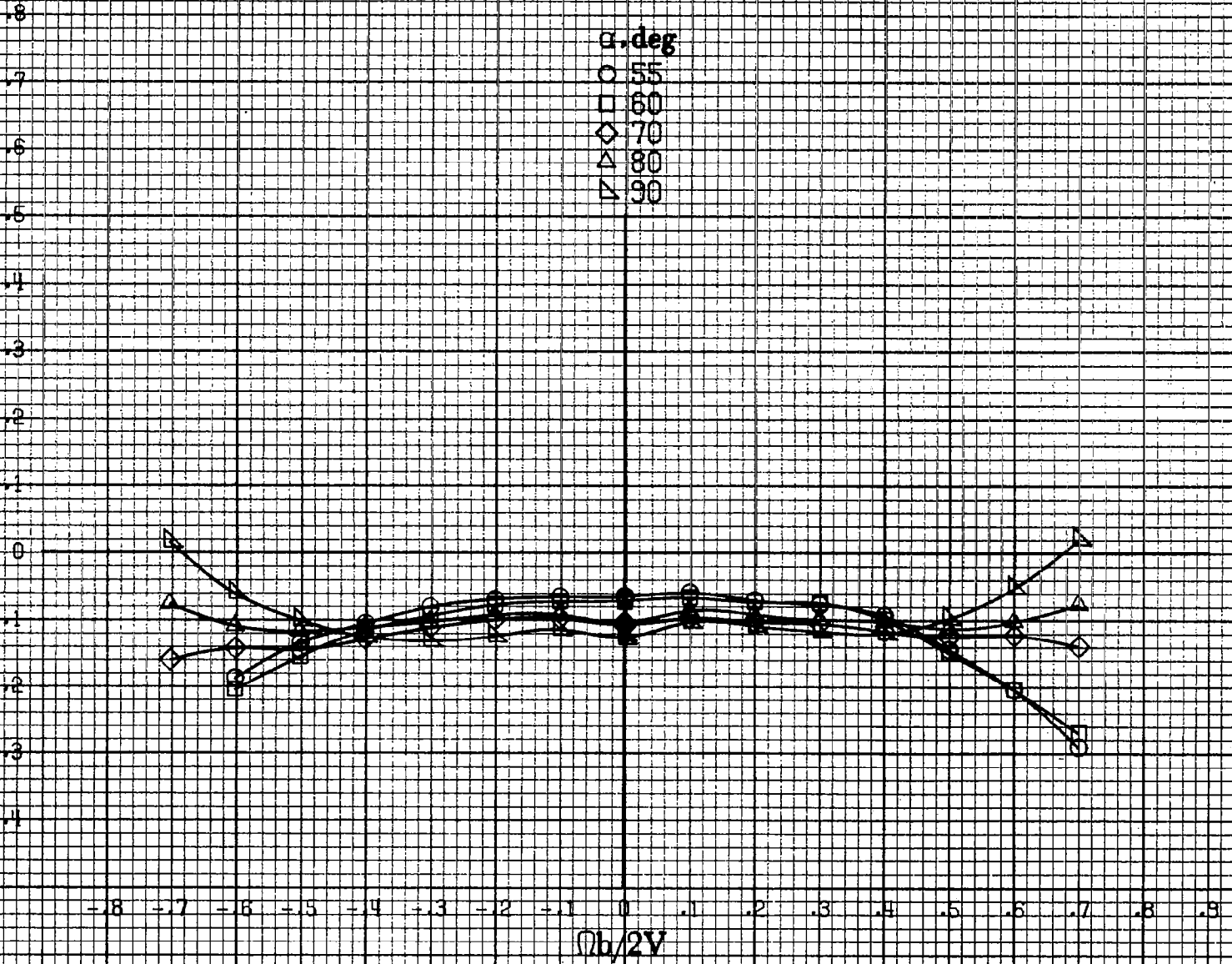
(d) \alpha = 55 to 90 deg, SR = 0 . Figure A 42.-Concluded.
