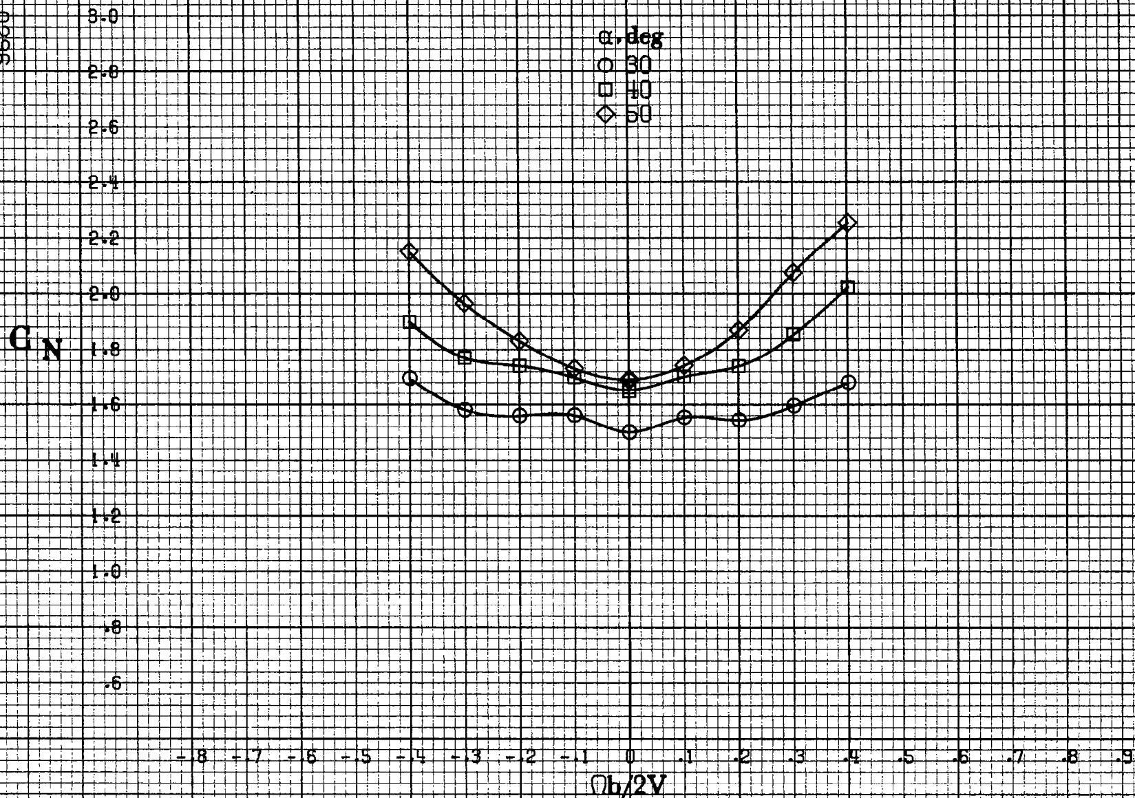
Figure A82.-Effect of rotation rate and angle of attack on normal-force coefficient for basic configuration. \delta_e = 0^\circ , \delta_s = 20.0^\circ , \delta_d = 6^\circ , \delta_r = 0^\circ , \beta = 0^\circ .
