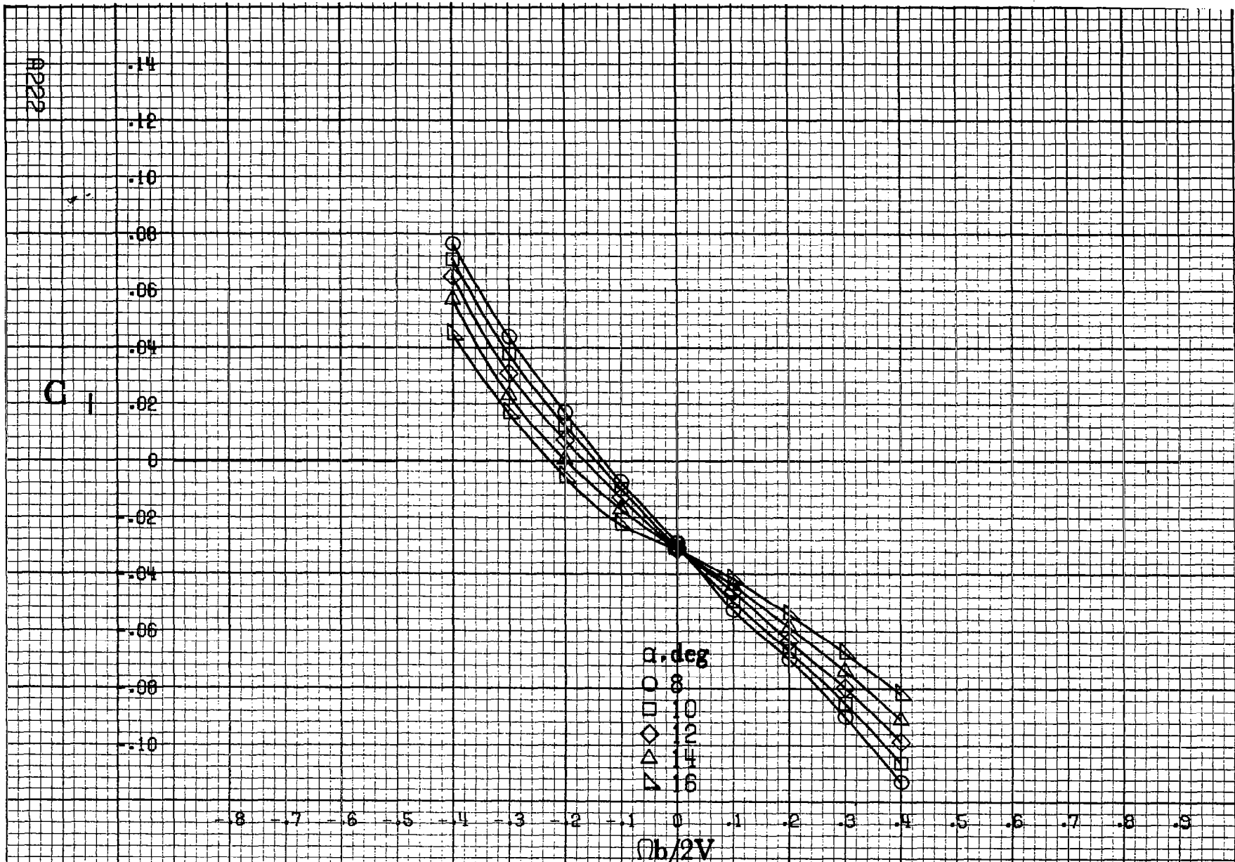
(a) \alpha=8 to 16 deg, SR=182.9 cm (72 in). Figure A 62.- Effect of rotation rate and angle of attack on rolling-moment coefficient for basic configuration. \delta_e=0^\circ , \delta_a=0^\circ , \delta_a=6^\circ , \delta_r=0^\circ . \theta=10^\circ .
