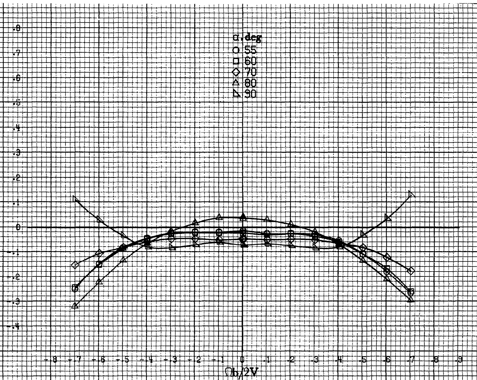
(d) \alpha = 55 to 90 deg, SR = 0 . Figure A18.-Concluded.
