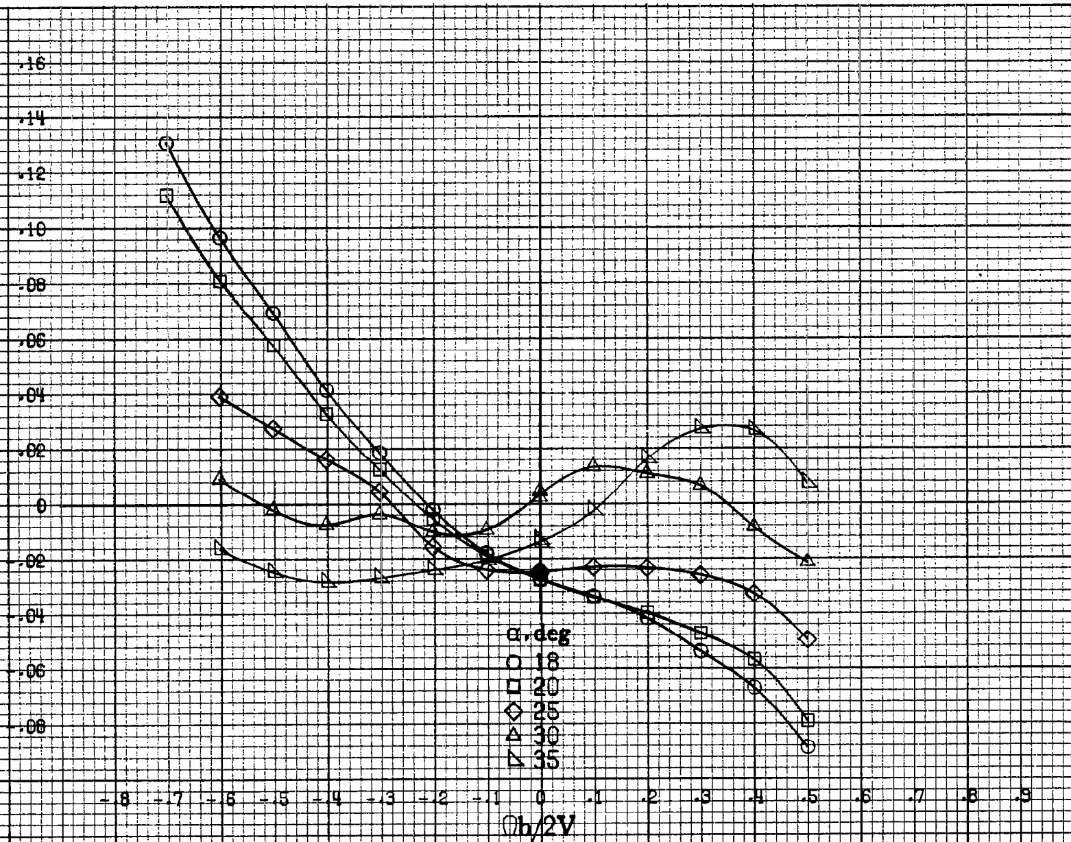
(b) \alpha = 18 to 35 deg, SR = 182.9 cm (72 in). Figure A32.-Continued.
