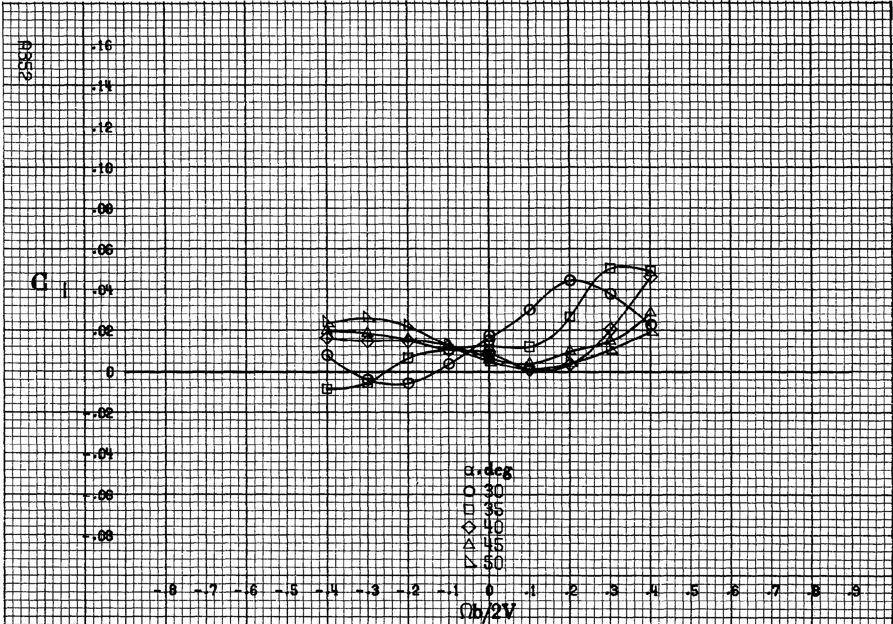
Figure A110.-Effect of rotation rate and angle of attack on rolling-moment coefficient for basic configuration. \delta_1 = 0^\circ , \delta_2 = -20.0^\circ , \delta_3 = -6^\circ , \delta_4 = 30^\circ , \beta = 10^\circ
