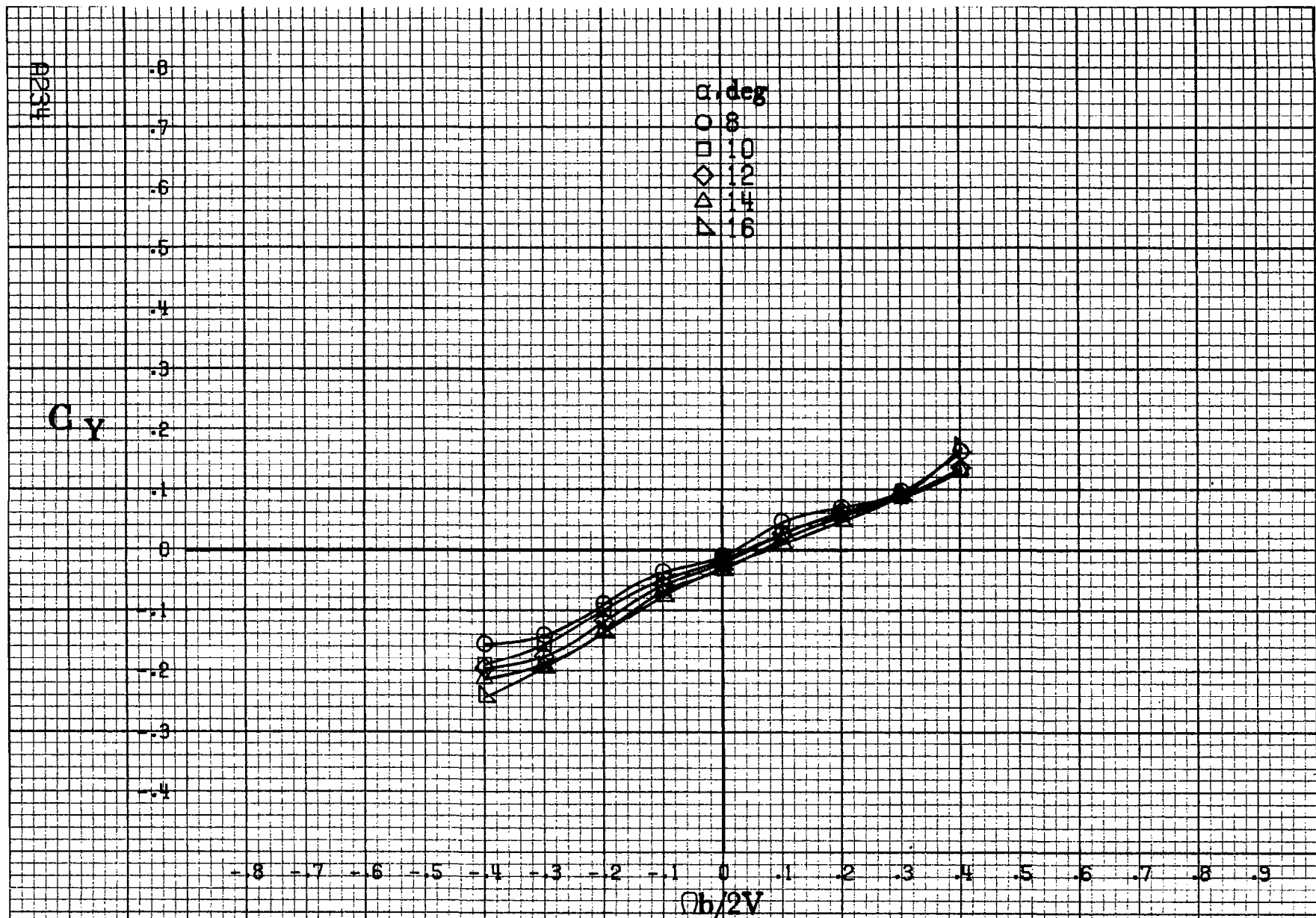
Figure A65.- Effect of rotation rate and angle of attack on side-force coefficient for basic configuration. \delta_c = 0^\circ , \delta_a = 0^\circ , \delta_d = 6^\circ , \delta_r = 0^\circ , \beta = 10^\circ .
