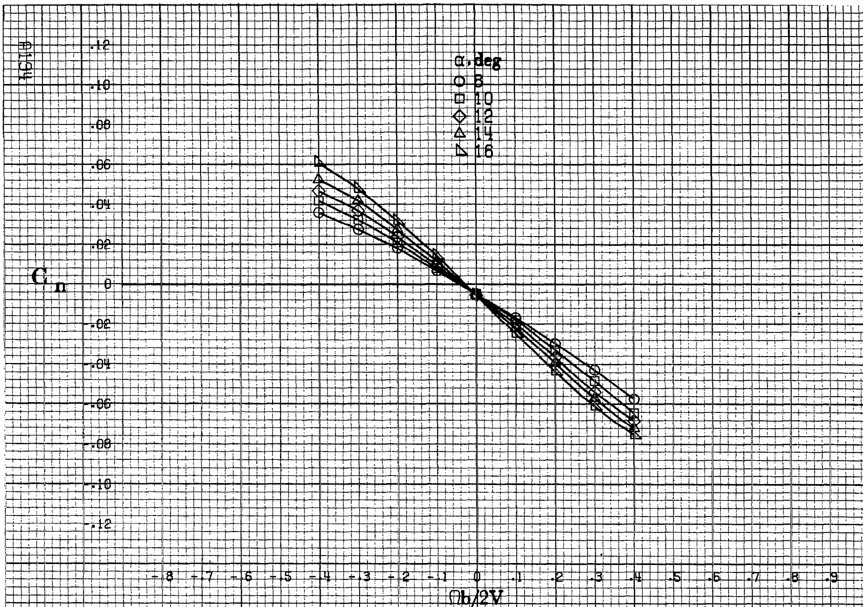
Figure A55 - Effect of rotation rate and angle of attack on yawing-moment coefficient for basic configuration. \delta_e = 0^\circ , \delta_a = 0^\circ , \delta_d = 6^\circ , \delta_r = 0^\circ , \beta = 0^\circ .
