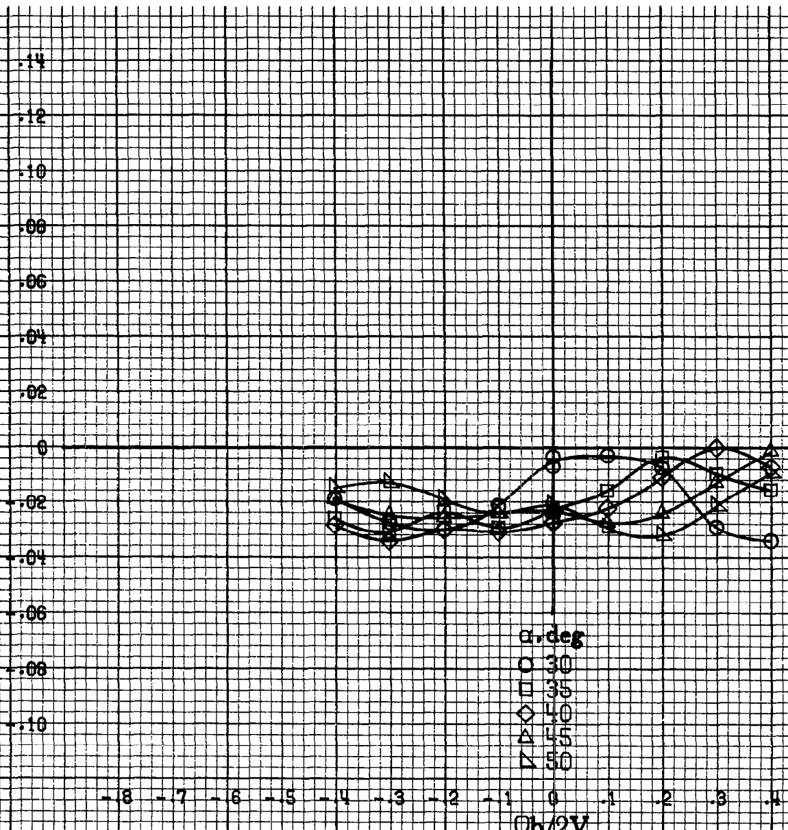
Figure A98.-Effect of rotation rate and angle of attack on rolling-moment coefficient for basic configuration. \delta_e = 0^\circ , \delta_s = 20.0^\circ , \delta_a = 6^\circ , \delta_r = -15^\circ , \beta = 10^\circ .
