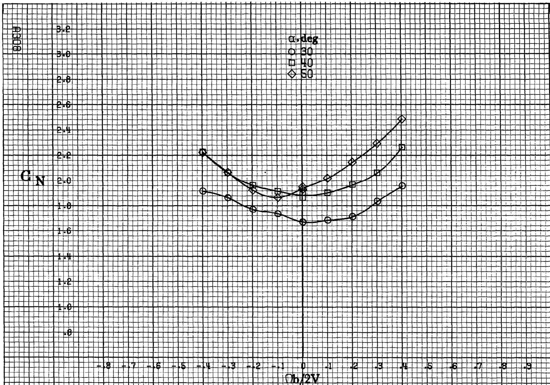
Figure A88 - Effect of rotation rate and angle of attack on normal-force coefficient for basic configuration. \delta_c = 0^\circ , \delta_a = 20.0^\circ , \delta_d = 6^\circ , \delta_r = 0^\circ , \beta = 10^\circ .
