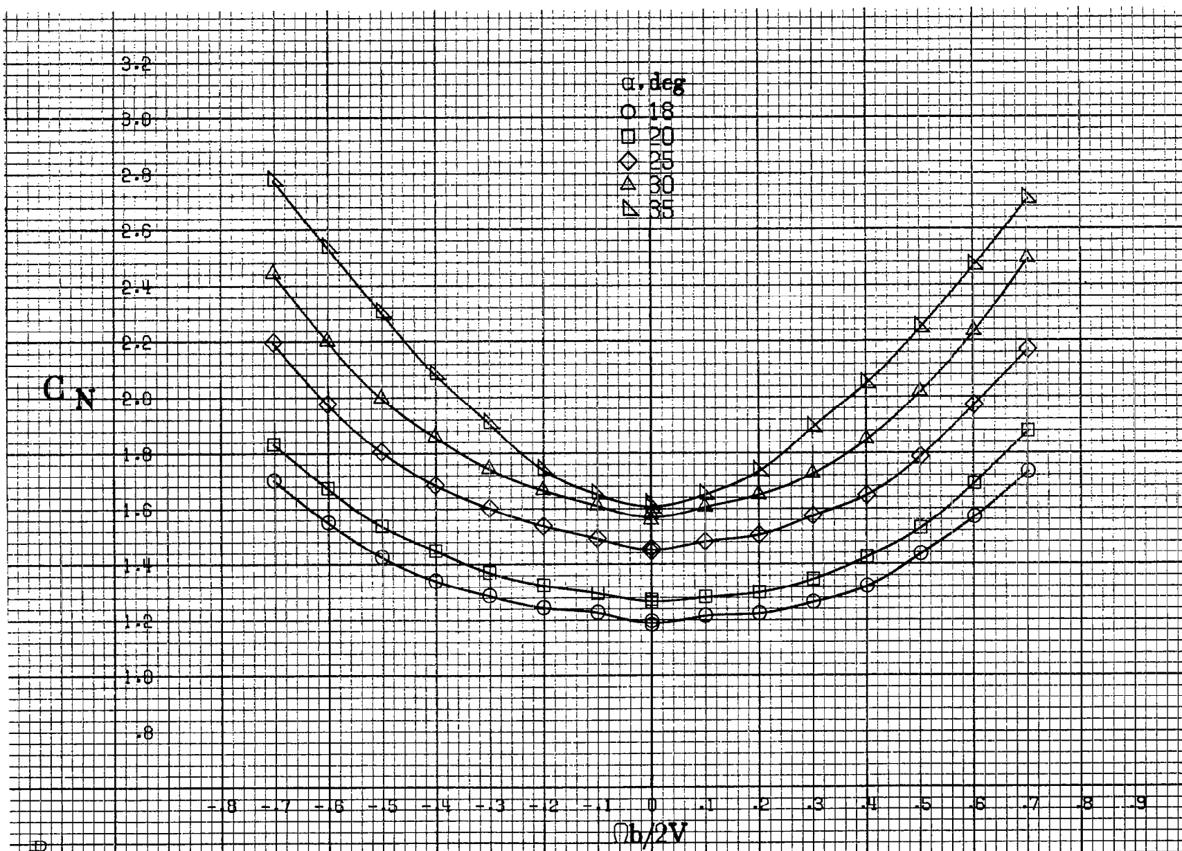
(h) \alpha=18 to 35 deg. SR = 182.9 cm (72 in). Figure A10.-Continued.
