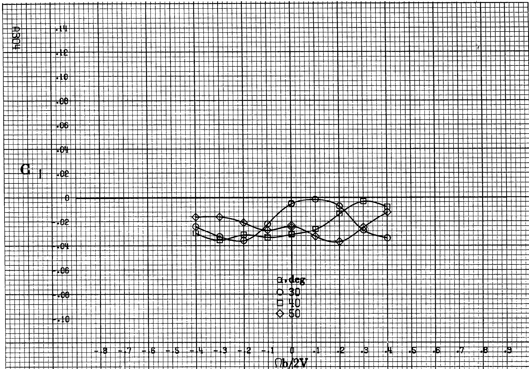
Figure A 86.- Effect of rotation rate and angle of attack on rolling-moment coefficient for basic configuration. \delta_e = 0^\circ , \delta_a = 20.0^\circ , \delta_{\dot{a}} = 6^\circ , \delta_r = 0^\circ , \beta = 10^\circ .
