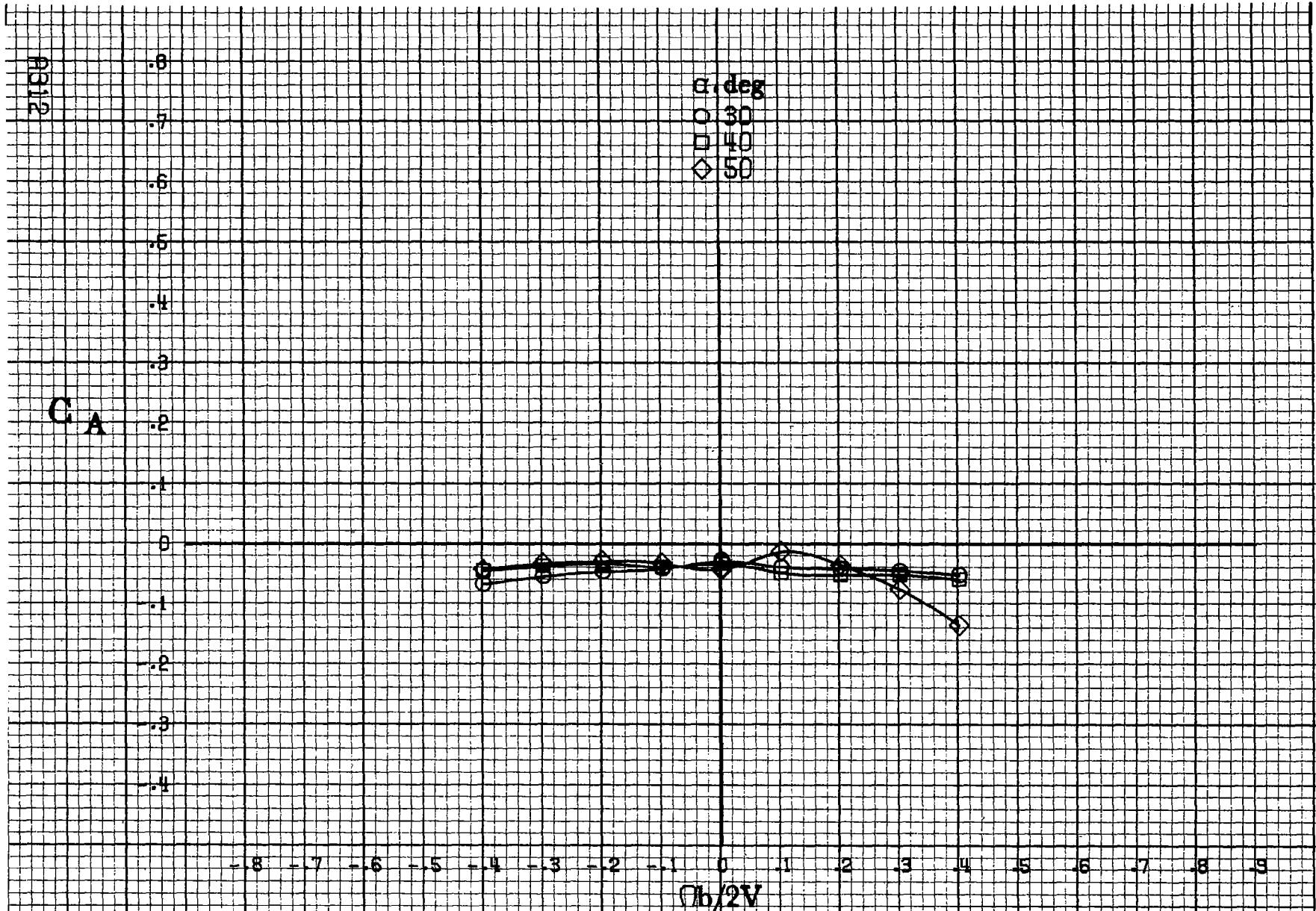
Figure A90.-Effect of rotation rate and angle of attack on axial-force coefficient for basic configuration. \delta_e = 0^\circ , \delta_a = 20.0^\circ , \delta_a = 6^\circ , \delta_r = 0^\circ , \beta = 10^\circ .
