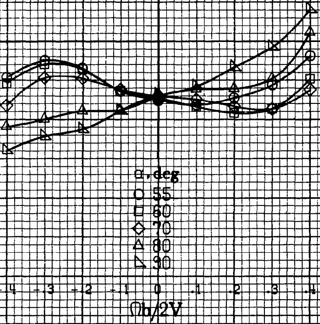
(b) \alpha=55 to 90 deg, SR=0 . Figure A85.-Concluded.
