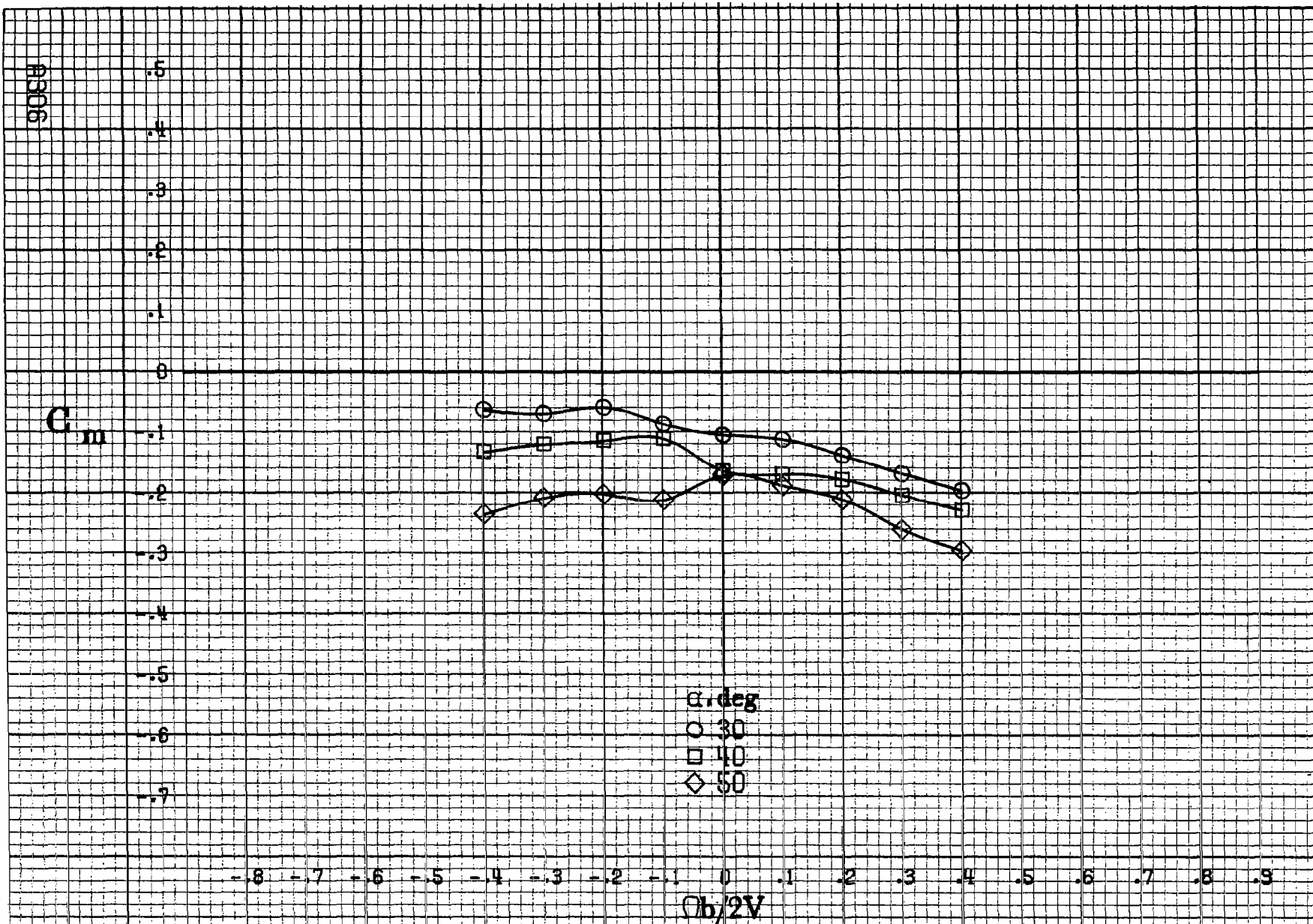
Figure A87.-Effect of rotation rate and angle of attack on pitching-moment coefficient for basic configuration. \delta_a = 0^\circ , \delta_s = 20.0^\circ , \delta_d = 6^\circ , \delta_r = 0^\circ , \beta = 10^\circ .
