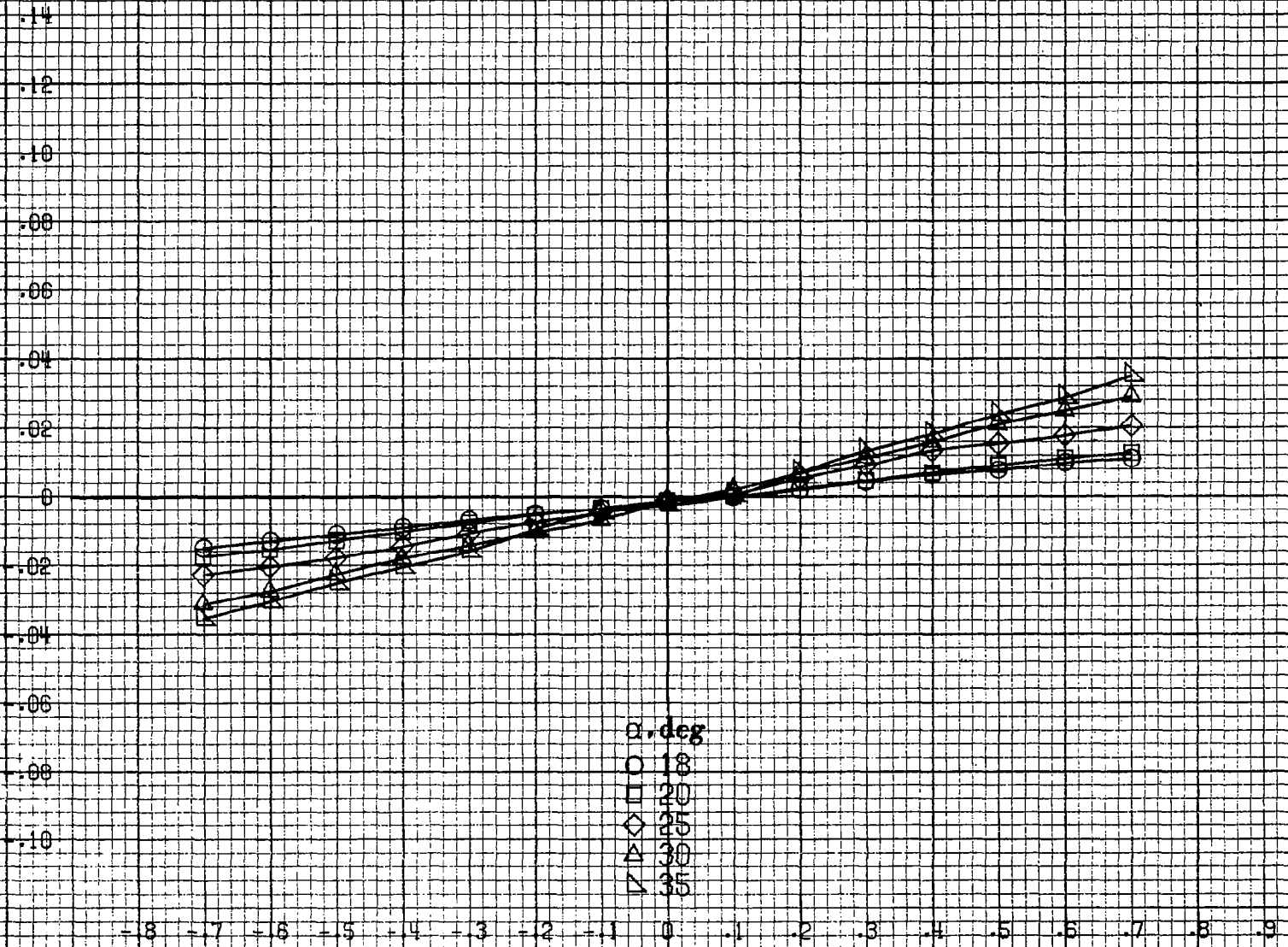
(b) \alpha = 18 to 35 deg, SR = 182.9 cm (72 in). Figure A2. - Continued.
