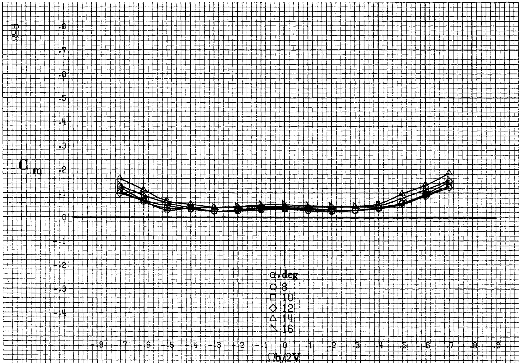
Figure A15.-Effect of rotation rate and angle of attack on pitching-moment coefficient for body wing vertical tail configuration \delta_e = 0^\circ , \delta_a = 0^\circ , \delta_r = 0^\circ , \delta = 0^\circ .
