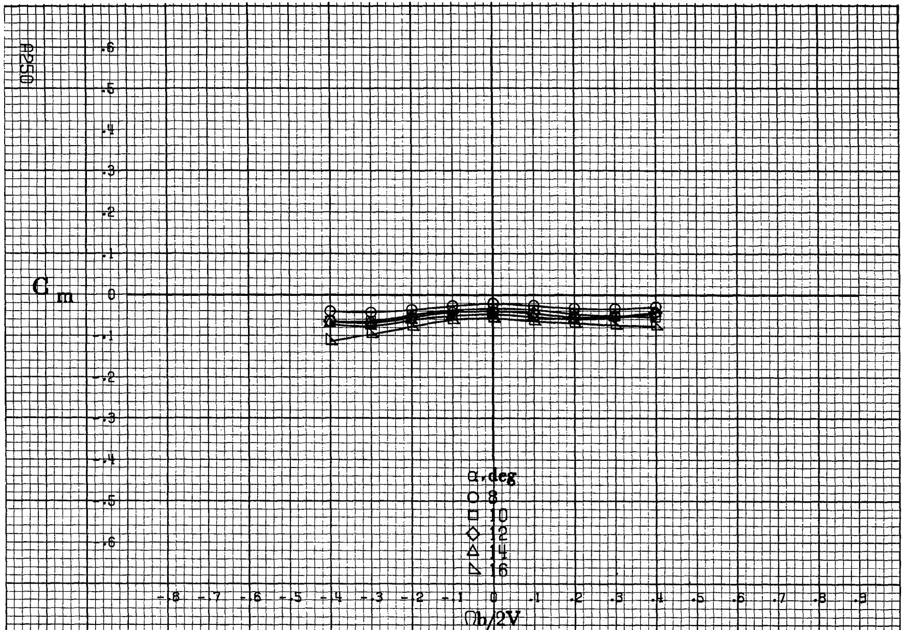
(a) \alpha = 8 to 16 deg, SR = 182.9 \text{ cm (72 in)} .
