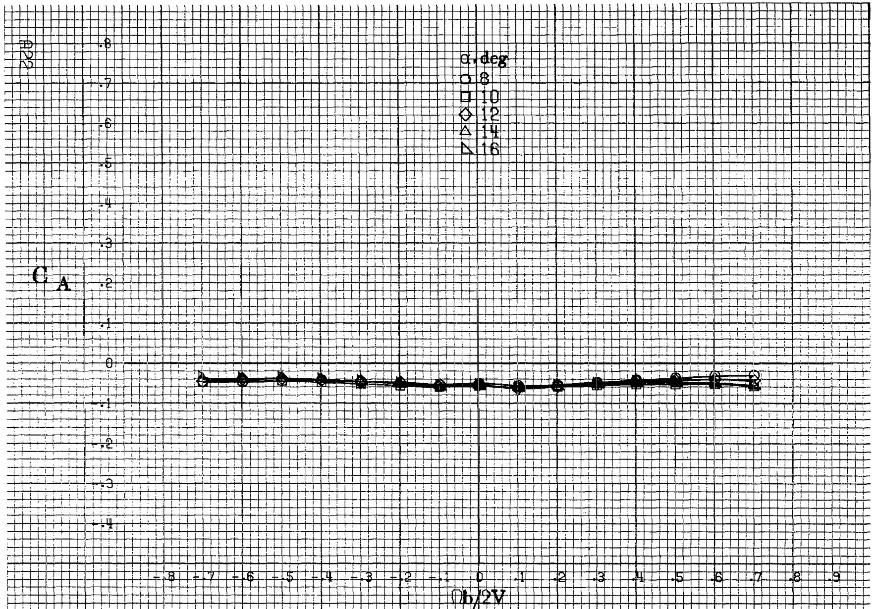
Figure A 6. Effect of rotation rate and angle of attack on axial force coefficient for body alone configuration. \delta_a = 0^\circ , \delta_s = 0^\circ , \delta_r = 0^\circ , \beta = 0^\circ .
