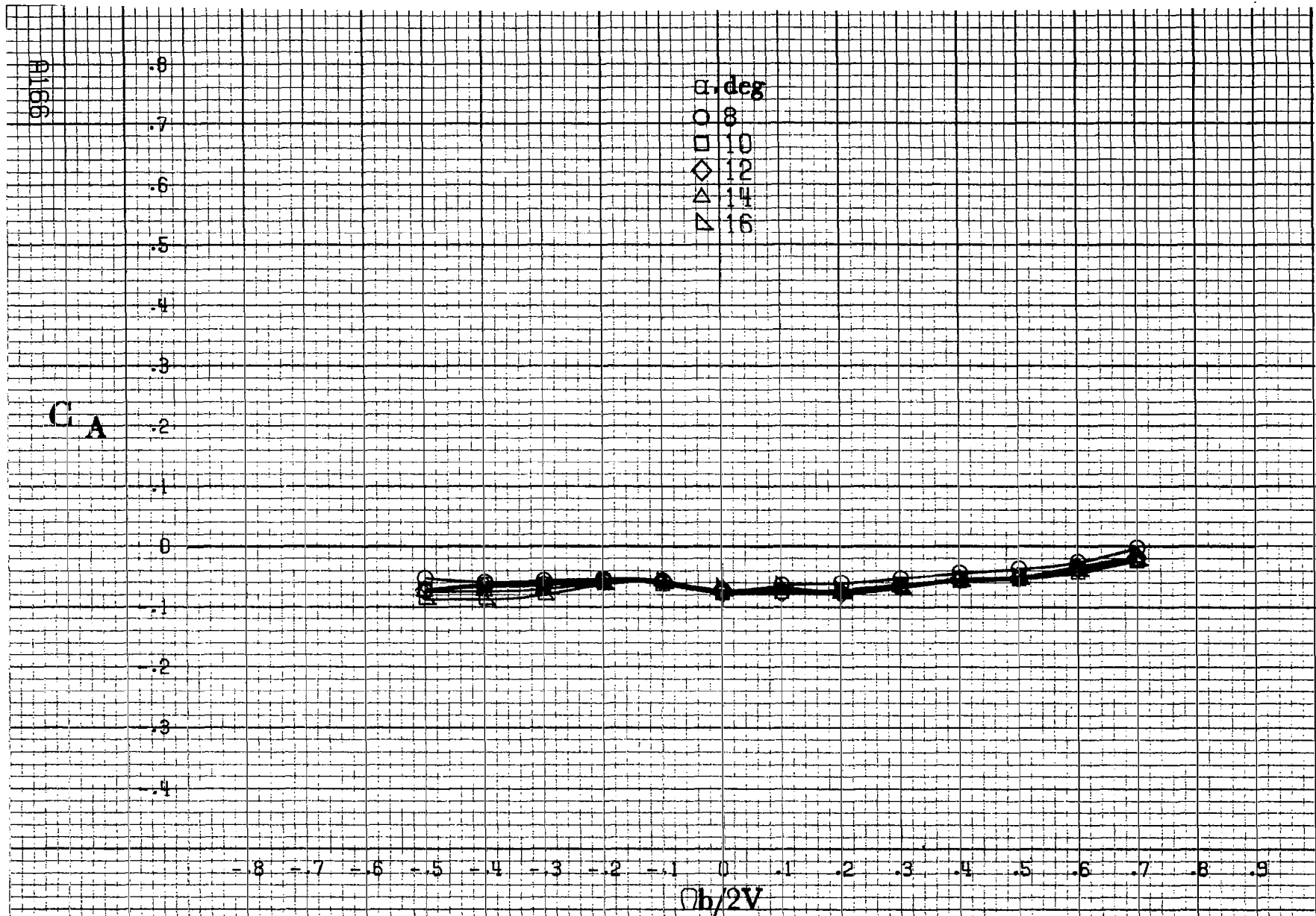
Figure A42.-Effect of rotation rate and angle of attack on axial force coefficient for basic configuration. \delta_e = 0^\circ , \delta_a = 0^\circ , \delta_a = 0^\circ , \delta_r = 0^\circ , \beta = -10^\circ .
