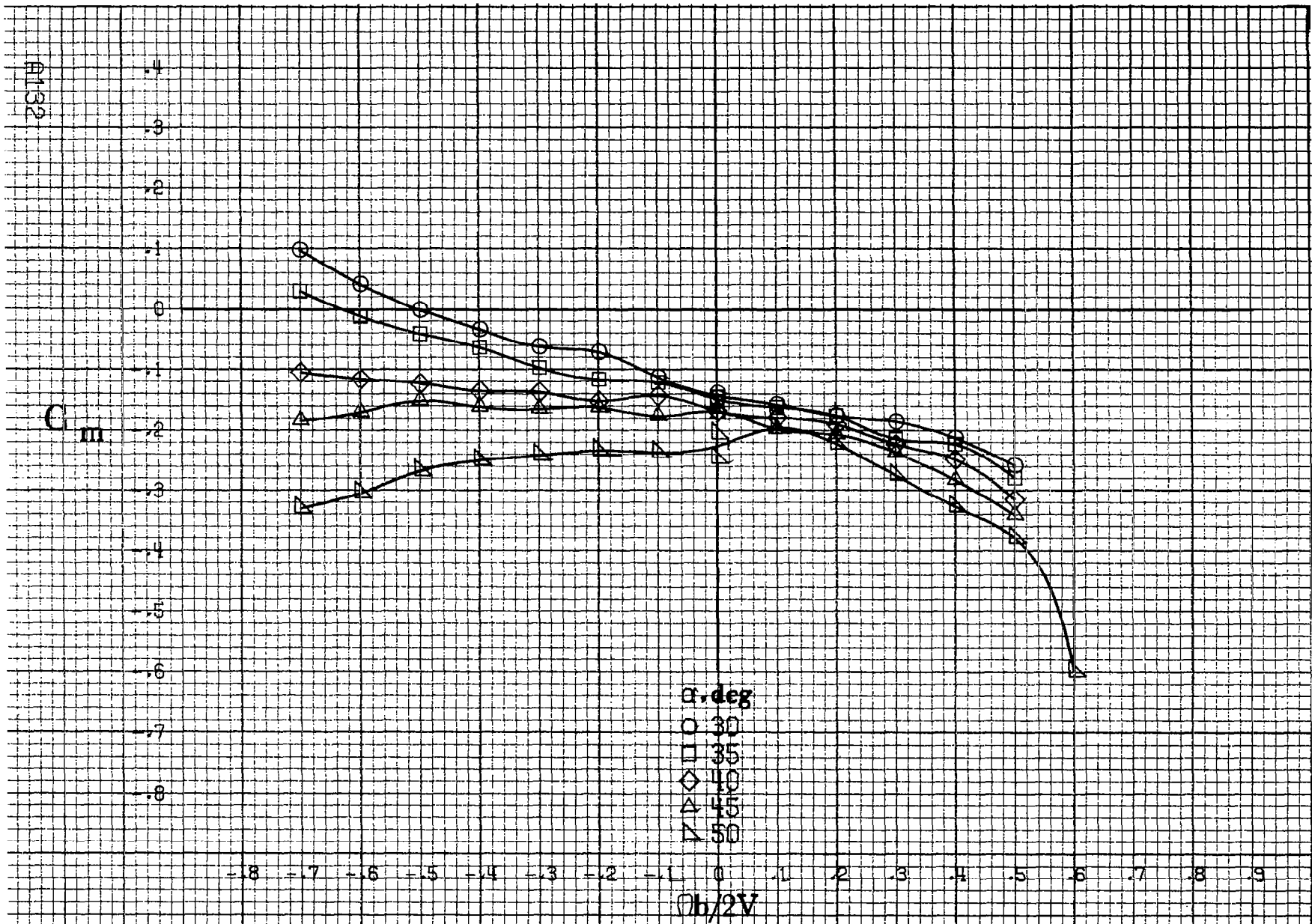
(c) \alpha = 30 to 50 deg, SR = 0 . Figure A 82 - Continued.
