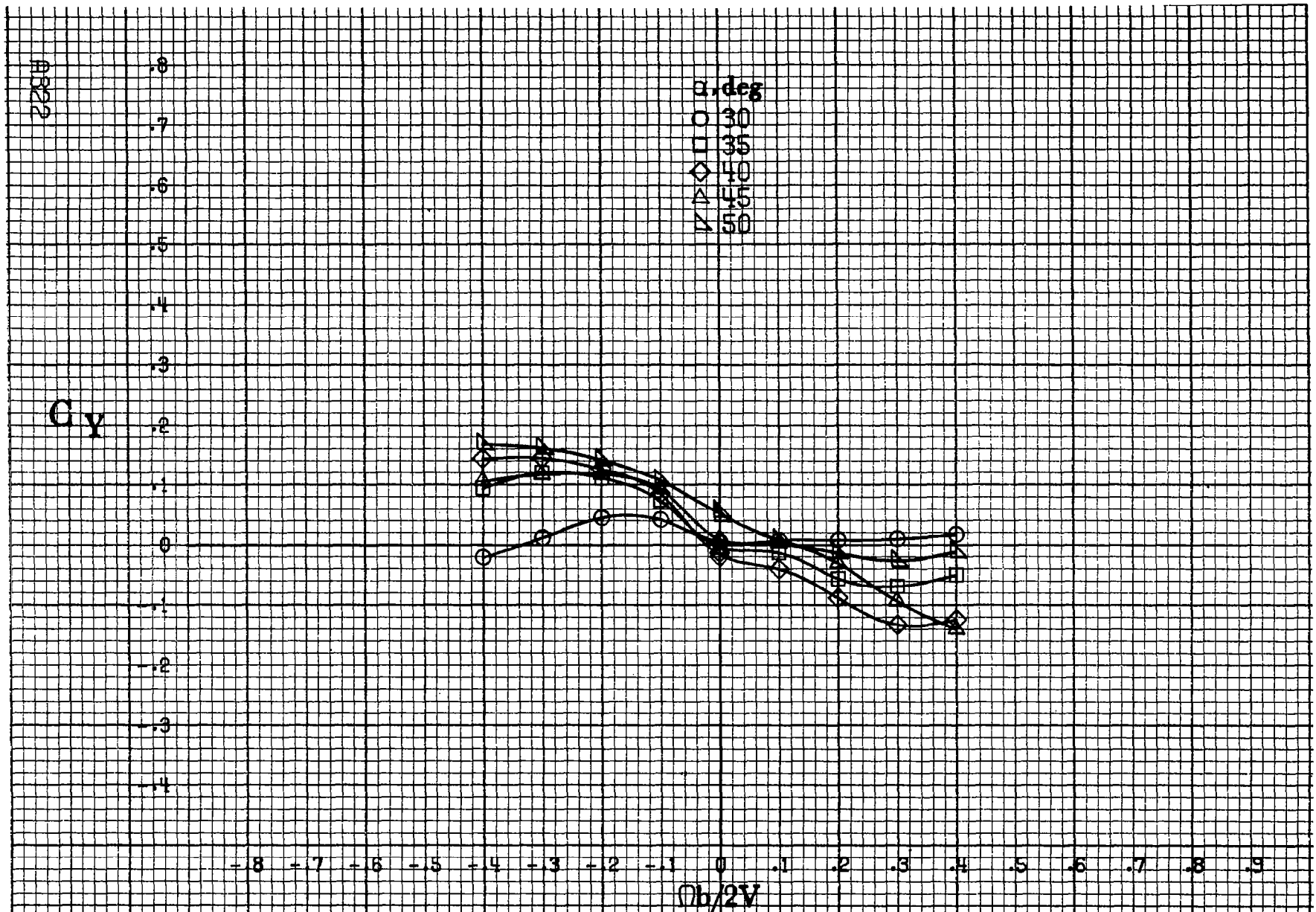
Figure A95 - Effect of rotation rate and angle of attack on side-force coefficient for basic configuration. \delta_c = 0^\circ , \delta_a = 20.0^\circ , \delta_d = 6^\circ , \delta_r = -15^\circ , \beta = 0^\circ .
