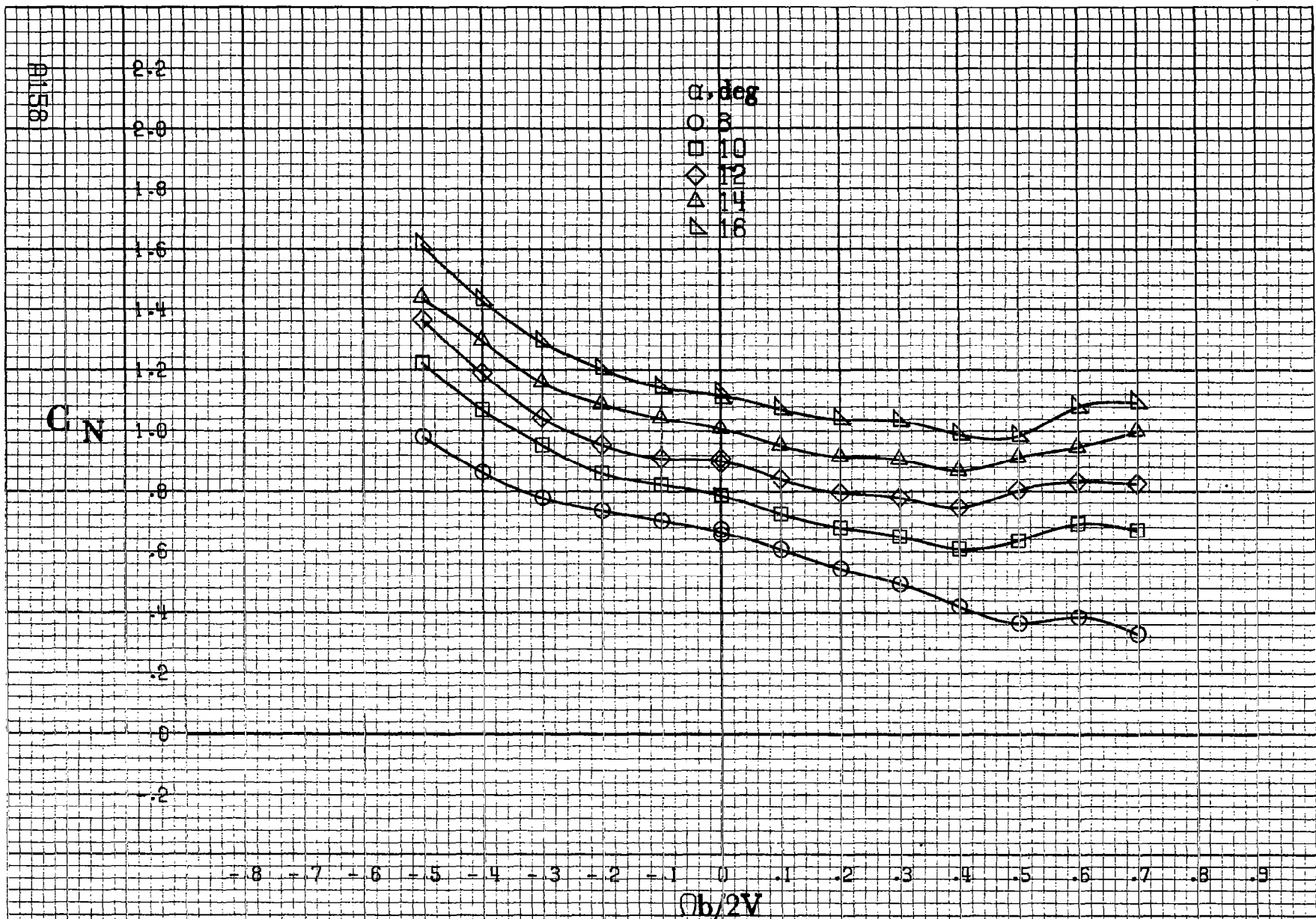
Figure A40.-Effect of rotation rate and angle of attack on normal-force coefficient for basic configuration. \delta_s = 0^\circ , \delta_a = 0^\circ , \delta_a = 0^\circ , \delta_r = 0^\circ , \beta = -10^\circ .
