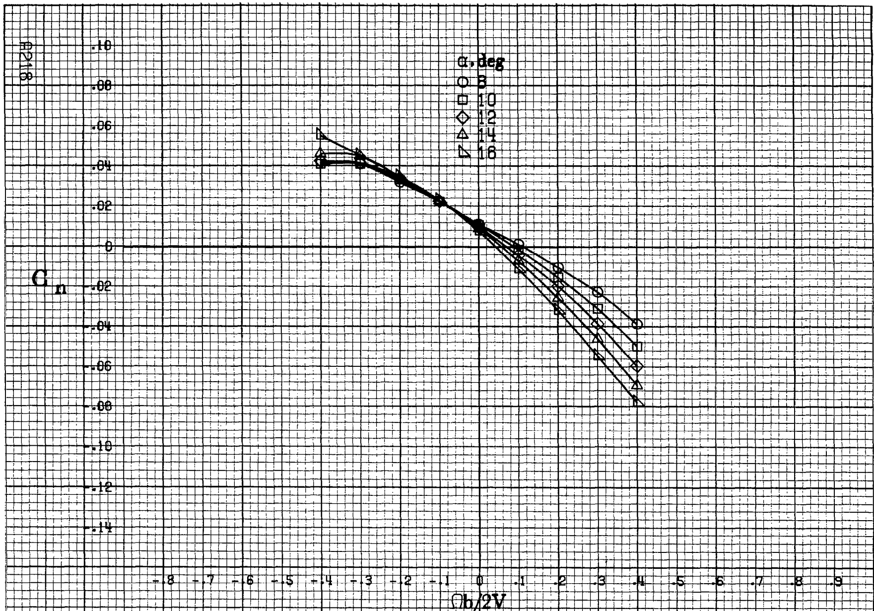
Figure A61.-Effect of rotation rate and angle of attack on yawing-moment coefficient for basic configuration. \delta_e=0^\circ , \delta_a=0^\circ , \delta_d=6^\circ , \delta_r=0^\circ , \beta=10^\circ .
