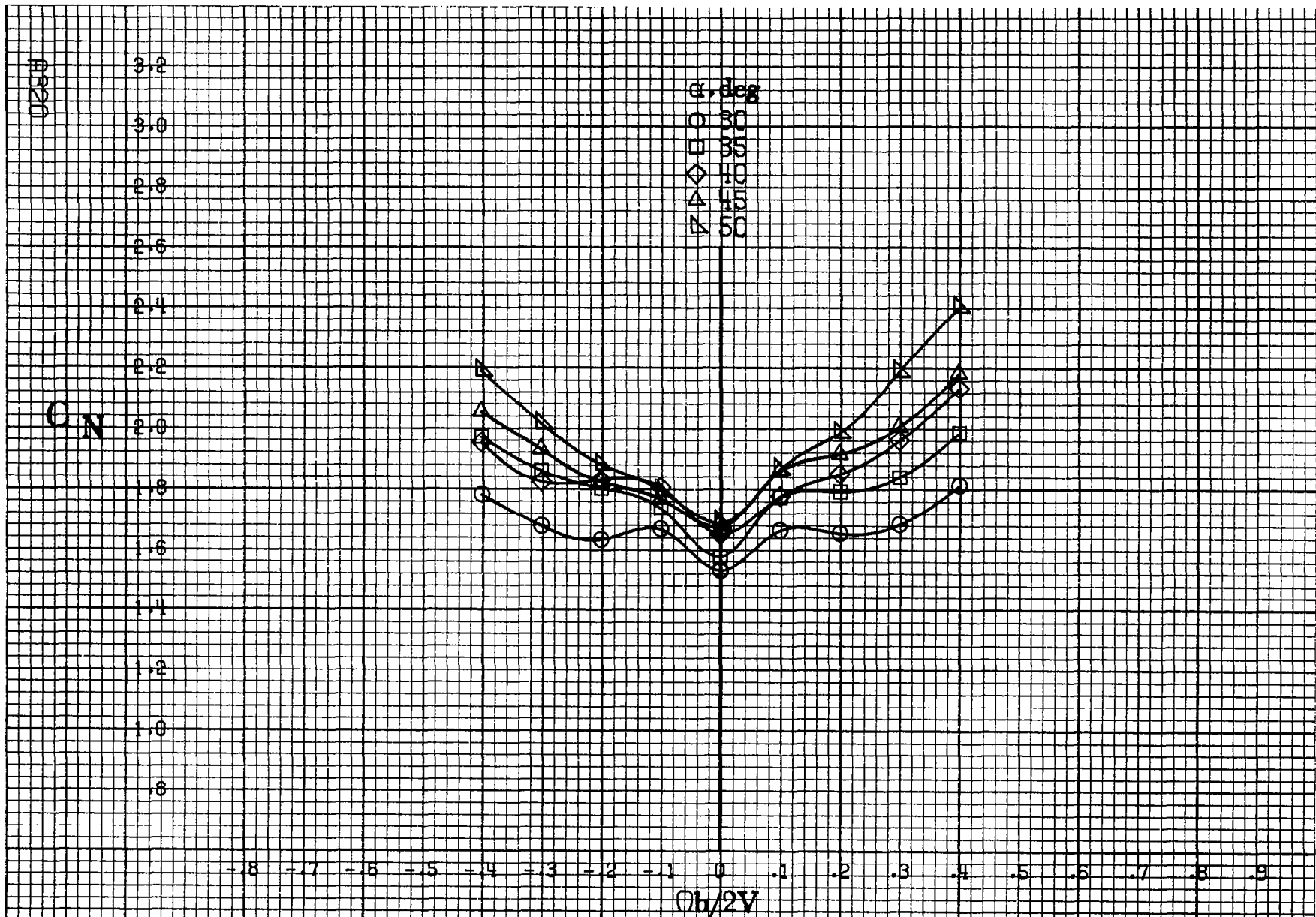
Figure A 94. Effect of rotation rate and angle of attack on normal-force coefficient for basic configuration. \delta_a = 0^\circ , \delta_s = 20.0^\circ , \delta_d = 6^\circ , \delta_r = -15^\circ , \beta = 0^\circ .
