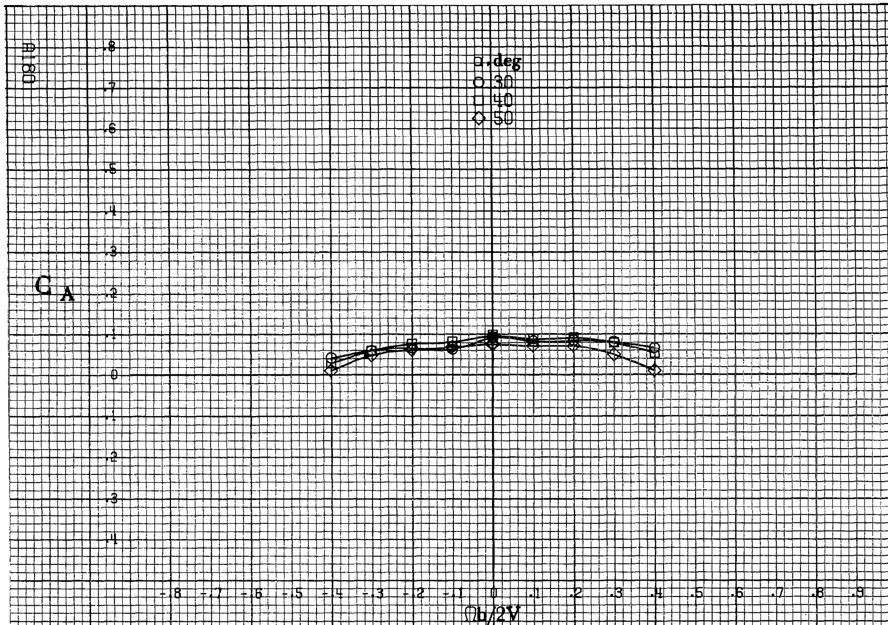
Figure A48.- Effect of rotation rate and angle of attack on axial-force coefficient for basic configuration. \delta_e = -25^\circ , \delta_a = 0^\circ , \delta_d = 0^\circ , \delta_r = 0^\circ . B = 0^\circ .
