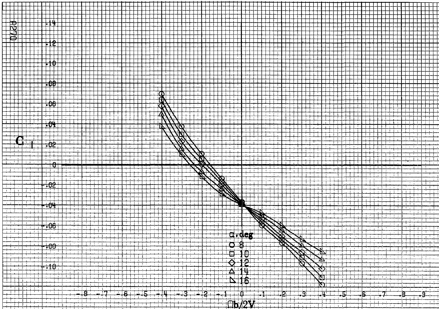
Figure A74.- Effect of rotation rate and angle of attack on rolling-moment coefficient for basic configuration. \delta_e = 0^\circ , \delta_a = 0^\circ , \delta_d = 11^\circ , \delta_r = 0^\circ , \beta = 10^\circ .
