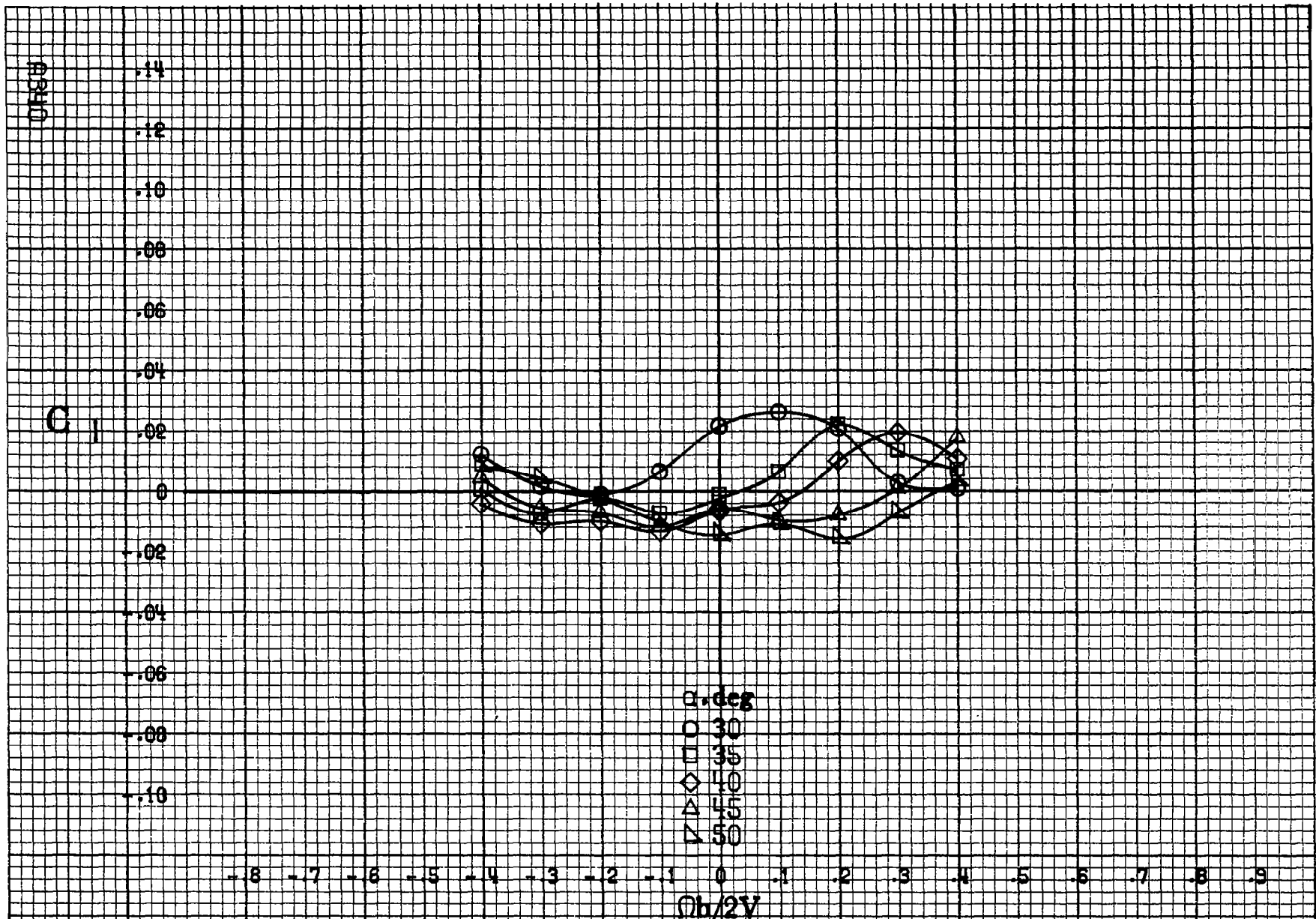
Figure A104.-Effect of rotation rate and angle of attack on rolling-moment coefficient for basic configuration. \delta_e = 0^\circ , \delta_a = -20.0^\circ , \delta_{\dot{a}} = -6^\circ , \delta_r = 30^\circ , \delta = 0^\circ .
