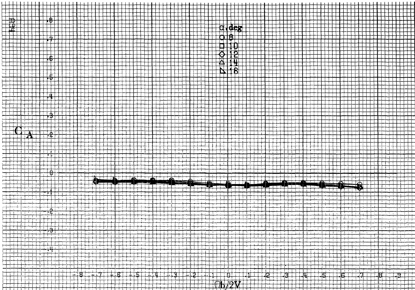
Figure A24. Effect of rotation rate and angle of attack on axial-force coefficient for body wing horizontal tail configuration \delta_a = 0^\circ , \delta_r = 0^\circ , \delta_T = 0^\circ , \beta = 0^\circ .
