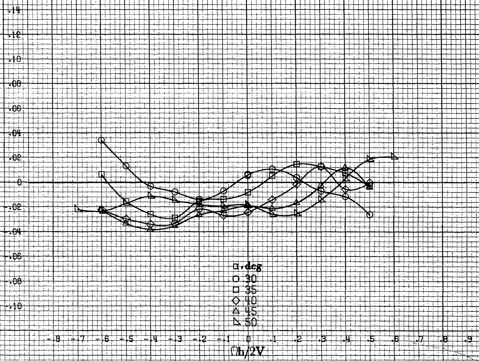
(c) \alpha = 30 to 50 deg, SR = 0 . Figure A 82.-Continued.
