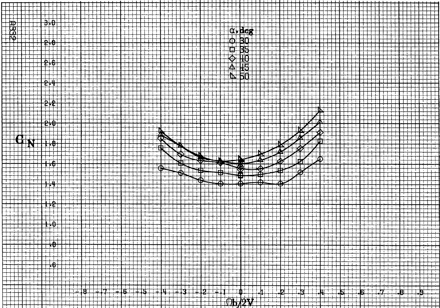
Figure A100.-Effect of rotation rate and angle of attack on normal-force coefficient for basic configuration. \delta_c = 0^\circ , \delta_s = 20.0^\circ , \delta_d = 8^\circ , \delta_r = -15^\circ , B = 10^\circ .
