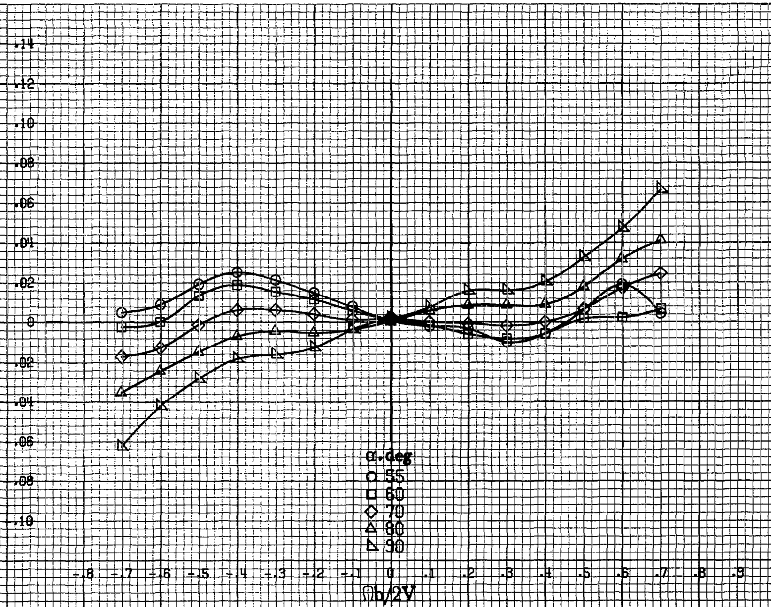
(d) \alpha = 55 to 90^\circ , SR = 0 . Figure A8. - Concluded.
