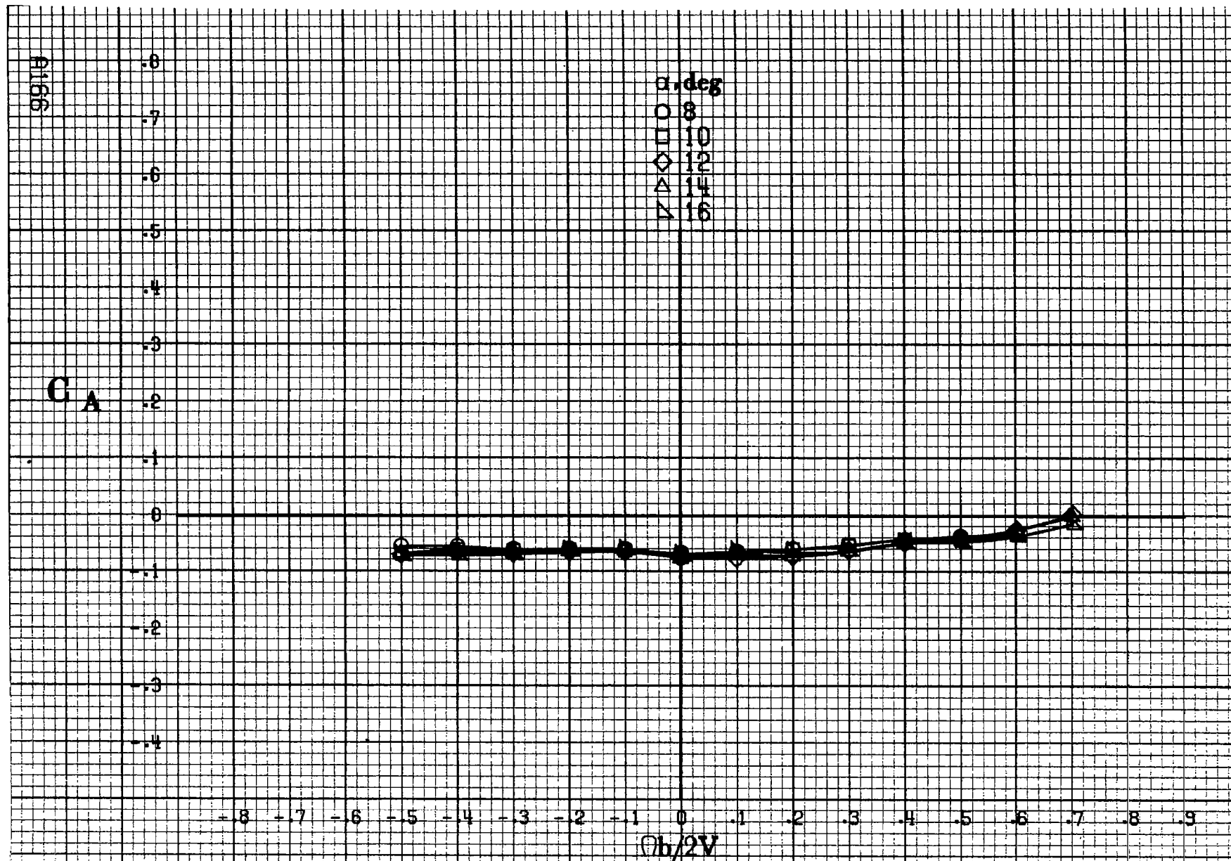
Figure A 42 - Effect of rotation rate and angle of attack on axial-force coefficient for basic configuration. \delta_e = 0^\circ , \delta_a = 0^\circ , \delta_{\alpha} = 0^\circ , \delta_r = 0^\circ , \beta = -10^\circ .
