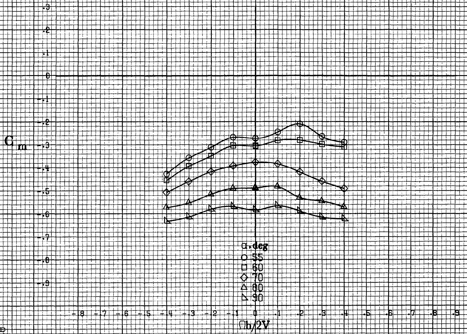
(b) \alpha = 55 to 90 deg, SR = 0 . Figure A93.-Concluded.
