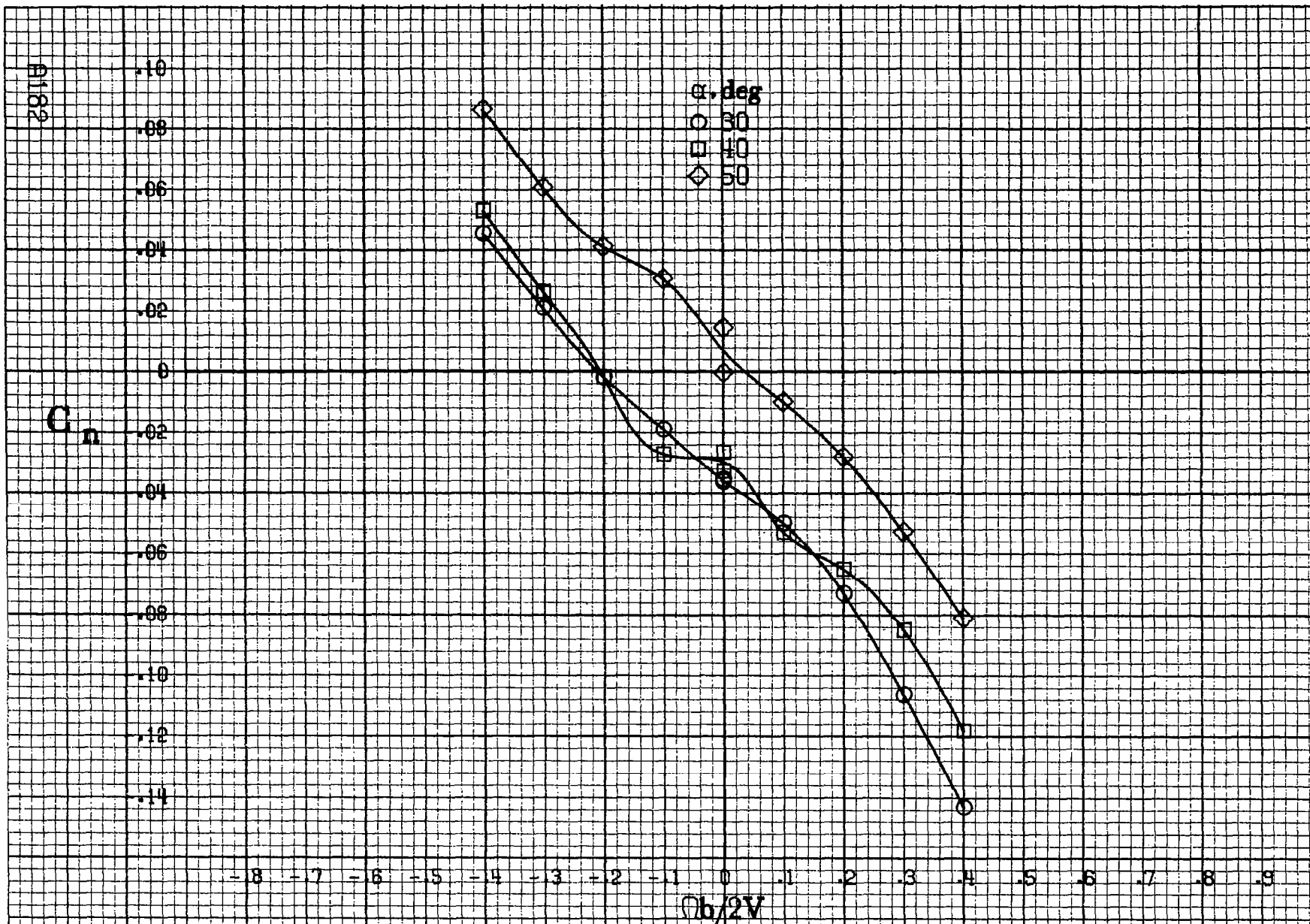
Figure A49.- Effect of rotation rate and angle of attack on yawing-moment coefficient for basic configuration. \delta_c = -25^\circ , \delta_a = 0^\circ , \delta_d = 0^\circ , \delta_r = 0^\circ , \beta = 10^\circ .
