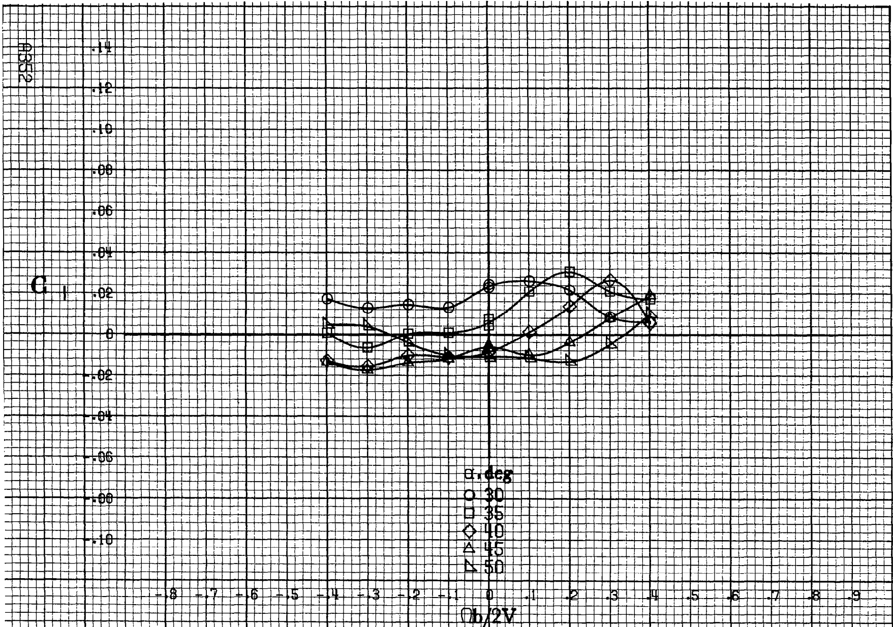
Figure A110.-Effect of rotation rate and angle of attack on rolling-moment coefficient for basic configuration. \delta_a = 0^\circ , \delta_s = -20.0^\circ , \delta_a = -6^\circ , \delta_r = 30^\circ , \beta = 10^\circ
