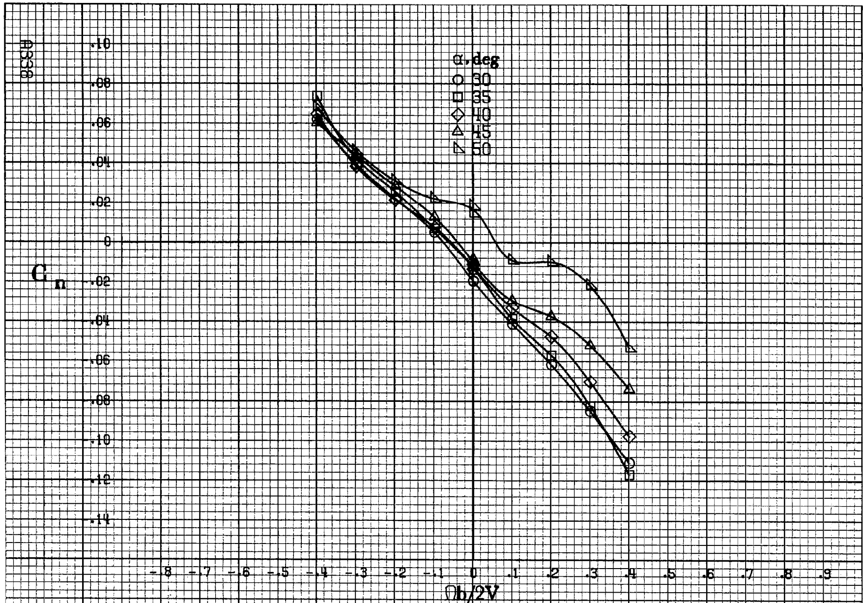
Figure A103.-Effect of rotation rate and angle of attack on yawing-moment coefficient for basic configuration. \delta_e=0^\circ , \delta_a=-20.0^\circ , \delta_d=-6^\circ , \delta_r=30^\circ , \beta=0^\circ .
