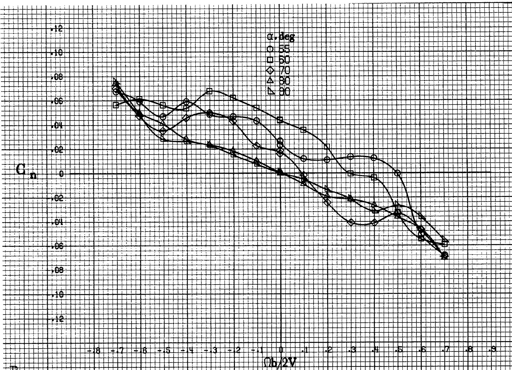
(d) \alpha = 55 to 90 deg, SR = 0 . Figure A1 - Concluded.
