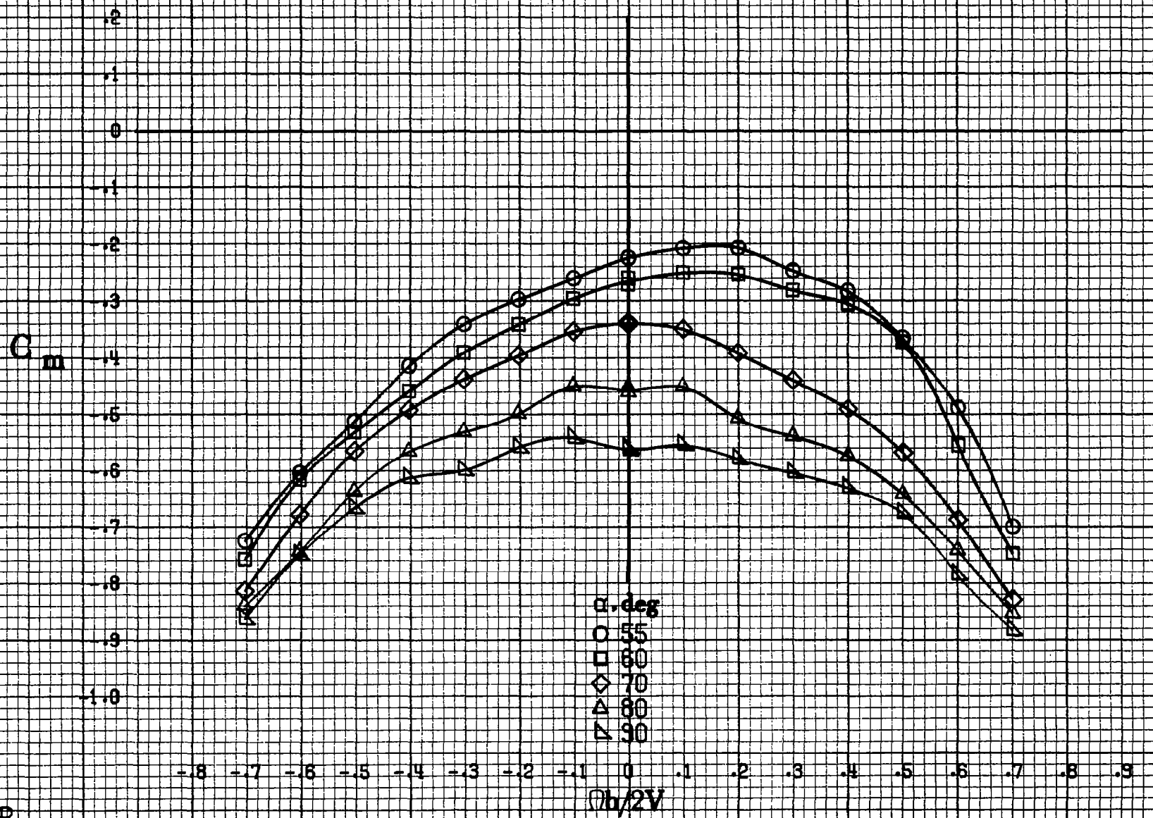
(d) \alpha = 55 to 90 deg, SR = 0 . Figure A21.-Concluded.
