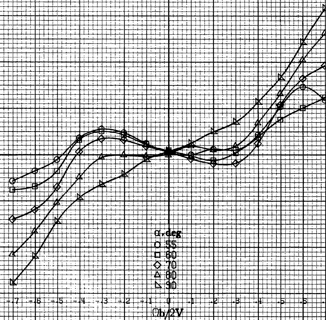
(d) \alpha=55 to 90 deg, SR=0 . Figure A26.-Concluded.
