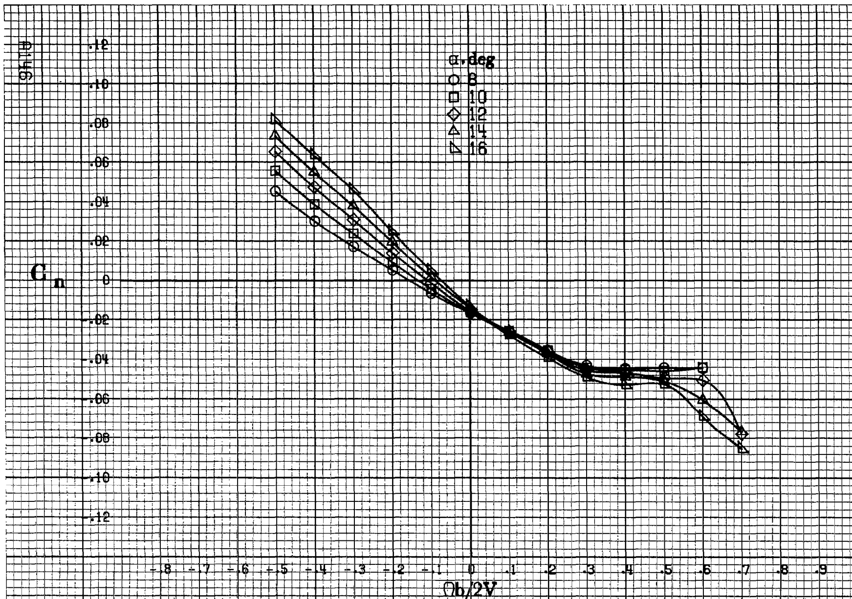
Figure A.37.-Effect of rotation rate and angle of attack on yawing-moment coefficient for basic configuration. \delta_e = 0^\circ , \delta_a = 0^\circ , \delta_d = 0^\circ , \delta_r = 0^\circ , \beta = -10^\circ .
