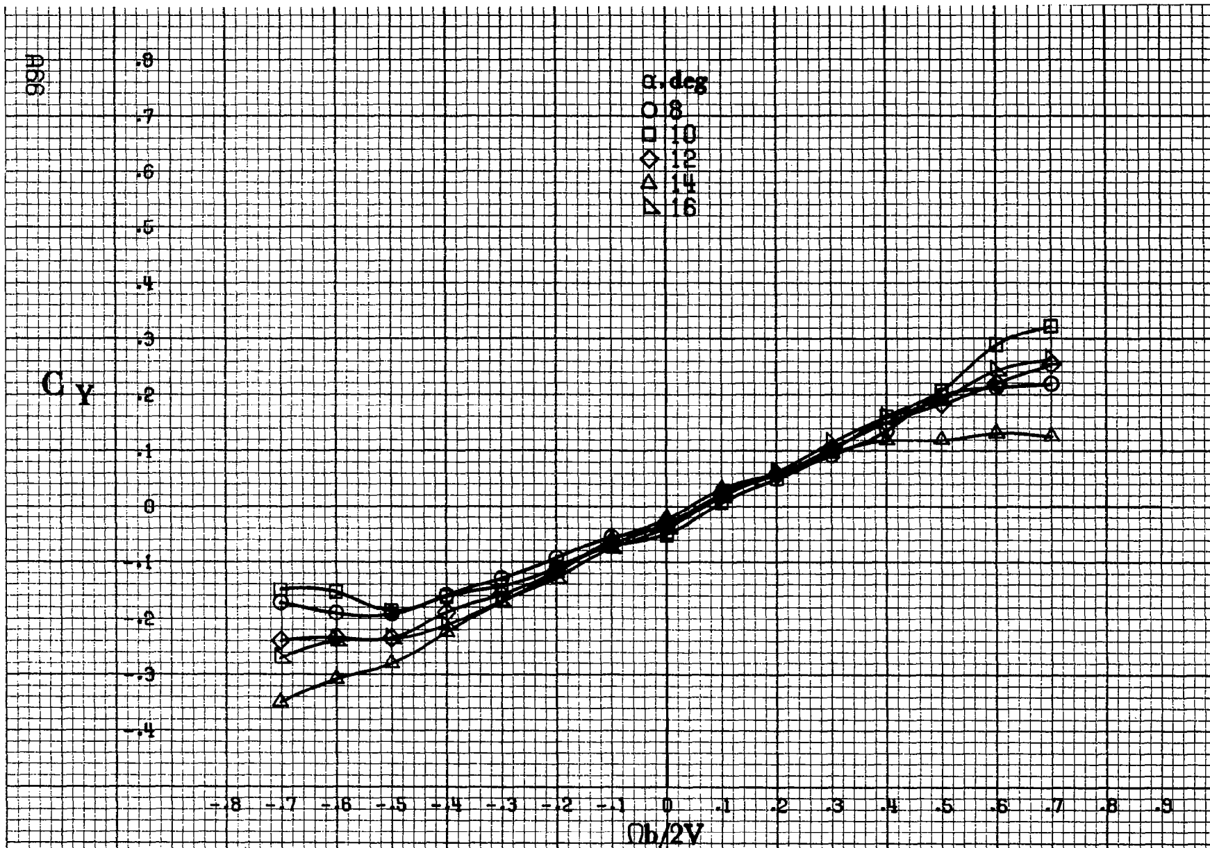
Figure A17.-Effect of rotation rate and angle of attack on side-force coefficient for body wing vertical tail configuration. \delta_a = 0^\circ , \delta_s = 0^\circ , \delta_r = 0^\circ . B = 0^\circ .
