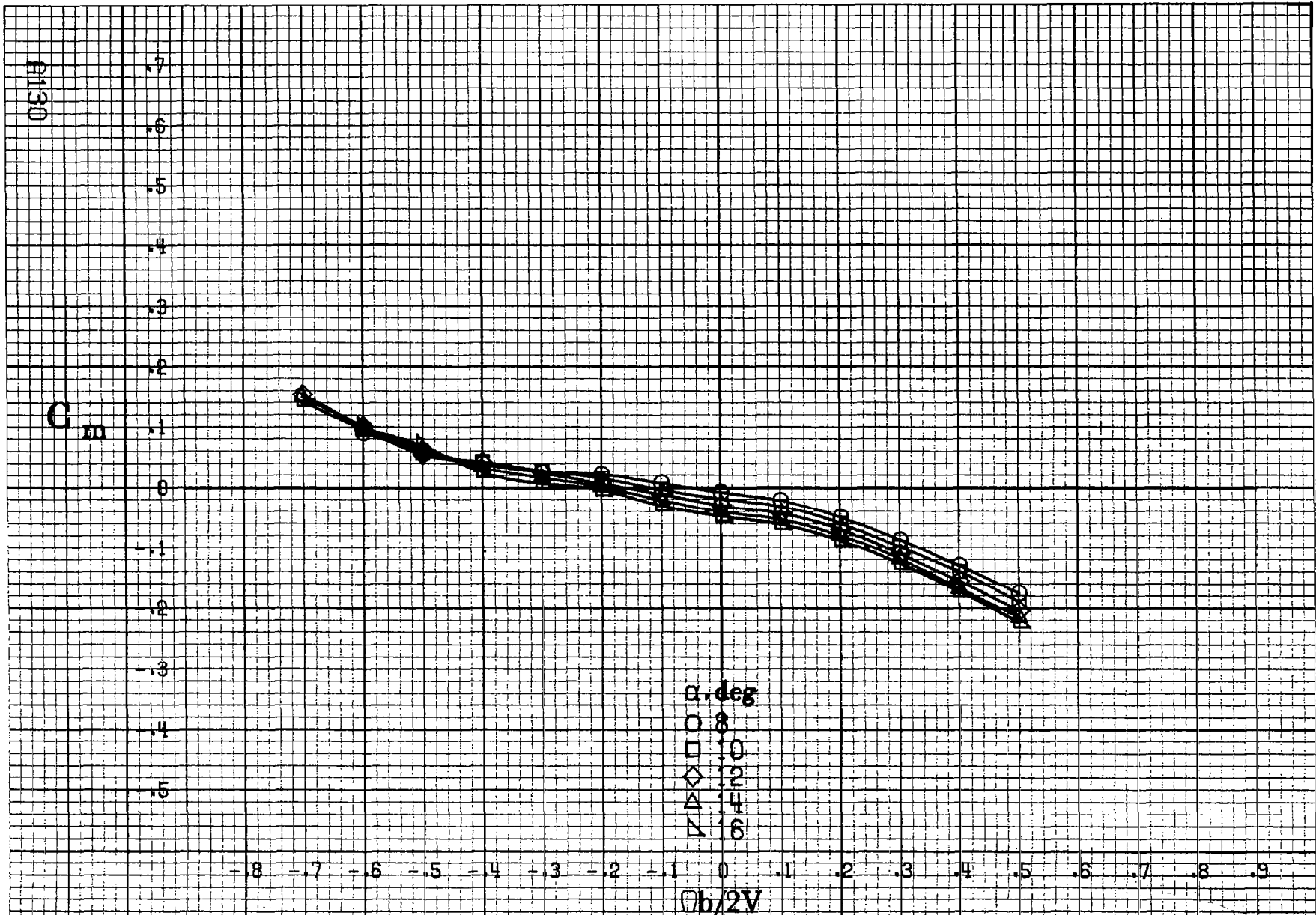
Figure A33.-Effect of rotation rate and angle of attack on pitching-moment coefficient for basic configuration. \delta_e = 0^\circ , \delta_a = 0^\circ , \delta_{\delta a} = 0^\circ , \delta_r = 0^\circ , \beta = 10^\circ .
