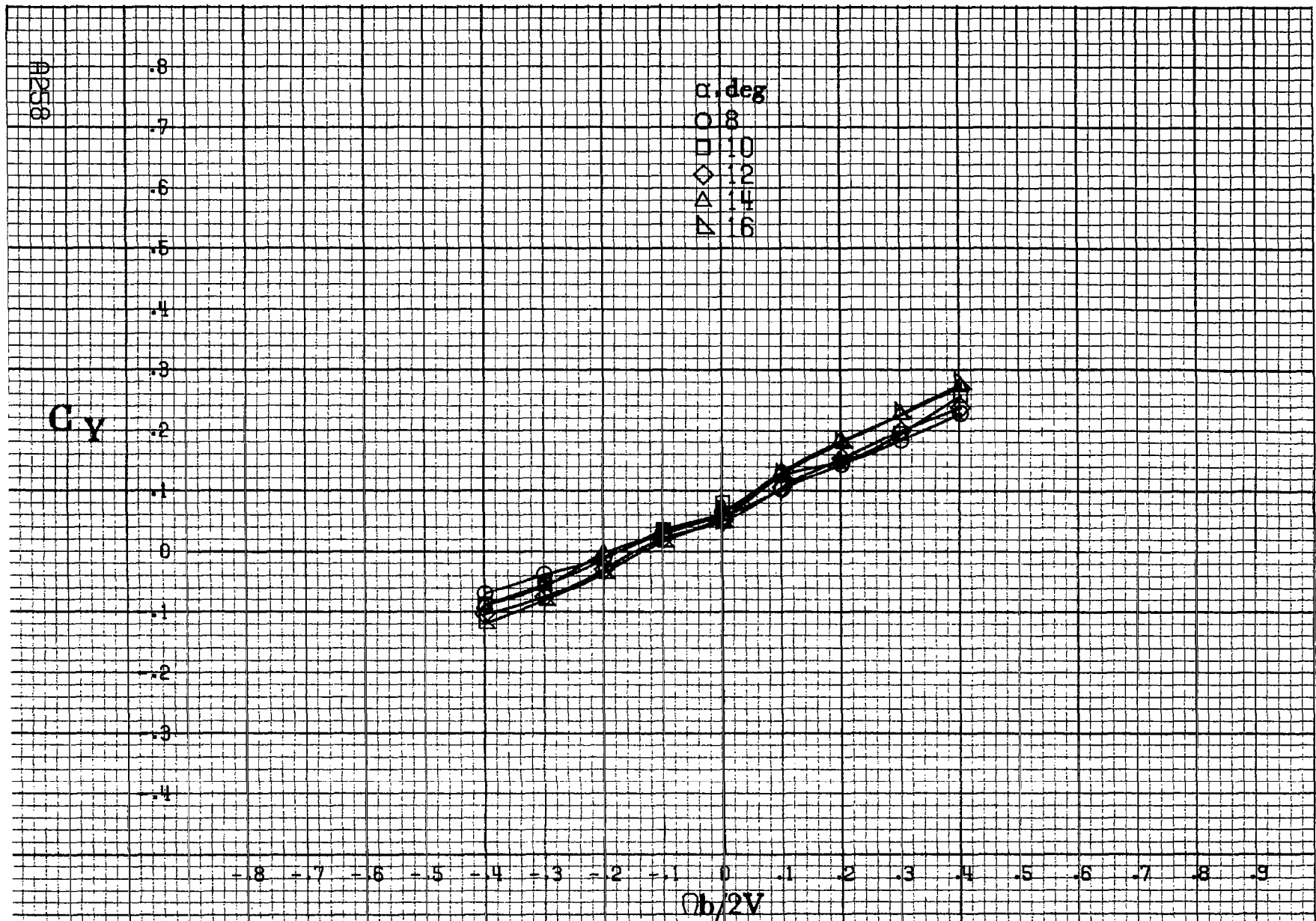
Figure A 71.-Effect of rotation rate and angle of attack on side-force coefficient for basic configuration. \delta_c = 0^\circ , \delta_a = 0^\circ , \delta_d = 11^\circ , \delta_r = 0^\circ , \beta = 0^\circ .
