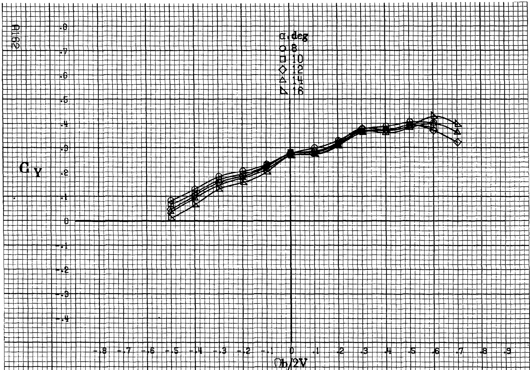
Figure A41. Effect of rotation rate and angle of attack on side force coefficient for basic configuration. \delta_r = 0^\circ , \delta_a = 0^\circ , \delta\alpha = 0^\circ , \delta\tau = 0^\circ . \beta = -10^\circ .
