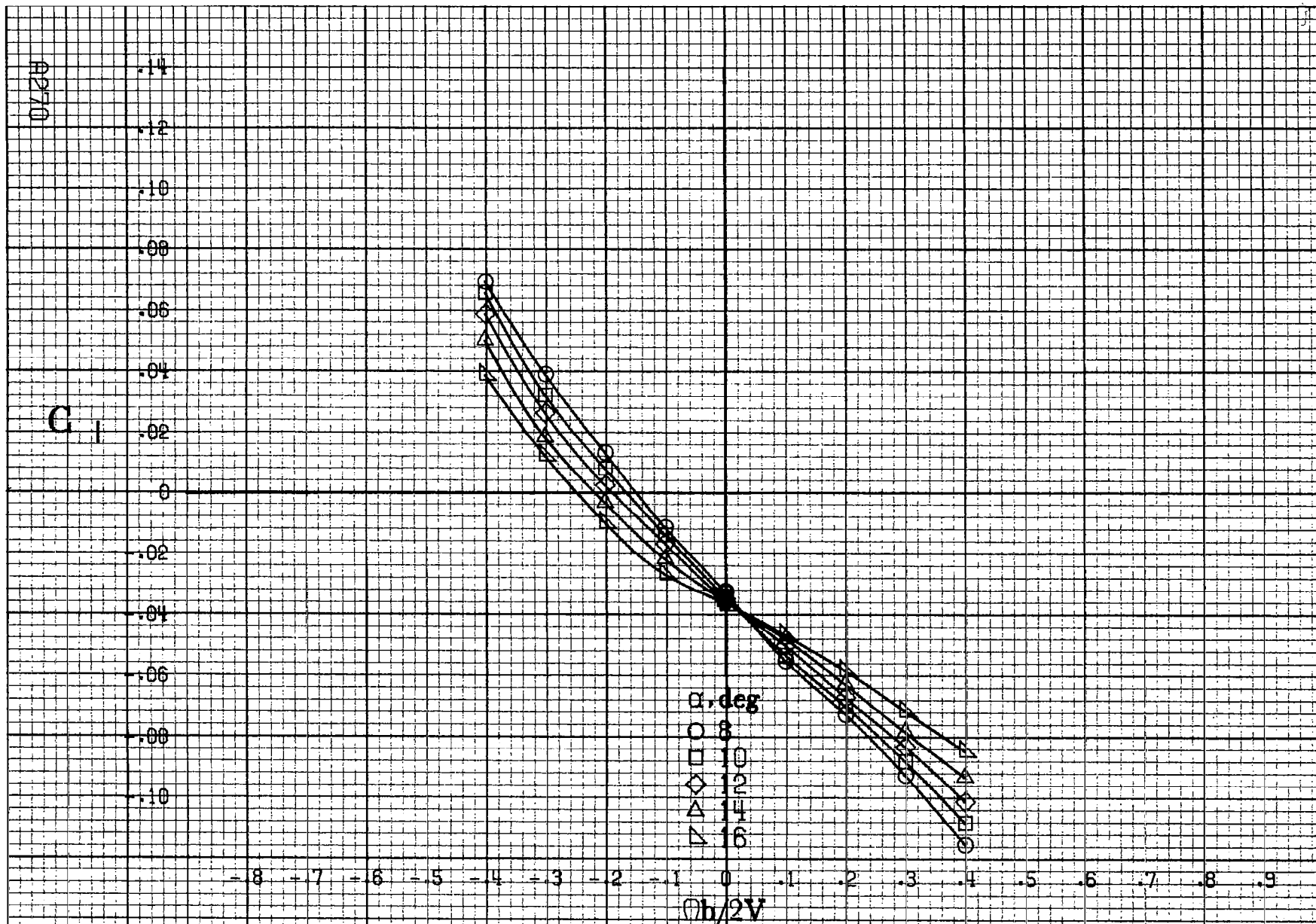
Figure A.74 - Effect of rotation rate and angle of attack on rolling-moment coefficient for basic configuration. \delta_e = 0^\circ , \delta_a = 0^\circ , \delta_a = 11^\circ , \delta_r = 0^\circ . B = 10^\circ .
