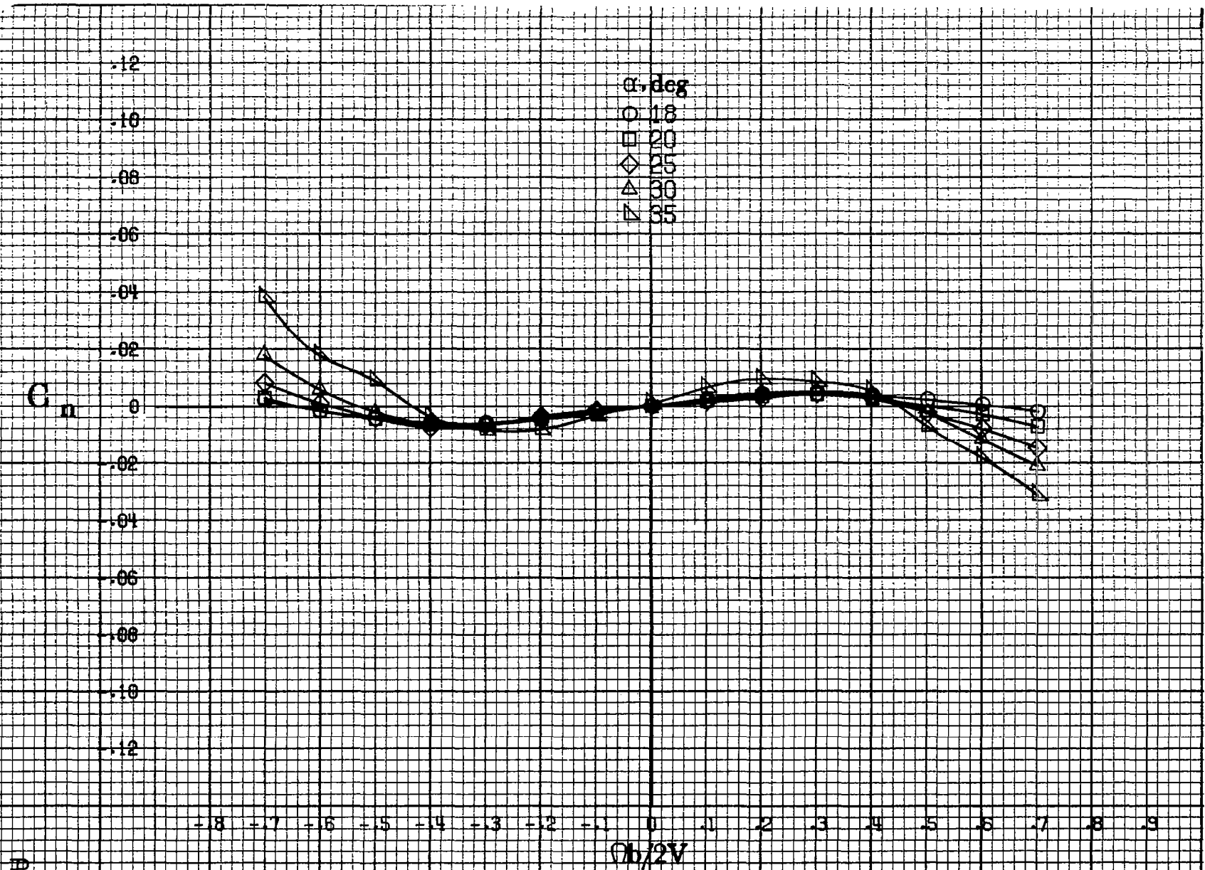
(b) \alpha = 18 to 35 deg, SR = 182.9 cm (72 in). Figure A1.-Continued.
