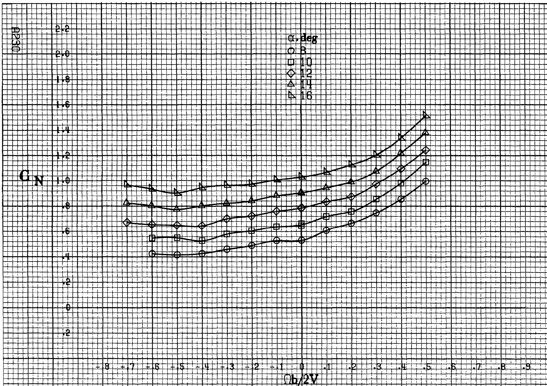
Figure A 64 - Effect of rotation rate and angle of attack on normal-force coefficient for basic configuration. \delta_c = 0^\circ , \delta_s = 0^\circ , \delta_a = 6^\circ , \delta_r = 0^\circ , \beta = 10^\circ .
