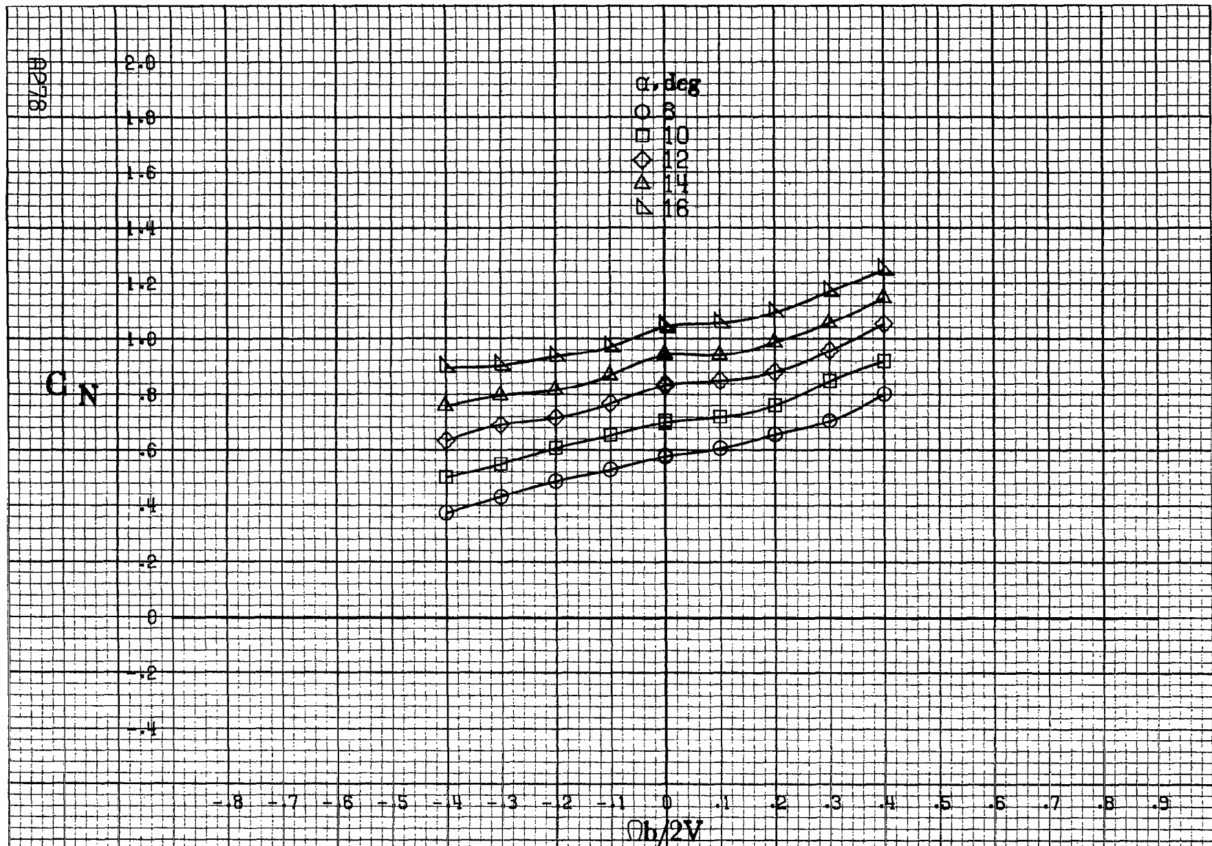
Figure A76.-Effect of rotation rate and angle of attack on normal-force coefficient for basic configuration. \delta_e = 8^\circ , \delta_a = 0^\circ , \delta_{\alpha} = 11^\circ , \delta_r = 0^\circ , \beta = 10^\circ .
