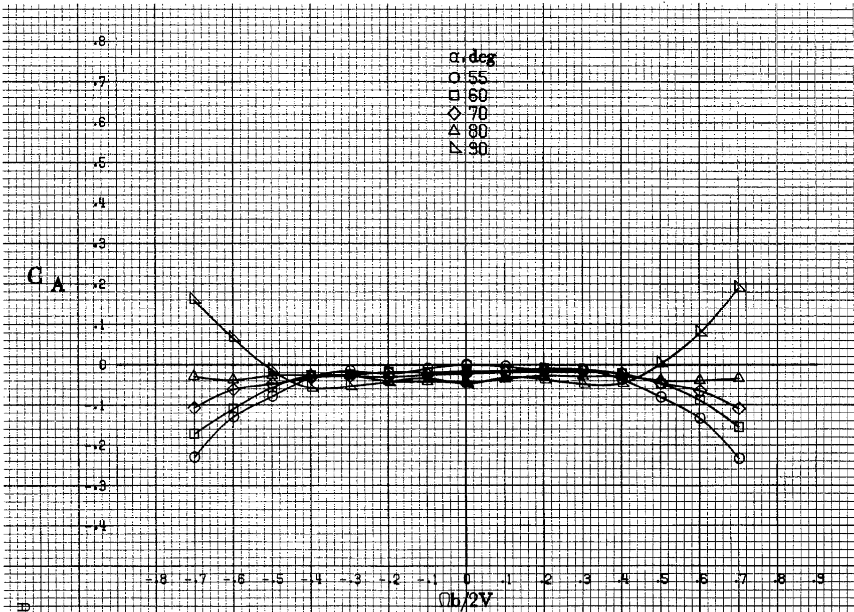
(d) \alpha = 55 to 90 deg, SR = 0 . Figure A18.-Concluded.
