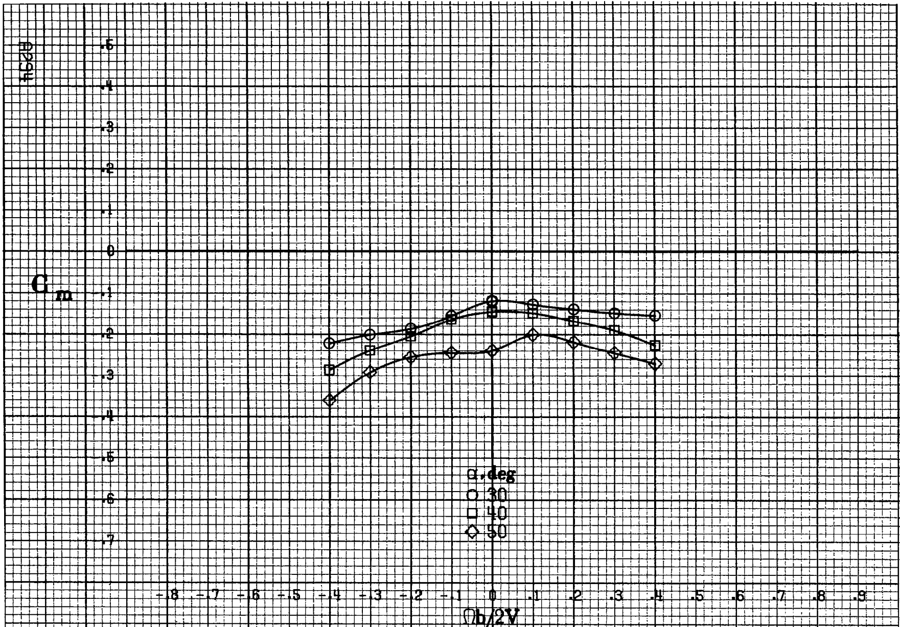
Figure A81.- Effect of rotation rate and angle of attack on pitching-moment coefficient for basic configuration. \delta_a = 0^\circ , \delta_s = 20.0^\circ , \delta_d = 6^\circ , \delta_r = 0^\circ , \beta = 0^\circ .
