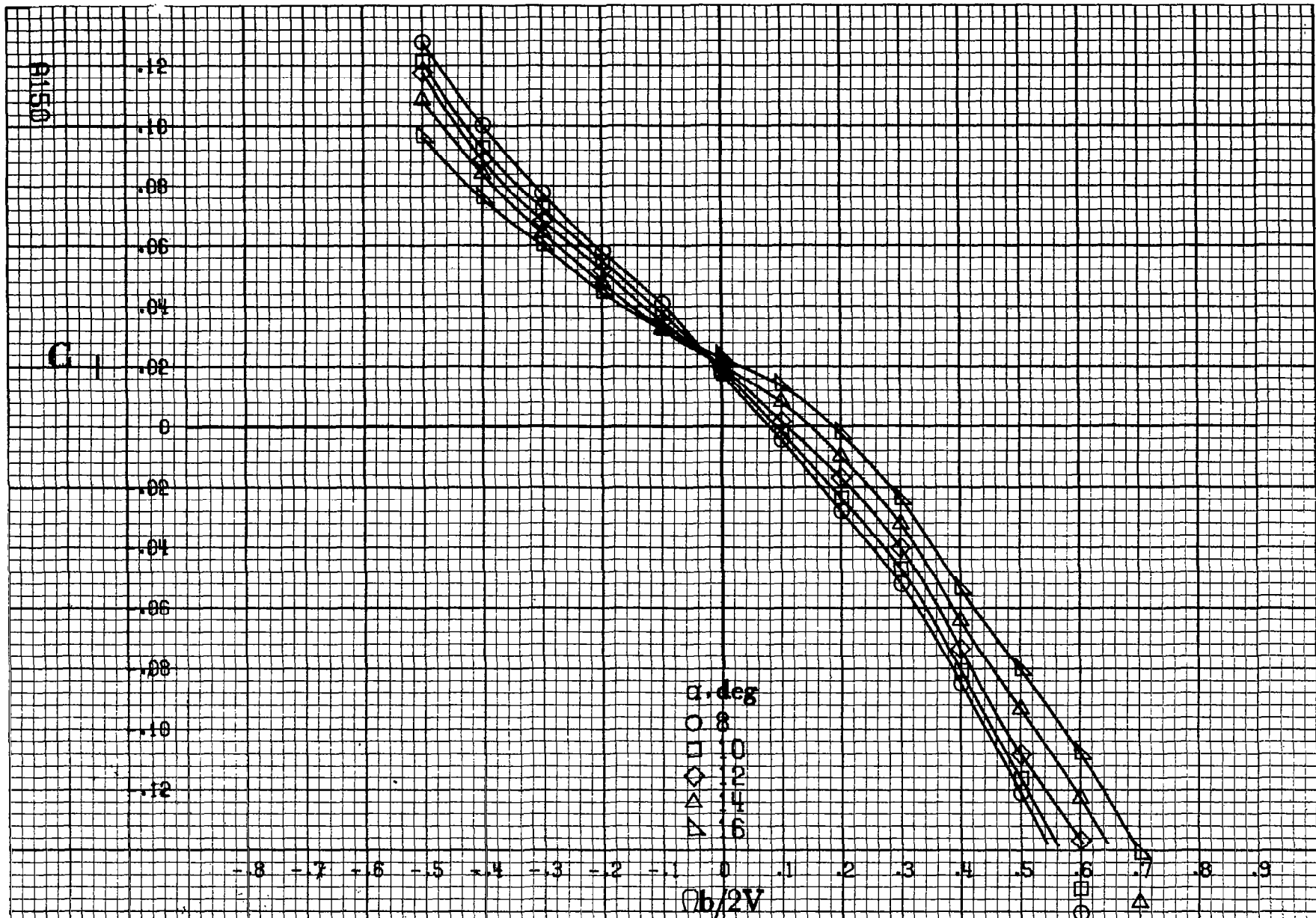
Figure A 38 - Effect of rotation rate and angle of attack on rolling-moment coefficient for basic configuration, \delta_e = 0^\circ , \delta_a = 0^\circ , \delta_d = 0^\circ , \delta_r = 0^\circ , \beta = -10^\circ .
