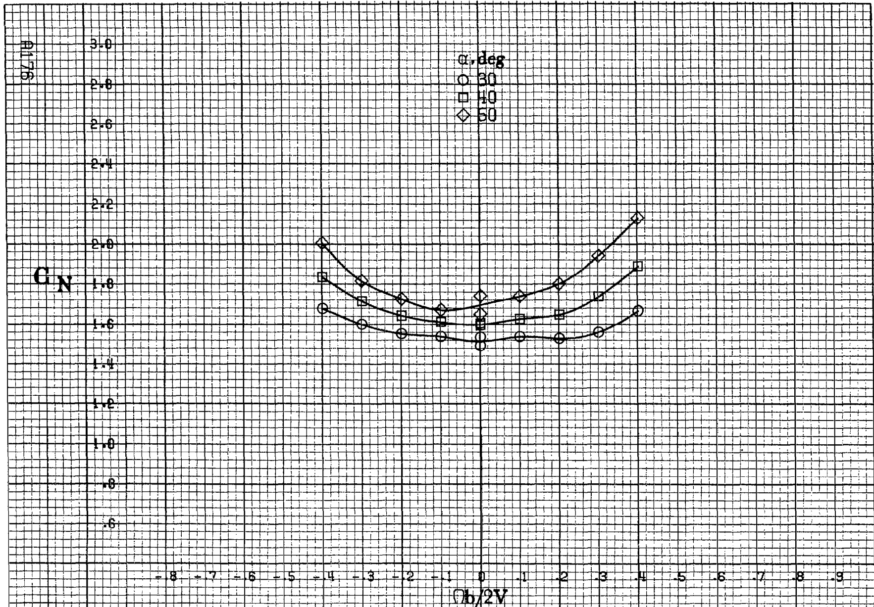
Figure A 46.- Effect of rotation rate and angle of attack on normal-force coefficient for basic configuration. \delta_e = -25^\circ , \delta_a = 0^\circ , \delta_d = 0^\circ , \delta_r = 0^\circ , \beta = 0^\circ .
