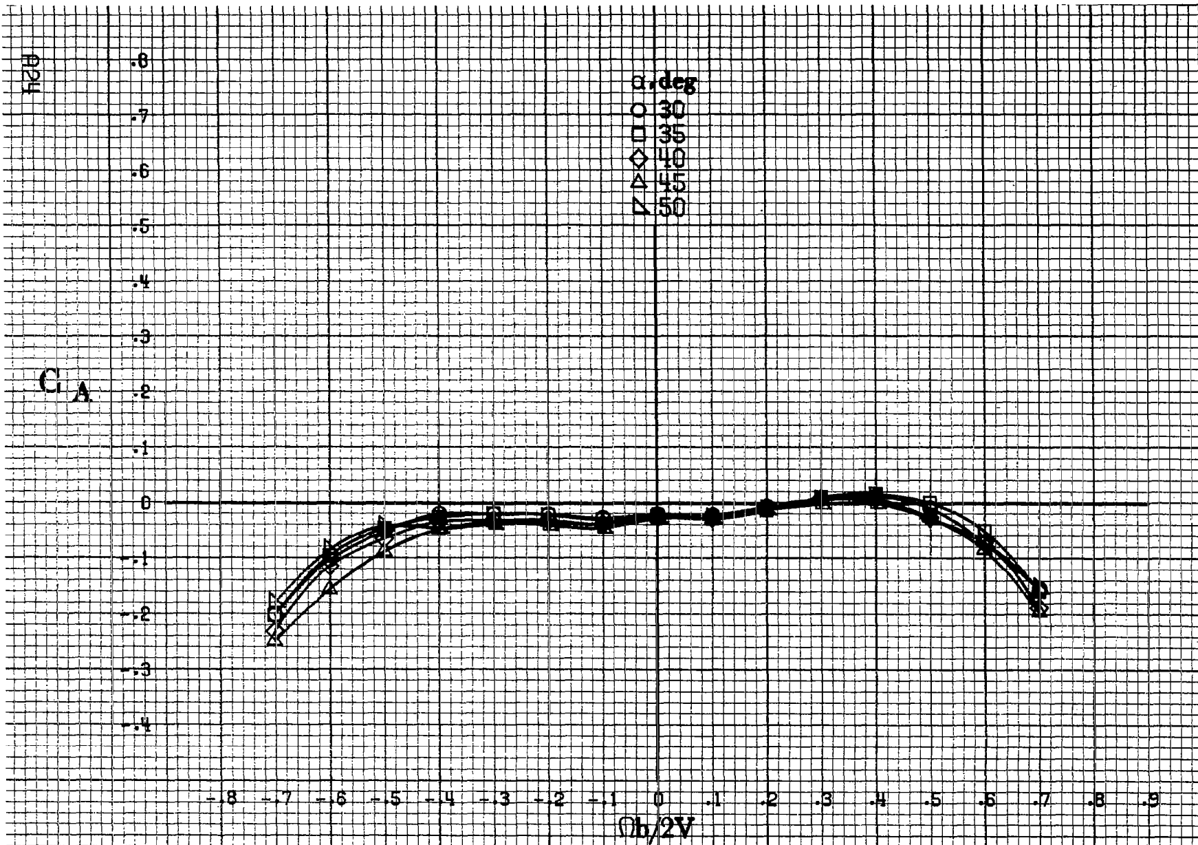
(c) \alpha = 30 to 50 deg, SR = 0 . Figure A 6.-Continued.
