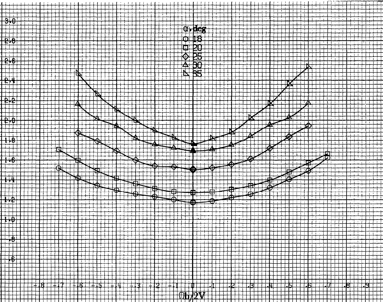
(b) \alpha = 18 to 35 deg, SR = 182.9 cm (72 in). Figure A28.-Continued.
