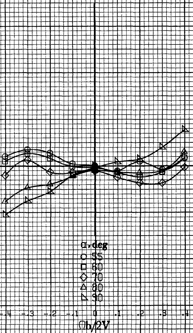
(d) \alpha=55 to 90 deg, SR=0 . Figure A 68.-Concluded.
