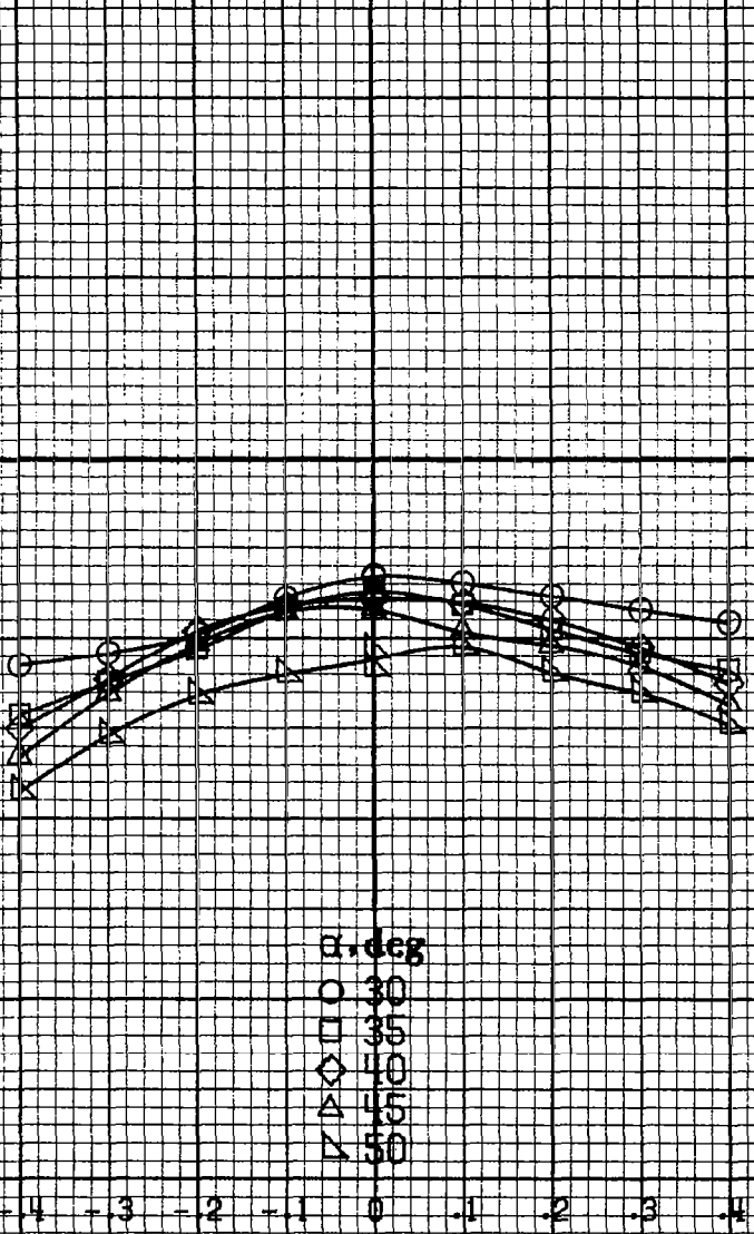
Figure A93 - Effect of rotation rate and angle of attack on pitching-moment coefficient for basic configuration. \delta_c = 0^\circ , \delta_a = 20.0^\circ , \delta_a = 6^\circ , \delta_r = -15^\circ , \beta = 0^\circ .
