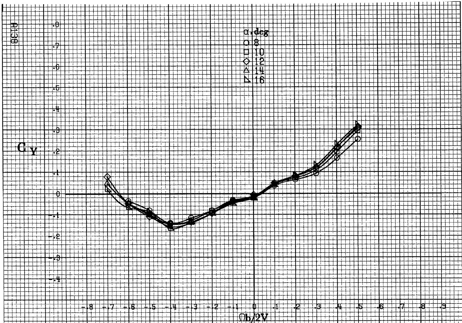
Figure A 35.-Effect of rotation rate and angle of attack on side-force coefficient for basic configuration. \delta_e = 0^\circ , \delta_a = 0^\circ , \delta_{\delta a} = 0^\circ , \delta_r = 0^\circ , \beta = 10^\circ .
