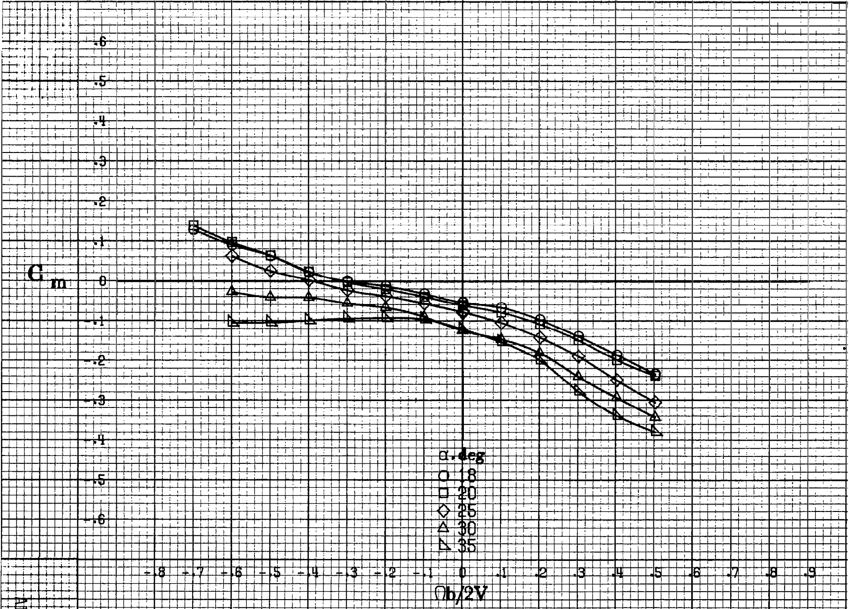
(b) \alpha = 18 to 35 deg, SR = 182.9 cm (72 in). Figure A33.-Continued.
