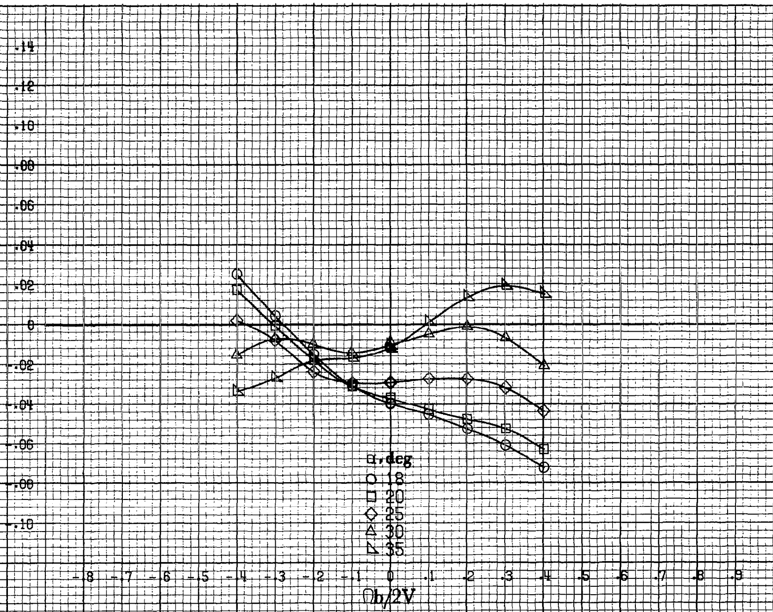
(b) \alpha = 18 to 35 deg, SR = 182.9 cm (72 in). Figure A 74.-Continued.
