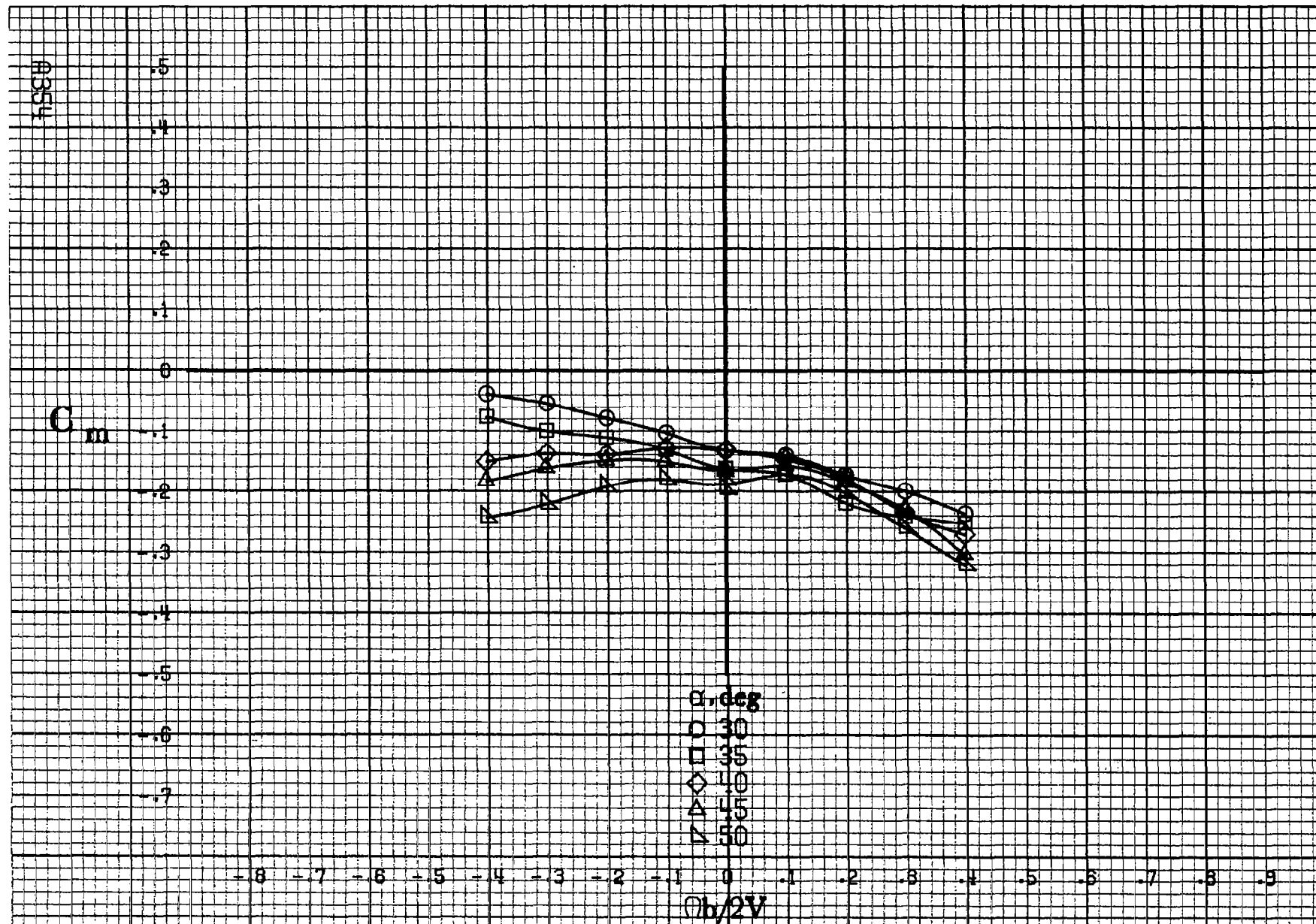
Figure A111.-Effect of rotation rate and angle of attack on pitching-moment coefficient for basic configuration. \delta_e = 0^\circ , \delta_s = -20.0^\circ , \delta_d = -6^\circ , \delta_r = 30^\circ , \beta = 10^\circ
