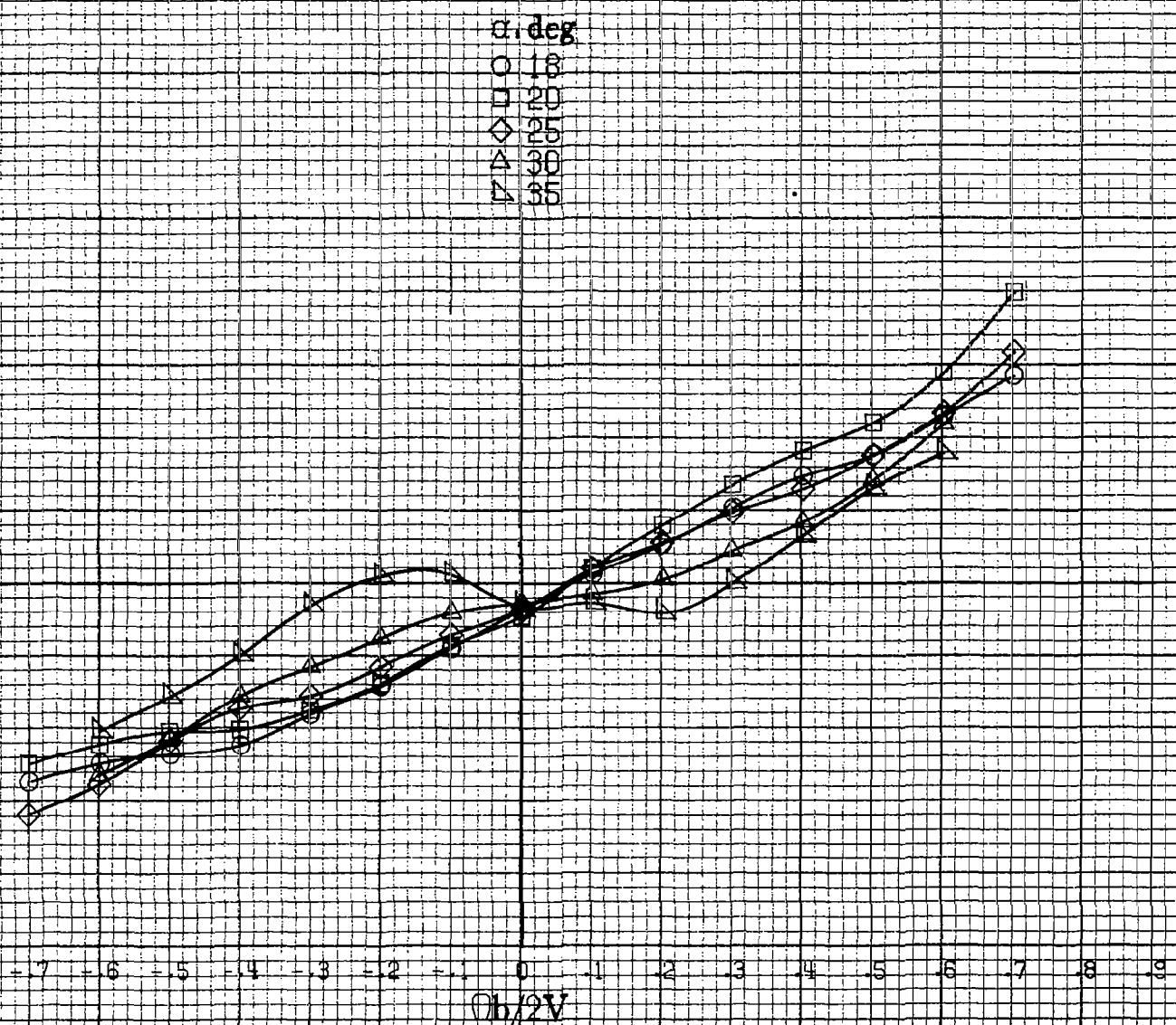
(b) \alpha = 18 to 35 deg, SR = 182.9 cm (72 in). Figure A17.-Continued.
