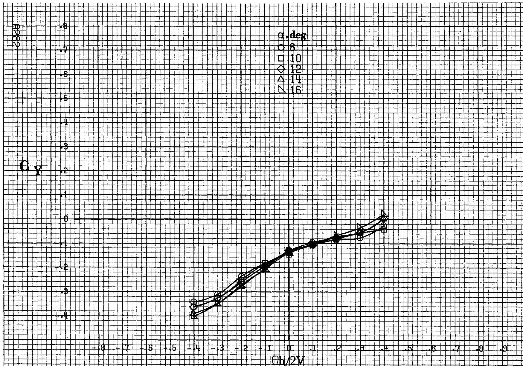
Figure A.77.-Effect of rotation rate and angle of attack on side-force coefficient for basic configuration. \delta_e = 0^\circ , \delta_a = 0^\circ , \delta_d = 11^\circ , \delta_r = 0^\circ , \beta = 10^\circ .
