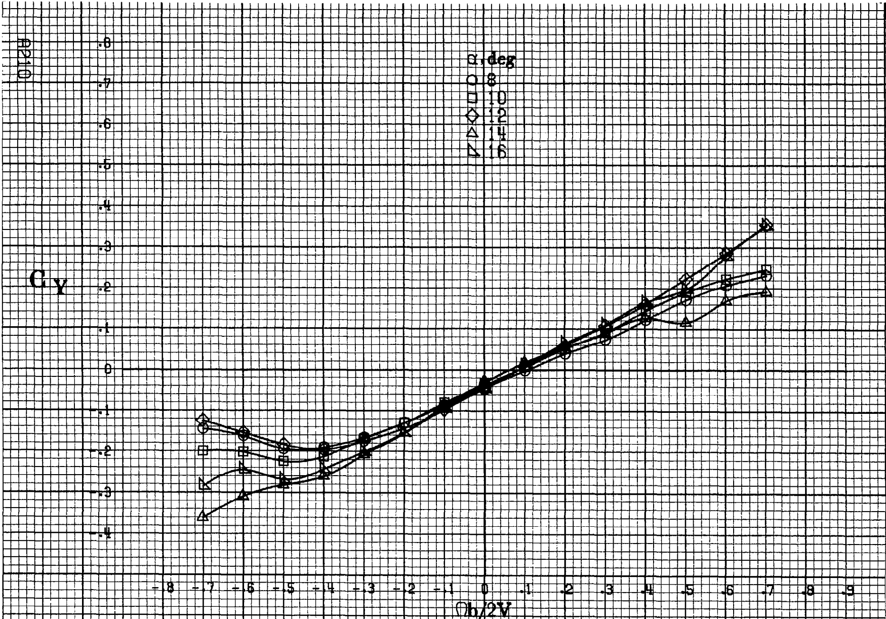
Figure A59.-Effect of rotation rate and angle of attack on side-force coefficient for basic configuration. \delta_c = 0^\circ , \delta_a = 0^\circ , \delta_R = 16^\circ , \delta_r = 0^\circ , \beta = 0^\circ .
