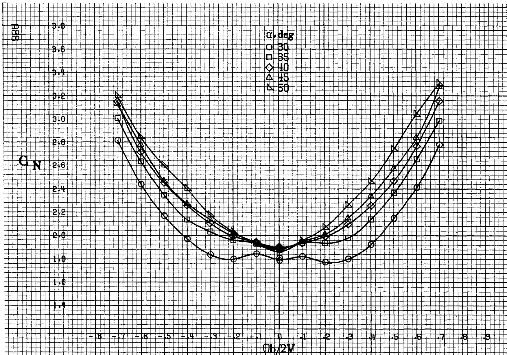
(c) \alpha = 30 to 50 deg, SR = 0 . Figure A 22.-Continued.
