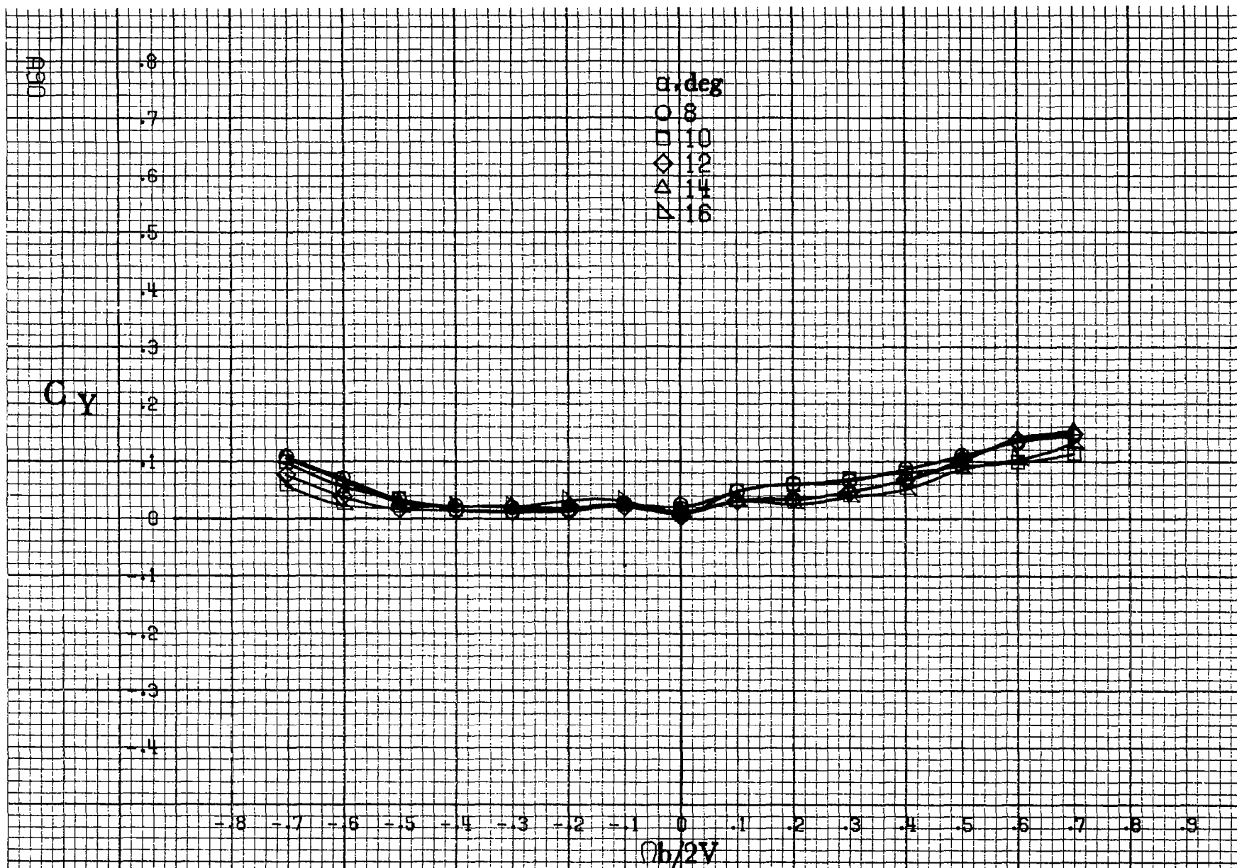
Figure A 23. - Effect of rotation rate and angle of attack on side-force coefficient for body wing horizontal tail configuration. \delta_c = 0^\circ , \delta_s = 0^\circ , \delta_w = 0^\circ , \beta = 0^\circ .
