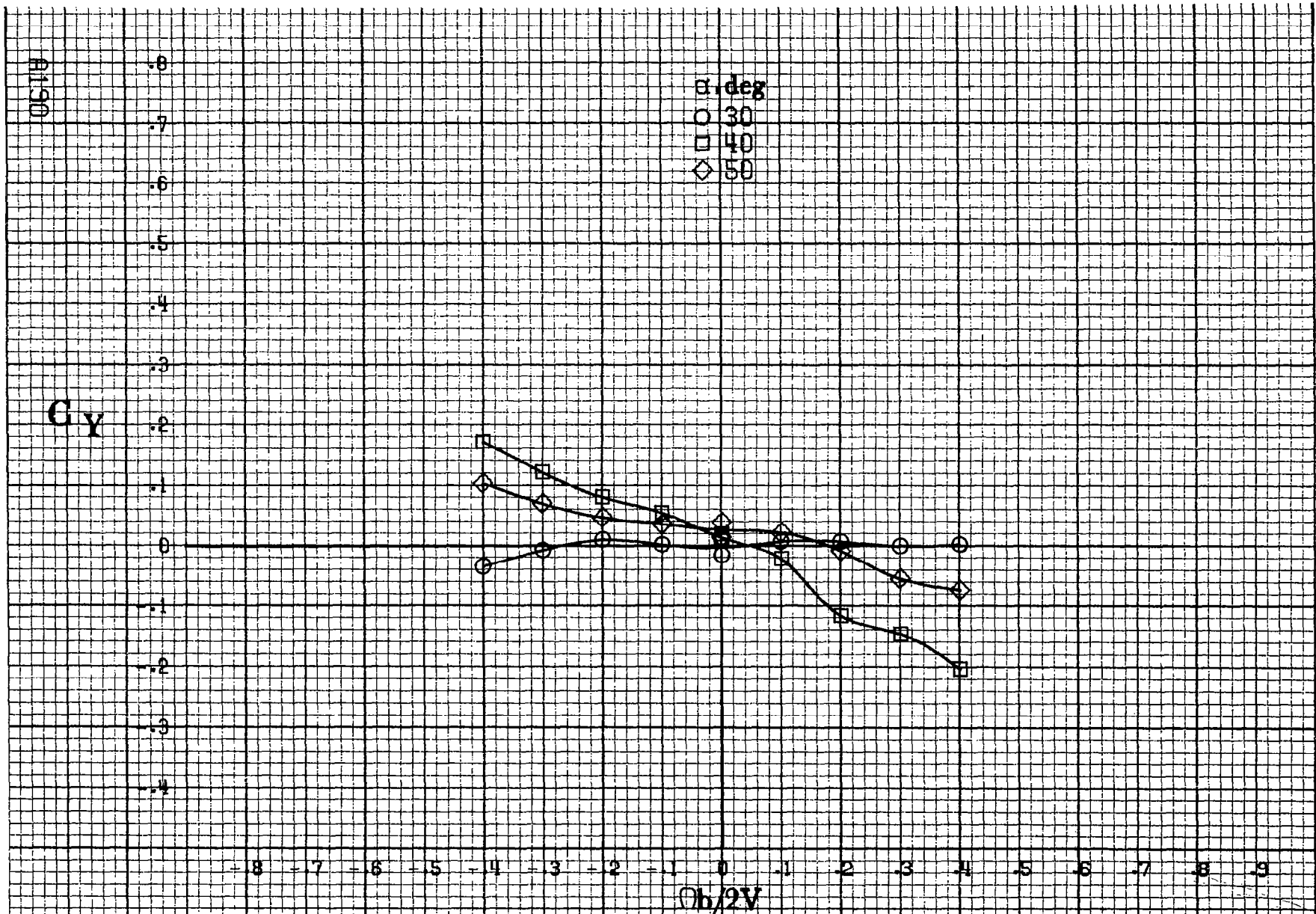
Figure A53. Effect of rotation rate and angle of attack on side-force coefficient for basic configuration. \delta_e = -25^\circ , \delta_a = 0^\circ , \delta_d = 0^\circ , \delta_r = 0^\circ , \theta = 10^\circ .
