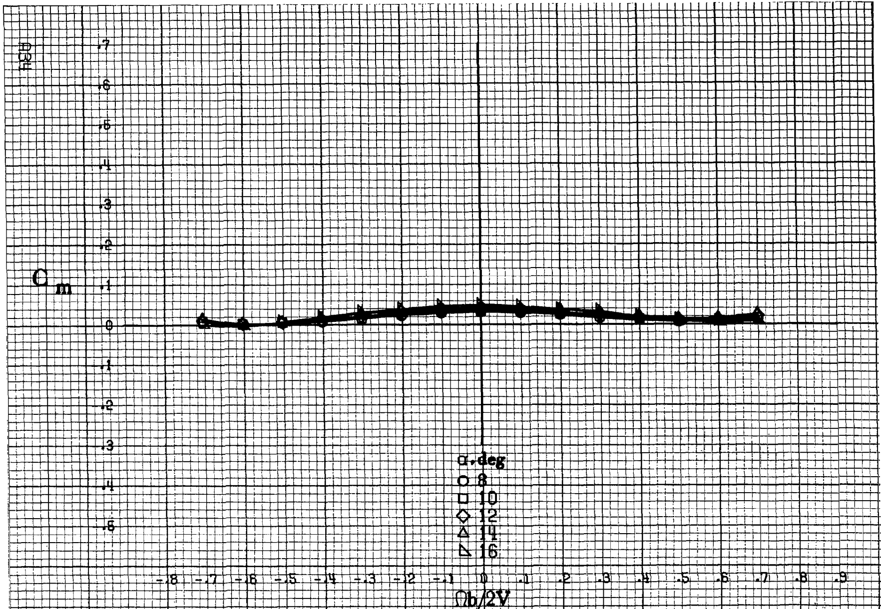
Figure A9.-Effect of rotation rate and angle of attack on pitching-moment coefficient for body wing configuration. \delta_a = 0^\circ , \delta_s = 0^\circ , \delta_r = 0^\circ , \beta = 0^\circ .
