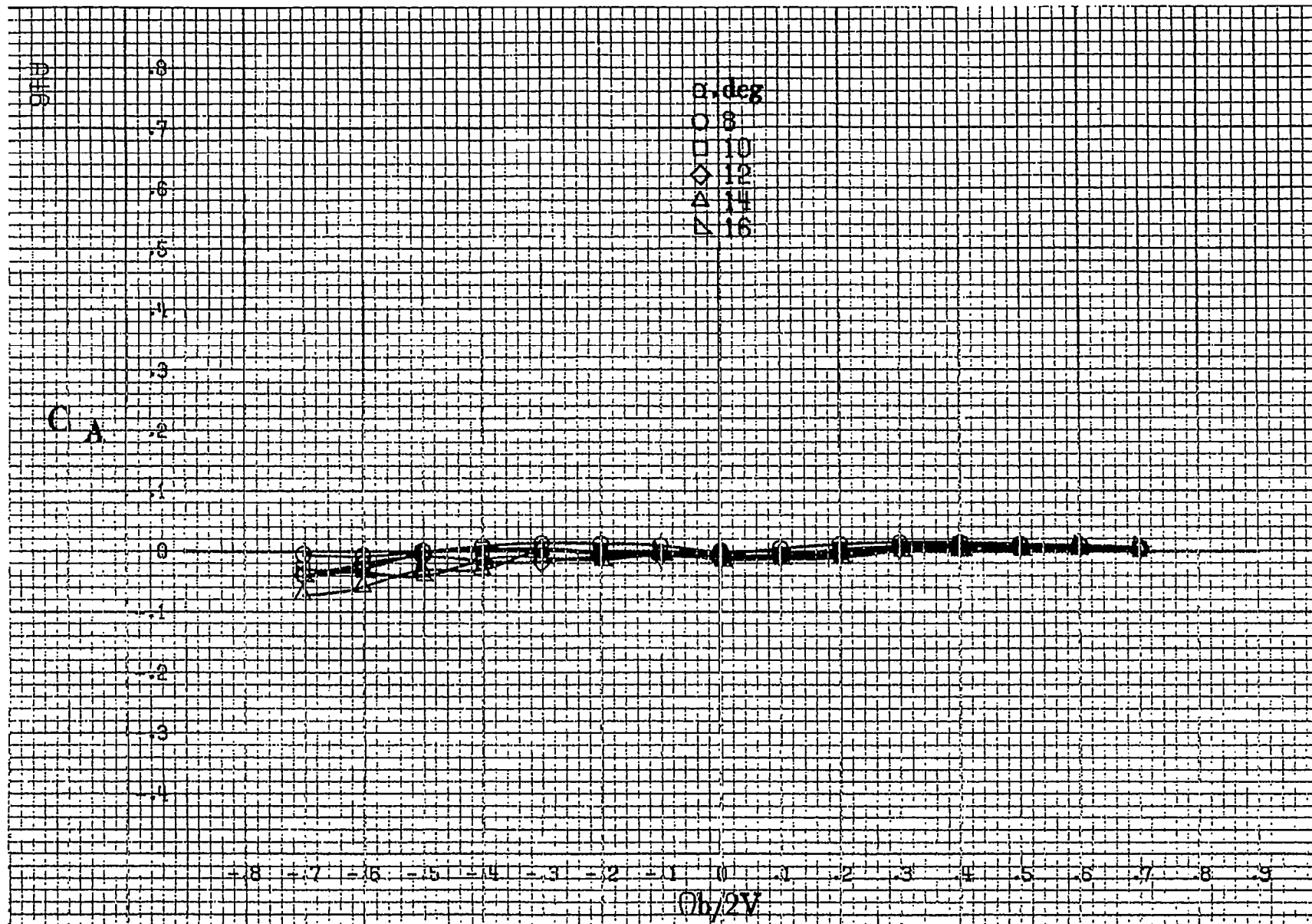
Figure A12 - Effect of rotation rate and angle of attack on axial-force coefficient for body wing configuration. \delta_z = 0^\circ , \delta_x = 0^\circ , \delta_r = 0^\circ , \delta = 0^\circ .
