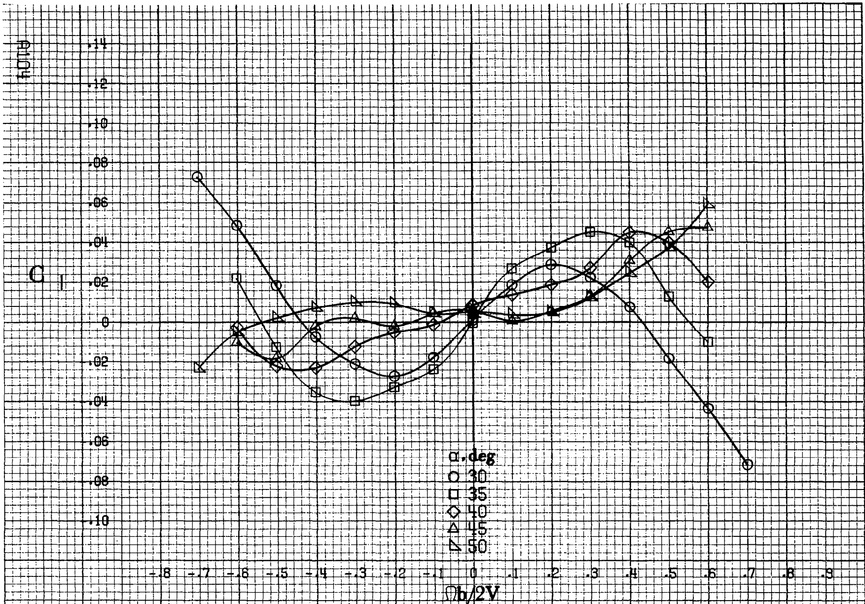
(c) \alpha = 30 to 50 deg. SR = 0 . Figure A26.-Continued.
