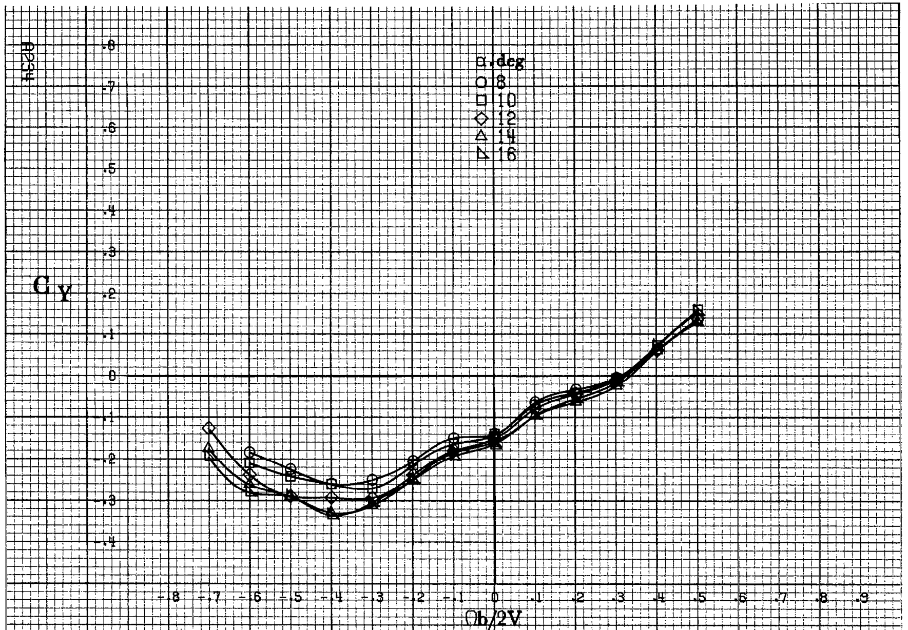
Figure A65 - Effect of rotation rate and angle of attack on side-force coefficient for basic configuration. \delta_e = 0^\circ , \delta_a = 0^\circ , \delta_{\dot{a}} = 6^\circ , \delta_r = 0^\circ , \beta = 10^\circ .
