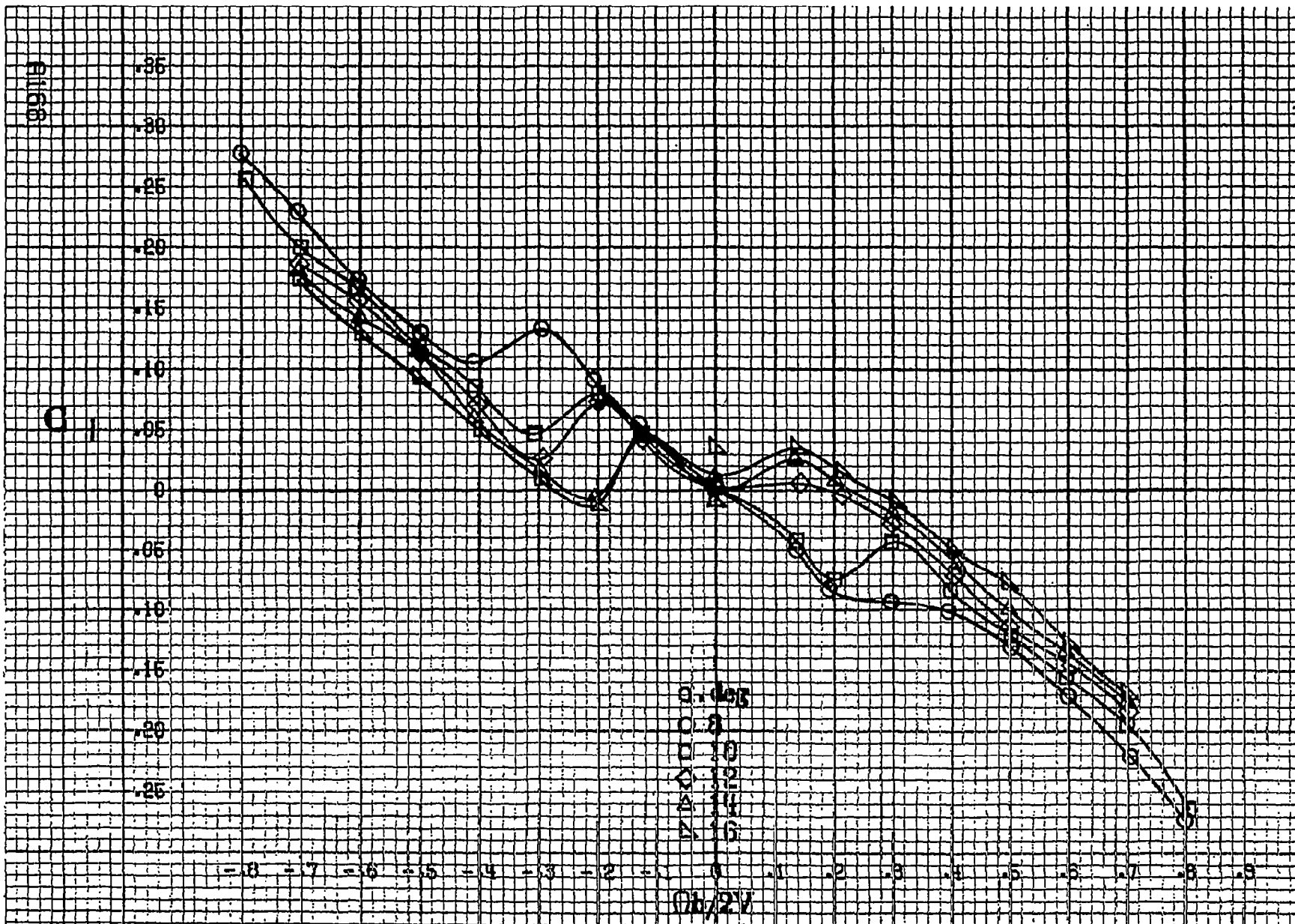
Figure A13. Effect of rotation rate and angle of attack on rolling moment coefficient for full-span LL wing drop with large nose radius. \delta_a = 0^\circ , \delta_r = 0^\circ , \beta = 0^\circ . (a) \alpha = 81 \pm 16 deg, SR = 1.82, \rho = 72 ft/s.
