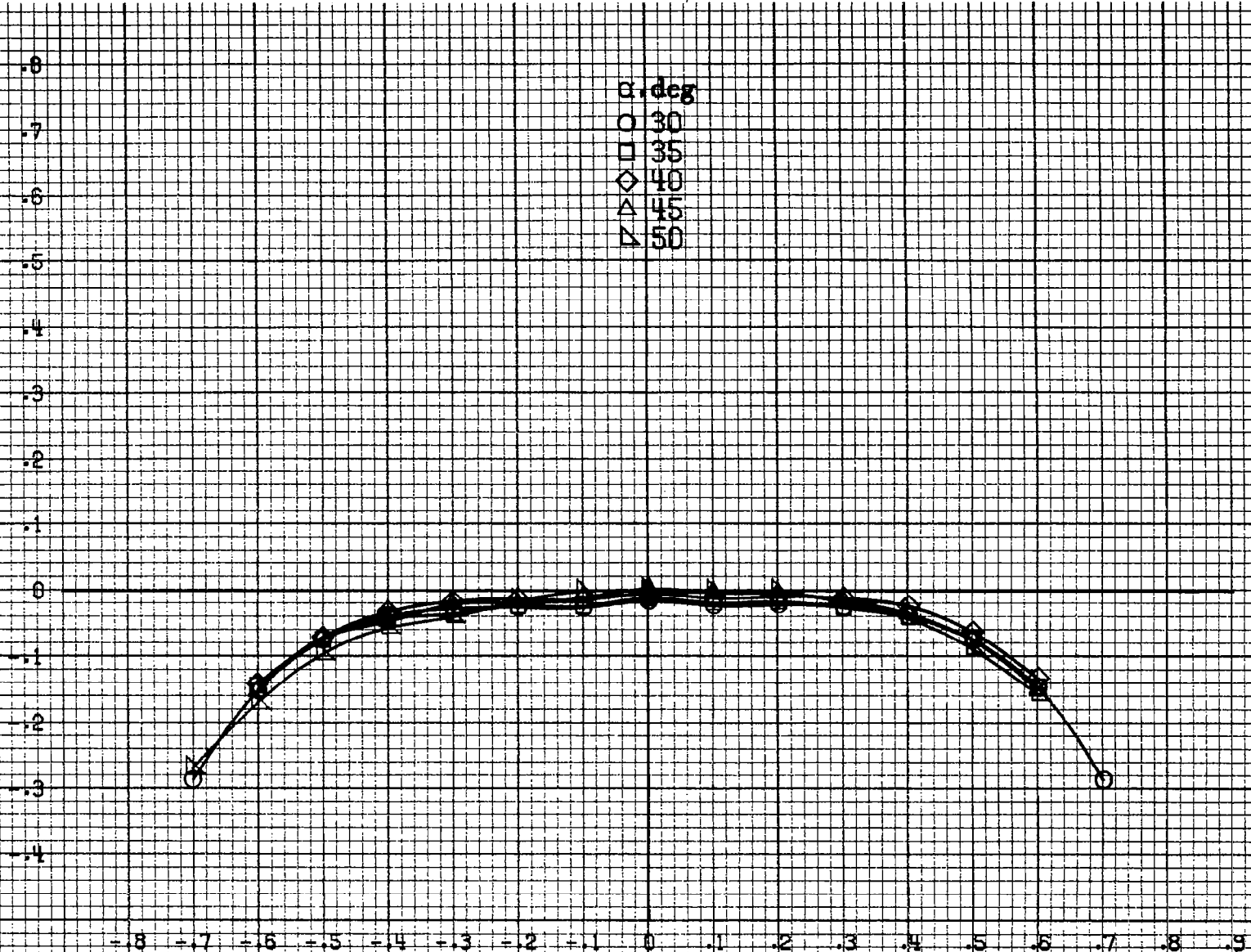
(c) \alpha=30 to 50 deg, SR=0 . Figure A18.-Continued.
