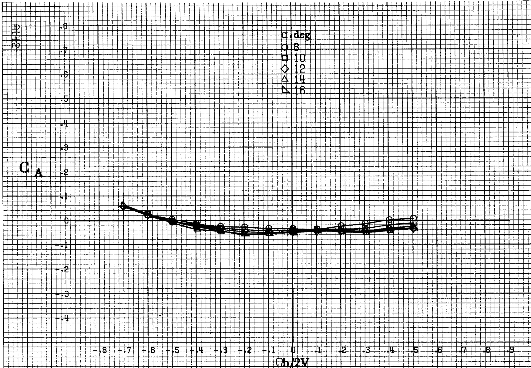
Figure A36.-Effect of rotation rate and angle of attack on axial-force coefficient for basic configuration. \delta_r = 0^\circ , \delta_a = 0^\circ , \delta_d = 0^\circ , \delta_r = 0^\circ , \beta = 10^\circ .
