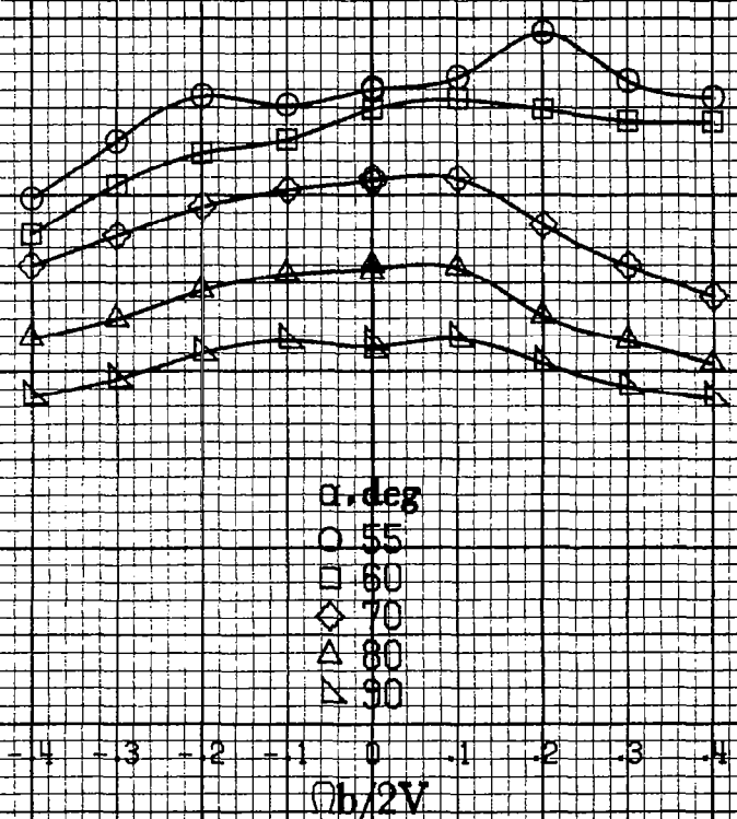
(d) \alpha = 55 to 90 deg, SR = 0 . Figure A 69.- Concluded.
