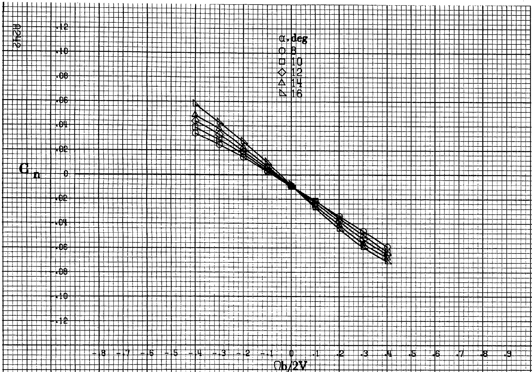
Figure A67.-Effect of rotation rate and angle of attack on yawing-moment coefficient for basic configuration. \delta_e=0^\circ , \delta_a=0^\circ , \delta_a=11^\circ , \delta_r=0^\circ , \beta=0^\circ .
