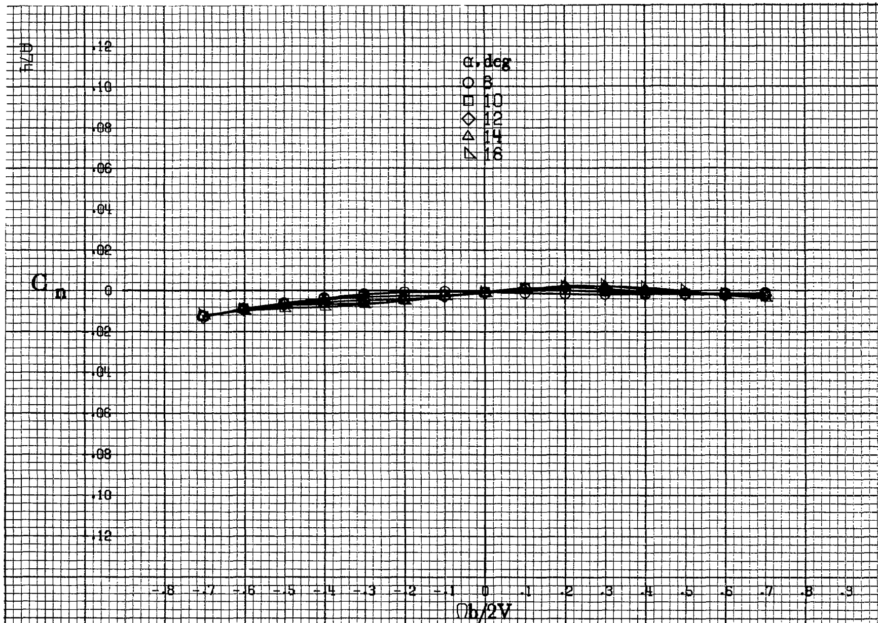
Figure A19. Effect of rotation rate and angle of attack on yawing-moment coefficient for body wing horizontal tail configuration. \delta_e = 0^\circ , \delta_r = 0^\circ , \delta_x = 0^\circ , \beta_1 = 0^\circ .
