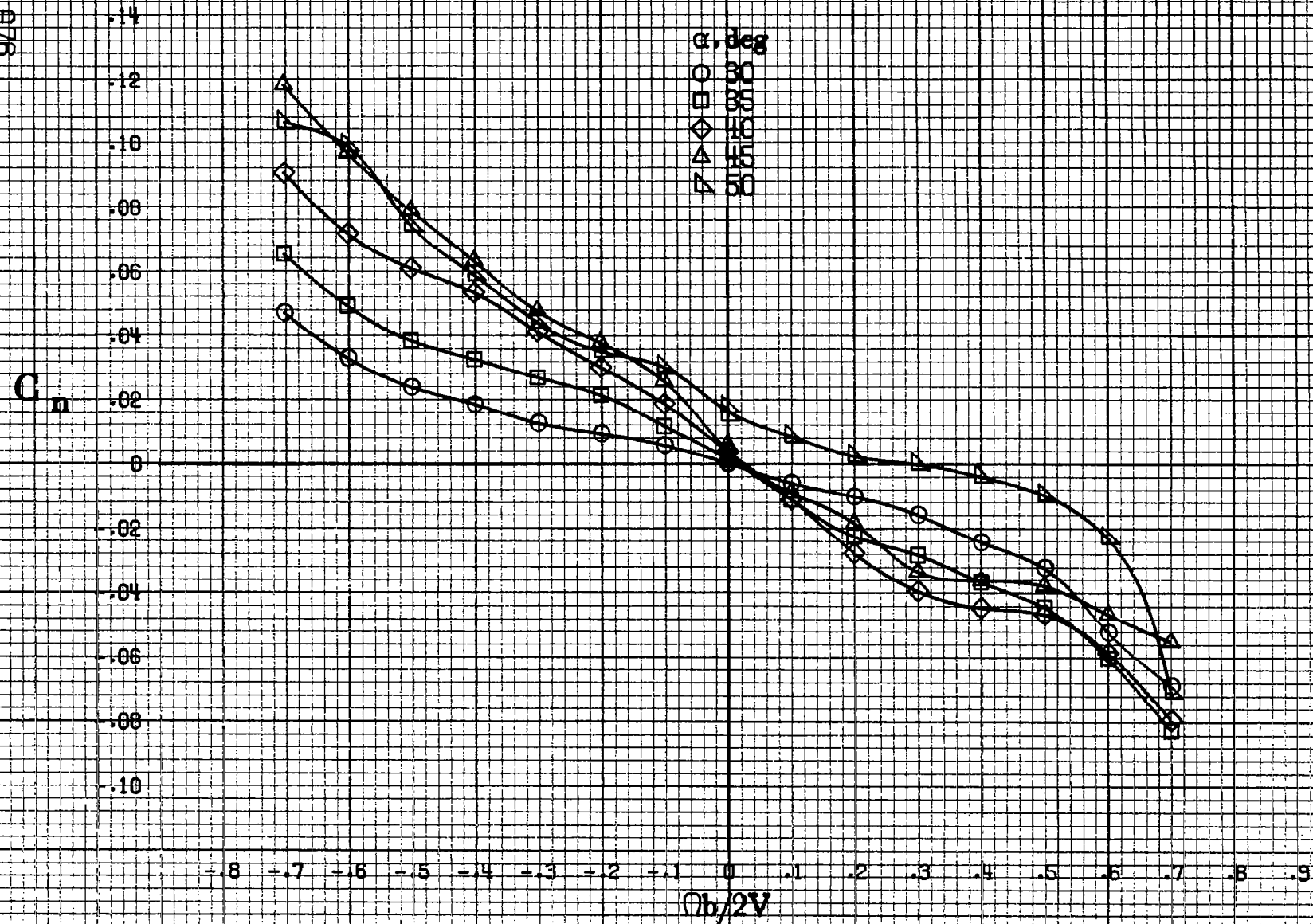
(c) \alpha=30 to 50 deg, SR=0 . Figure A19.-Continued.
