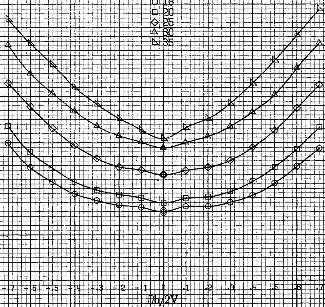
(b) \alpha = 18 to 35 deg, SR = 182.9 cm (72 in). Figure A22.-Continued.
