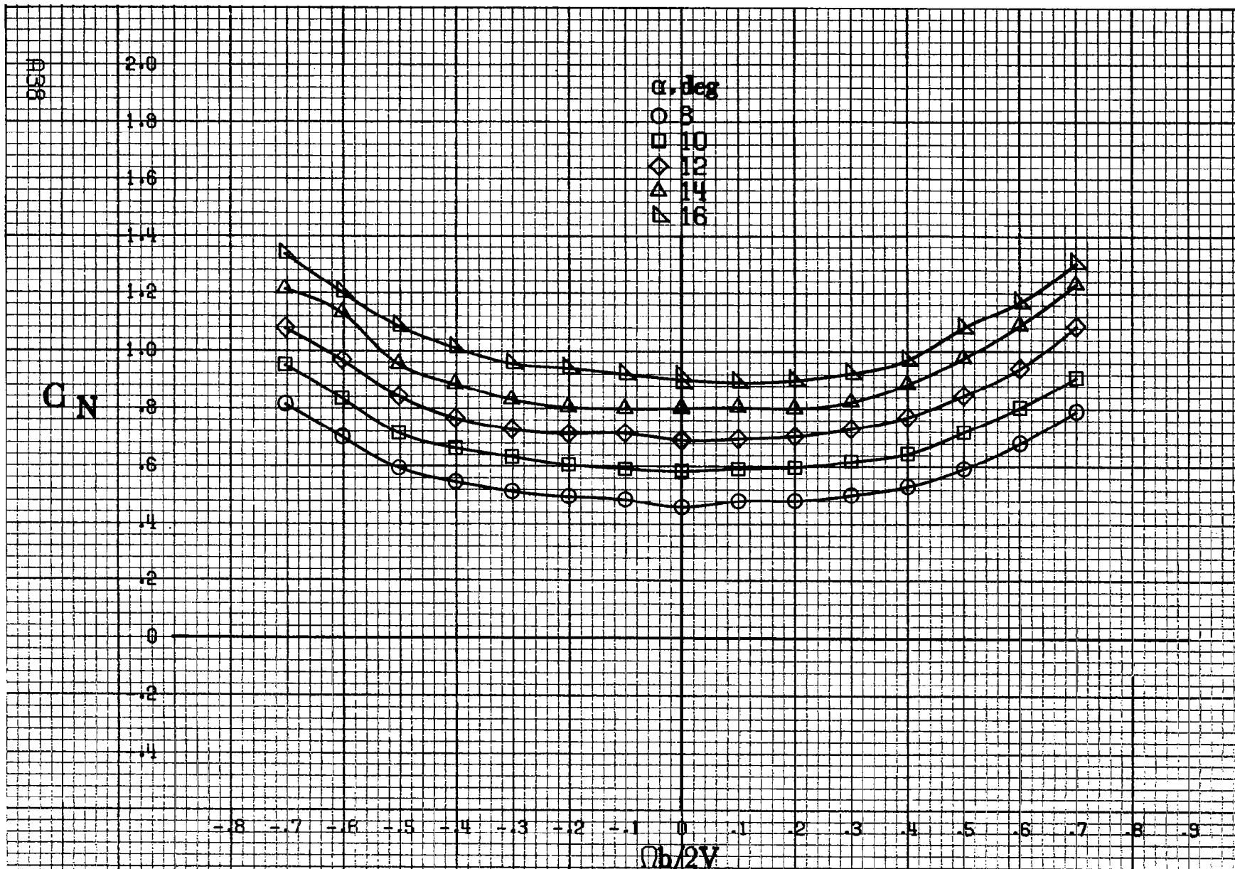
Figure A.10 - Effect of rotation rate and angle of attack on normal-force coefficient for body wing configuration. \delta_e = 0^\circ , \delta_a = 0^\circ , \delta_r = 0^\circ , \delta = 0^\circ .
