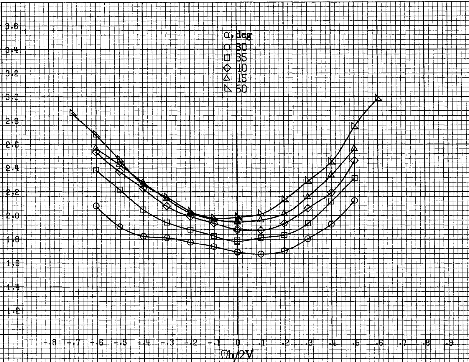
(c) \alpha=30 to 50 deg, SR=0 . Figure A34.-Continued.
