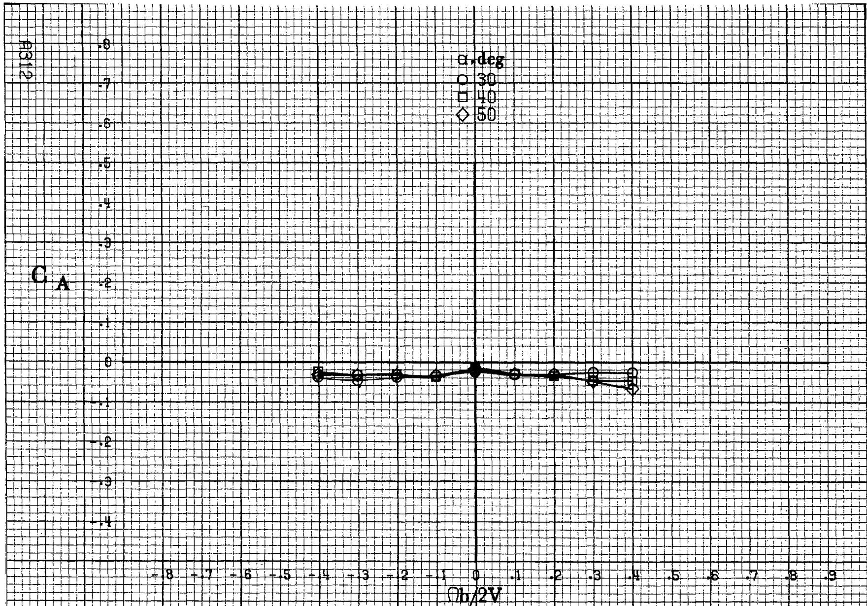
Figure A.90.- Effect of rotation rate and angle of attack on axial-force coefficient for basic configuration. \delta_c = 0^\circ , \delta_a = 20.0^\circ , \delta_d = 6^\circ , \delta_r = 0^\circ , \beta = 10^\circ .
