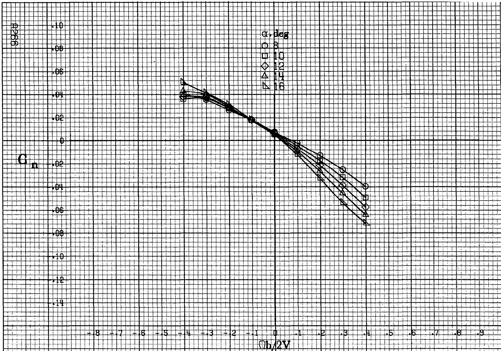
Figure A73.- Effect of rotation rate and angle of attack on yawing-moment coefficient for basic configuration. \delta_e = 0^\circ , \delta_s = 0^\circ , \delta_a = 11^\circ , \delta_r = 0^\circ . B = 10^\circ .
