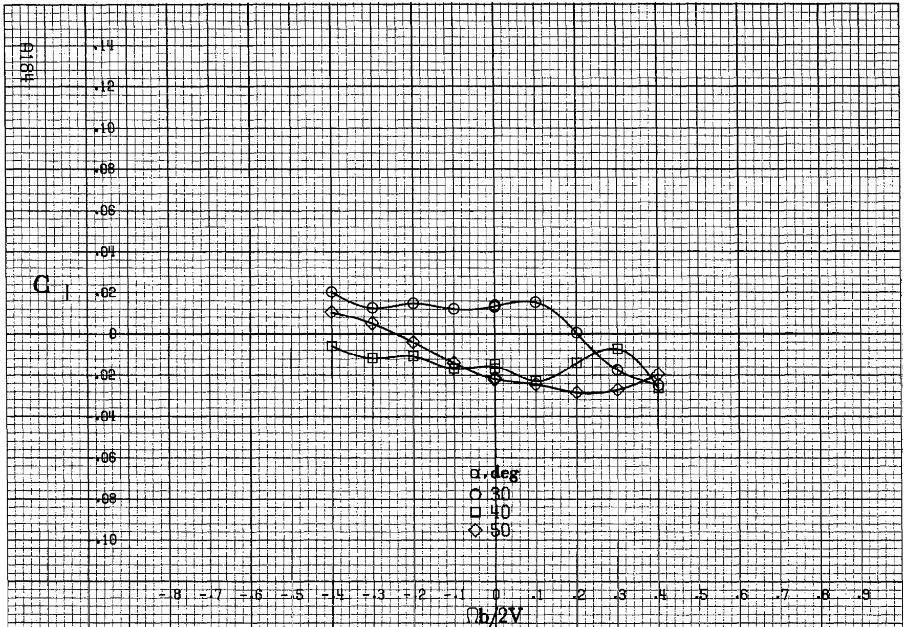
Figure A 50. - Effect of rotation rate and angle of attack on rolling-moment coefficient for basic configuration. \delta_e = -25^\circ , \delta_a = 0^\circ , \delta_c = 0^\circ , \delta_r = 0^\circ , \beta = 10^\circ .
