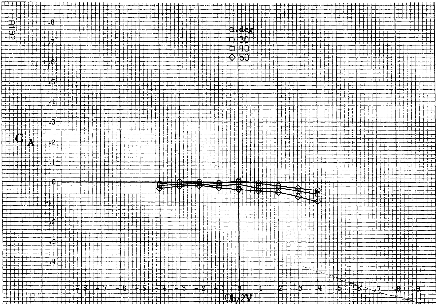
Figure A.54 - Effect of rotation rate and angle of attack on axial-force coefficient for basic configuration. \delta_e = -25^\circ , \delta_s = 0^\circ , \delta_a = 0^\circ , \delta_r = 0^\circ , \beta = 10^\circ .
