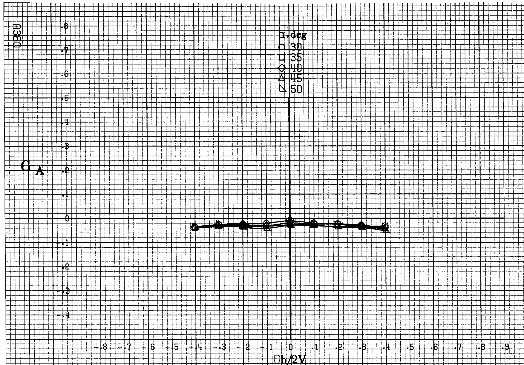
Figure A114.-Effect of rotation rate and angle of attack on axial-force coefficient for basic configuration. \delta_c = 0^\circ , \delta_s = -20.0^\circ , \delta_a = -6^\circ , \delta_r = 30^\circ , \beta = 10^\circ
