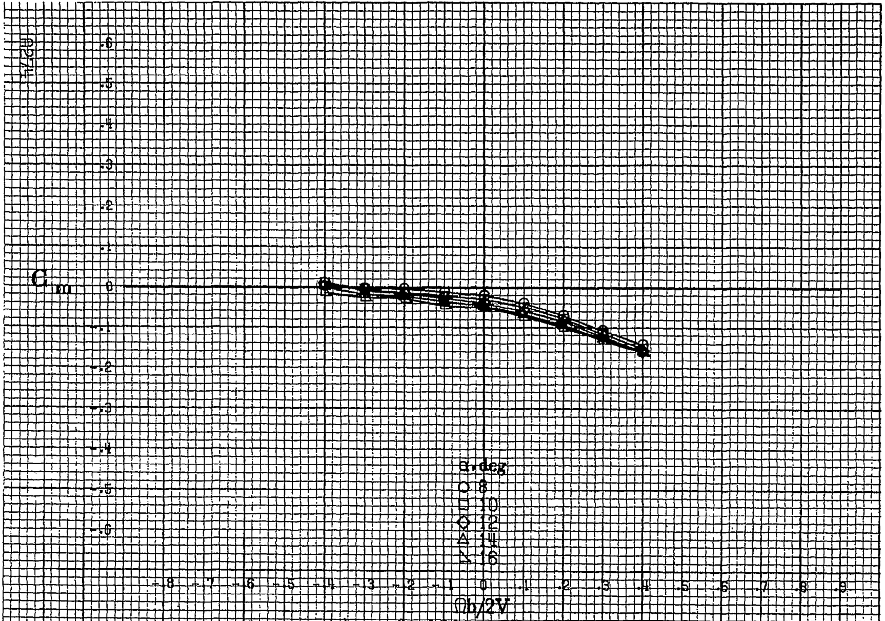
Figure A.75.- Effect of rotation rate and angle of attack on pitching-moment coefficient for basic configuration. \delta_a = 0^\circ , \delta_s = 0^\circ , \delta_a = 11^\circ , \delta_r = 0^\circ , \beta = 0^\circ .
