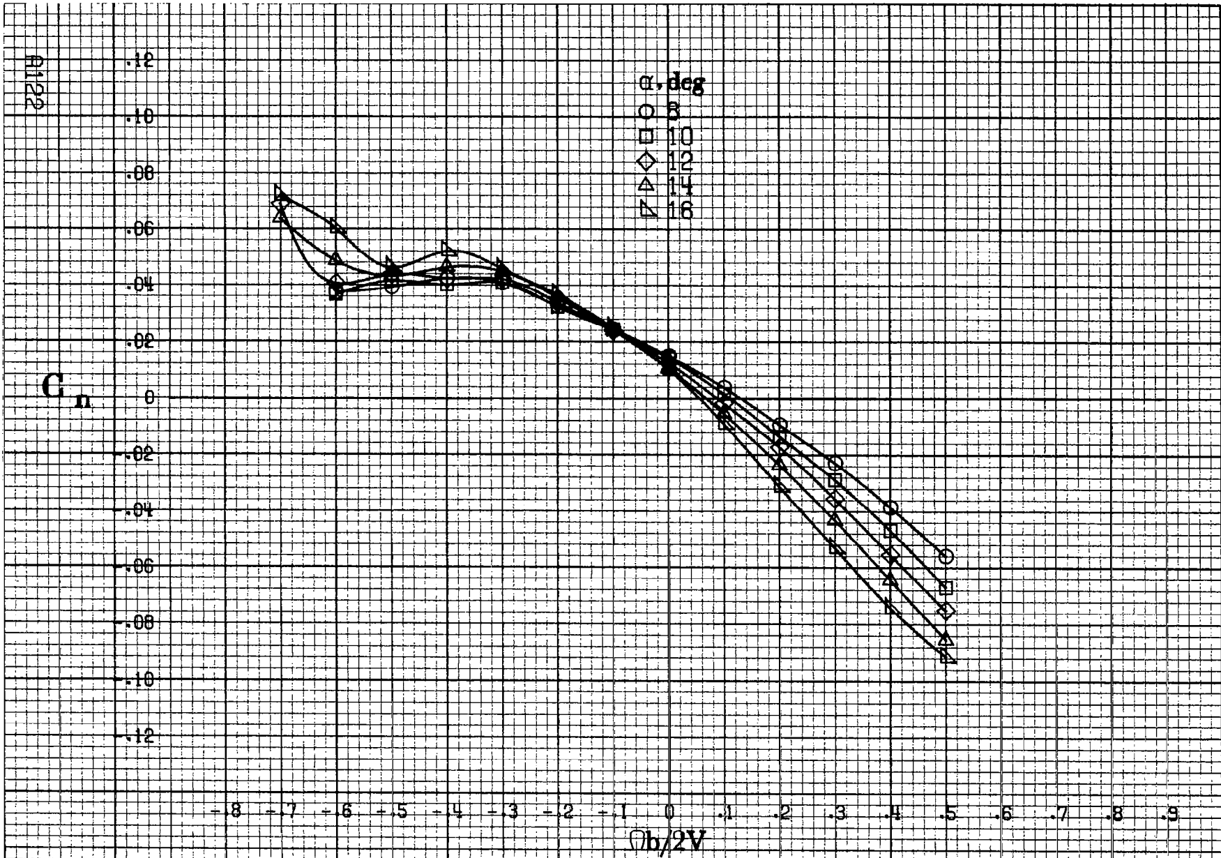
Figure A31.- Effect of rotation rate and angle of attack on yawing-moment coefficient for basic configuration. \delta_c = 0^\circ , \delta_a = 0^\circ , \delta_d = 0^\circ , \delta_r = 0^\circ , \beta = 10^\circ .
