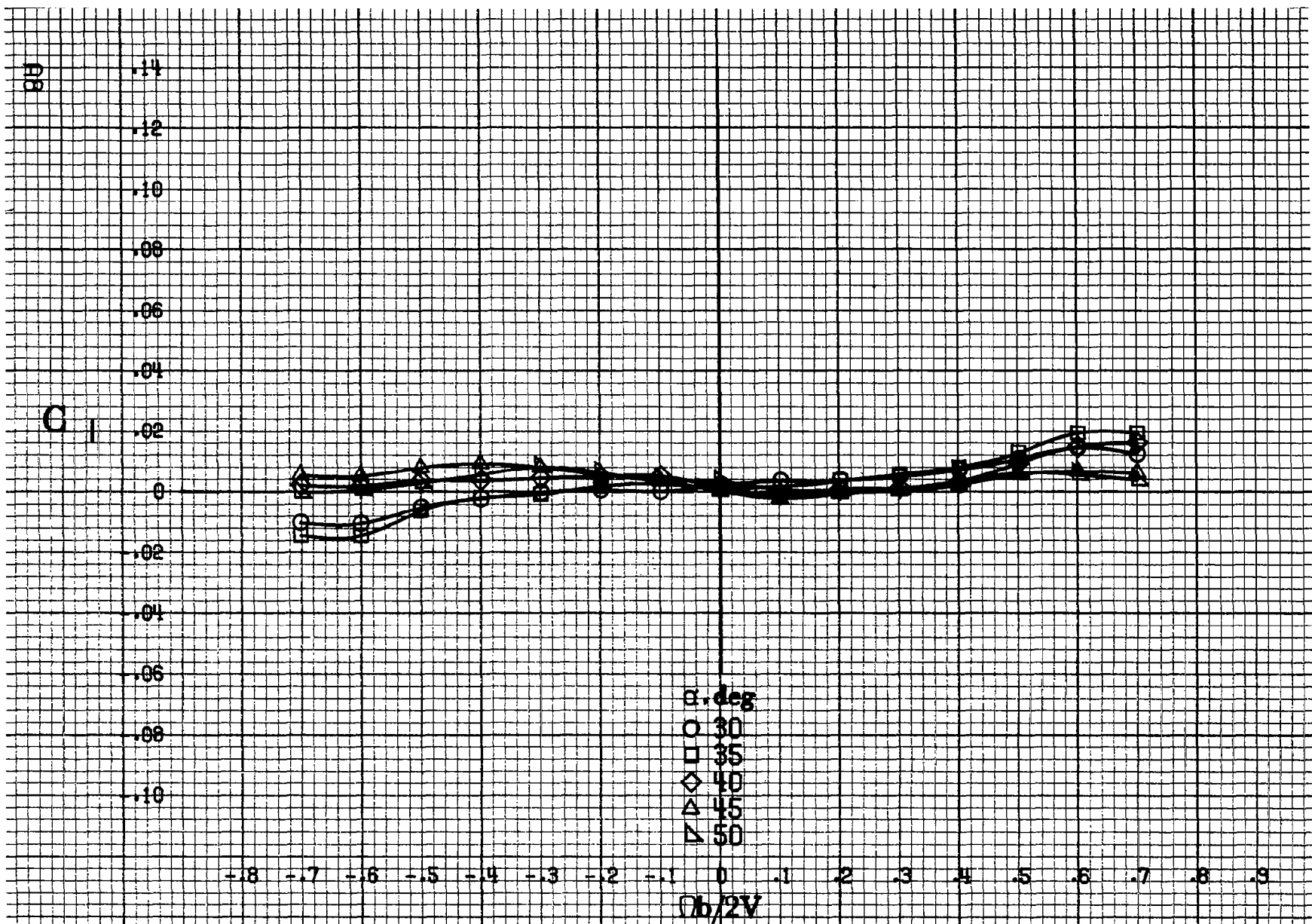
(c) \alpha = 30 to 50 deg, SR = 0 . Figure A2.-Continued.
