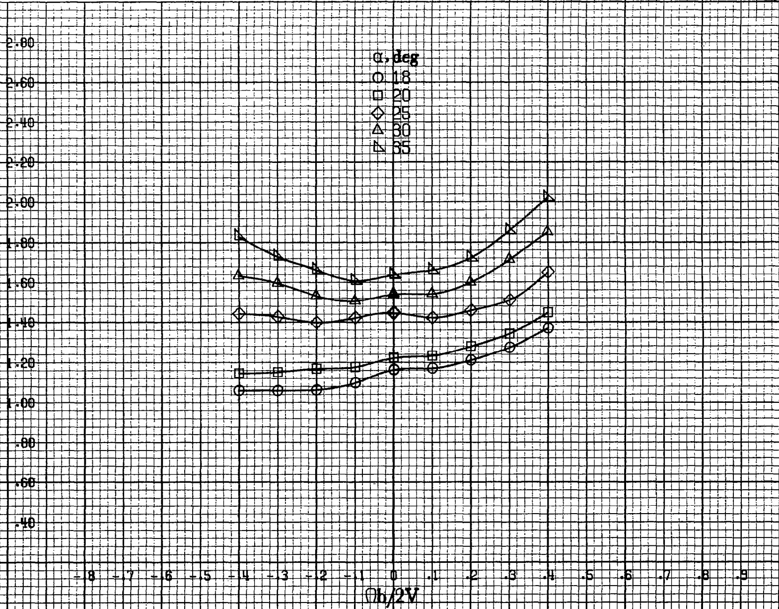
(b) \alpha = 18 to 35 deg. SR = 182.9 cm (72 in). Figure A76.-Continued.
