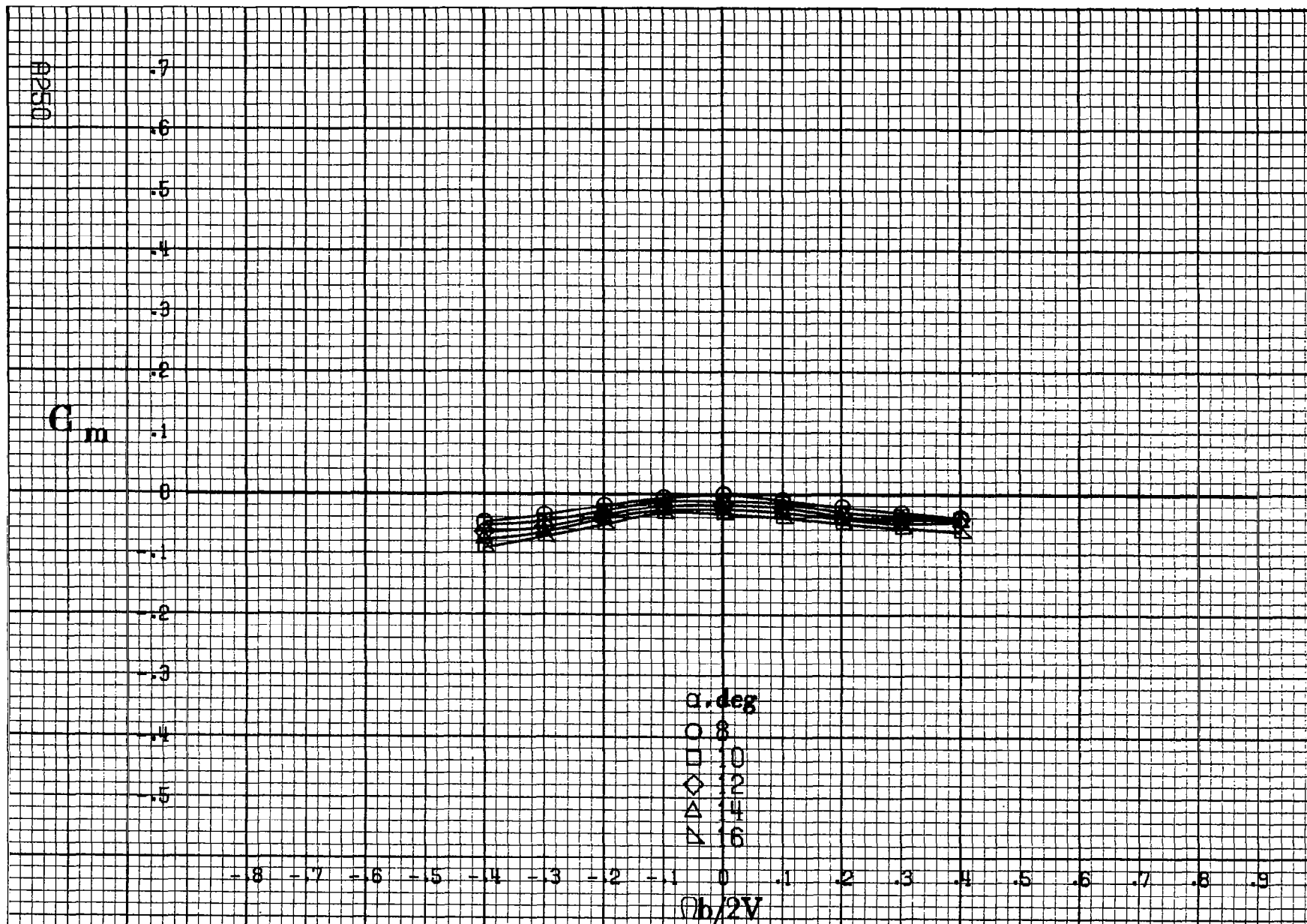
Figure A69.-Effect of rotation rate and angle of attack on pitching-moment coefficient for basic configuration. \delta_c = 0^\circ , \delta_s = 0^\circ , \delta_d = 11^\circ , \delta_r = 0^\circ , \beta = 0^\circ .
