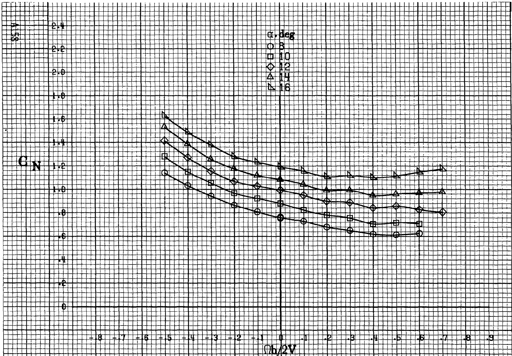
Figure A40 - Effect of rotation rate and angle of attack on normal-force coefficient for basic configuration. \delta_e = 0^\circ , \delta_a = 0^\circ , \delta_d = 0^\circ , \delta_r = 0^\circ , B = -10^\circ .
