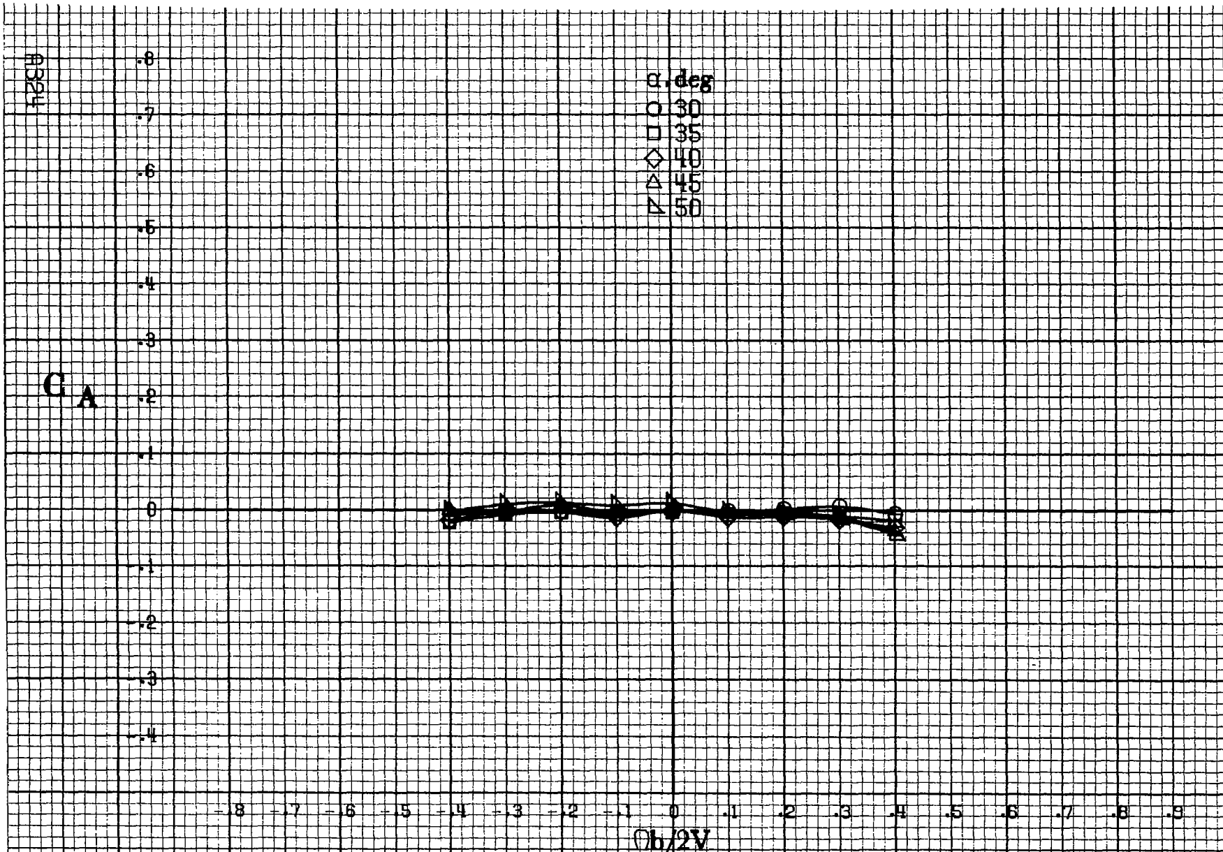
Figure A96.-Effect of rotation rate and angle of attack on axial-force coefficient for basic configuration. \delta_c=0^\circ , \delta_s=20.0^\circ , \delta_a=6^\circ , \delta_r=-15^\circ , \beta=0^\circ .
