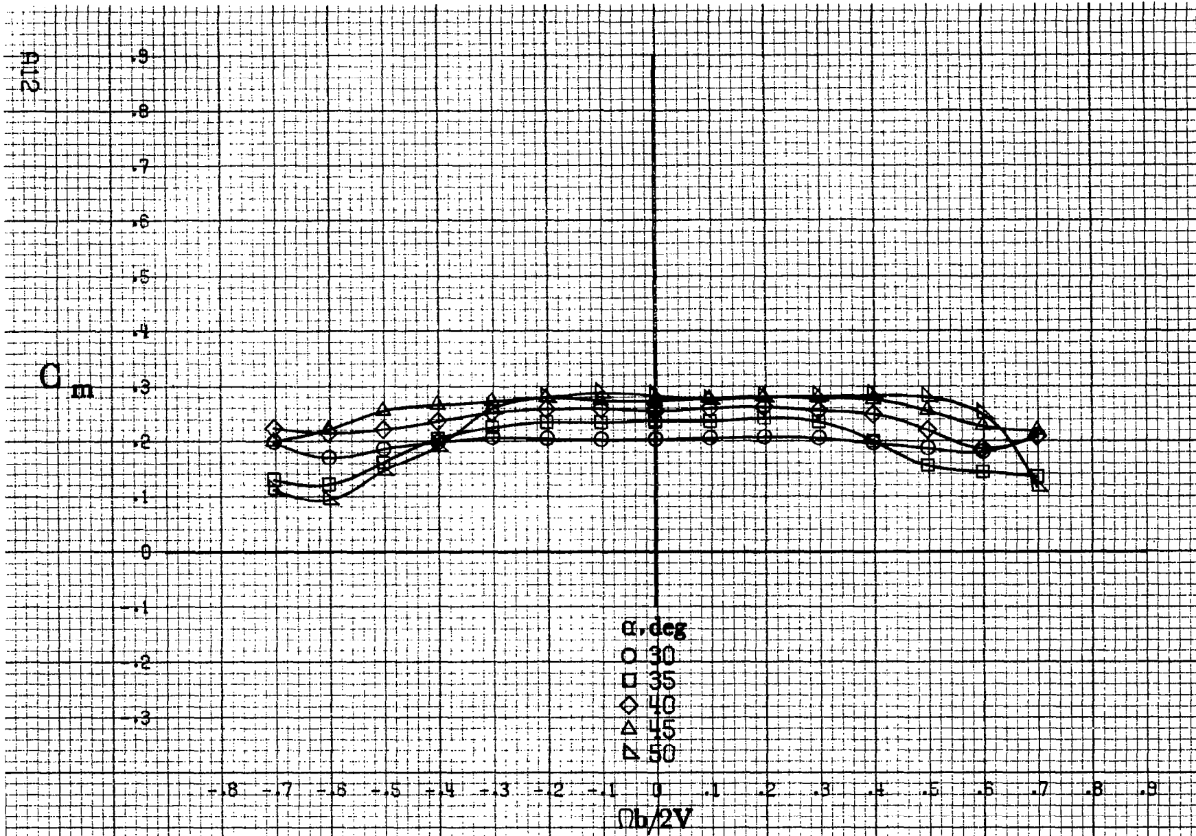
(c) \alpha=30 to 50 deg, SR=0 . Figure A3.-Continued.
