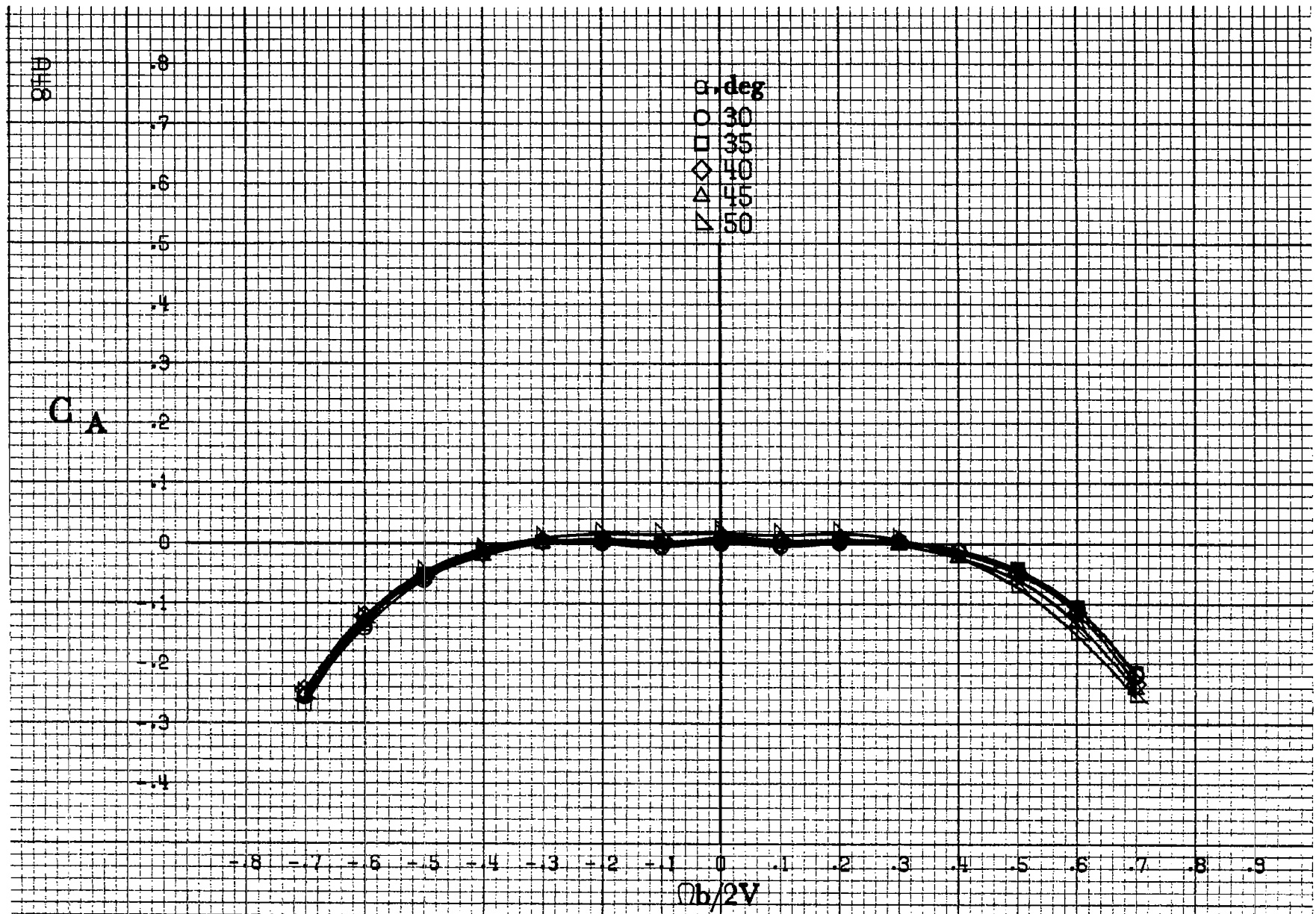
(c) \alpha = 30 to 50 deg, SR = 0 . Figure A12.-Continued.
