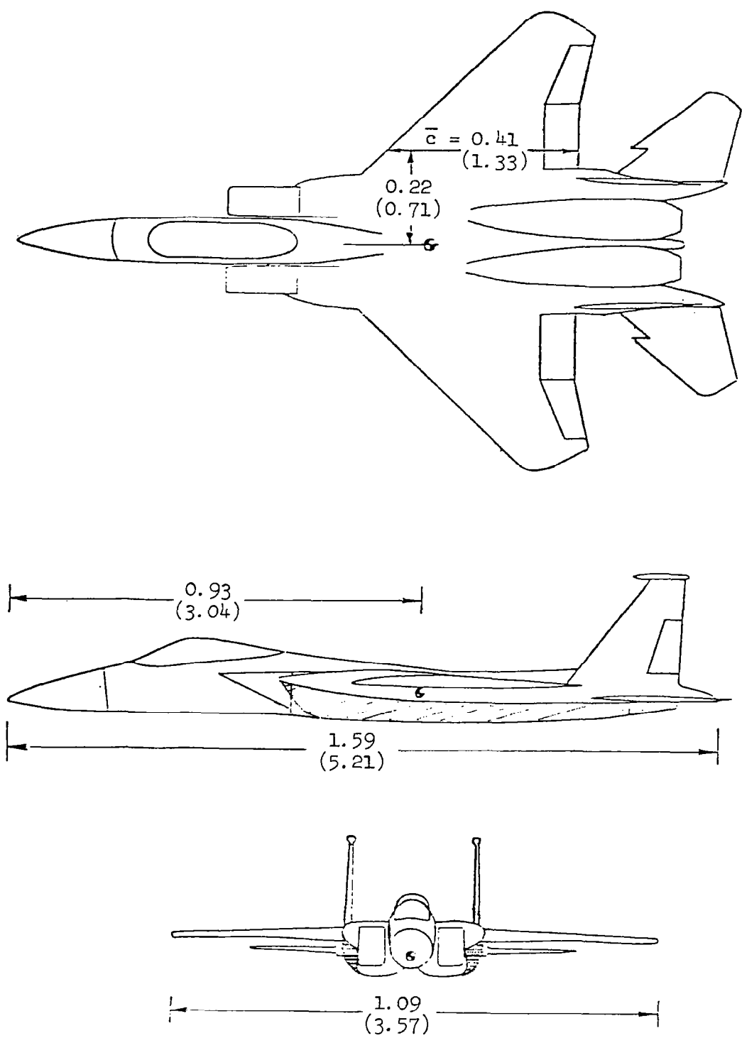
Figure 3.- Three-view sketch of 1/12-scale model. Dimensions are given in meters(feet).
