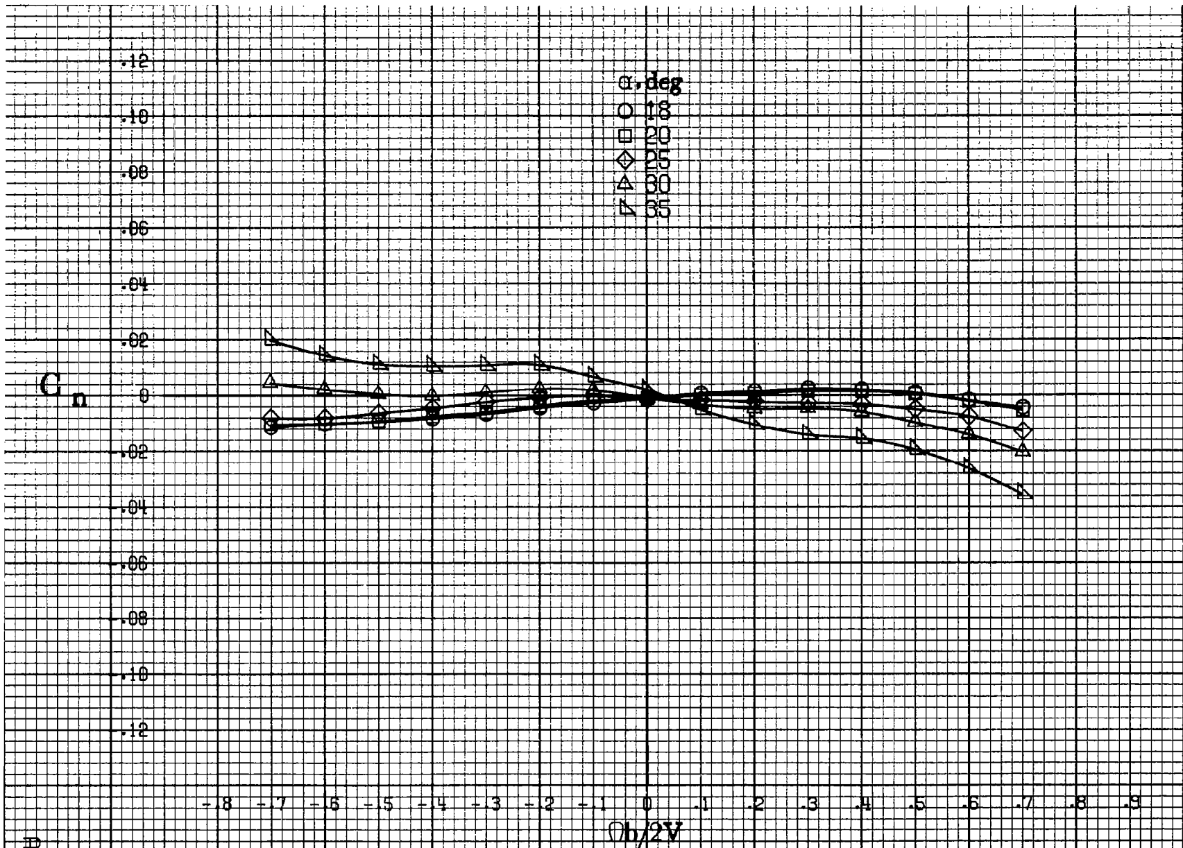
(b) \alpha = 18 to 35 deg, SR = 182.9 cm (72 in). Figure A19.-Continued.
