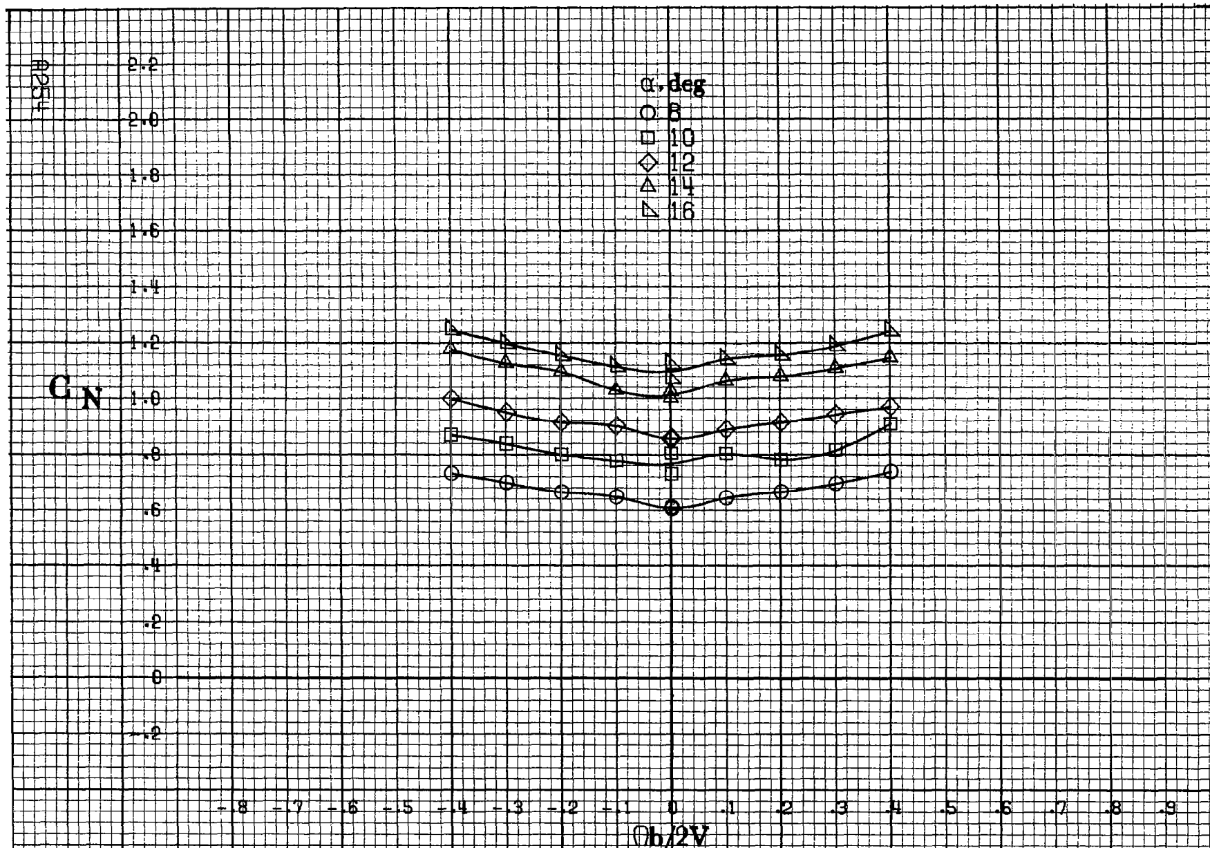
Figure A70.-Effect of rotation rate and angle of attack on normal-force coefficient for basic configuration. \delta_c = 0^\circ , \delta_a = 0^\circ , \delta\alpha = 11^\circ , \delta_r = 0^\circ , \beta = 0^\circ .
