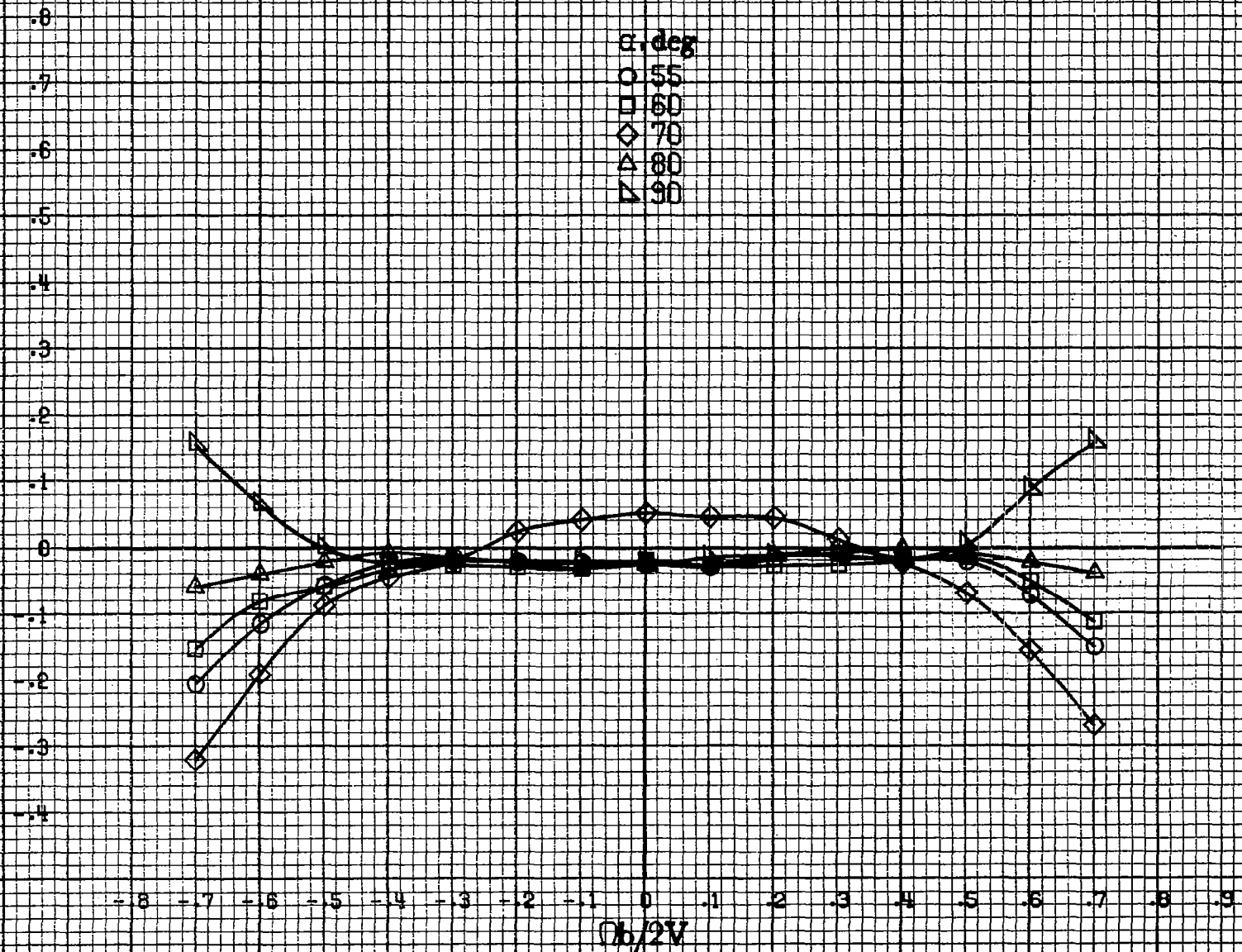
(d) \alpha = 55 to 90 deg, SR = 0 . Figure A6.-Concluded.
