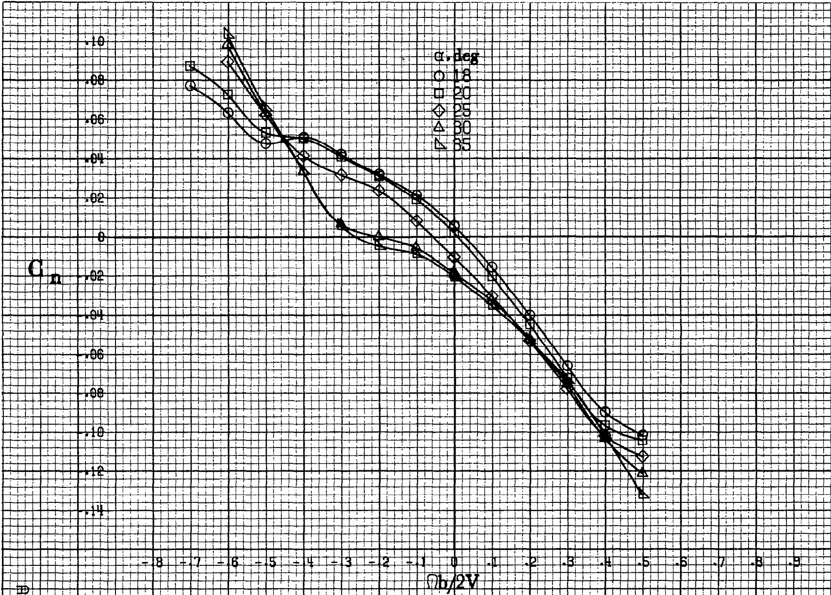
(b) \alpha = 18 to 35 deg. SR = 182.9 cm (72 in). Figure A61. - Continued.
