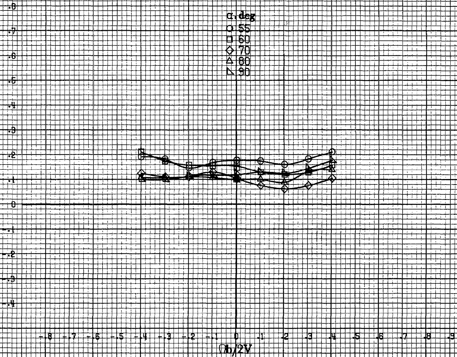
(b) \alpha = 55 to 90 deg, SR = 0 . Figure A 47.- Concluded.
