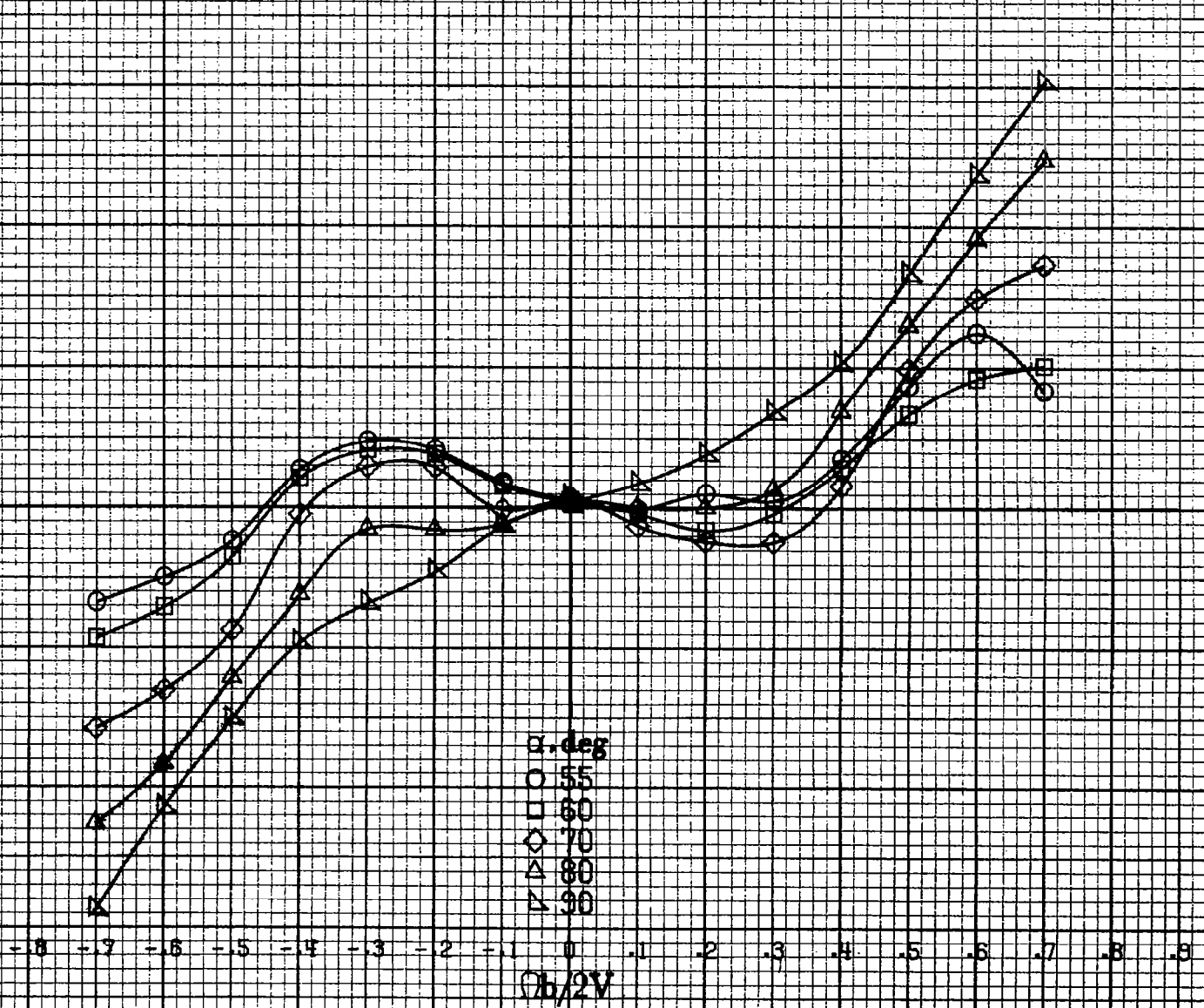
(d) \alpha=55 to 90 deg, SR=0 . Figure A56.- Concluded.
