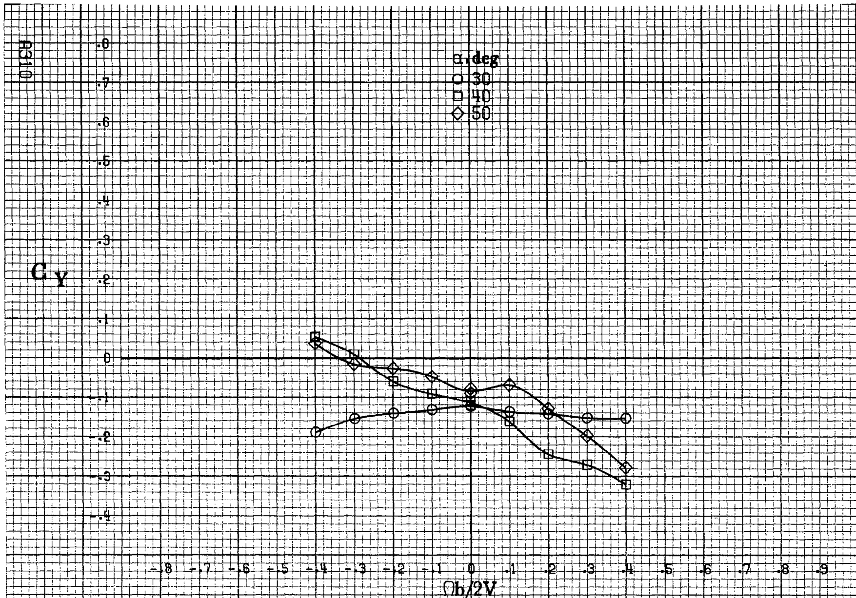
Figure A 89.- Effect of rotation rate and angle of attack on side-force coefficient for basic configuration. \delta_e = 0^\circ , \delta_s = 20.0^\circ , \delta_d = 6^\circ , \delta_r = 0^\circ , \beta = 10^\circ .
