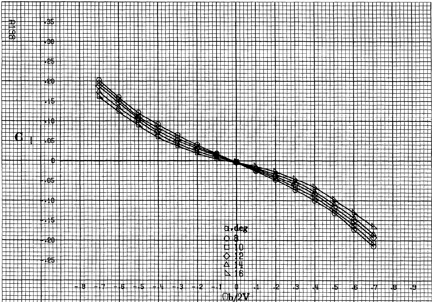
Figure A56.-Effect of rotation rate and angle of attack on rolling-moment coefficient for basic configuration. \delta_e = 0^\circ , \delta_a = 0^\circ , \delta_a = 6^\circ , \delta_r = 0^\circ , \beta = 0^\circ .
