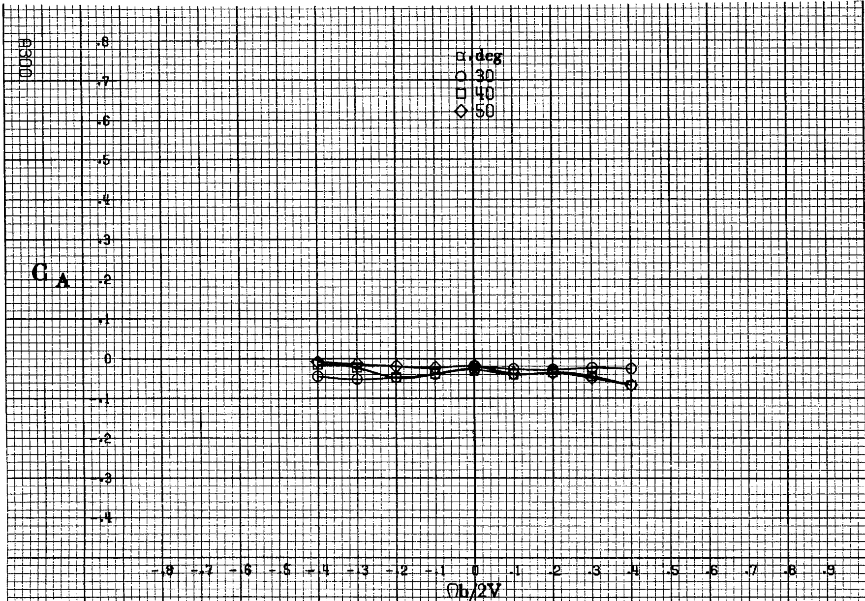
Figure A84 - Effect of rotation rate and angle of attack on axial-force coefficient for basic configuration. \delta_e = 0^\circ , \delta_s = 20.0^\circ , \delta_a = 6^\circ , \delta_r = 0^\circ , \beta = 0^\circ .
