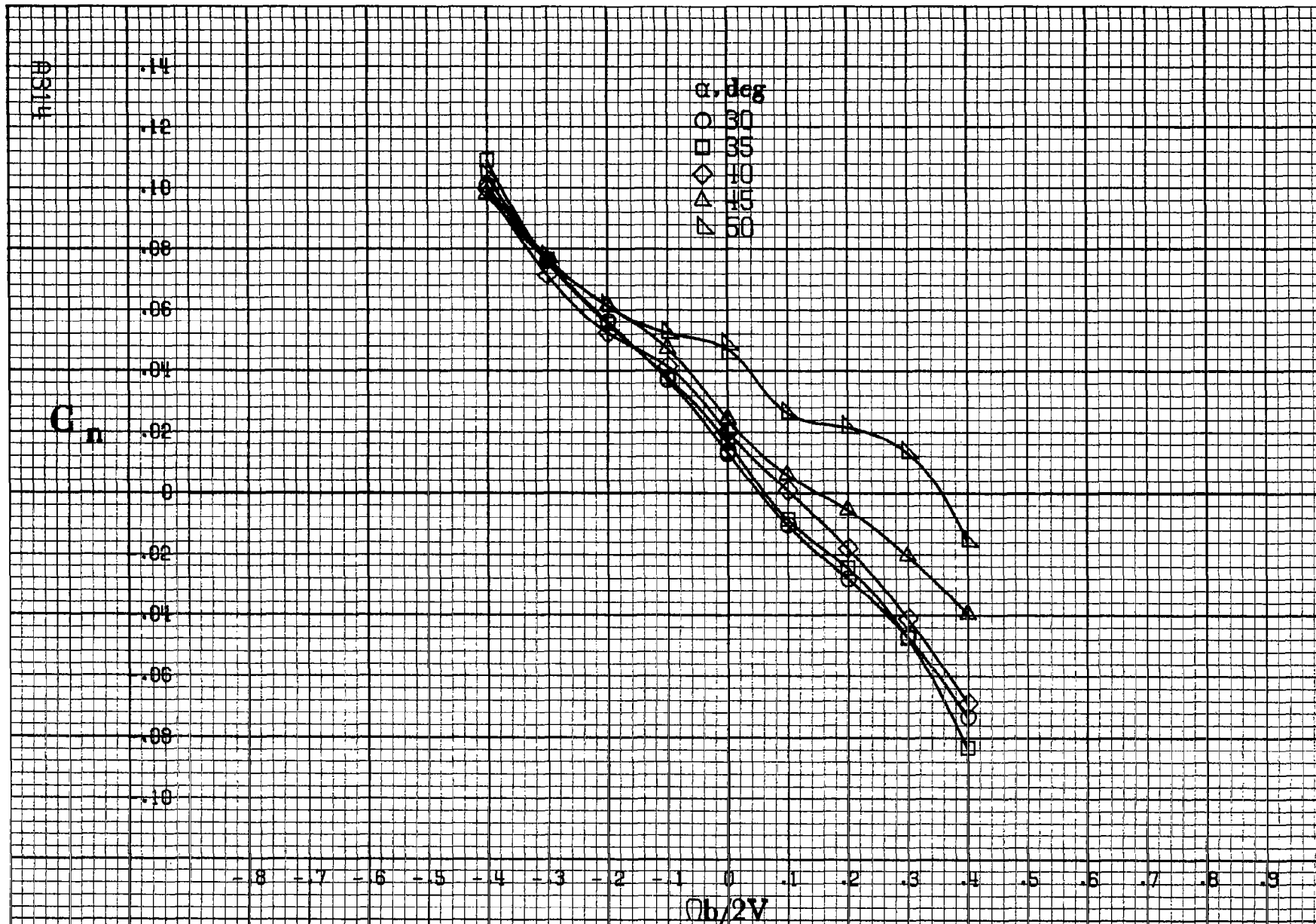
Figure A91.- Effect of rotation rate and angle of attack on yawing-moment coefficient for basic configuration. \delta_e = 0^\circ , \delta_a = 20.0^\circ , \delta_d = 6^\circ , \delta_r = -15^\circ , \beta = 0^\circ .
