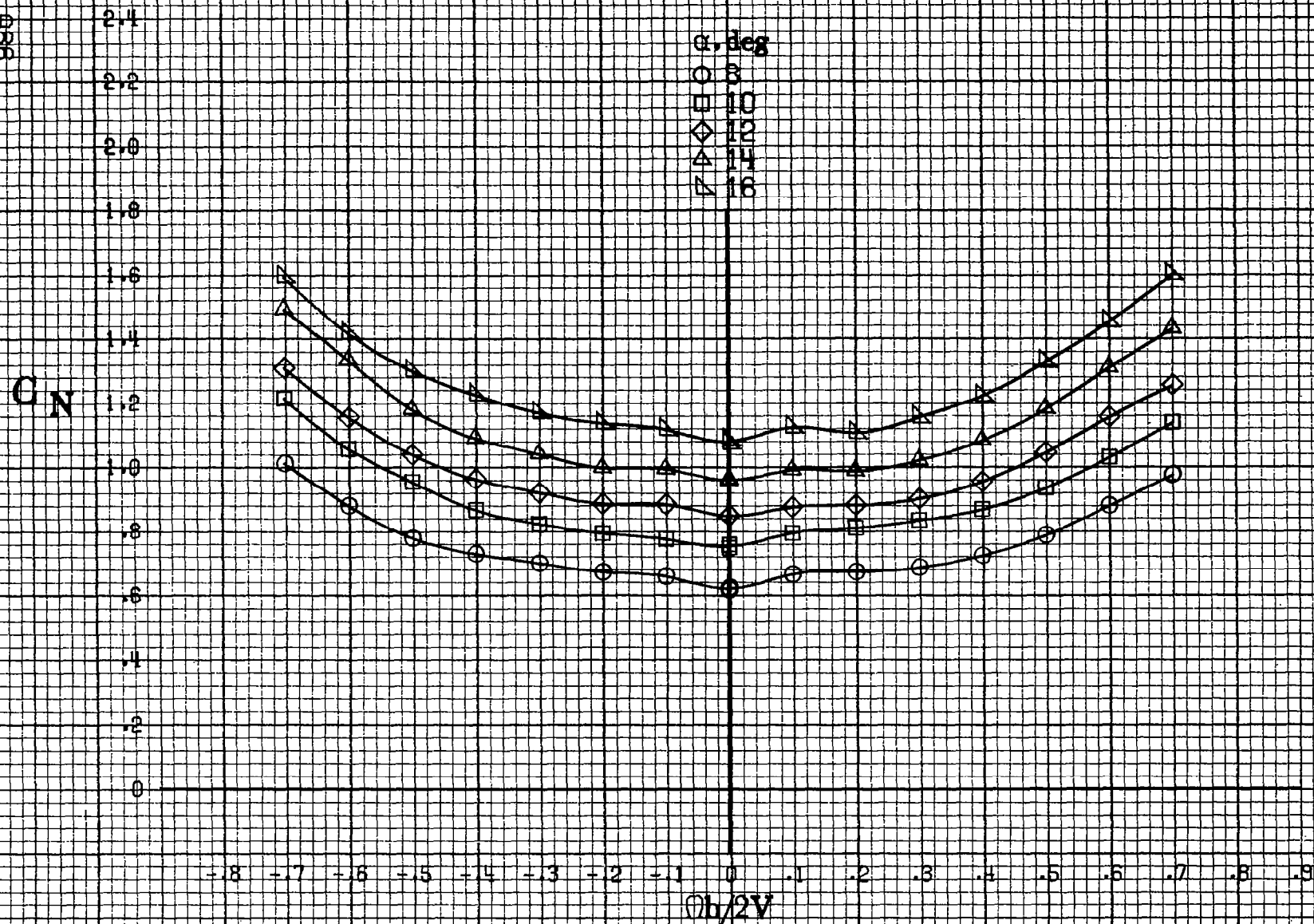
Figure A22.-Effect of rotation rate and angle of attack on normal-force coefficient for body wing horizontal tail configuration. \delta_c = 0^\circ , \delta_s = 0^\circ , \delta_r = 0^\circ , \beta = 0^\circ .
