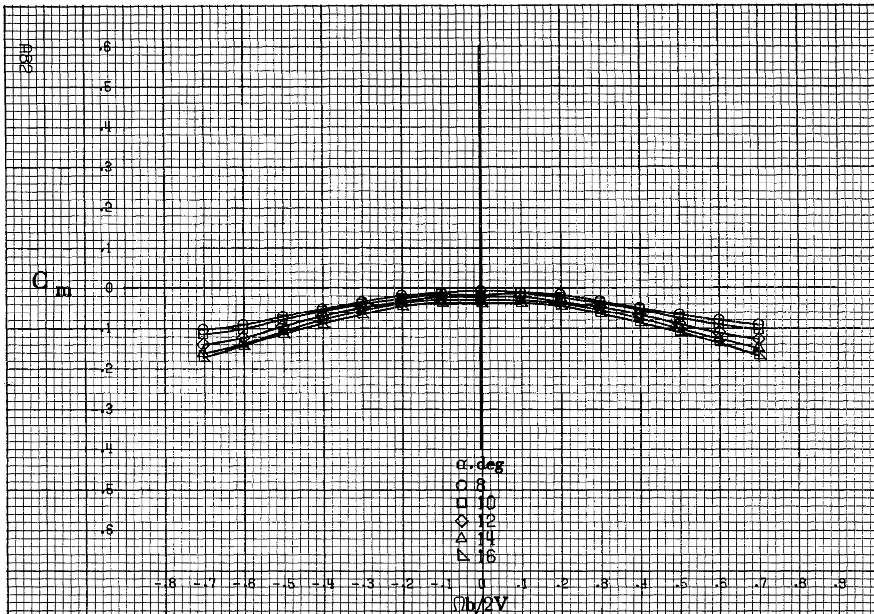
Figure A21.- Effect of rotation rate and angle of attack on pitching-moment coefficient for body wing horizontal tail configuration. \delta_a = 0^\circ , \delta_s = 0^\circ , \delta_r = 0^\circ , \beta = 0^\circ .
