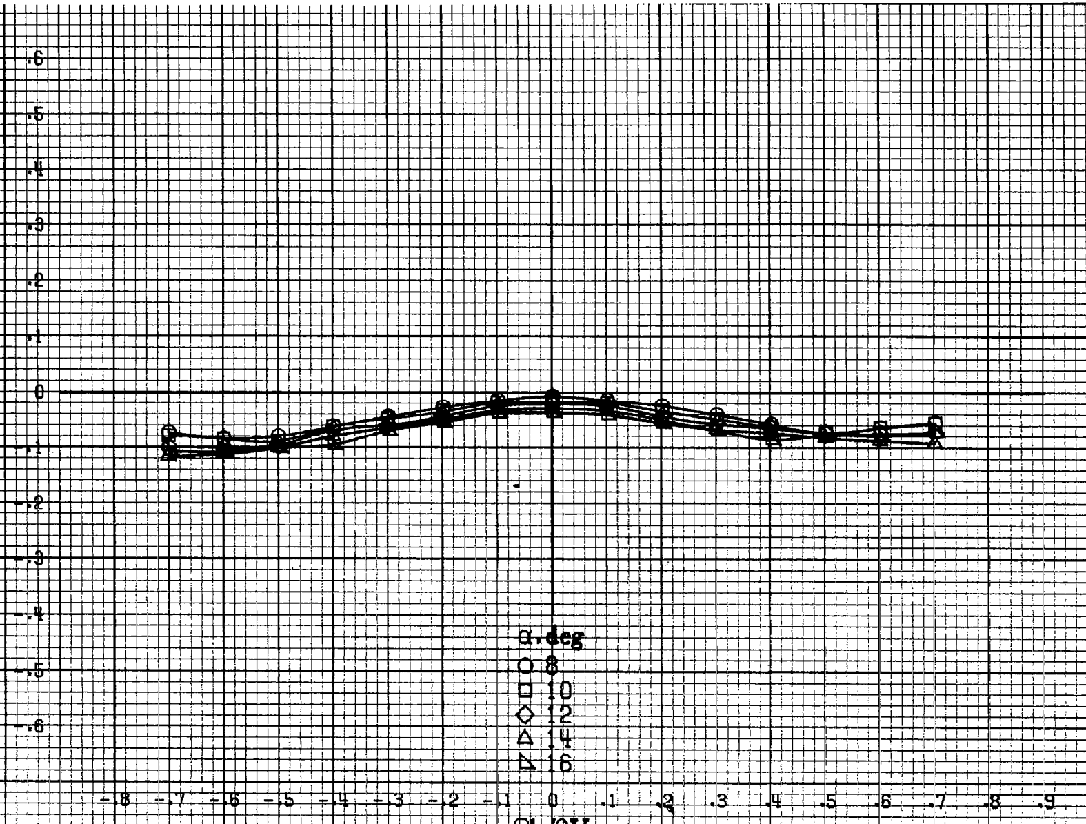
Figure A57.-Effect of rotation rate and angle of attack on pitching-moment coefficient for basic configuration. \delta_r = 0^\circ , \delta_a = 0^\circ , \delta_a = 6^\circ , \delta_r = 0^\circ , \beta = 0^\circ .
