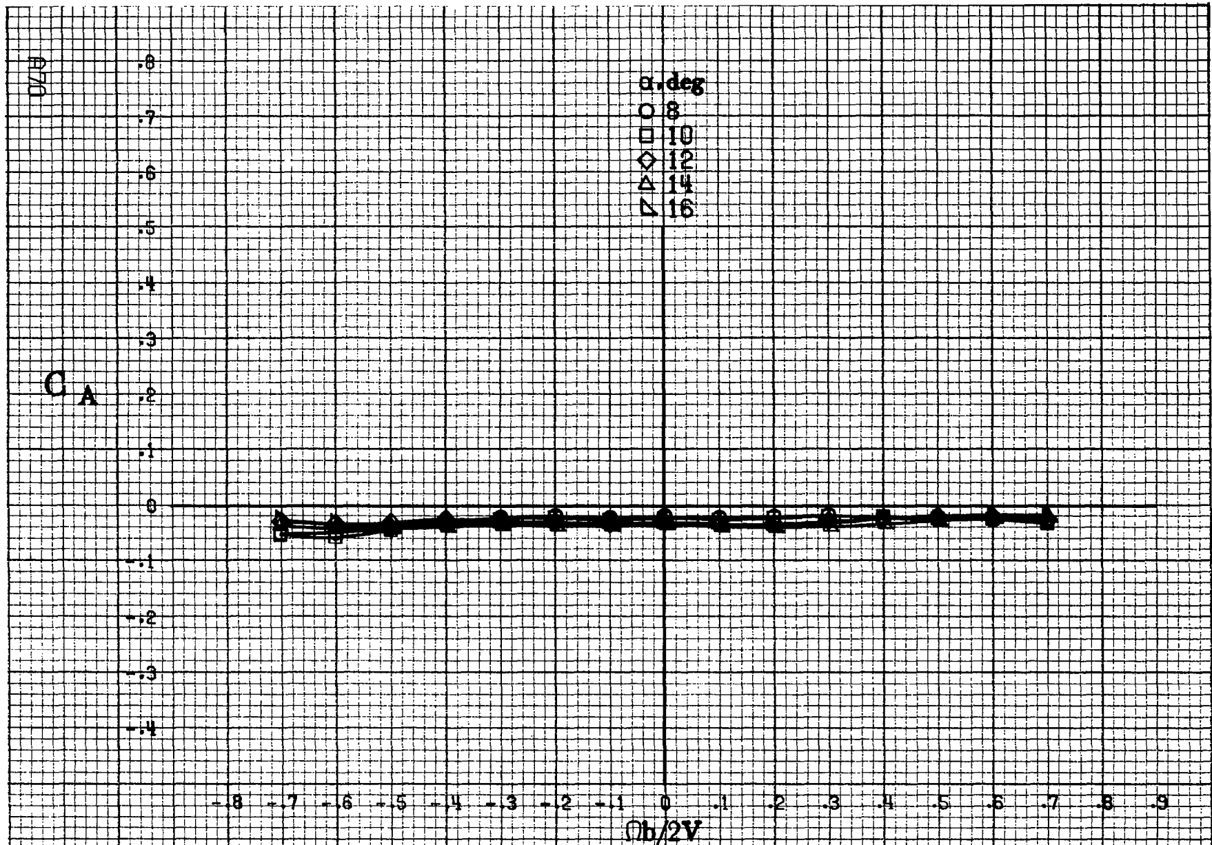
Figure A18 - Effect of rotation rate and angle of attack on axial-force coefficient for body wing vertical tail configuration. \delta_e = 0^\circ , \delta_a = 0^\circ , \delta_r = 0^\circ , \delta_l = 0^\circ .
