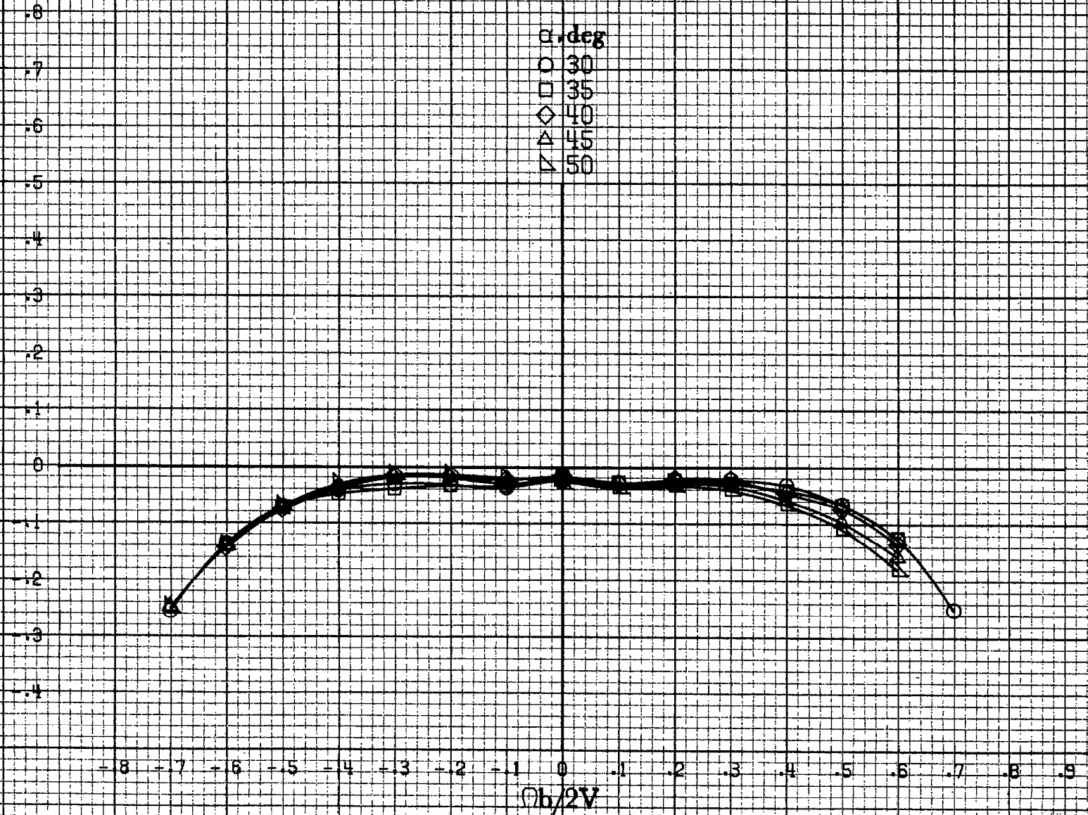
(c) \alpha=30 to 50 deg, SR=0 . Figure A 60.-Continued.
