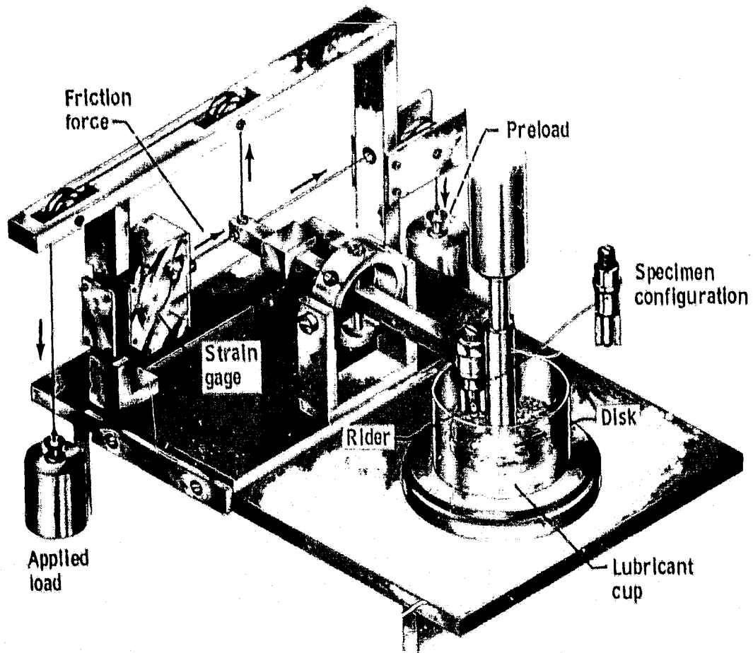
Figure 1. - Pin-on-disk sliding friction apparatus.
