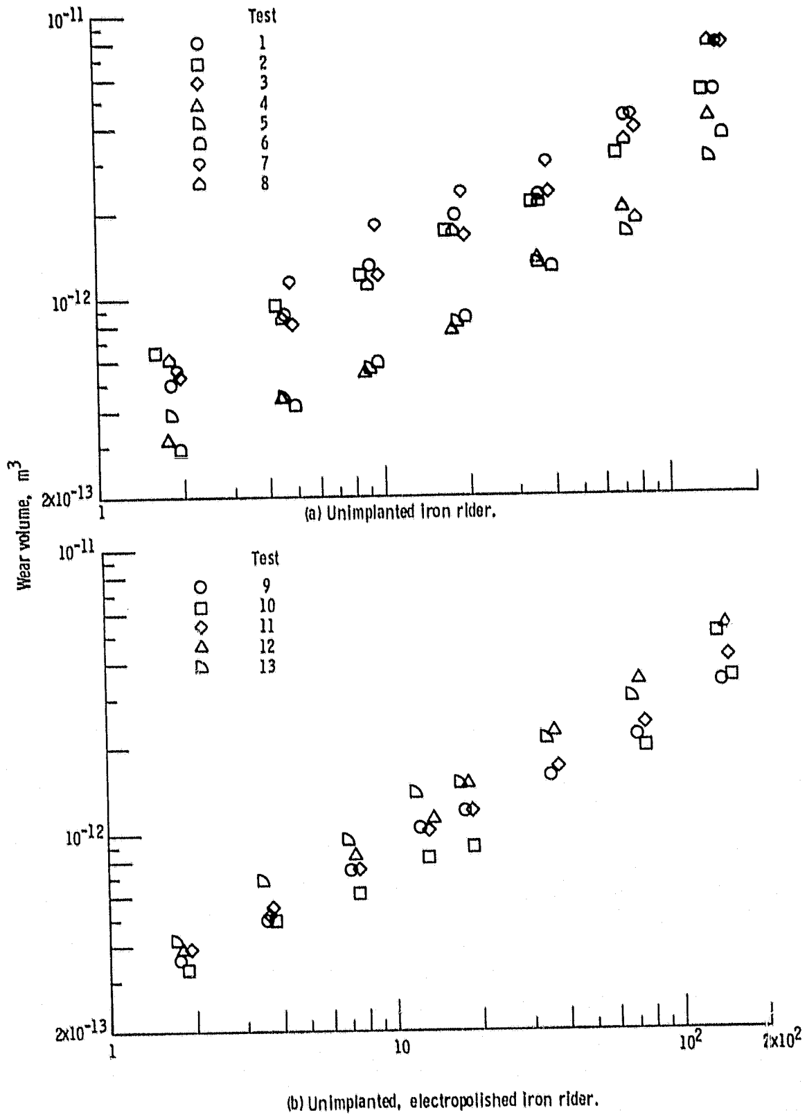
Figure 3. - Rider wear volume as a function of sliding distance. Load, 4.9 N; sliding velocity \sim 0.07 m/sec; lubricant, n-hexadecane; disk, unimplanted M-50 steel.
